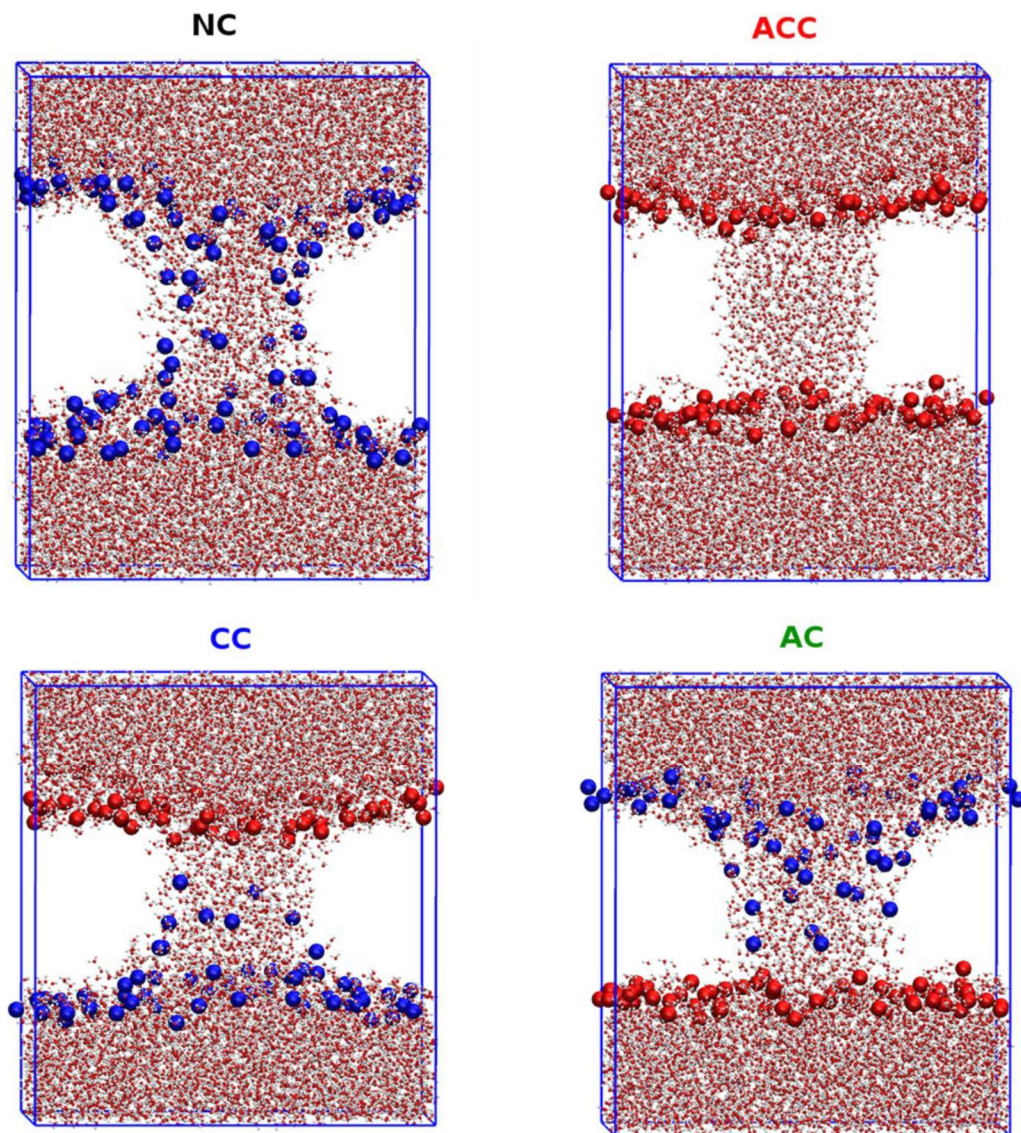
Figure 3. Mechanically constrained pores for ion transport studies [2]. NC – no constraint; ACC – anode and cathode sides constrained; CC – cathode side constrained; AC – anode side constrained.
