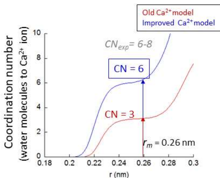
Figure 2. Calcium ion water coordination number for CHARMM36 systems containing either the ion model distributed with CHARMM36 (red line) or the modified ion model created in this work (blue line). Experimentally determined values are in the range 6 to 8.
