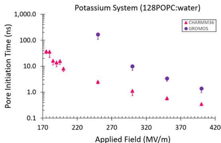
Figure 1. Pore initiation time as a function of applied electric field for GROMOS-OPLS and CHARMM36 systems containing potassium ions.
