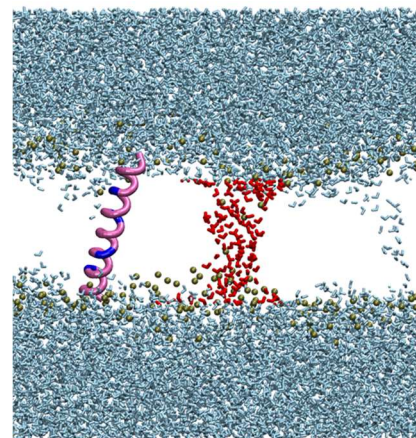
Figure 4. Lipid bilayer (POPC) with a transmembrane peptide, a lipid pore, and a water bridge.
