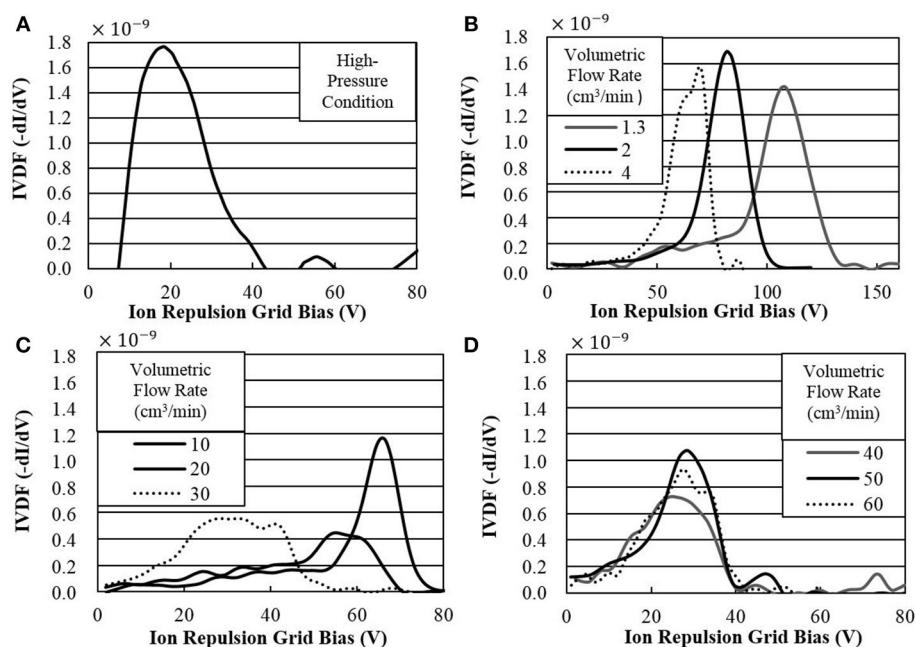
FIGURE 3 | IVDFs (uncorrected) measured at the exit plane for (A) “High-Pressure” condition and (B–D) “Low-Pressure” condition.
