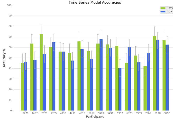
Figure 54. Overall model accuracy of the Time Series dataset.
