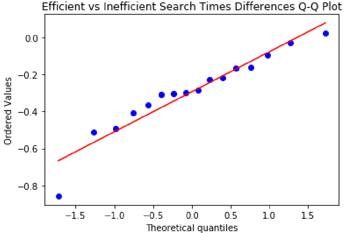
Figure 40. The assumption of normal distribution holds.
