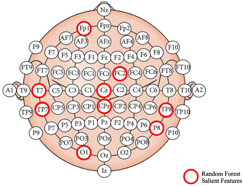
Figure 58. EEG Electrode Locations and Salient Features
