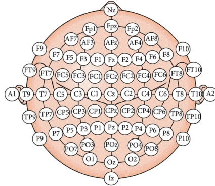
Figure 24. The International 10-20 Electrode Placement
