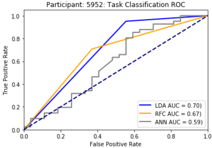
Figure 32. A ROC curve.
