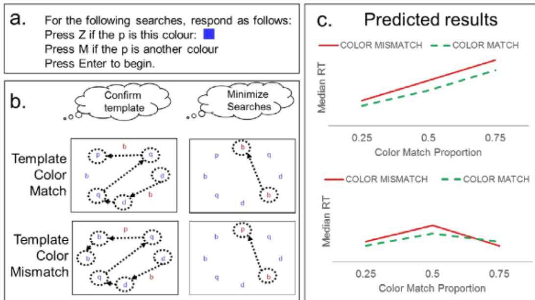
Figure 8. Rajsic's 2015 experiment. The instructions presented to the subject, along with a template color match and mismatch, and the predicted results can be seen.
