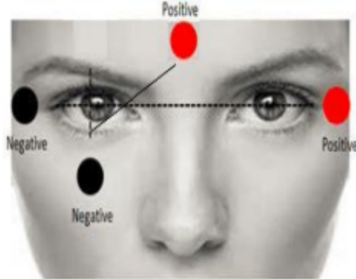
Figure 26. Vertical and Horizontal EOG Electrodes Placement
