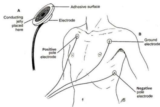
Figure 25. ECG Electrodes Placement
