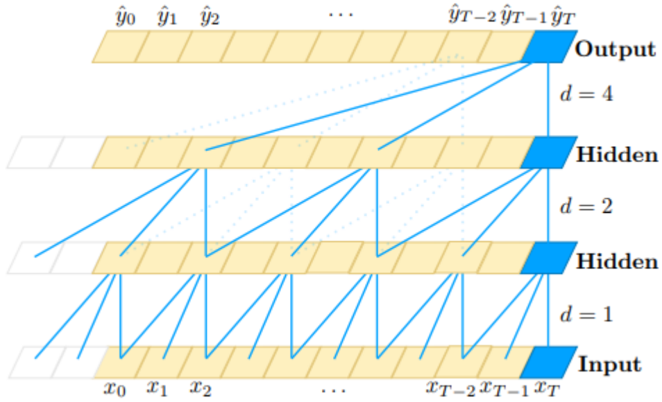
Figure 6. The architecture of a TCN.
