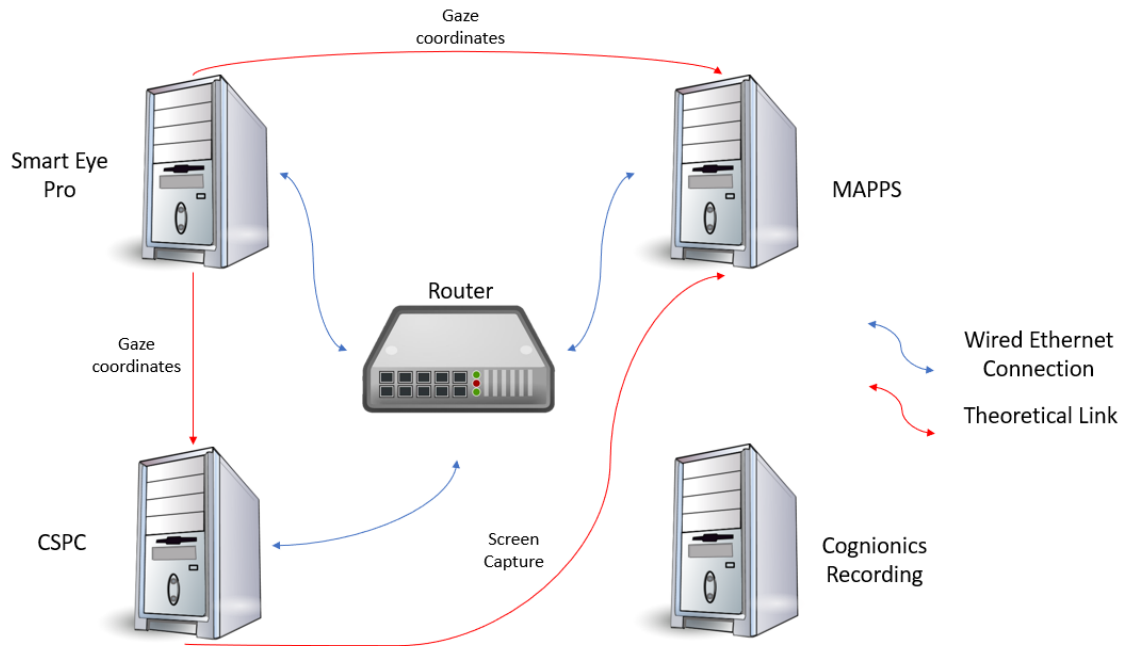
Figure 20. The layout of the computers used in the ESE. More information about the cognionics recording computer and its use can be seen in Section 3.4.7.1.
