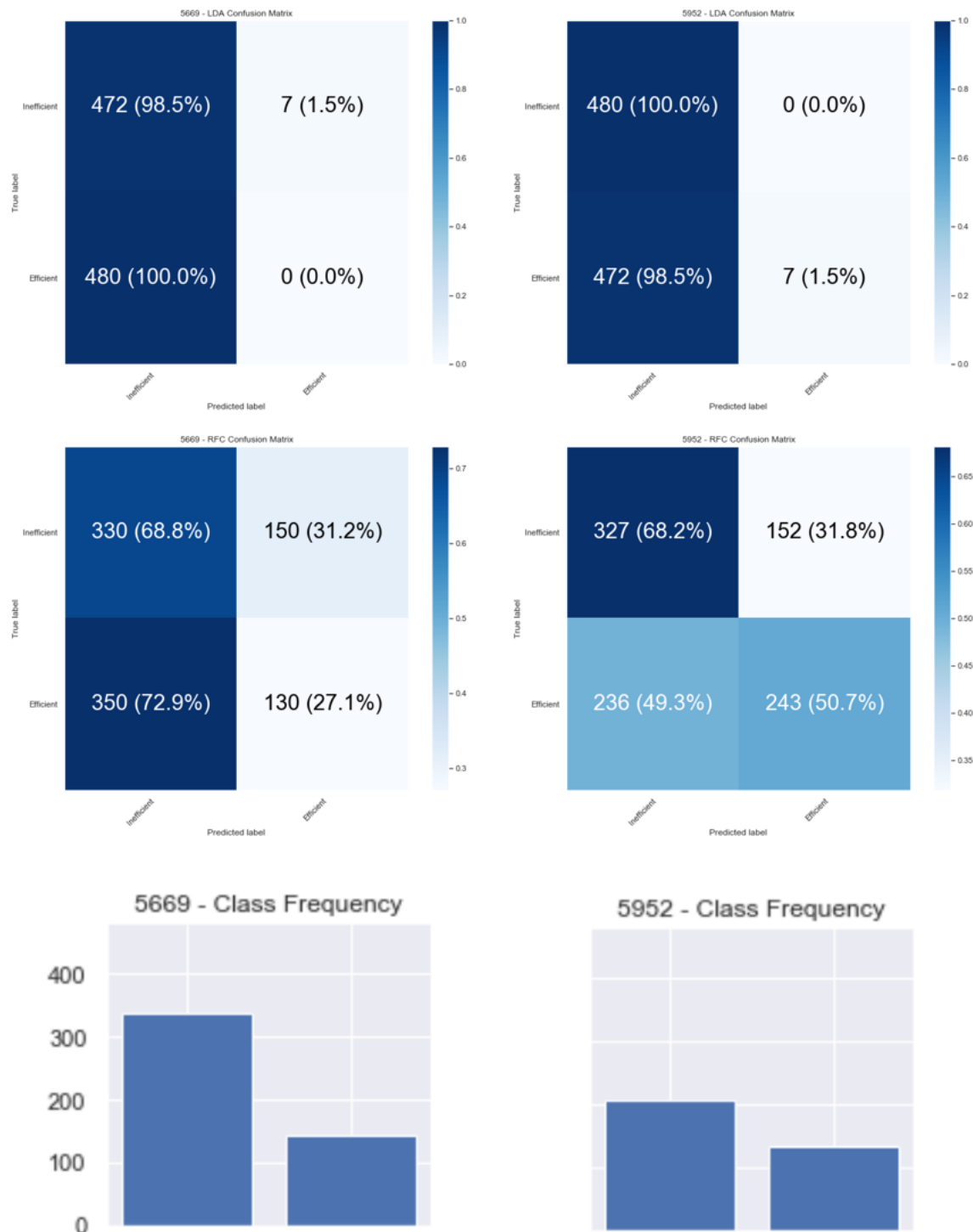
Figure 53. The top performer vs the lowest performer on the frequency feature dataset.
