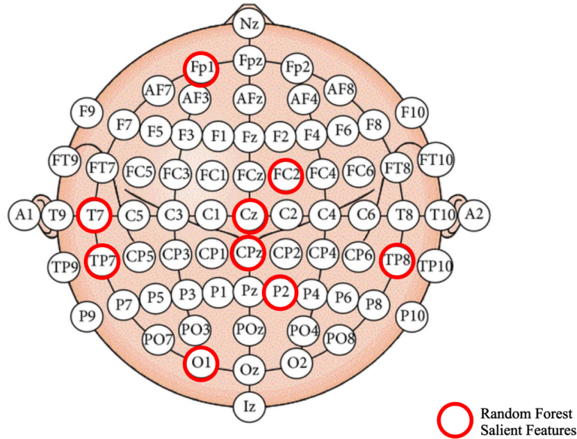
Figure 59. EEG Electrode Locations and Salient Features with High Performance
