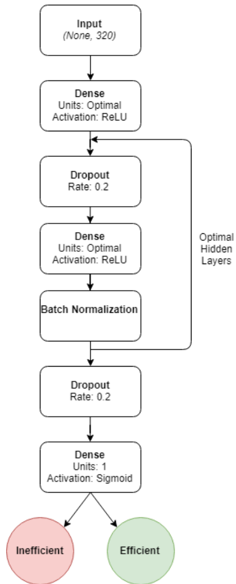
Figure 28. The ANN architecture.
