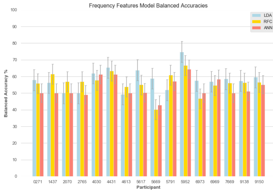
Figure 51. Overall model balanced accuracy of the Frequency Features dataset.
