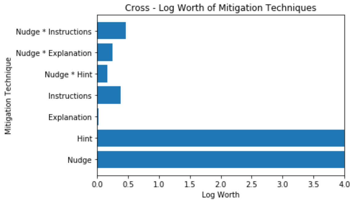
Figure 45. The log worth for all participants. The larger the blue bar, the more of an effect the mitigation technique had.
