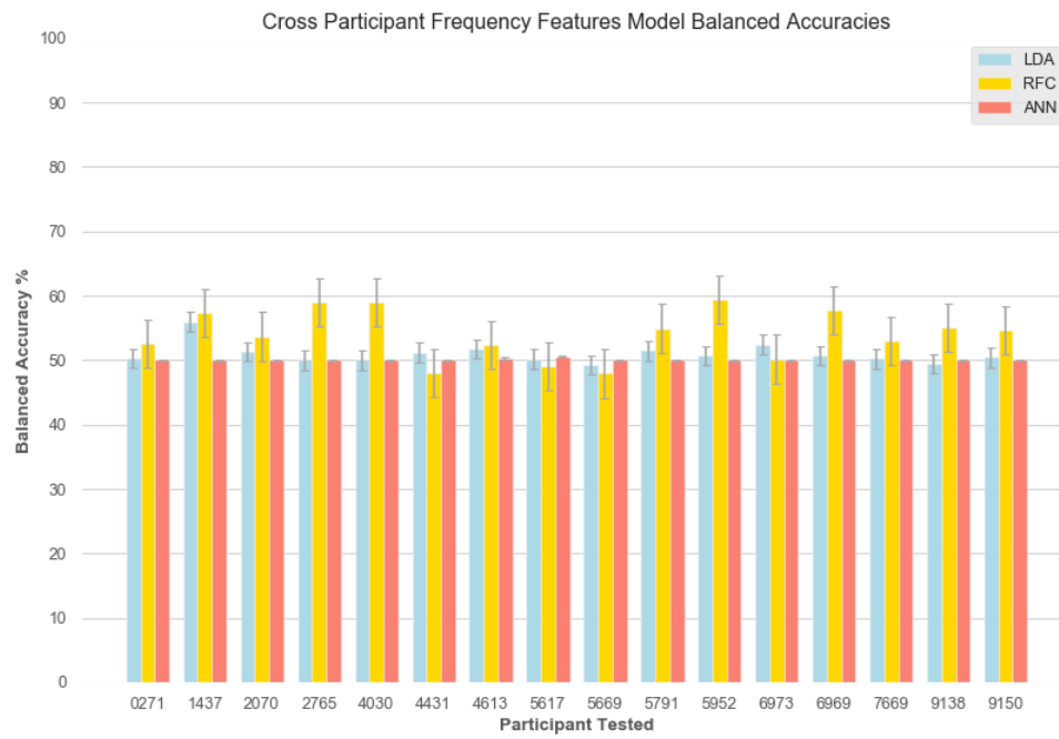
Figure 60. Cross-Participant Frequency Feature Balanced Accuracies
