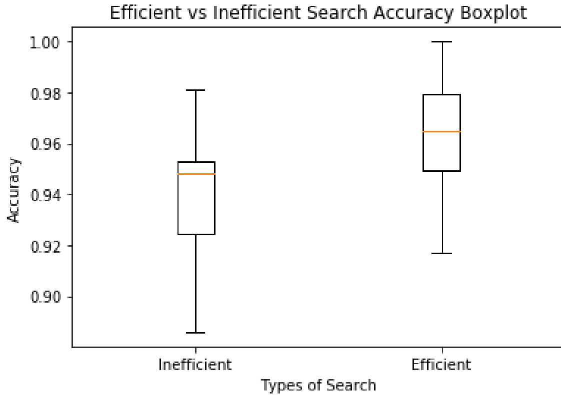
Figure 35. There does not appear to be any outliers in either the efficient accuracies or the inefficient accuracies.
