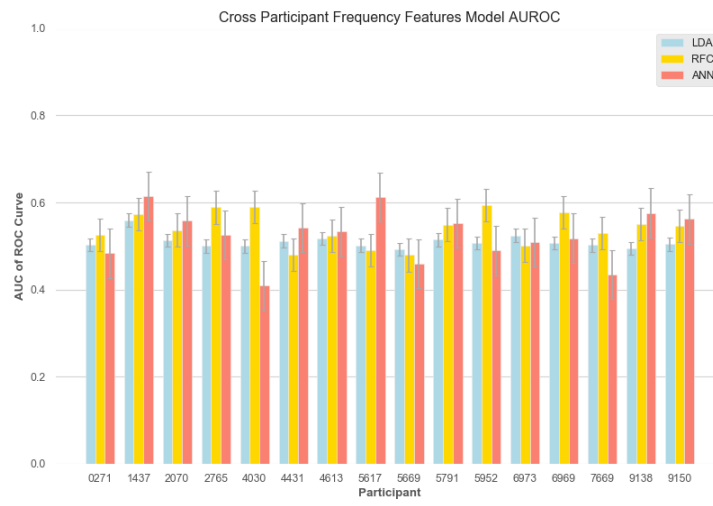
Figure 61. Cross-Participant Frequency Feature AUROCs
