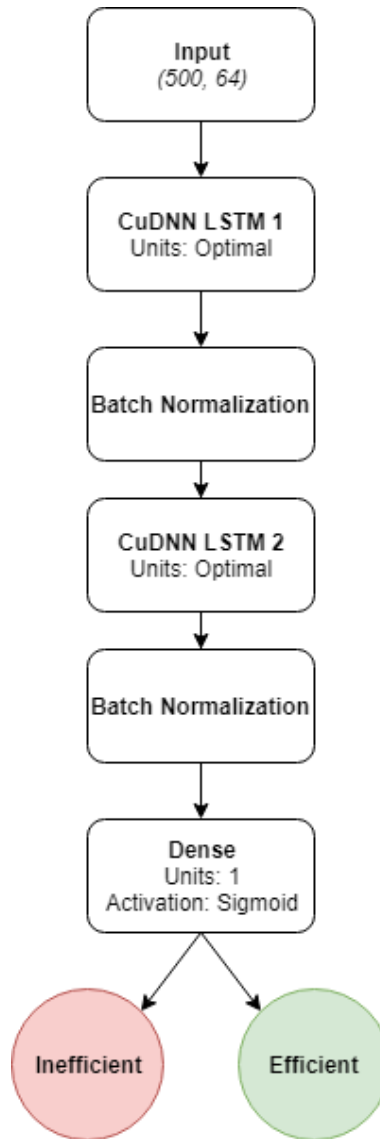
Figure 29. The LSTM model architecture.
