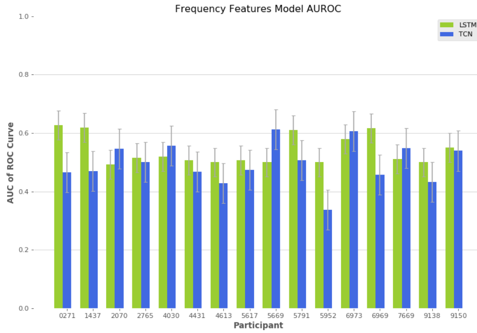
Figure 56. Overall model AUROC of the Time Series dataset.
