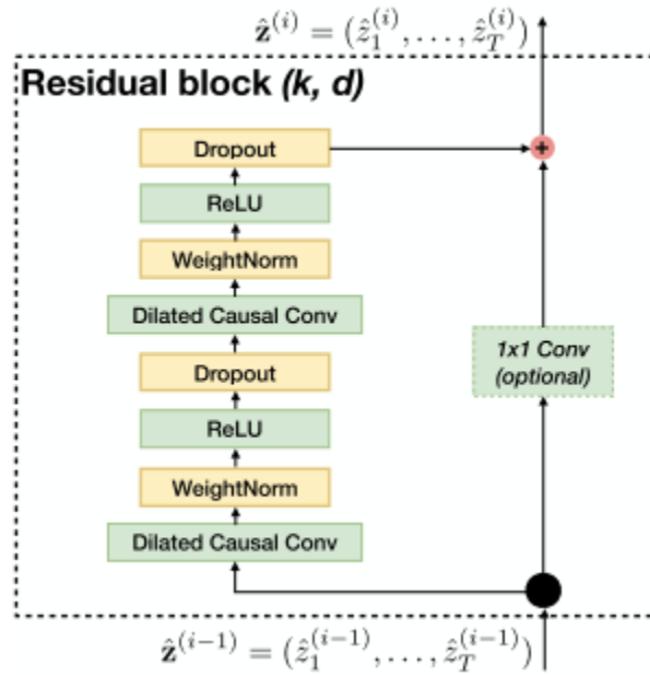
Figure 7. A residual block [91].
