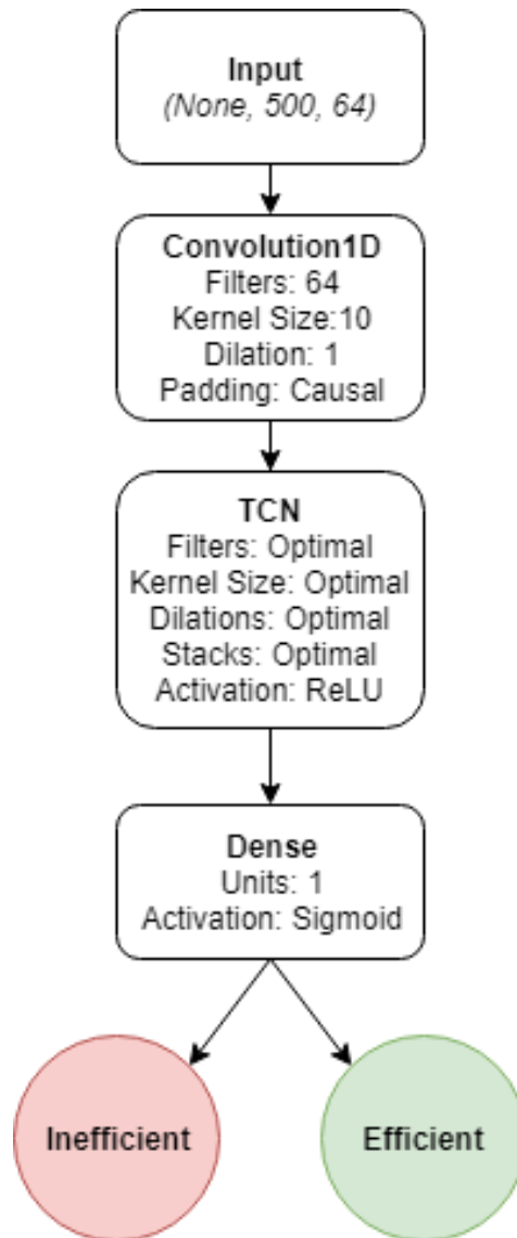
Figure 30. The TCN model architecture.
