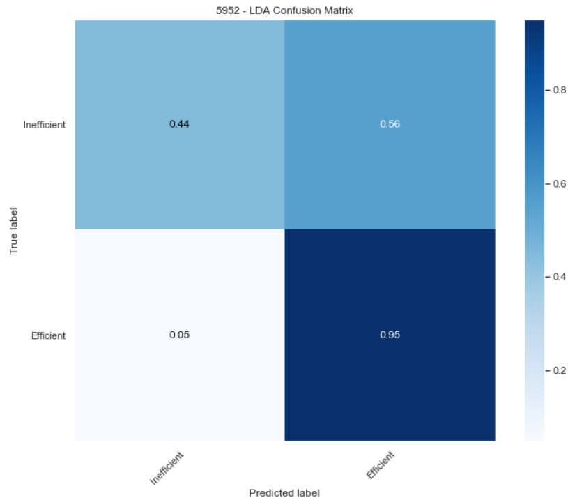
Figure 31. A confusion matrix.
