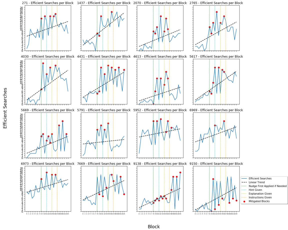
Figure 42. The number of efficient searches vs block number. Mitigation attempts and their locations are indicated on the graphs. The trend line of efficient searches is plotted.
