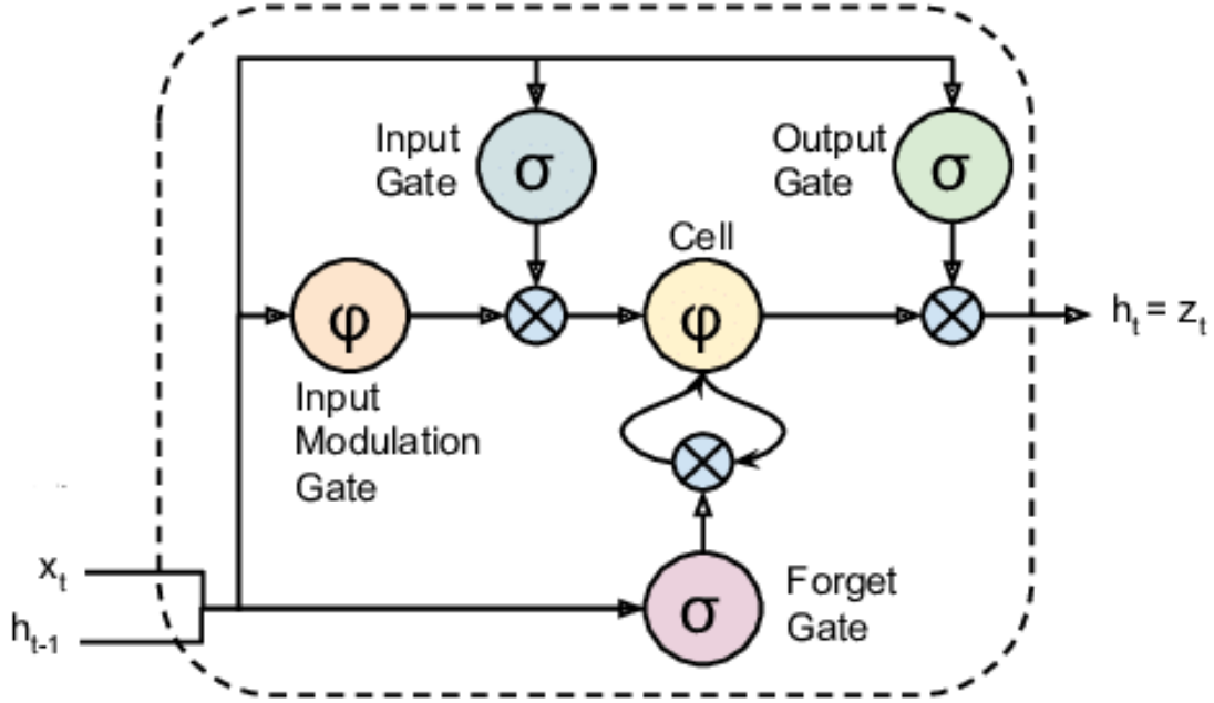
Figure 5. This is an example of a single LSTM [89].
