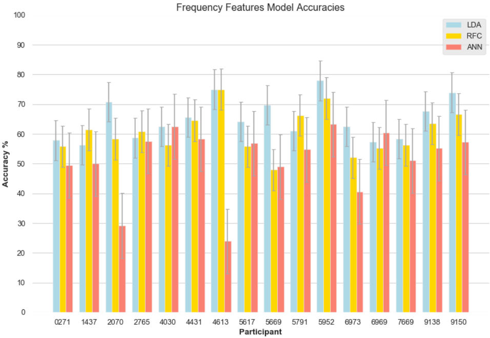
Figure 50. Overall model accuracy of the Frequency Features dataset.
