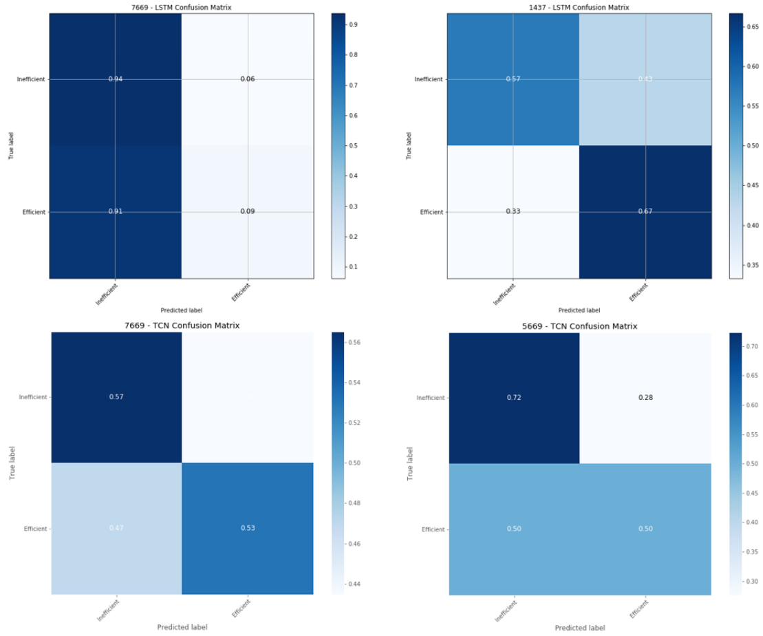
Figure 57. The top row of images are confusion matrices from the LSTM model while the bottom row are from the TCN model. The left column is the lowest performers while the right column is the highest performers.
