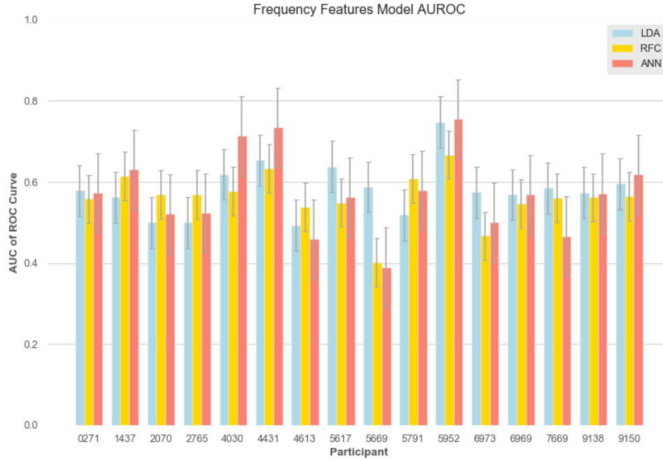
Figure 52. Overall model AUROC of the frequency feature dataset.
