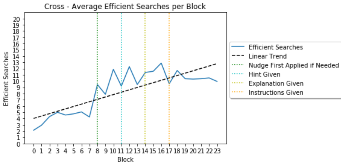
Figure 43. The number of efficient searches vs block number for all participants.
