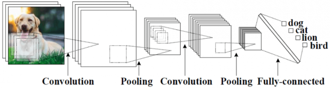
Figure 3. In this CNN, an image of an animal is taken as an input and the output is the type of animal [87].
