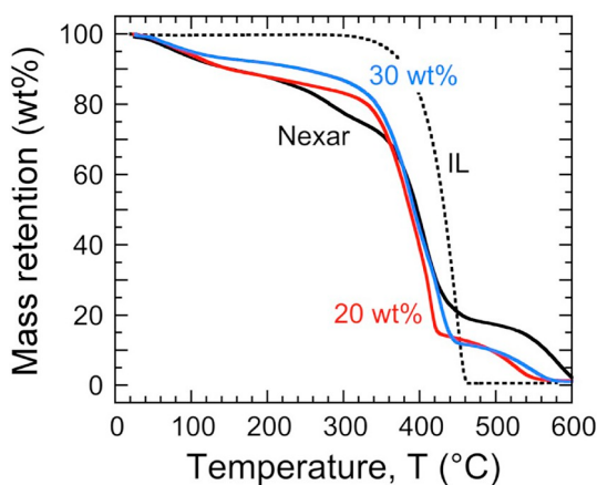
Fig. 4. Mass retention presented as a function of temperature, as measured by TGA, for neat Nexar and the [Bmim][BF 4 ] IL, as well as Nexar/IL hybrid materials (labeled according to wt% and color-coded). (For interpretation of the references to color in this figure legend, the reader is referred to the Web version of this article.)
