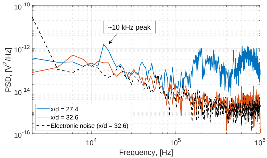
Figure 4.13.: PSD of PCB132 data from either side of the shock tube joint; nominal pressures p_{driven} = 0.4 mbar, p_{driver} = 336 mbar.
