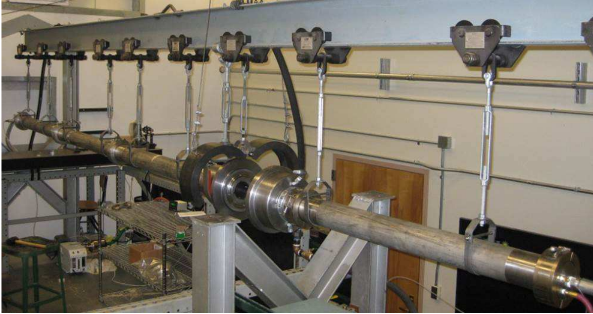
Figure 1: Photograph of Shock Tube for Calibrating Fast Pressure Sensors. Reproduced from Fig. 3.1 in Ref. [9]
