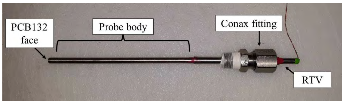
Figure 2.10.: PCB132 mounted in pitot-probe for end-plate mounting in P3IST.
