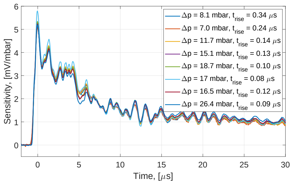
Figure 6.20.: Step sensitivity for PCB132A SN 6994 from P3IST pitot-mode testing.
