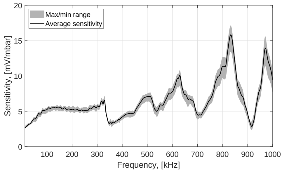
Figure B.1.: PCB132A21 SN 6772. Pressure steps range from 20.1–70.4 mbar. Frequency response calculated from 150 \mu s of data. Grayed area indicates range of sensitivity.
