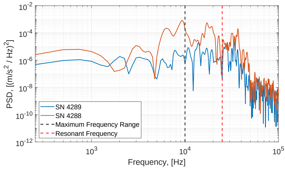
Figure 4.9.: PSD of vibrations measured before shock arrival by PCB606B01 SN 4288 at x/d = 27.4 , PCB606B01 SN 4289 at x/d = 32.6 ; p_{driver} = 335.91 mbar, p_{driven} = 0.400 mbar.
