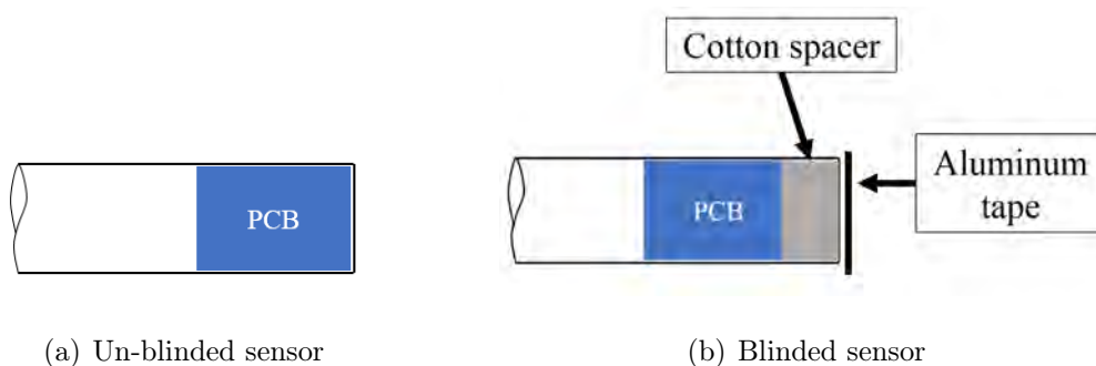
Figure 6.13.: Blinded PCB132 schematic.
