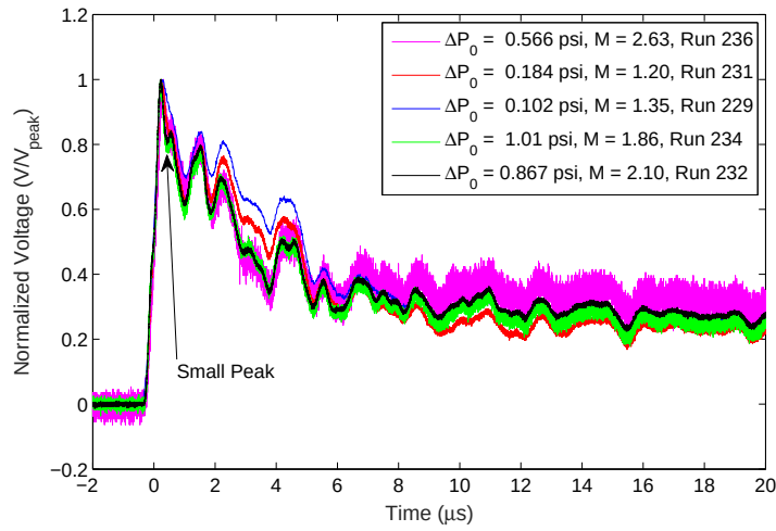
Figure 3: Normalized PCB-132 Response to Pressure Step Showing Good Linearity. Replotted from Fig. 8.9b in Ref. [9]
