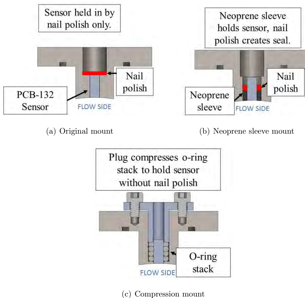
Figure 2.8.: Cross-sectional views of different static-mounting designs for PCB132 in P3IST.
