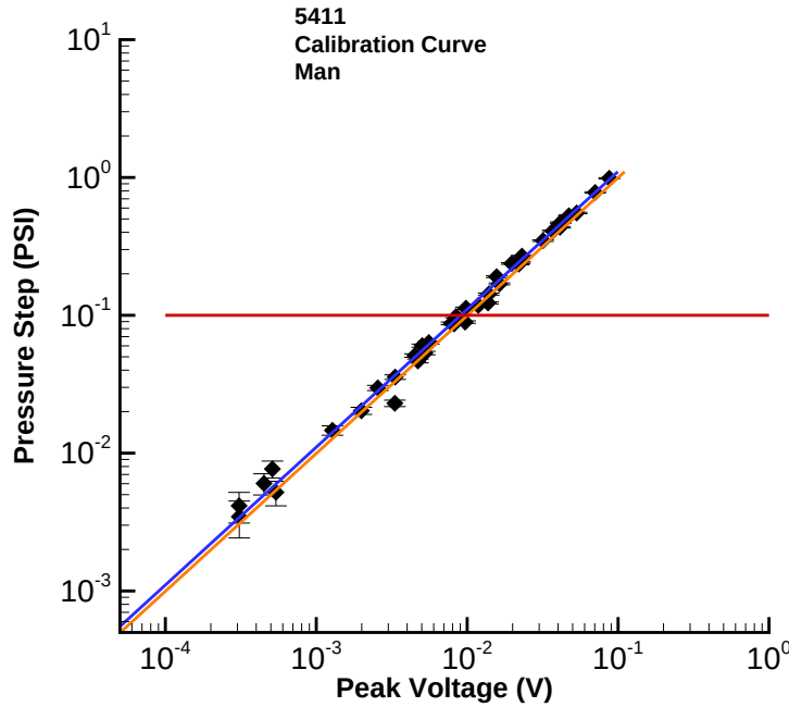
Figure 4: Linearity of Pressure Response to Amplitude Steps Varying by a Factor of 1000. Replotted from Fig. 7.1b in Ref. [9]
