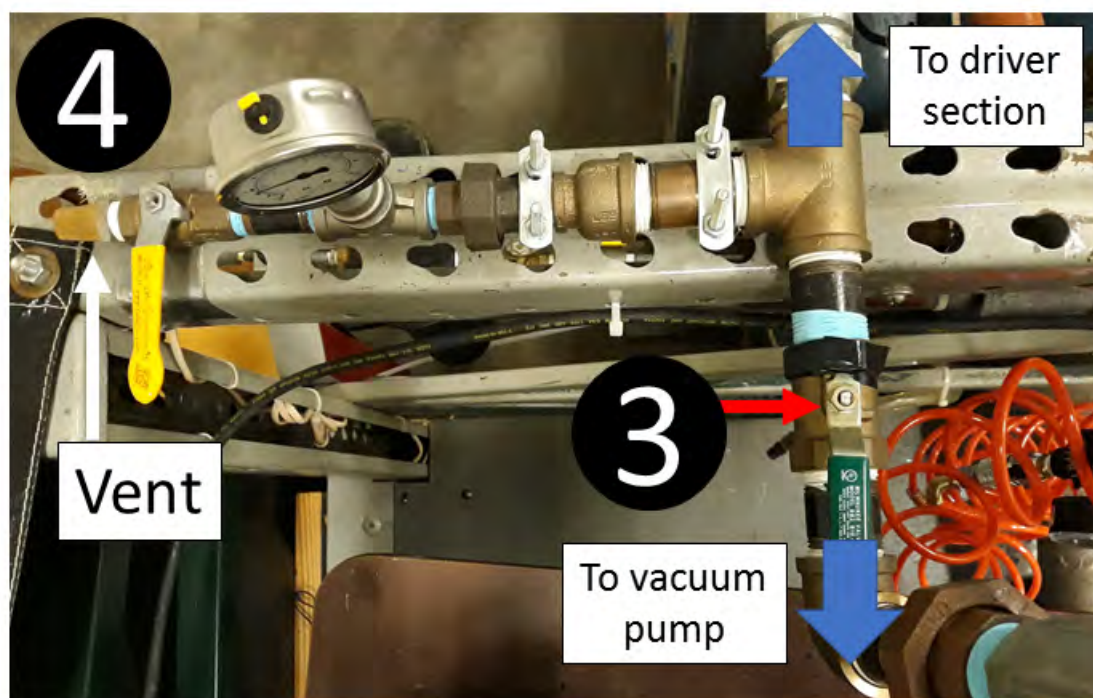
Figure C.4.: Valves 3 and 4, as shown in Figure C.1.
