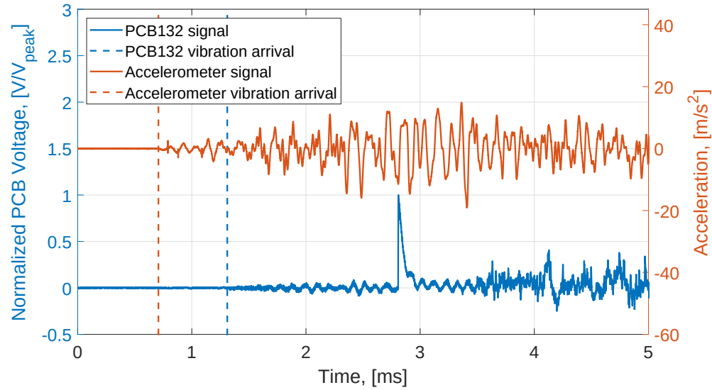
Figure 4.4.: Time trace from PCB132 and accelerometer located at x/d = 27.4 ; p_{driver} = 786.97 mbar, p_{driven} = 1.300 mbar.
