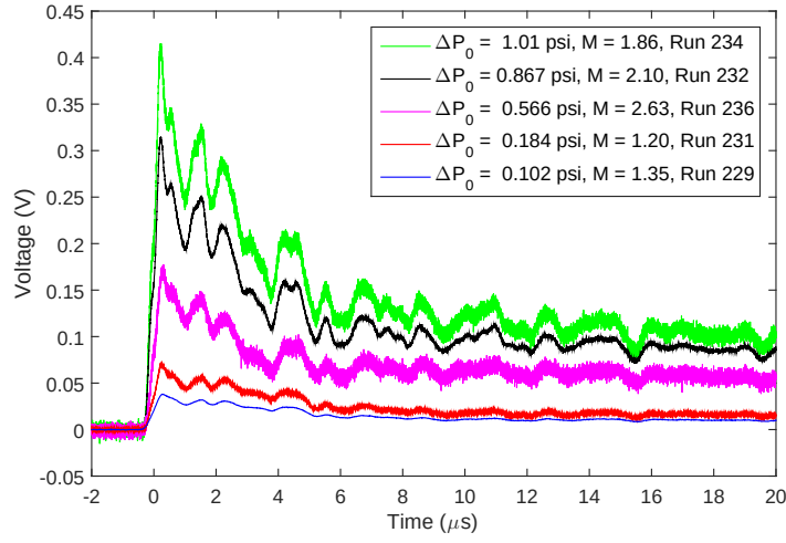
Figure 2: PCB-132 Response to Passage of Pressure Step due to Shock. Replotted from Fig. 8.9a in Ref. [9]
