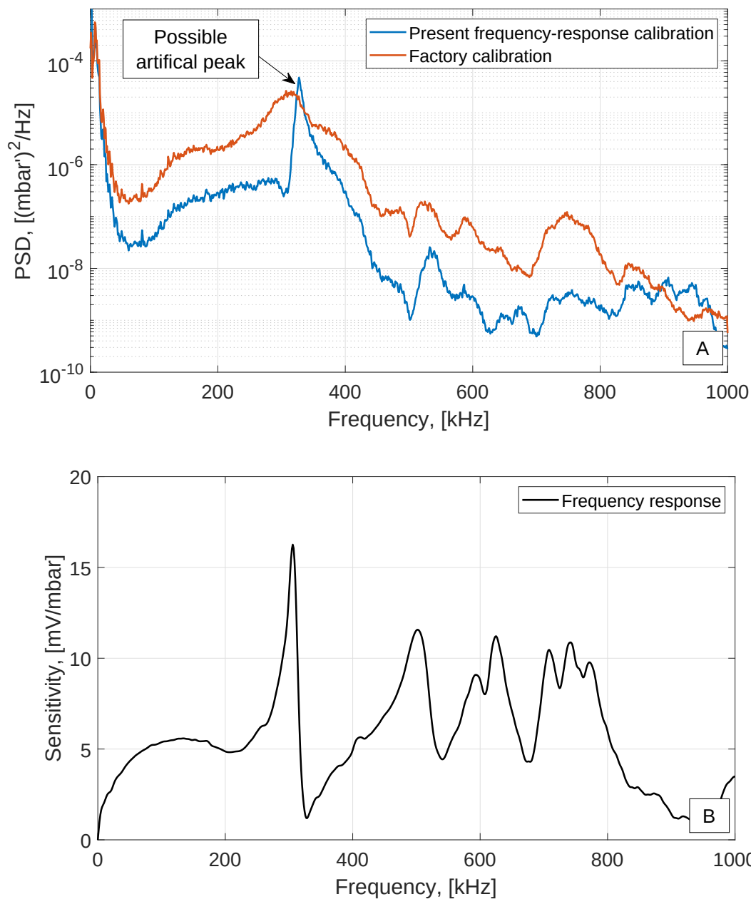
Figure 6.25.: PSD of data acquired by PCB132B (SN7949) in the BAM6QT at Re_m = 10.6 \times 10^6 , bleeds open (A). Averaged approximate frequency response (SN 7949) found with the P3IST (B); pressure steps range from 10.3–39.2 mbar; data length of 150 \mu s.
