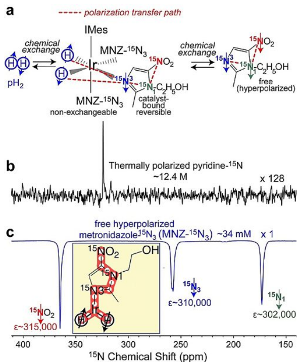
Figure 1. a) Schematic of the simultaneous chemical exchange of pH 2 and [ 15 N 3 ]metronidazole (MNZ- 15 N 3 ) on the Ir-IMes polarization transfer catalyst. [39] Note the dashed red lines indicate the likely path of spin-relayed polarization transfer from pH 2 -derived hydrides to the 15 NO 2 group via the 15 N 3 and 15 N 1 sites. b) Single-scan 15 N NMR signal reference spectrum of thermally polarized neat (no solvent) [ 15 N]pyridine (12.4 M). c) Single-scan 15 N NMR spectrum of HP [ 15 N 3 ]metronidazole in [D 4 ]MeOH. All NMR spectra were recorded at 1.4 T. The inset displays (in red) the path of chemical bonds over which the network of I = 1/2 spin relays is established. The following experimental conditions were employed for SABRE-SHEATH hyperpolarization: Room temperature, 6.7 atm overpressure of the medium-walled NMR tube, and a flow rate of 70 sccm (standard cubic centimeters per minute) of pH 2 controlled by a mass-flow controller (MFC).
