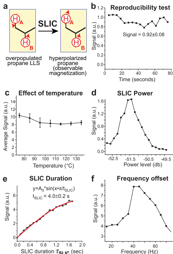
Figure 3. Results from SLIC pulse optimization with HP propane data acquired using the 0.0475 T NMR spectrometer setup shown in Scheme 1 at a production/reactor/reaction temperature of 60 \pm 1 ^{\circ}\text{C} (except for display (c) where the temperature was varied). (a) Diagram showing the transformation of LLS of HP propane (denoted schematically as a singlet) into observable magnetization achieved using a SLIC pulse. (b) Results from a test of the shot-to-shot reproducibility of the intensity of the HP propane signal. (c) Temperature dependence of the average (over three data points) HP propane SLIC-induced signal using a 1:1 gas mixture of \text{pH}_2 and propylene. (d) Optimization of RF power of the SLIC pulse (note the x-axis is provided in db units of the Kea NMR spectrometer due to the nonlinearity of the RF amplifier at low power levels; the maximum is expected at the B_1 RF strength between 10 and 30 Hz 63 ). (e) The dependence of the HP propane signal on the SLIC pulse duration (experimental data: black points; a fit using a sinusoidal function is shown by the solid red curve). (f) The dependence of the HP propane signal on the SLIC pulse frequency offset. Note a SLIC pulse duration of 500 ms was employed for the data acquisition in panels (b–d,f). Connecting lines in displays (b–d,f) are meant only to guide the eye.
