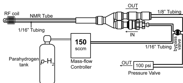
Figure 3. Schematic of polarizer setup for homogeneous PHIP hyperpolarization.
