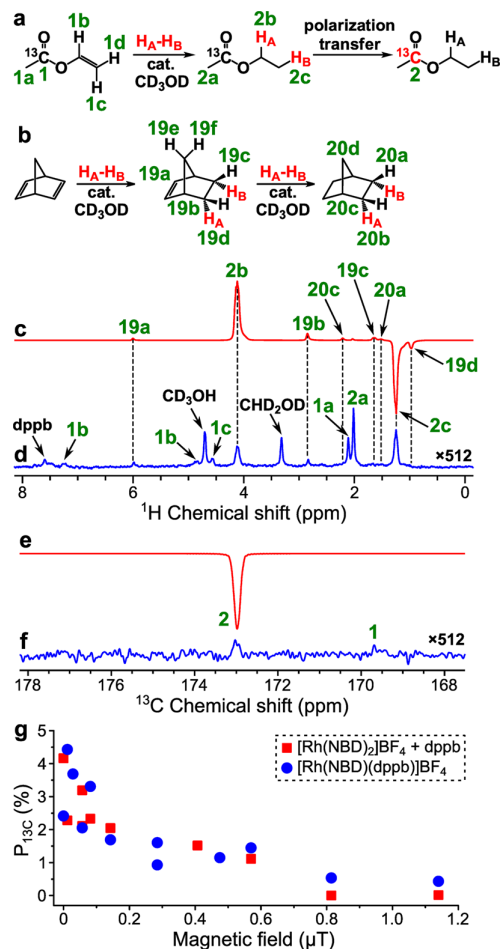
Figure 2. (a) Reaction scheme of pairwise addition of p\text{-H}_2 to vinyl 1- ^{13}\text{C} -acetate in \text{CD}_3\text{OD} followed by polarization transfer to ^{13}\text{C} nuclei ( \text{H}_\text{A} and \text{H}_\text{B} are two atoms from the same p\text{-H}_2 molecule, cat. = [\text{Rh}(\text{NBD})(\text{dppb})]\text{BF}_4 ). (b) Reaction scheme of the competing process of norbornadiene hydrogenation with p\text{-H}_2 . (c) ^1\text{H} NMR spectrum acquired after ^1\text{H} ALTADENA hyperpolarization of ethyl acetate with 15 s p\text{-H}_2 bubbling duration. (d) Corresponding thermal ^1\text{H} NMR spectrum acquired after relaxation of hyperpolarization (multiplied by a factor of 512). \epsilon_{\text{H}} = 3750 , P_{\text{H}} = 8.6\% (8.1% at 85% p\text{-H}_2 fraction). Note that spectra (c) and (d) were acquired on a 7.05 T NMR spectrometer. (e) ^{13}\text{C} NMR spectrum acquired after ^{13}\text{C} hyperpolarization of ethyl 1- ^{13}\text{C} -acetate using MFC at near 0 \mu\text{T} magnetic field. (f) Corresponding thermal ^{13}\text{C} NMR spectrum acquired after relaxation of hyperpolarization (multiplied by a factor of 512). \epsilon_{^{13}\text{C}} = 3560 , P_{^{13}\text{C}} = 2.75\% (4.2% at 85% p\text{-H}_2 fraction). (g) Dependence of P_{^{13}\text{C}} (at 85% p\text{-H}_2 fraction) of ethyl 1- ^{13}\text{C} -acetate on magnetic field used in MFC experiments (red squares, data points obtained with the [\text{Rh}(\text{NBD})(\text{dppb})]\text{BF}_4 catalyst prepared from [\text{Rh}(\text{NBD})_2]\text{BF}_4 and dppb; blue circles, data points obtained with the commercial [\text{Rh}(\text{NBD})(\text{dppb})]\text{BF}_4 catalyst).
