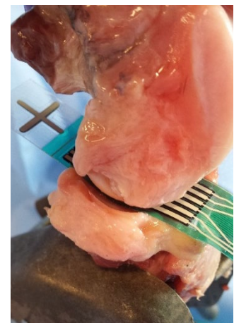
Figure 3. Experimental setup for contact pressure testing in canine BioJoint samples.
