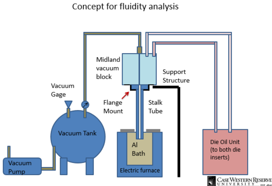
Figure 4.1: Schematic for fluidity test based on vacuum suction into thin walled mold
