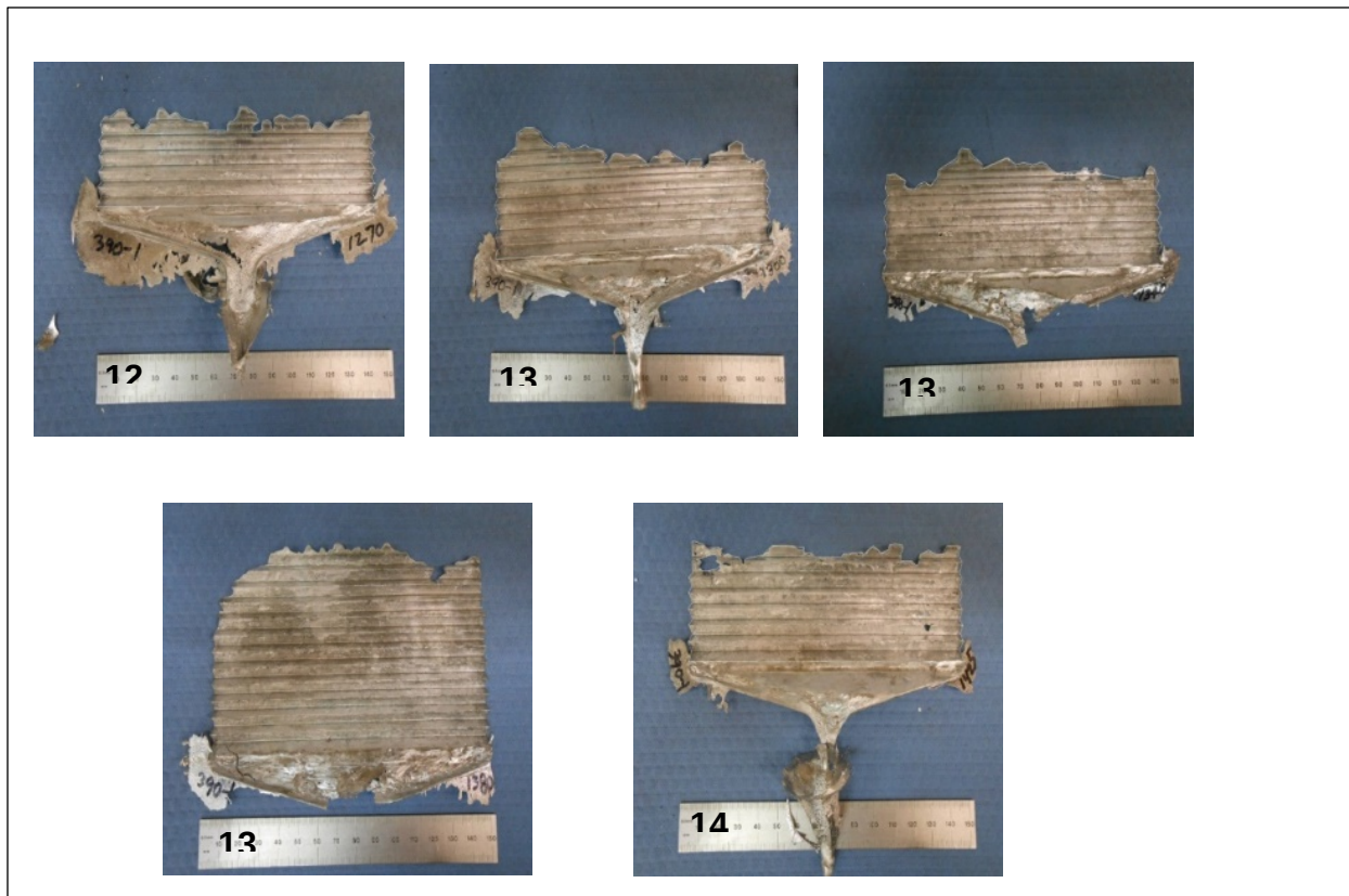
Figure 5.2.4: Thin foil 390-1 alloy solidified in the vent block: the area of the cast aluminum foil increases as a function of temperature
