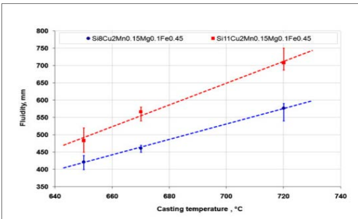
Figure 3.2.2: Casting temperature v. fluidity: alloys with high Si content exhibit higher fluidity
