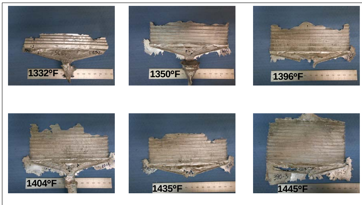
Figure 5.2.8: Thin foil 390-3 alloy film solidified in the vent block
