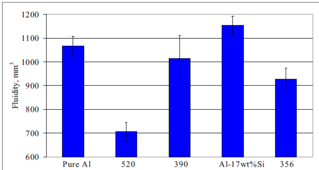
Figure 3.2.4: Relative fluidity of commercial foundry aluminum alloys
