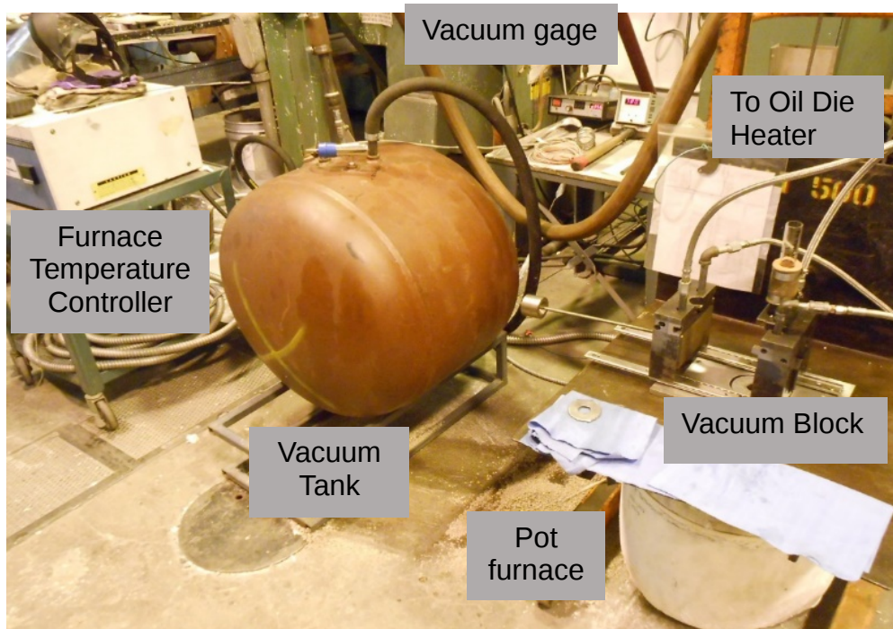
Figure 4.3: Fluidity measurement system
