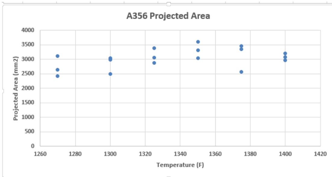
Figure 5.1.2: Projected area of A356 castings as a function of temperature
