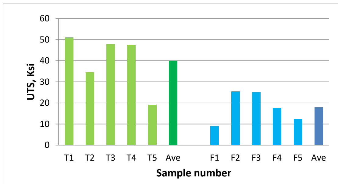
Figure 6.5: UTS of 206 squeeze cast plates in the as-cast (F) and heat treated (T6) state
