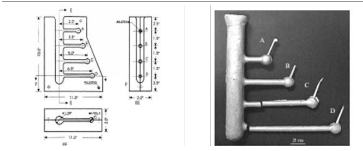
Figure 6.6: Constrained Rod Casting (CRC) for Hot Tearing Evaluation
