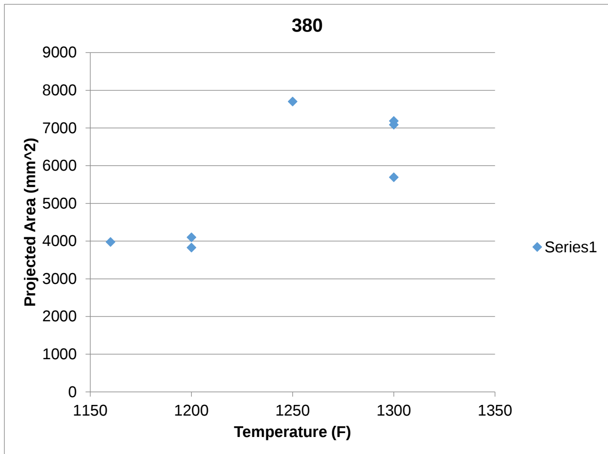
Figure 5.1.4: The area of the 380 alloy cast foil increases as a function of temperature
