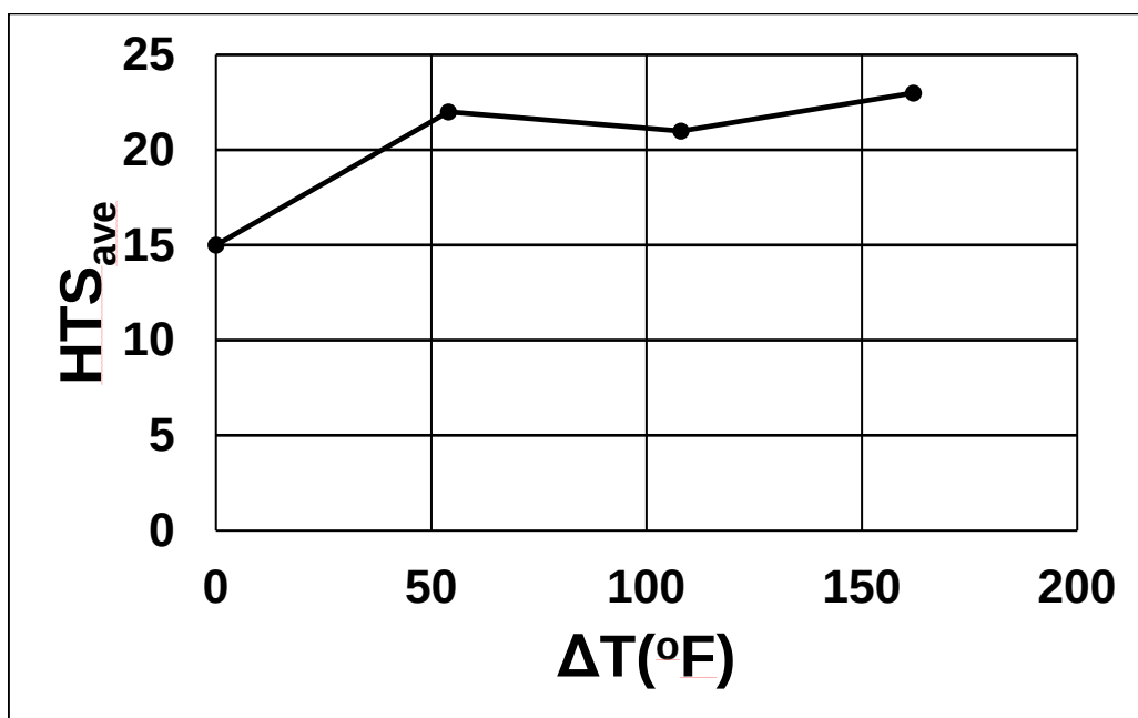
Figure 6.7: Hot tearing tendency of the 206 alloy as a function of superheat.
