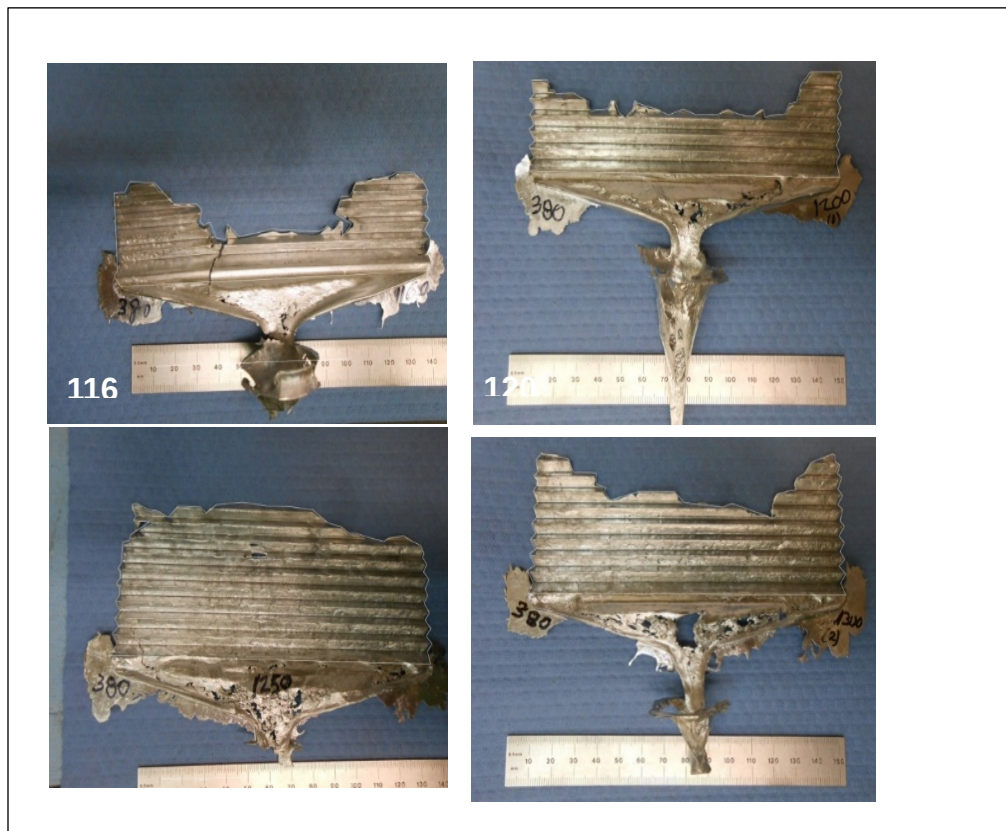
Figure 5.1.3: Thin foil 380 alloy solidified in the vent block: the area of the foil increases as a function of temperature
