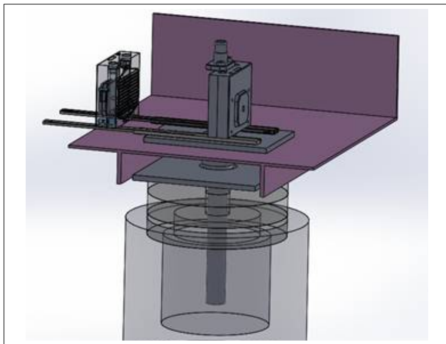
Figure 4.2: Movable vent block
