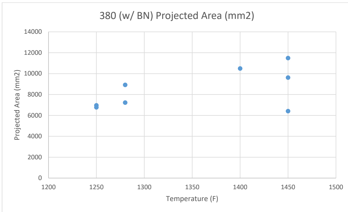
Figure 5.2.10: Fluidity of A380 using a BN-coated vent block
