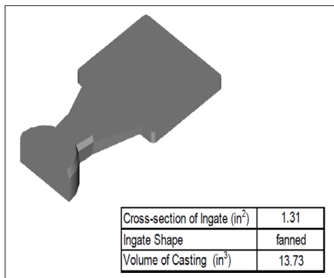
Figure 6.2: Squeeze cast plate solid model
