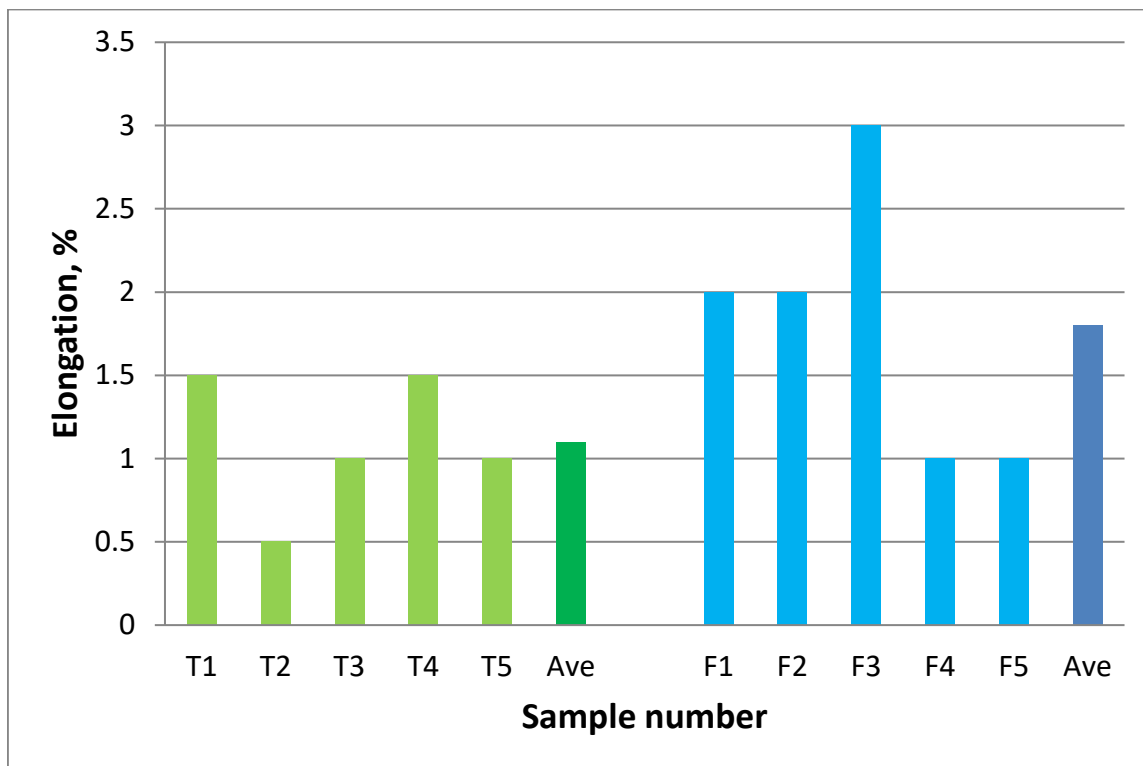
Figure 6.6: Elongation of 206 squeeze cast plate in as-cast (F) and heat treated (T6) condition
