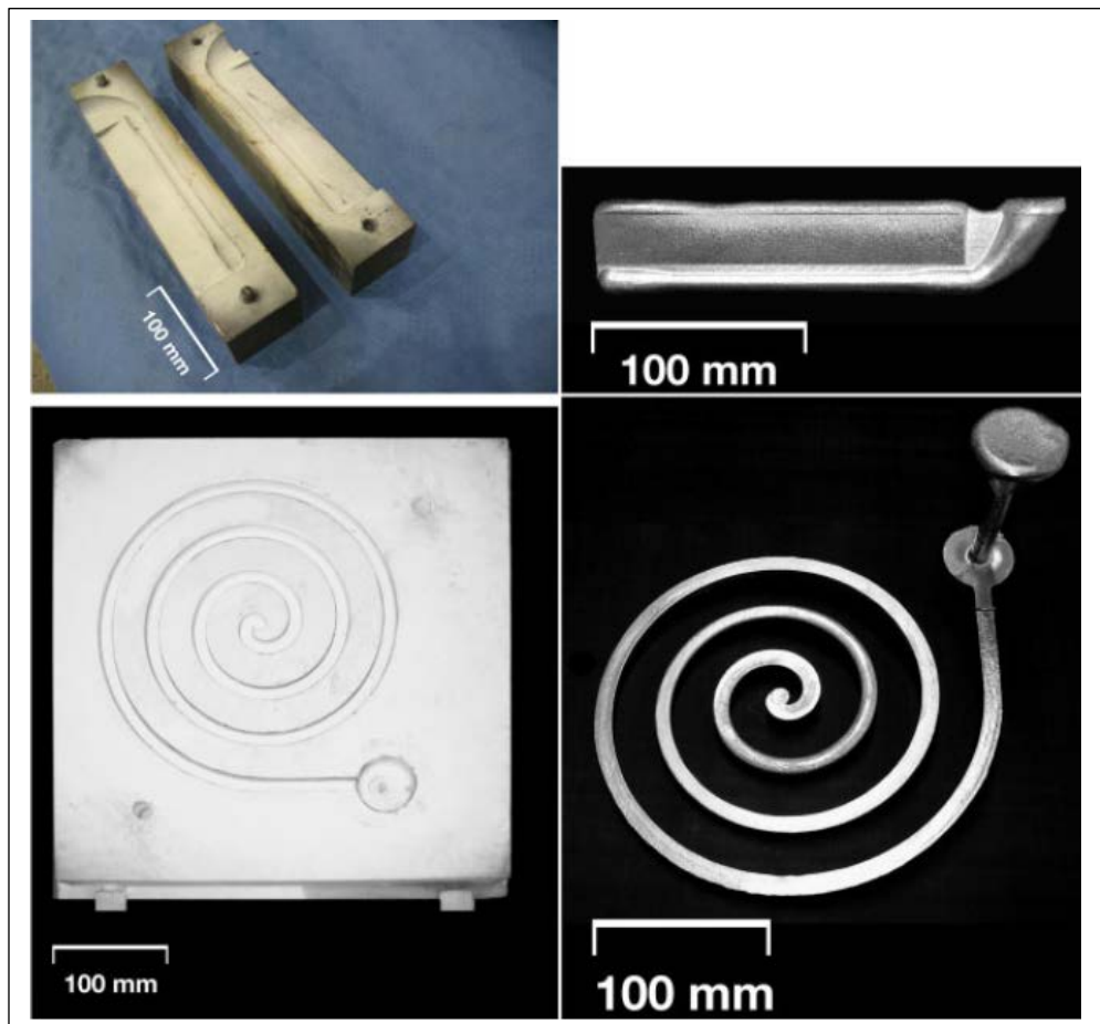
Figure 3.2.1: Typical spiral mold configuration used in fluidity studies of casting alloys
