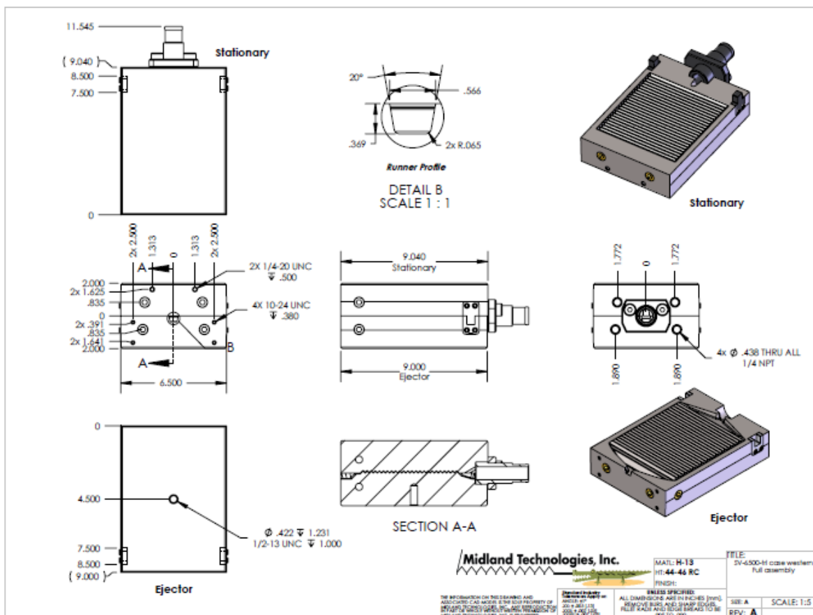
Figure 4.7: Schematics of the large vent block
