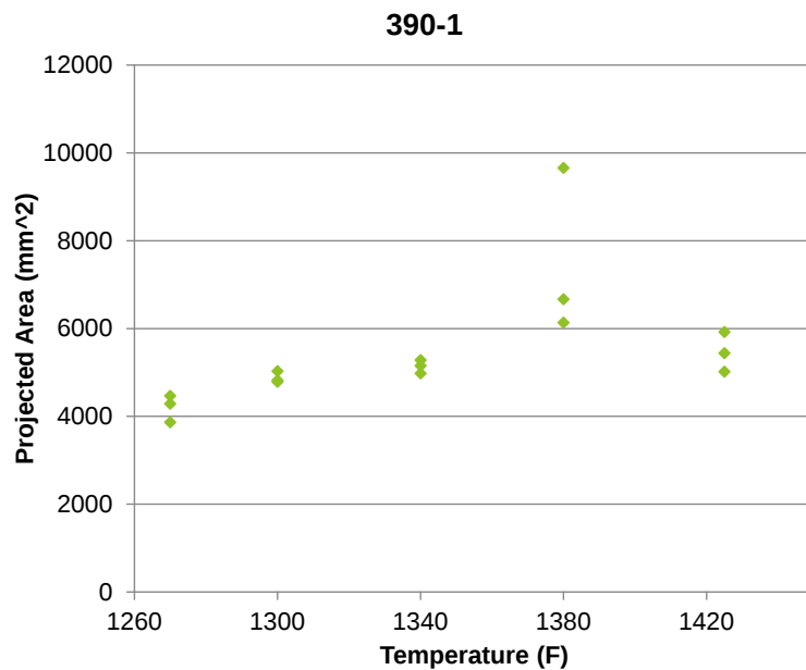
Figure 5.2.5: The area of the 390-1 alloy cast foil increases as a function of temperature
