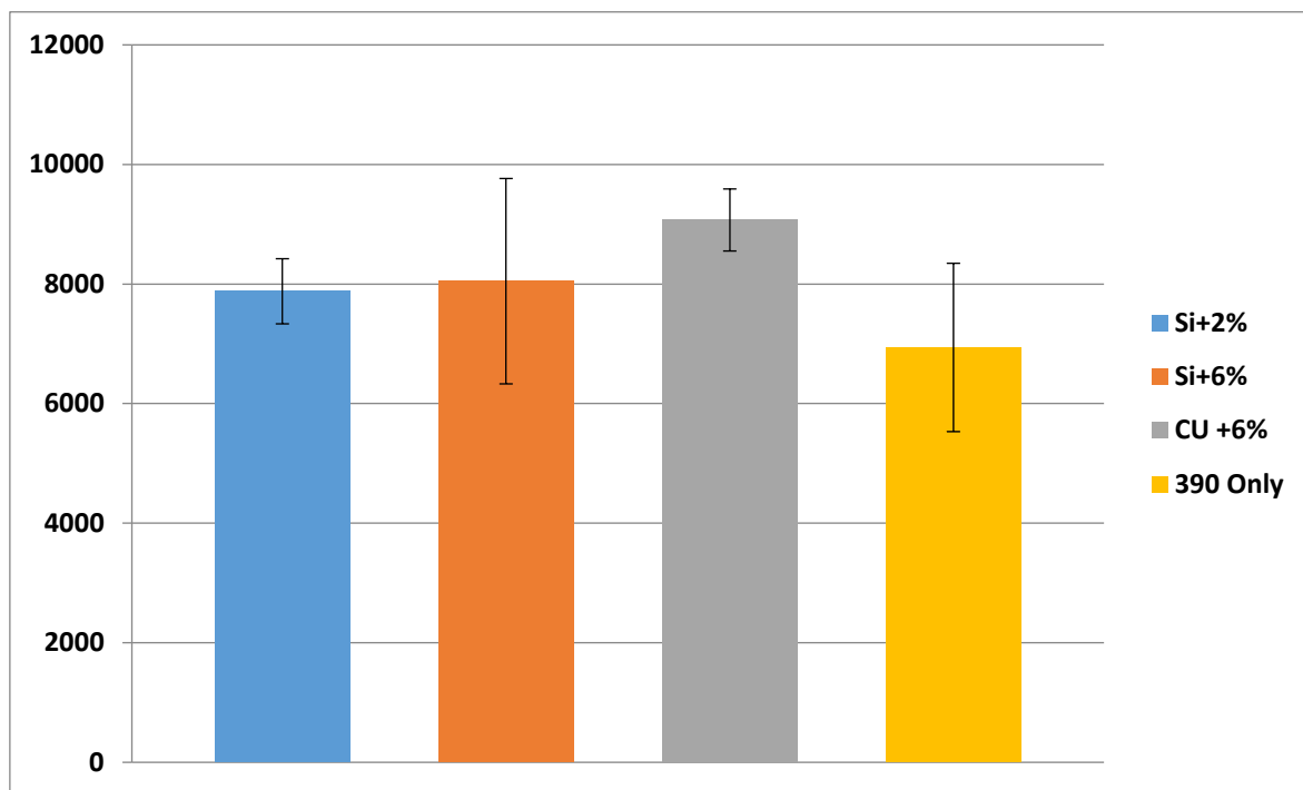
Figure 5.2.9: Increase in fluidity obtained by additions of Si and Cu to 390
