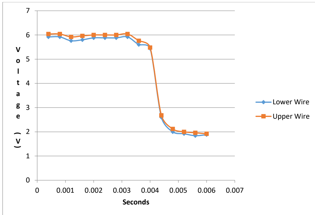
Figure 4.10: Time to fill used to determine fill velocity
