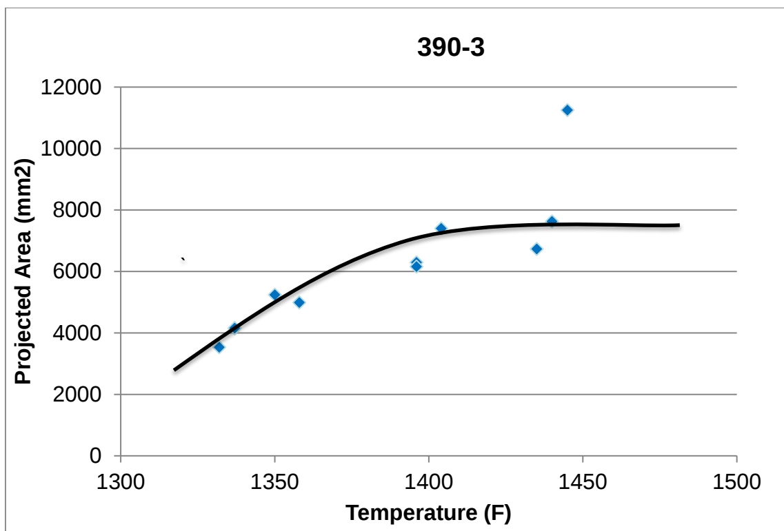
Figure 5.2.9: The area of the 390-3 alloy cast foil increases as a function of temperature
