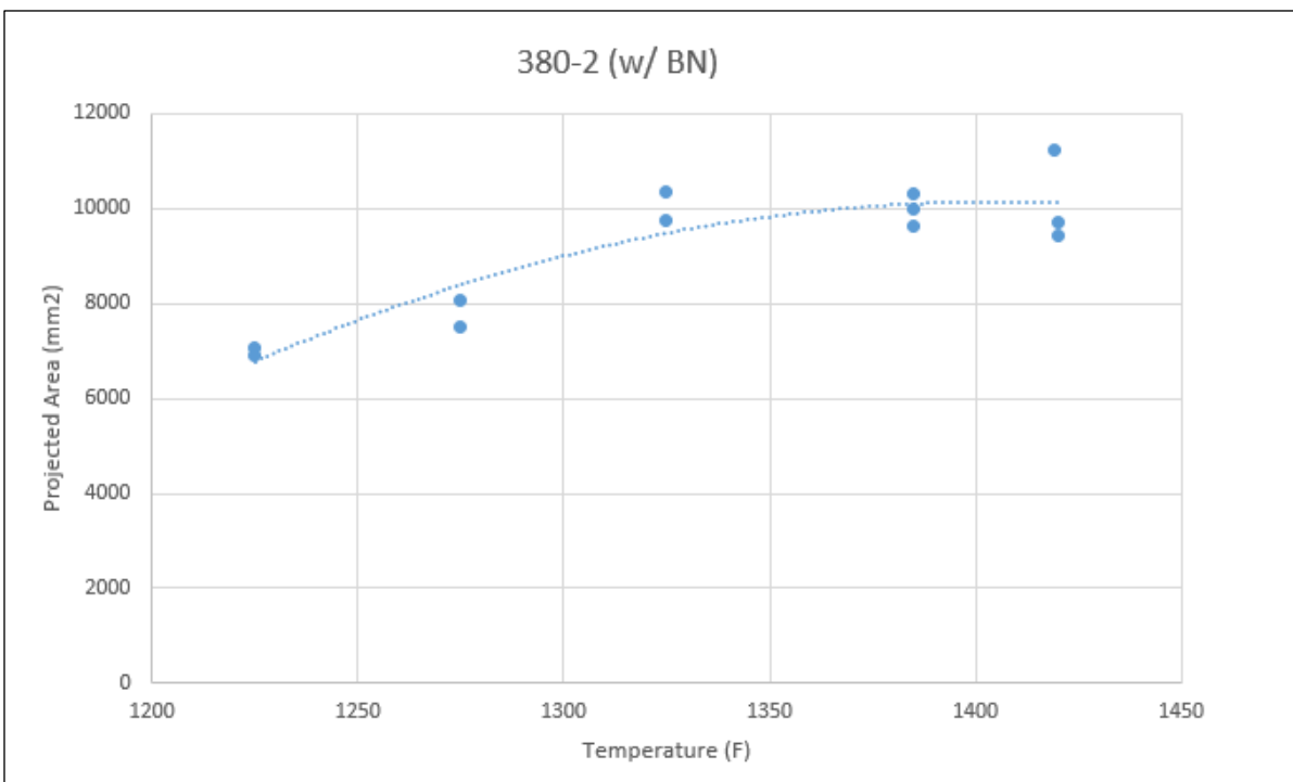
Figure 5.2.11: Fluidity of A380-2 using a BN-coated mold
