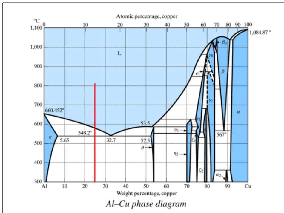
Figure 5.2.1: Al-Cu phase diagram
