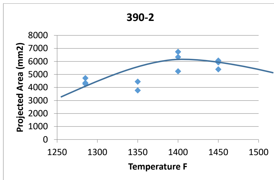
Figure 5.2.7: The area of the 390-2 cast alloy as a function of temperature
