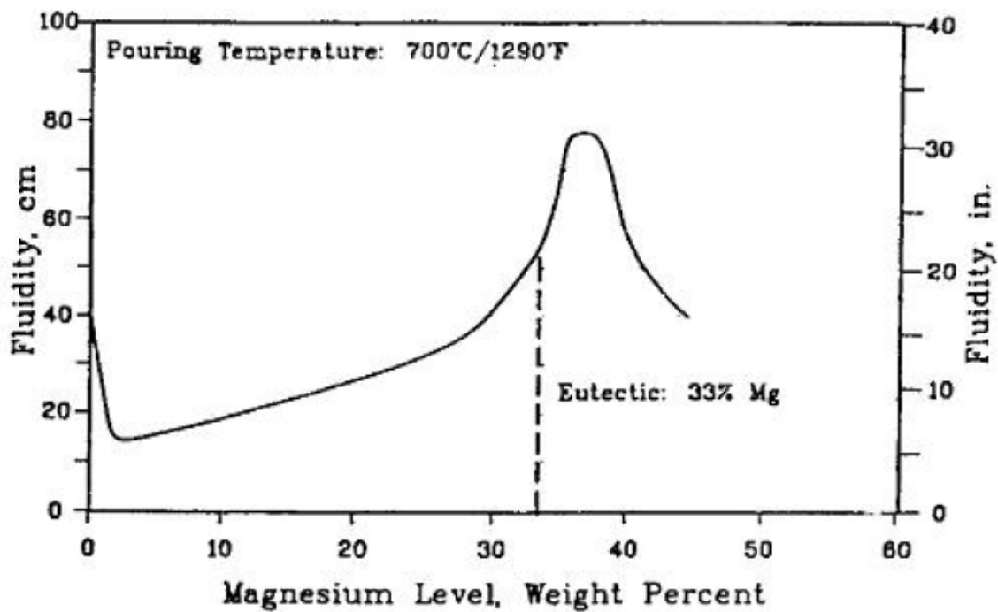
Figure 3.2.6: Effect of magnesium on fluidity in aluminum binary alloys
