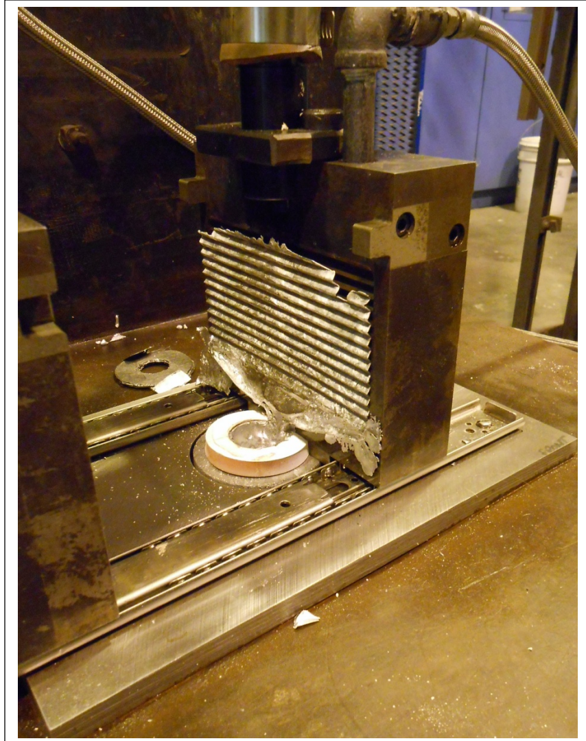
Figure 4.6: Open vent block demonstrating filling with aluminum
