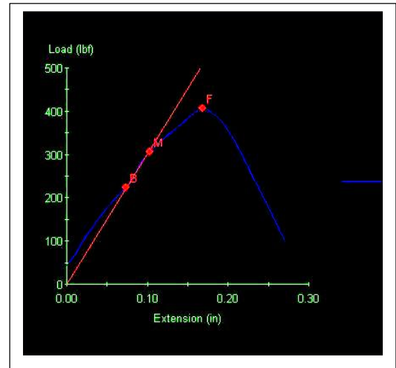
Figure 5.4.4: Pull-out plots for the rough surface rod (a) first pull-out (b) second pull-out
