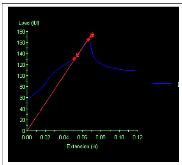
Figure 5.4.4: Pull-out plots for the rough surface rod (a) first pull-out (b) second pull-out
