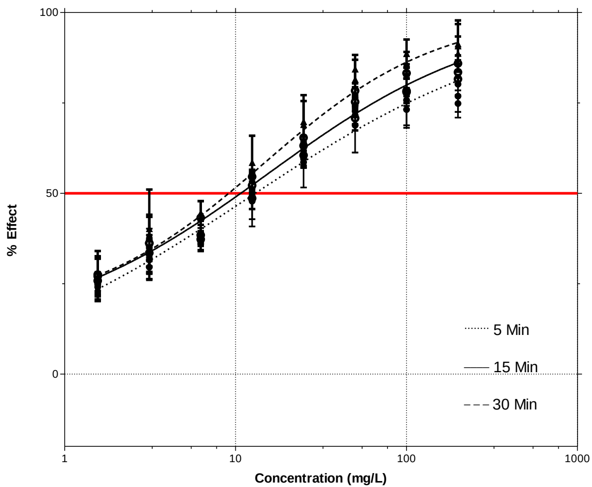
Figure G-1 – Microtox Toxicity of OBF-OH - Red line represents median effect
