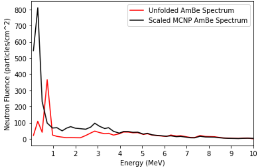
Figure 34. Neutron spectra resulting from the MAXED unfolding of the BSS data with the MCNP modelled spectrum as the a priori spectrum and the scaled MCNP modelled spectrum.
