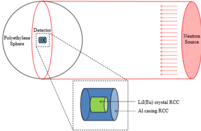
Figure 22. Diagram of the computational model used by MCNP6 to reproduce the response function for each moderated sphere [23].
