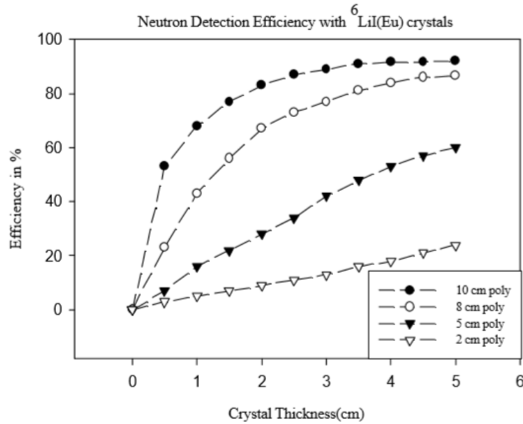
Figure 18. Thermal neutron detection efficiency by different thicknesses of ^6\text{LiI}(\text{Eu}) crystal. Layers of various thicknesses of polyethylene rings were used to optimize the neutron energy moderation. Reproduced with permission from [20].
