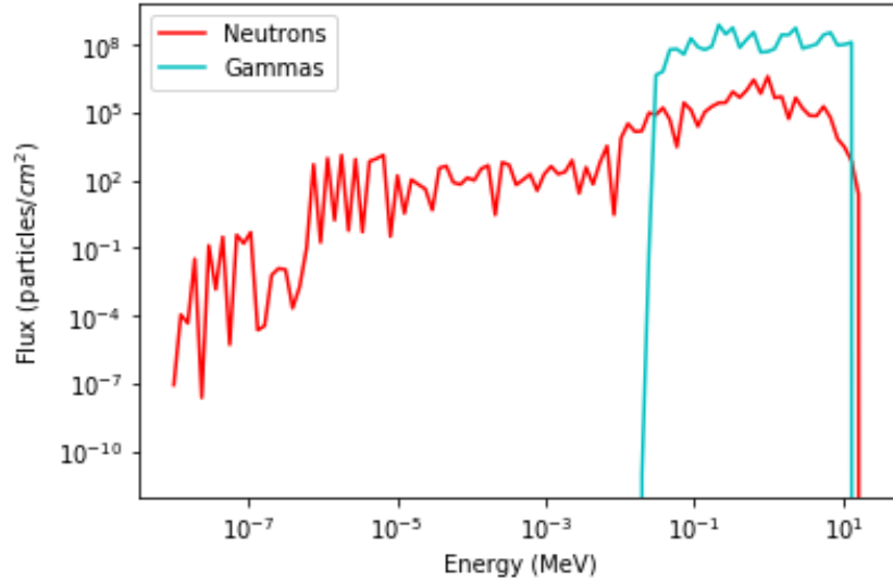
Figure 38. Neutron and photon flux for the single building model with 1 kT yield and 1 km HOB.
