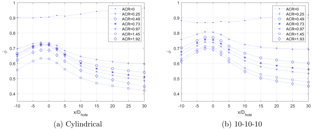
Figure 75. ACR effects on overall effectiveness for the cylindrical hole and 10-10-10 hole at Tu \approx 2\% .
