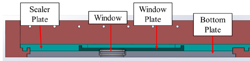
Figure 59. Viewport assembly [31].
