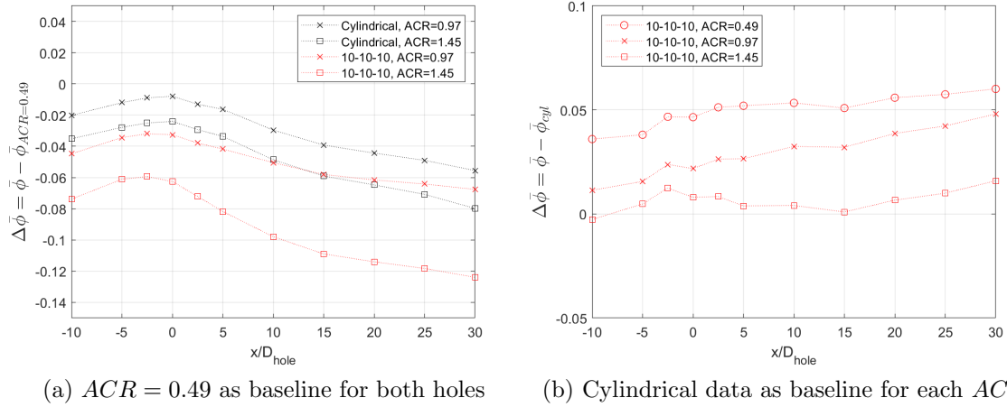
Figure 76. \Delta\bar{\phi} versus downstream distance for the cylindrical hole and 10-10-10 hole at Tu \approx 2\% .
