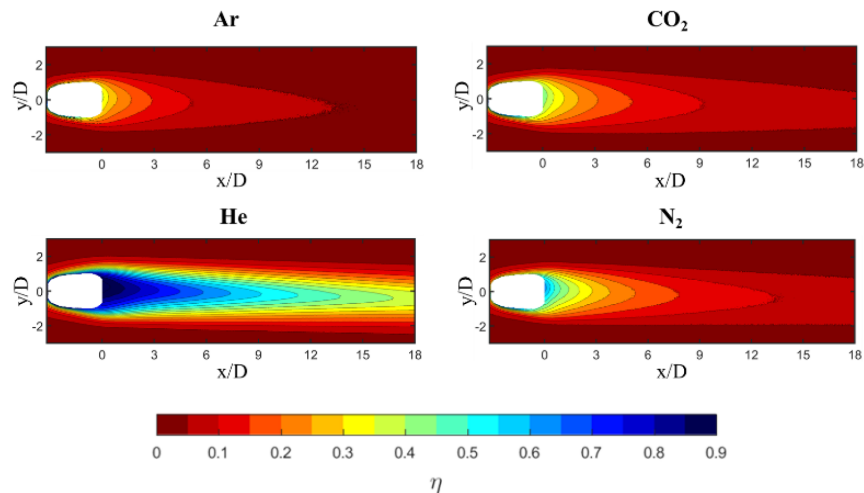
Figure 3. Contours of \eta at M = 0.25 , Tu = 0.67\% [13]
