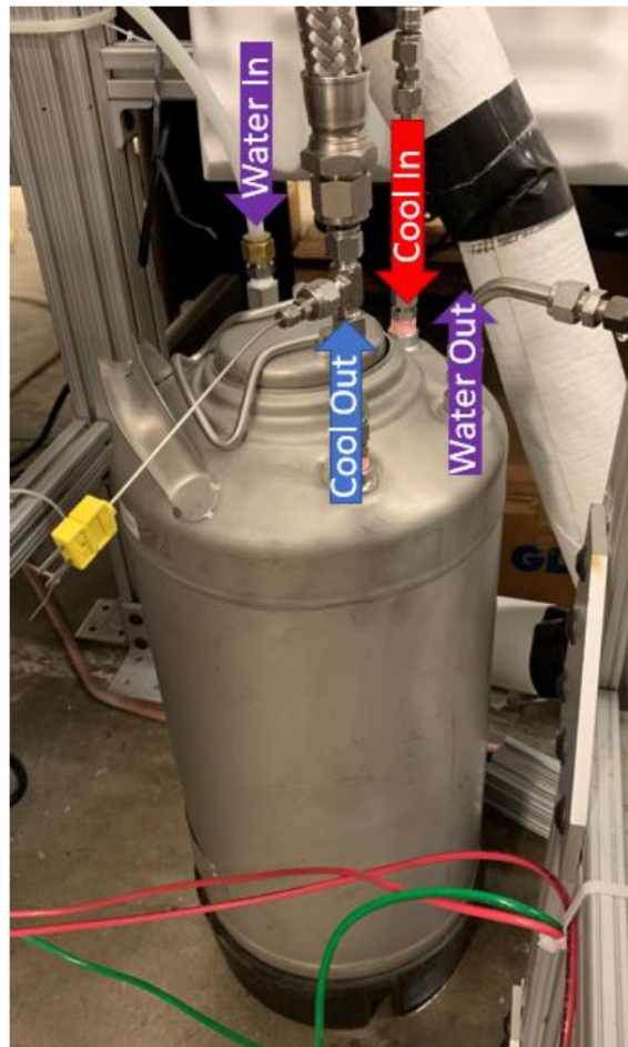
Figure 26. Water-cooling system used for coolant line [5].
