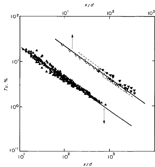
Figure 15. Decay of turbulence intensity downstream of SMS Grids. Curve fit: Tu = 1.13(x/d)^{-5/7} [26].
