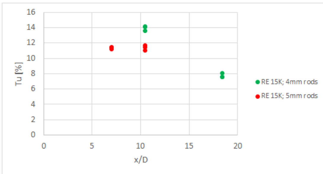
Figure 47. Turbulence decay downstream of the turbulence generator for Re_D = 15k .
