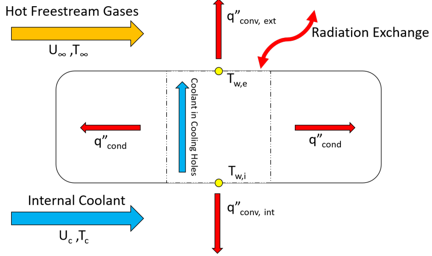
Figure 2. Modes of heat transfer in a cooled engine component.
