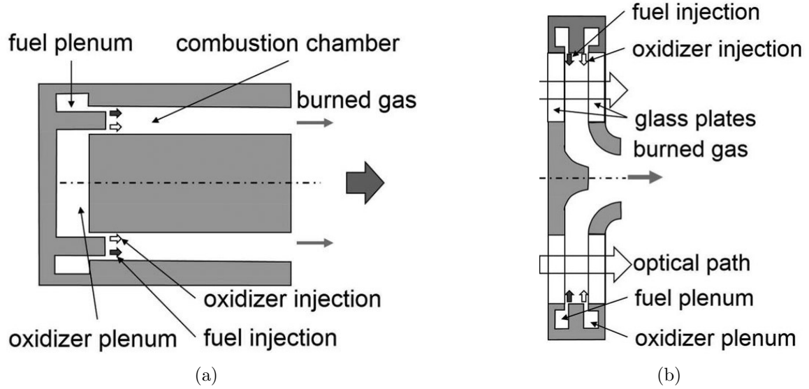
Figure 15. Basic comparison between an (a) Annular and (b) Radial RDE [2].
