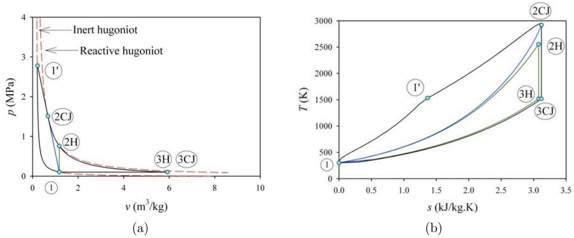
Figure 12. Humphrey Cycle (1-2H-3H-1), Fickett-Jacobs Cycle (1-2CJ-CJ-1), and ZND Cycle (1-1'-2CJ-3CJ-1) shown in (a) P-v and (b) T-s diagrams [14].
