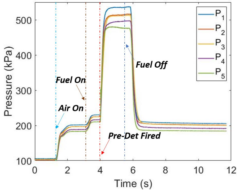
Figure 33. Sample pressure measurement from a test in stand-alone combustor configuration.
