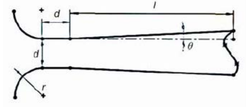
Figure 24. Cross-sectional view of sonic nozzle [24].
