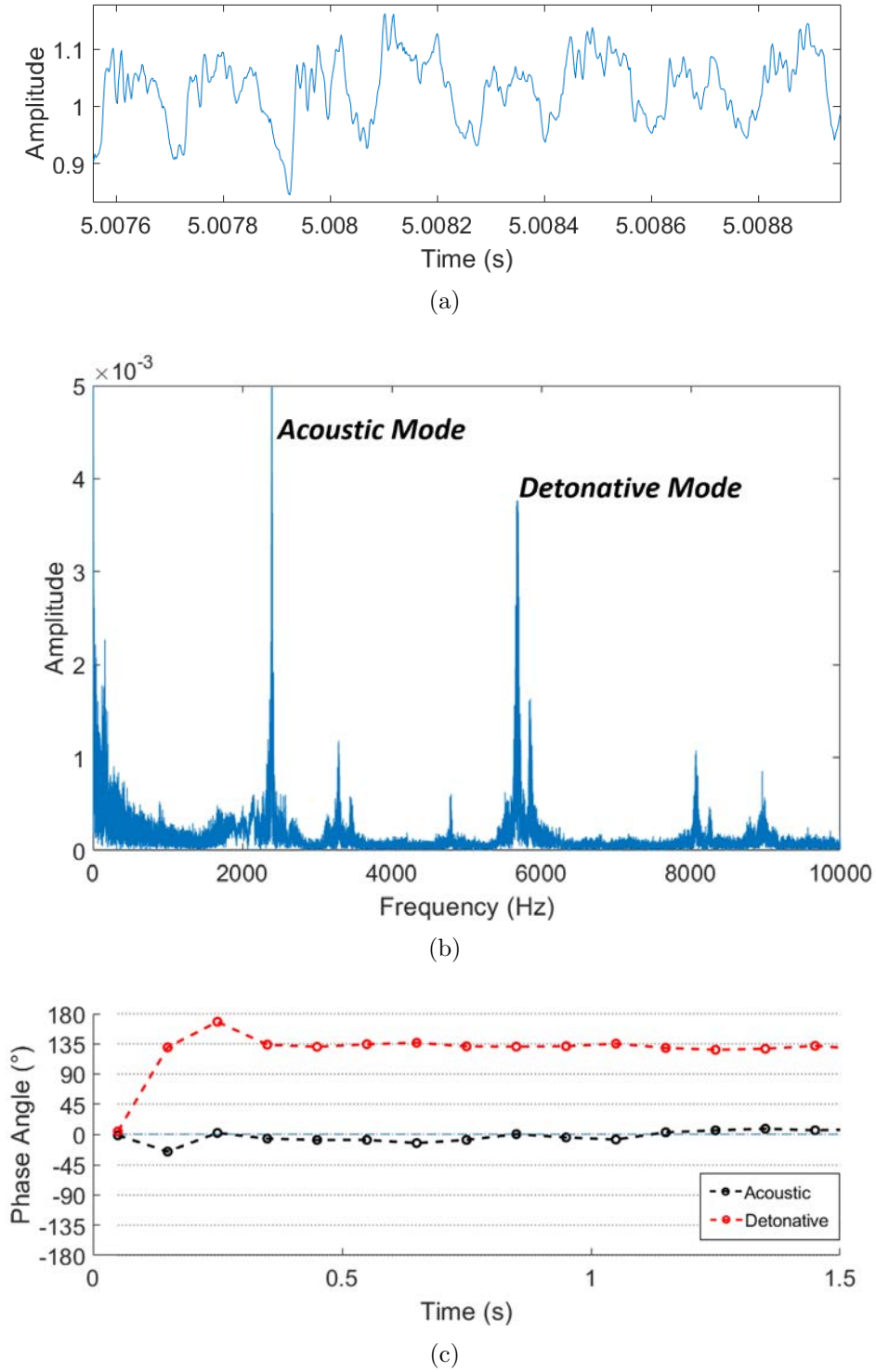
Figure 85. ITP measurements providing (a) transient signal, (b) FFT, (c) cross-correlation for both acoustic (2.4 kHz) and detonative (5.8 kHz) modes for BAT Configuration at h_c = 10.0 mm, \Phi = 1.0 with no vanes.
