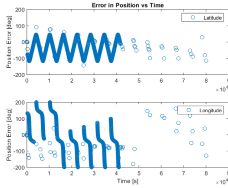
Figure 47. Woman (RANSAC/EKF)
