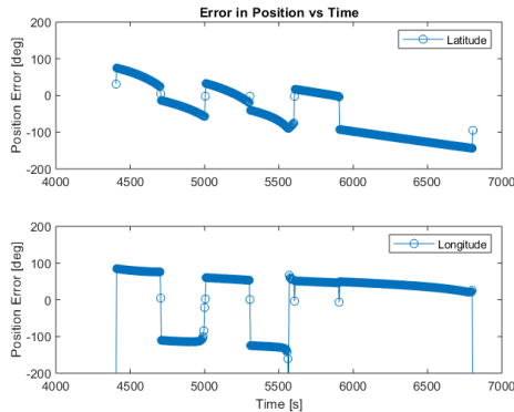
Figure 36. Short Run Veteran USA (No RANSAC/UKF) Figure 37. Short Run Veteran USA (RANSAC/EKF/Ground Track)
