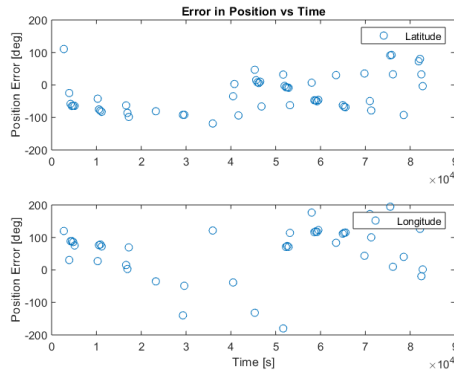
Figure 45. Veteran (RANSAC/No Filter)
