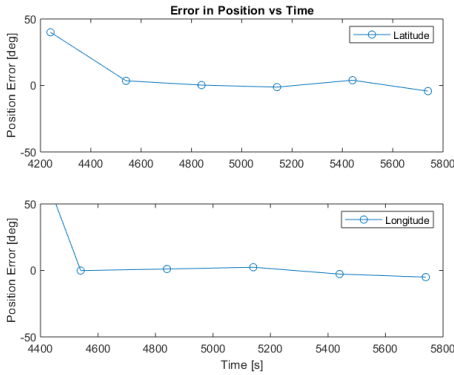
Figure 22. Short Run Woman (No RANSAC/No Filter)
