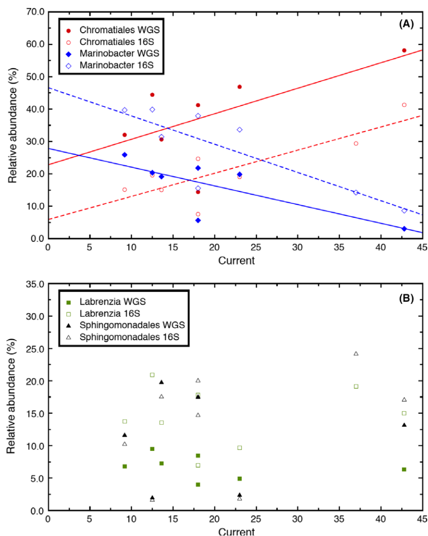
Fig. 3. Correlation of per cent abundance of (A) Marinobacter spp. (combined bin genomes) and the order Chromatiales (representing 'Ca. Tenderia electrophaga') to absolute current, as well as (B) Labrenzia sp. and the order Sphingomonadales (Kordiimonadales) using read counts associated with OTUs linked to longer 16S sequences or generated by whole-genome shotgun (WGS) sequencing and resolved by RAY-METABAT case 1b (BES key: 1 = 1031813, 2 = 2021213, 3 = 2031813, 5 = 3042313, 6 = 4021213, 7 = 4032113, 8 = 4040813).
