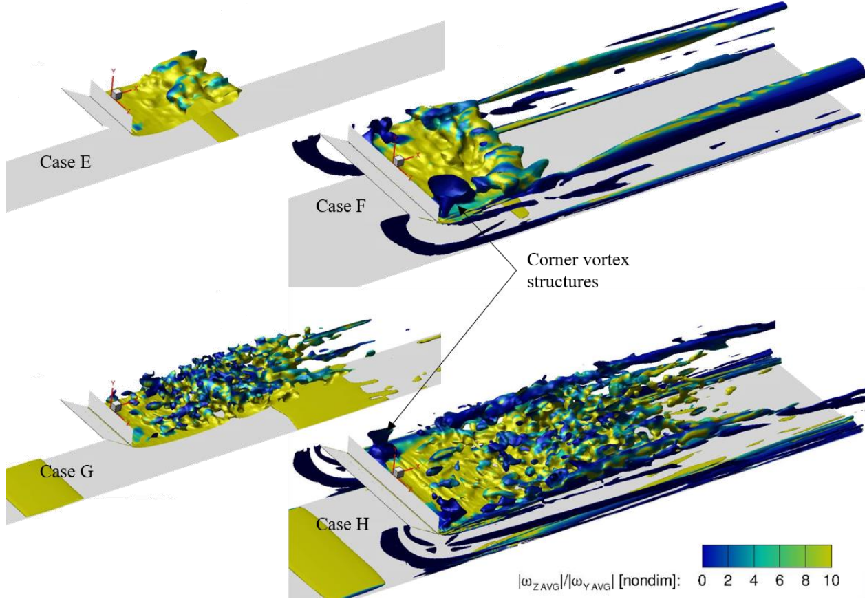
Fig. 12 Reacting case isosurfaces of Q -criterion colored by participation in either transverse or spanwise vortical structures. Only the bottom half of the domain is visualized to reveal the corner vortex structures.
