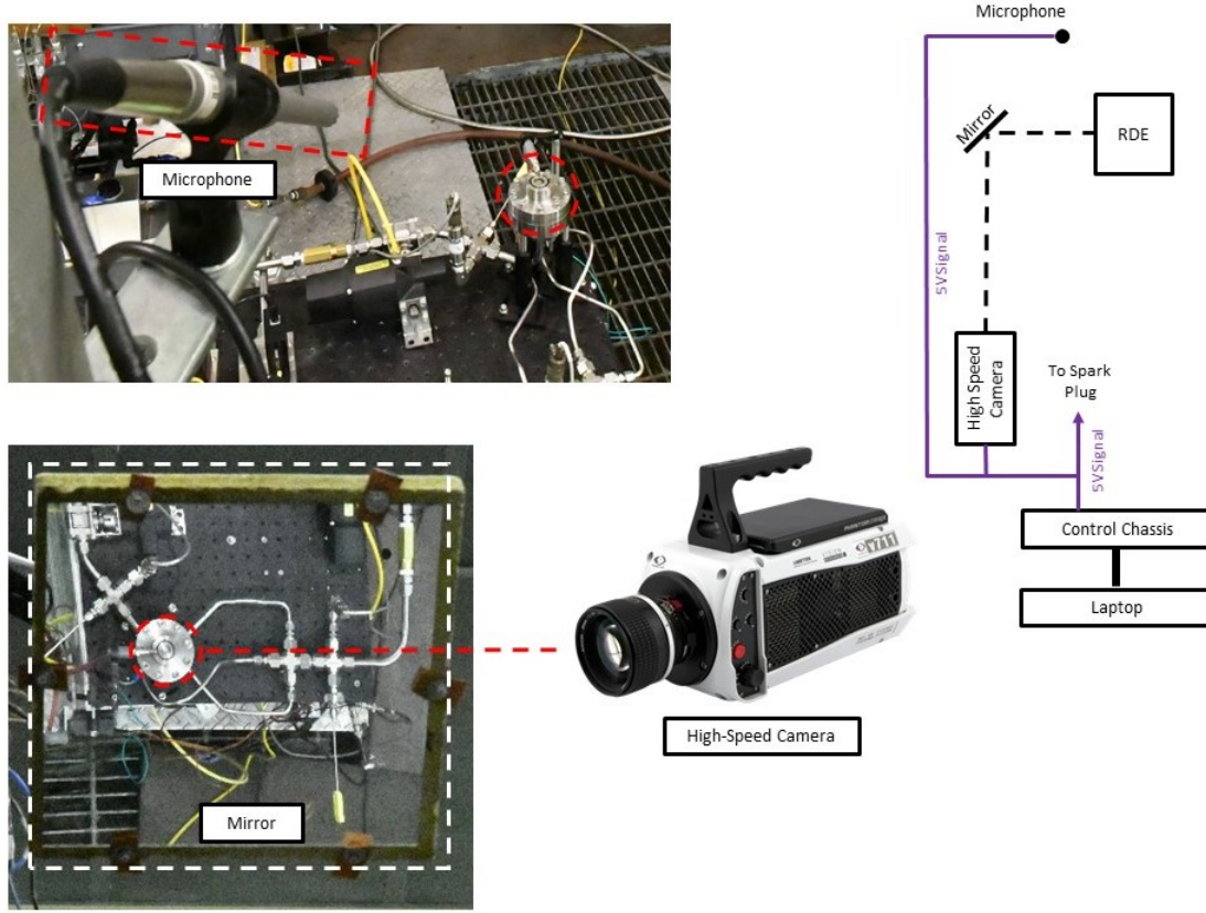
Figure 45. Layout of high-speed camera and microphone
