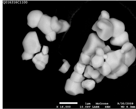
(b) \text{U}_3\text{O}_8 Particle that was incorrectly classified as ADU
