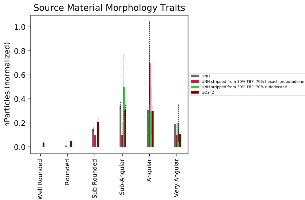
Figure 42. Source material morphology feature occurrence for step 3 of the lexicon chart.
