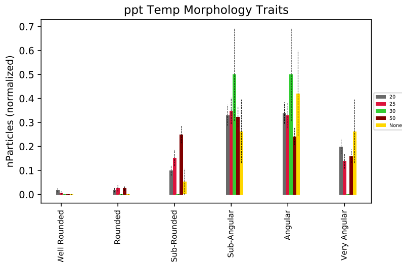
Figure 16. A step-wise comparison of particle morphology occurrence between creation condition parameters. In this case precipitation temperature [ ^{\circ}\text{C} ] is measured against particle angularity.
