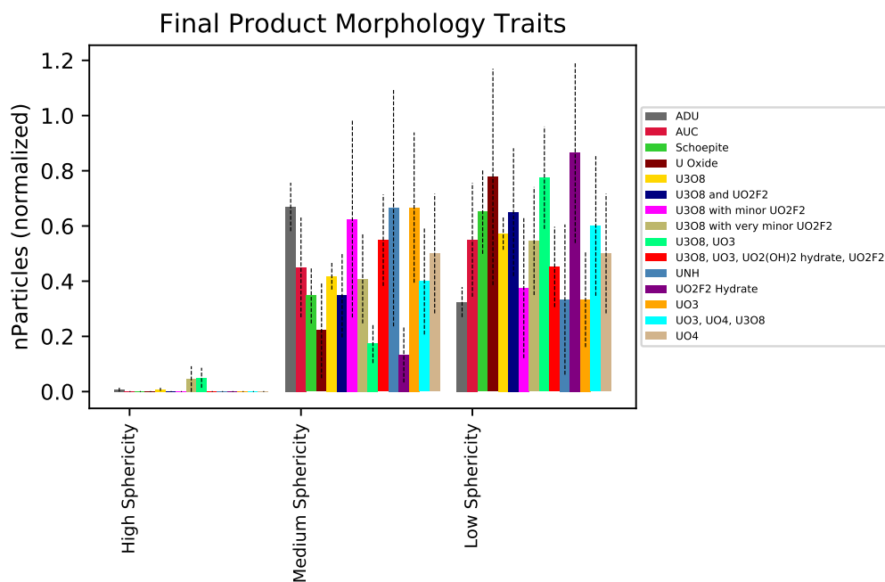
Figure 68. Final product morphology feature occurrence for step 4 of the lexicon chart.
