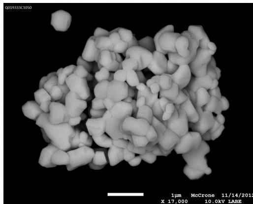
(b) ADU particle that was incorrectly classified as \text{U}_3\text{O}_8
