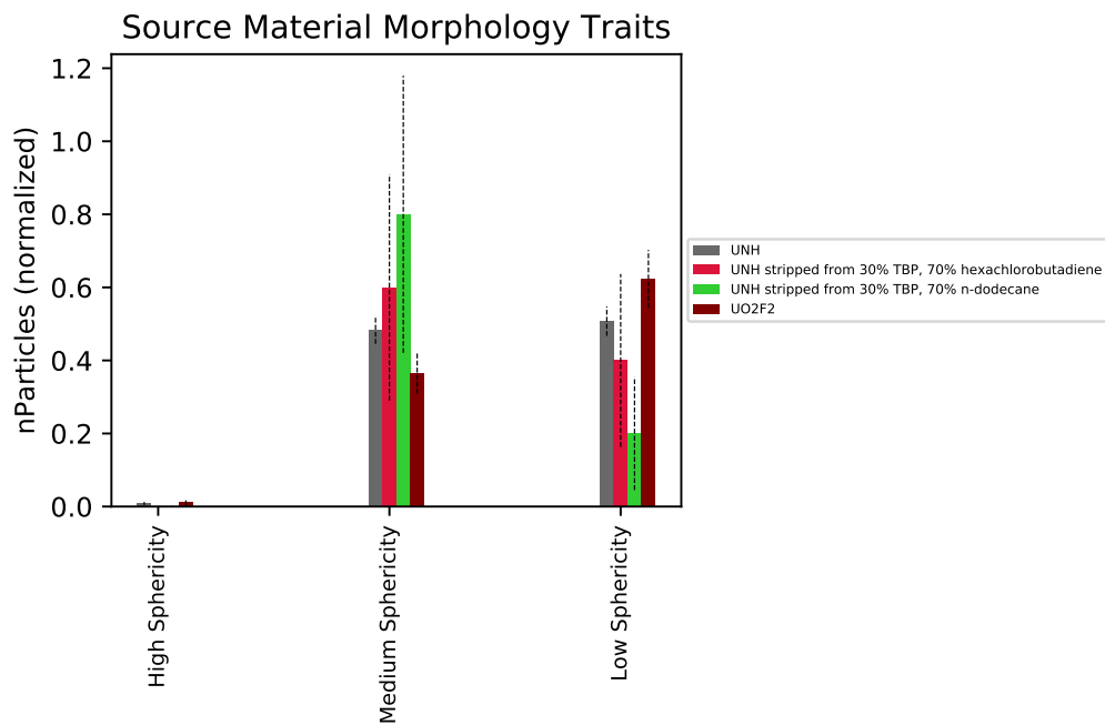
Figure 43. Source material morphology feature occurrence for step 4 of the lexicon chart.
