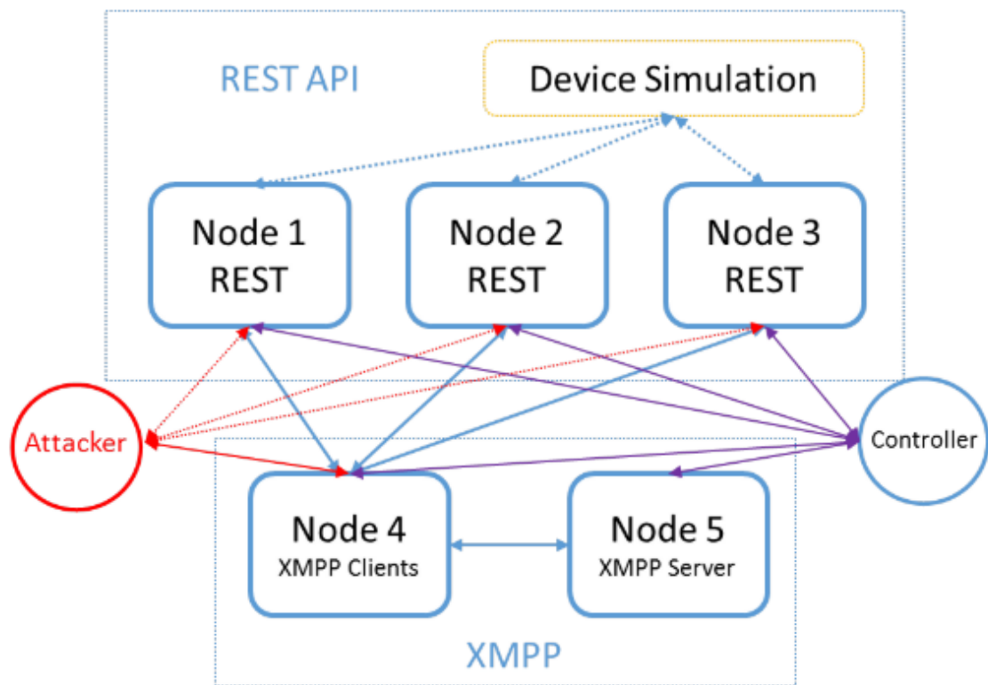
Figure 12. ThingPot Overview [57]
