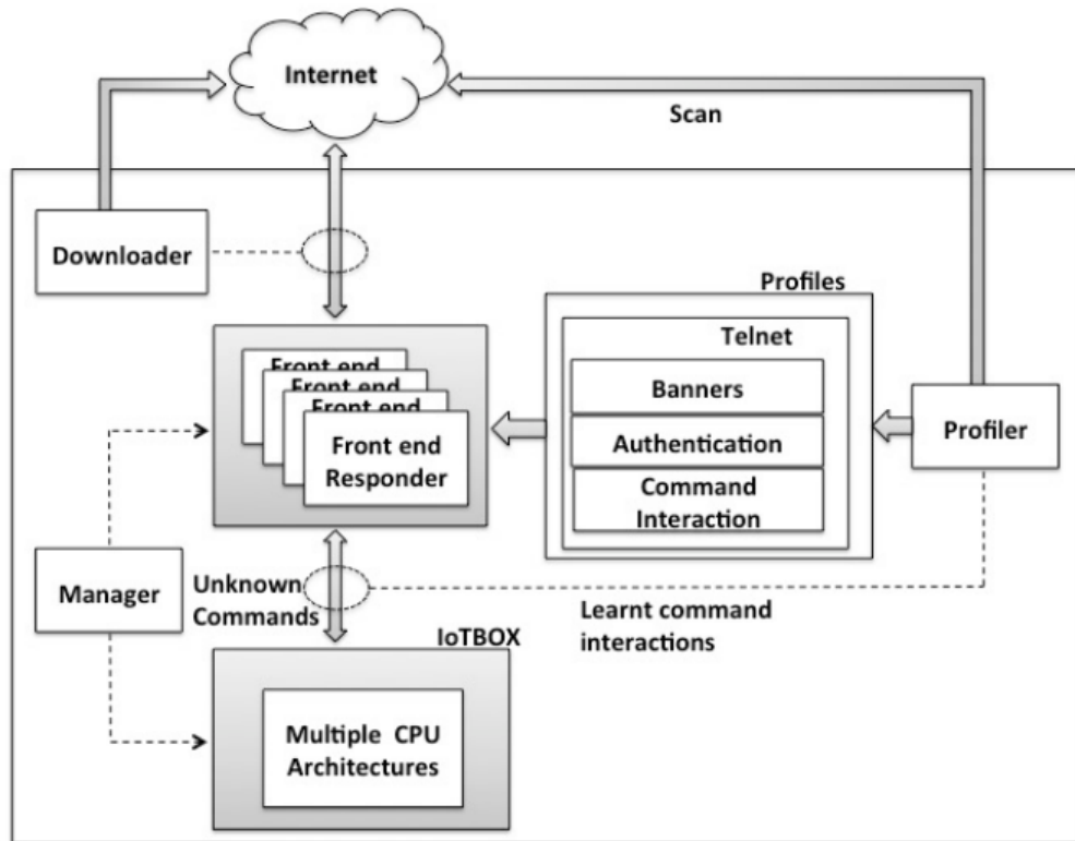
Figure 10. IoTPOt Overview [22]
