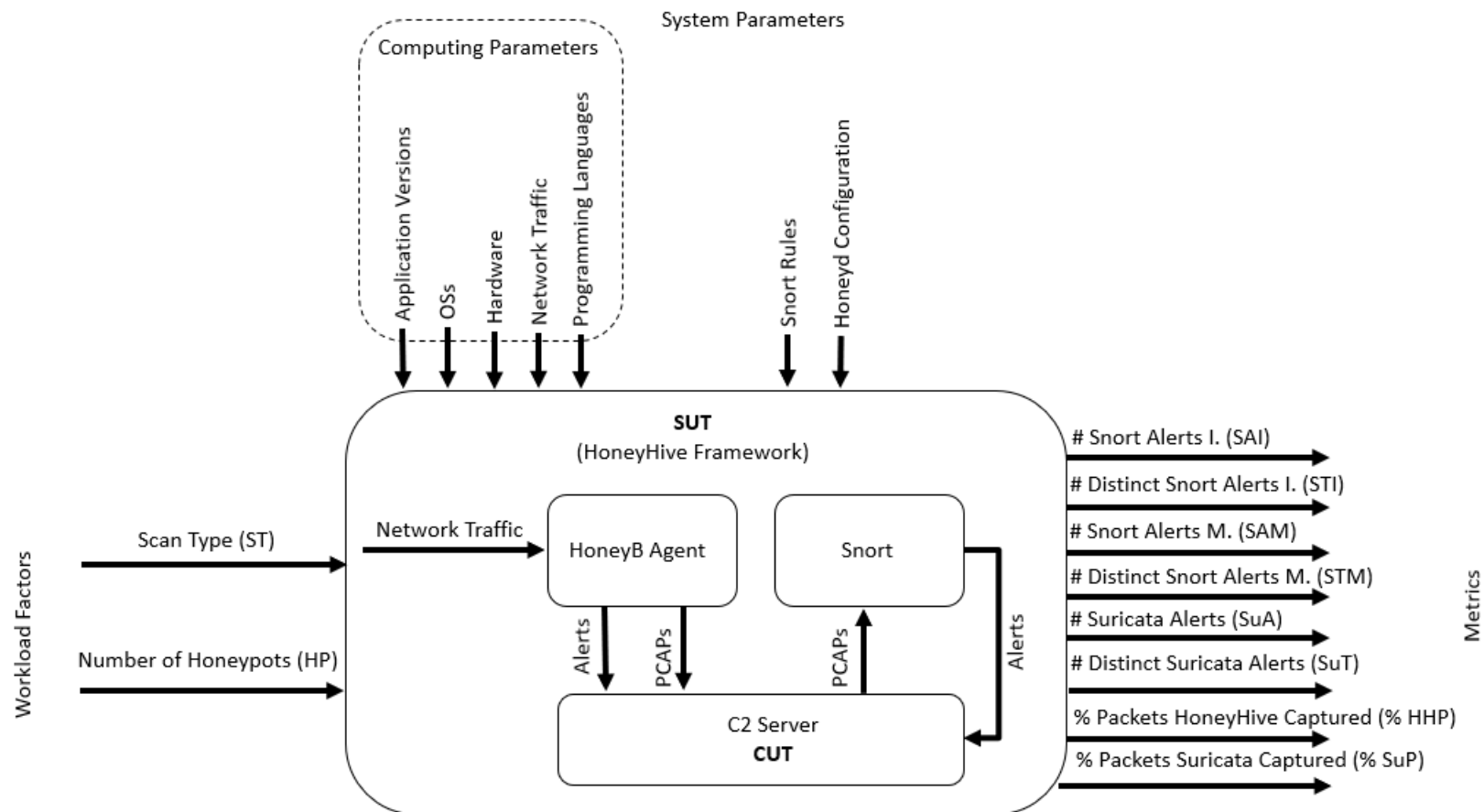
Figure 17. HoneyHive Framework
