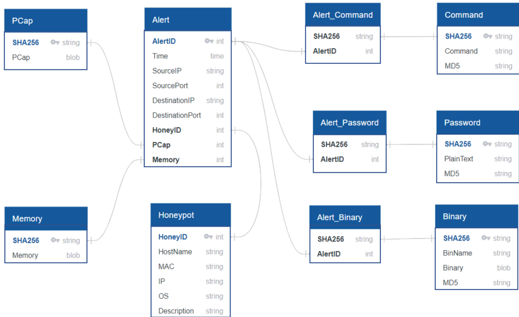
Figure 15. Database Schema
