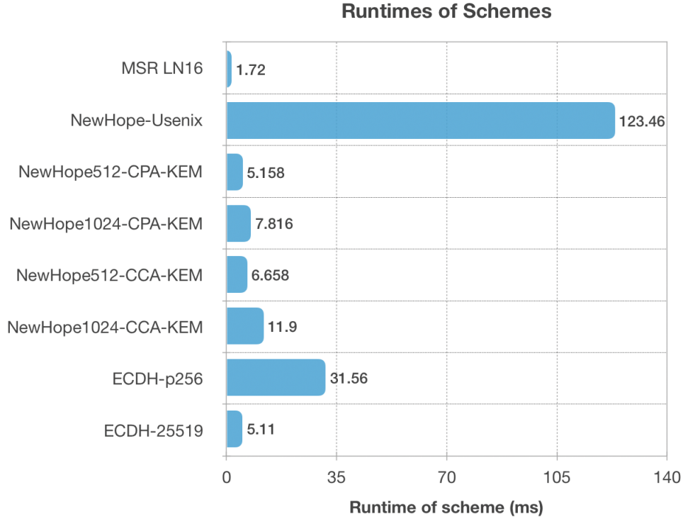
Figure 10: Comparison of the average runtime of schemes between NewHope mobile implementation to the work by Malina et al. [73](*)
