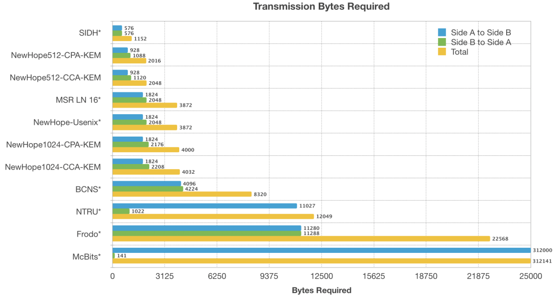
Figure 9: Comparison of the total number of bytes sent to achieve key establishment between NewHope mobile implementation to the work by Malina et al. [73](*)
