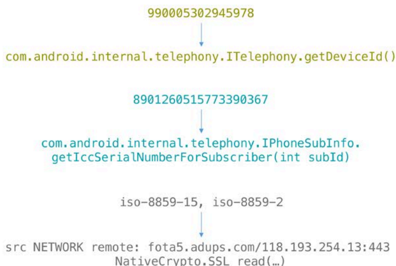
Figure 4.15: Three provenance examples from Adups 24-hour exfiltration.
