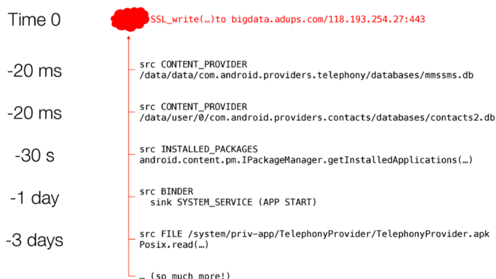
Figure 4.18: Timeline of reads of sensitive information relative to network send operation for 72-hour exfiltration.
