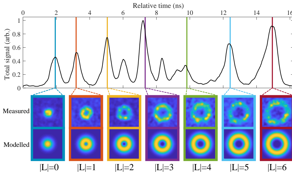
Fig. 3. The upper plot shows the integral intensity transmitted as a function of time from the 200 m length of OAM fiber. The vertical lines show the predicted arrival time of the optical modes. For each mode the measured intensity pattern and the respective modelled intensity of the OAM modes are shown. The unlabelled peaks in the plot are identified as higher order modes that were not included in the mode predictions. The images of the modes have been normalised giving each image the maximum contrast. The full data is shown in Visualization 3 .
