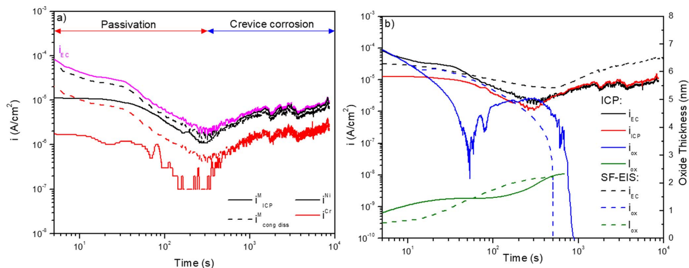
Figure 5. a) Calculated ICP-MS current densities for cation emission or dissolution versus the total element-specific current densities assuming congruent dissolution and b) ICP-MS and SF-EIS overall ( i_{EC} ), total dissolution ( i_{ICP} ), and oxidation ( i_{ox} ) current densities along with calculated film growth ( i_{ox} ) during passivation of Ni-22 Cr at +0.2 V SCE in 0.1 M NaCl pH 4. Instantaneous DC currents had their time convoluted in order to place them on the same scale as ICP-MS measurements.
