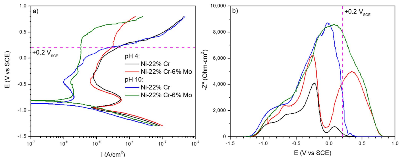
Figure 4. a) Current density and b) impedance variations during upward potentiodynamic polarization of Ni-22 Cr and Ni-22 Cr-6 Mo, wt%, in deaerated 0.1 M NaCl at pH 4 and 10 with the potential used in this study (+0.2 V SCE ) indicated.
