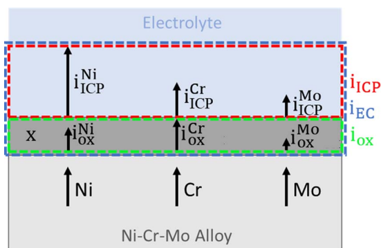
Figure 1. Schematic of the dissolution and oxidation reactions occurring for a Ni-Cr-Mo alloy with the corresponding current densities indicated.
