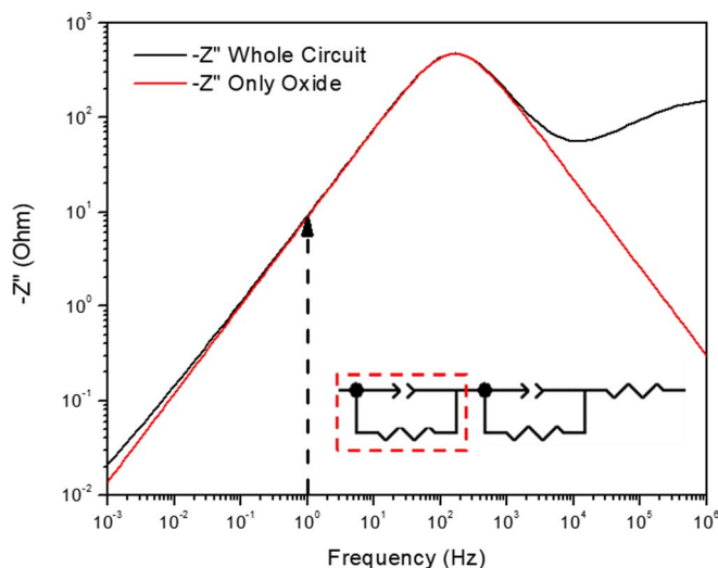
Figure 2. Comparison of the total -Z'' spectra of Ni-22 Cr-6 Mo, wt%, after 10 ks of potentiostatic polarization at +0.2 V_{SCE} in 0.1 M NaCl pH 4 versus a ZView simulation using a simplified circuit fit containing only a constant phase element and a resistor with the same measured Q_{CPE} , \alpha , and R_{ox} from fitting the total spectra, as indicated in the inset model where the red outline indicates the oxide portion, demonstrating that using -Z'' at 1 Hz correlates to the oxide properties.
