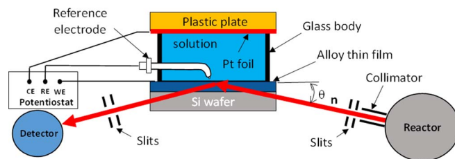
Figure 3. Schematic of the in-situ NR experiment at the D3 beamline of the NRU reactor.
