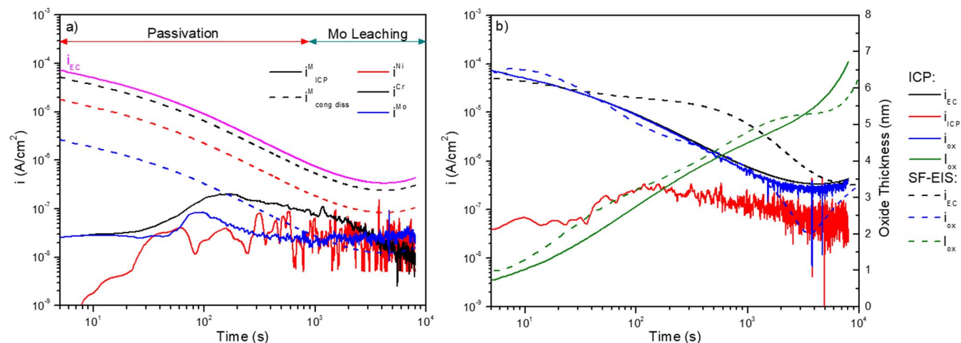
Figure 9. a) Calculated ICP-MS current densities for cation emission or dissolution versus the total element-specific current densities assuming congruent dissolution and b) ICP-MS and SF-EIS overall ( i_{EC} ), total dissolution ( i_{ICP} ), and oxidation ( i_{ox} ) current densities along with calculated film growth ( i_{ox} ) during passivation of Ni-22 Cr-6 Mo at +0.2 V SCE in 0.1 M NaCl pH 10. Instantaneous DC current densities had their time convoluted in order to put them on the same scale as ICP-MS measurements.
