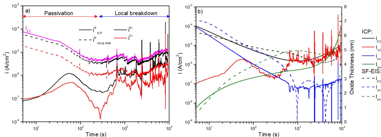
Figure 8. a) Calculated ICP-MS current densities for cation emission or dissolution versus the total element-specific current densities assuming congruent dissolution and b) ICP-MS and SF-EIS overall ( i_{EC} ), total dissolution ( i_{ICP} ), and oxidation ( i_{ox} ) current densities along with calculated film growth ( i_{ox} ) during passivation of Ni-22 Cr at +0.2 V SCE in 0.1 M NaCl pH 10. Instantaneous DC current densities had their time convoluted in order to put them on the same scale as ICP-MS measurements.
