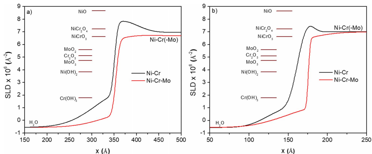
Figure 13. SLD profiles obtained for deposited Ni-20% Cr and Ni-20% Cr-10% Mo, wt%, films passivated up to +0.2 V SCE in a) 0.1 M NaCl pH 4 and b) 0.1 M NaCl pH 10 solutions with the theoretical SLD for various possible compounds shown to indicate their presence and distribution through the films.
