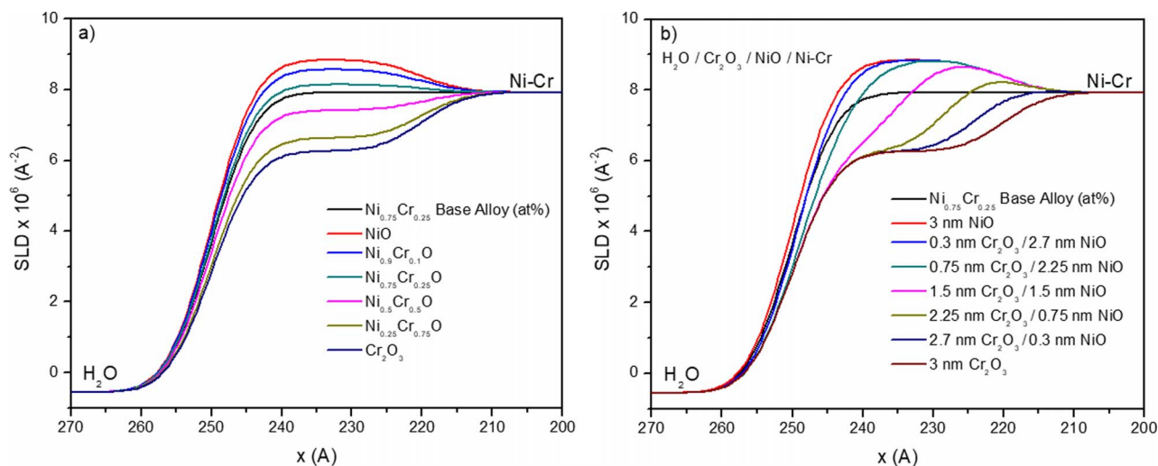
Figure 14. Simulated SLD profiles for a) a solute-captured rocksalt-structured oxide, \text{Ni}_{1-x}\text{Cr}_x\text{CrO}_x containing varying % \text{Cr}^{3+} and b) a bilayer oxide comprised of \text{Cr}_2\text{O}_3 and \text{NiO} with varying thicknesses of each conformal layer. An interfacial roughness of 5 Å was used to replicate the experimental parameters.
