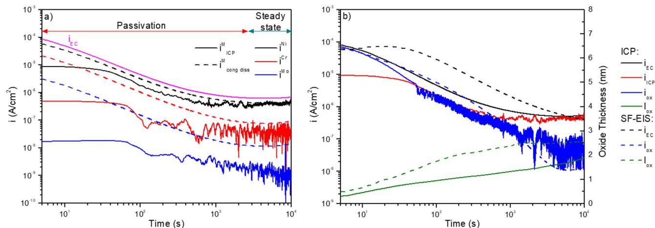
Figure 6. a) Calculated ICP-MS current densities for cation emission or dissolution versus the total element-specific current densities assuming congruent dissolution and b) ICP-MS and SF-EIS derived and overall ( i_{EC} ), total dissolution ( i_{ICP} ), and oxidation ( i_{ox} ) current densities along with calculated film growth ( i_{ox} ) during passivation of Ni-22 Cr-6 Mo at +0.2 V SCE in 0.1 M NaCl pH 4. Instantaneous DC currents densities had their time convoluted in order to place them on the same scale as ICP-MS measurements.
