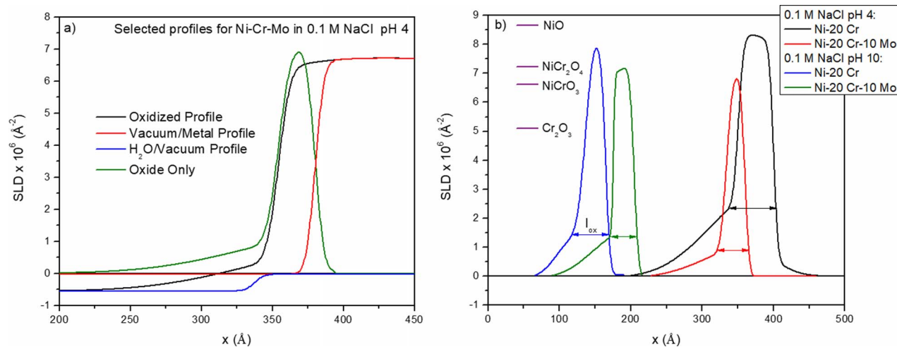
Figure 15. Analysis of the NR profiles given in Figure 13 where a) SLD profiles for the base metal on the Si substrate and for the electrolyte layer exposed to vacuum were simulated and subtracted from the overall SLD profile in order to obtain that of just the passive film for Ni-Cr-Mo in 0.1 M NaCl pH 4 and b) the oxide-only profiles for each alloy and environment combination are provided. The peak SLD correlates to the \text{Ni}^{2+} cation fraction (Figure 14a) and the approximate l_{\text{ox}} is indicated by the peak width.
