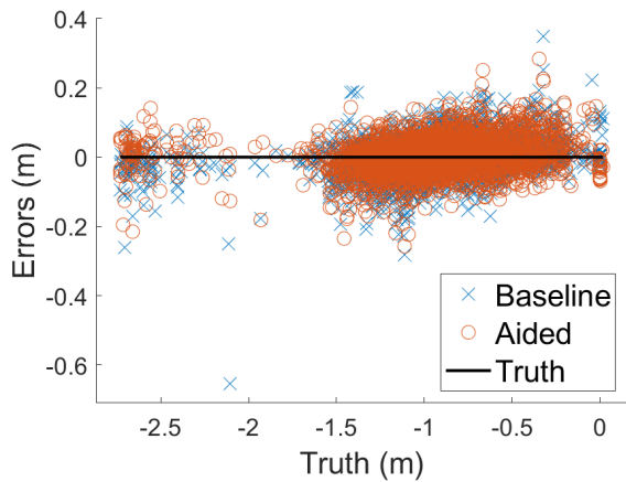
(e) 6-DoF Test Error - Translation Z
