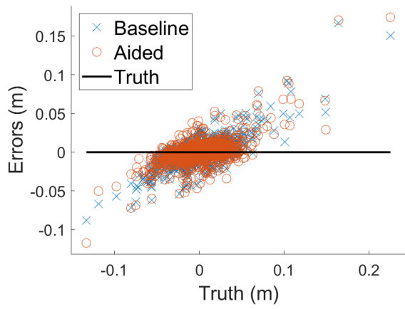
(a) 6-DoF Test Error - Translation X
