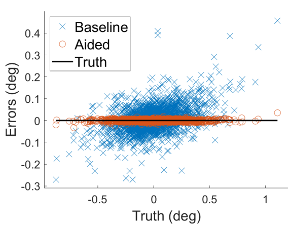
(a) 6-DoF Test Error - Rotation X
