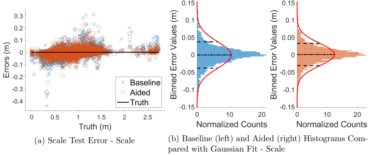
Figure 13: Test set errors for both the baseline and INS-aided Scale VO models.
