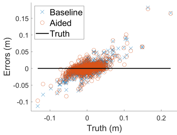
(a) Trans Test Error - Translation X
