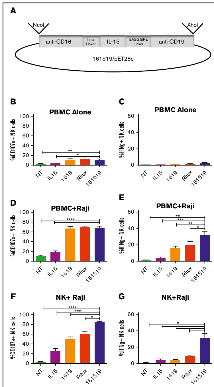
Figure 2. Functional validation of 161519 TriKE. (A) Simplified schema of 161519 TriKE construct, cloned into the pET28c vector via NcoI and XhoI restriction sites. The construct consists of 3 arms: an anti-CD16 scFv arm, IL-15 arm, and anti-CD19 scFv arm joined by 2 linkers (HMA and EASGGPE). Frozen PBMCs from healthy donors ( n = 6 ) were incubated with noted treatments (30 nM for everything but IL-15 [used at 0.3 nM]) to evaluate background CD107a expression (degranulation) (B) or intracellular IFN \gamma production (C) on CD56 ^{+} /CD3 ^{-} NK cells in a 4-hour assay. CD107a expression (D) and intracellular IFN \gamma (E) were also evaluated under the same conditions as stated before on NK cells within the PBMCs but in the presence of Raji targets at a 2:1 effector/target ratio. To evaluate the priming effects of the molecules on NK cells before target encounter, noted treatments (30 nM for everything but IL-15 [used at 0.3 nM]) were incubated overnight with enriched NK cells, and then CD107a (F) or IFN \gamma (G) was assessed after a 4-hour coculture with Raji targets on the next day ( n = 5 ). One-way analysis of variance (ANOVA) with repeated measures was used to calculate differences against the 161519 group. Error bars indicate the mean \pm standard error of the mean. Statistical significance are determined as *P < .05 , **P < .01 , ***P < .001 , and ****P < .0001 . NT, no treatment; Ritux, rituximab.
