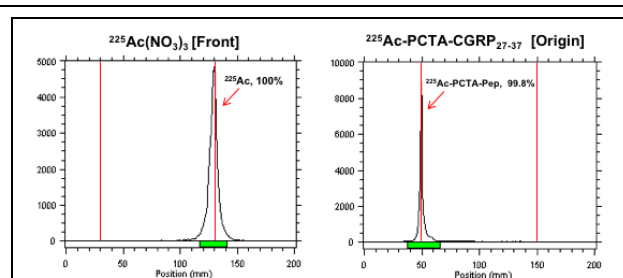
Fig. 2: Radiochemical purity of ^{225}\text{Ac} -PCTA-CGRP 27-37 by Radio-TLC.
