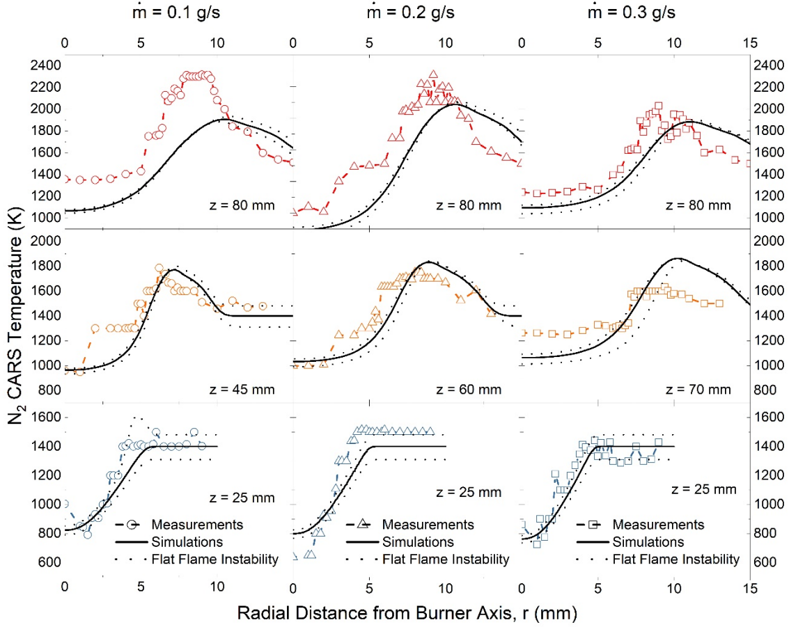
Fig. 53-Temperature profiles of propane gas jet from numerical simulations (solid lines) and N 2 CARS thermometry (dashed lines) for a propane flow rate of 0.1 g/s, 0.2 g/s and 0.3 g/s.
