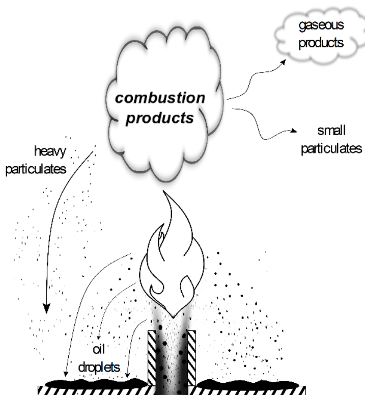
Fig. 4-Diagram of wellhead spray combustion behavior and the fate of the two-phase fuels.
