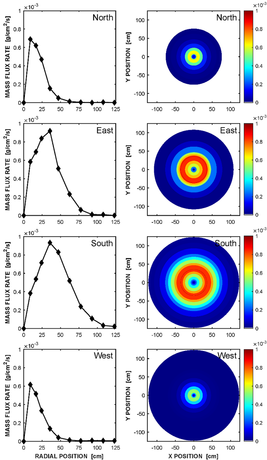
Fig. 6. Oil mass flux rate profiles (left) and full 2D distributions (right) for the four collection directions from one burn efficiency experiment.
