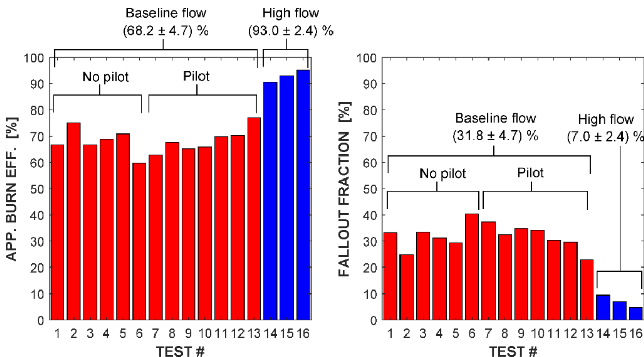
Fig. 51-Apparent burn efficiency (left) and fallout fraction (right) for gas/oil spray flame tests at two different flow conditions: baseline flow (3 g/s gas; 16 g/s oil) and high flow (6 g/s gas; 32 g/s oil).
