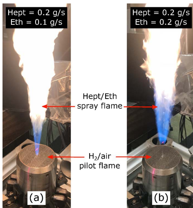
Fig. 18-Photographs of spray flame for two operating conditions: ethane flow rate = (a) 0.1 g/s and (b) 0.2 g/s. For both conditions, heptane flow rate = 0.2 g/s.
