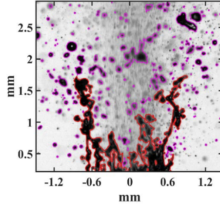
Fig. 42-Sample DBI image take near the exit of the OPA for a condition with 0.2 g/s of air and 0.4 g/s of water.
