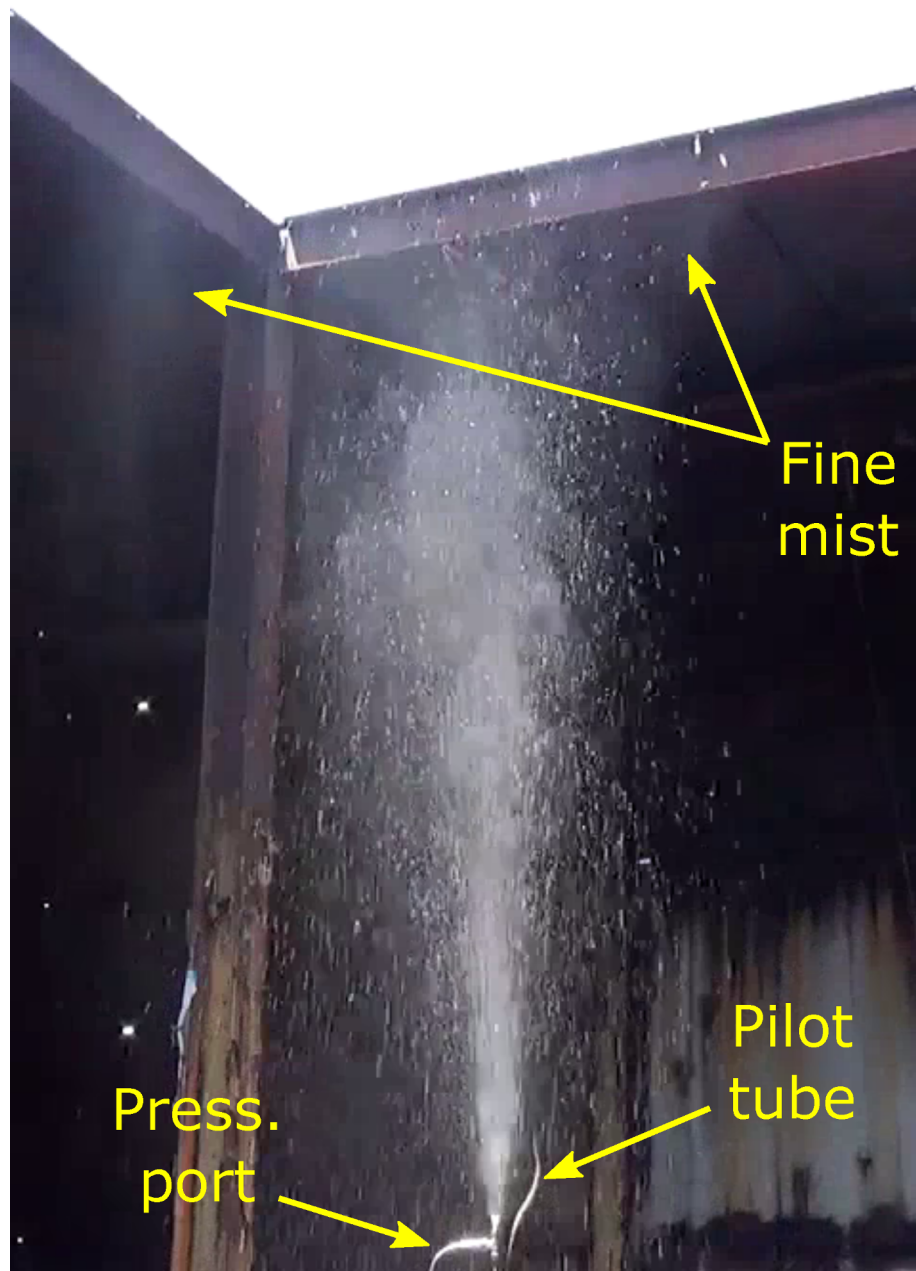
Fig. 8. Video/image of non-reacting air/water spray, taken from an air/water test on 21 May 2019. View is from the southeast corner of the chamber.
