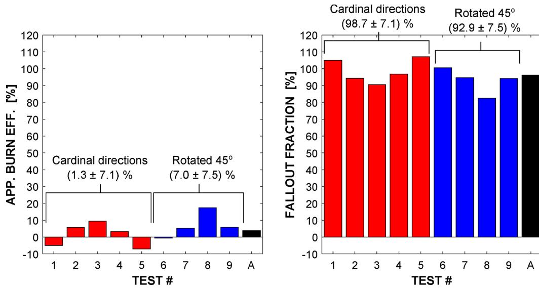
Fig. 9. Apparent burn efficiency (left) and fallout fraction (right) for non-reacting air/water spray tests.
