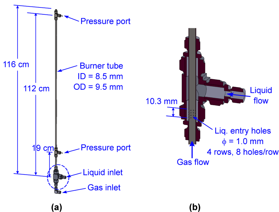
Fig. 2. Schematic of (a) overall burner and (b) gas-liquid mixing tee.
