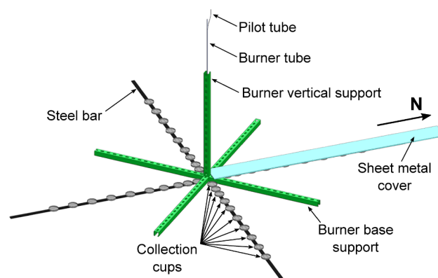
Fig. 4. Isometric view of experimental setup for collection of oil fallout.
