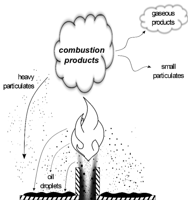
Fig. 1. Schematic illustrating wellhead ignition/burning and oil fallout.
