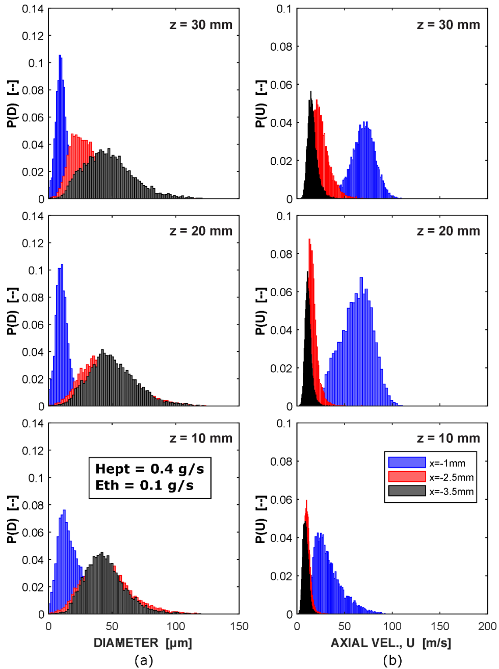
Fig. 36-Histograms of (a) droplet diameter ( D ) and (b) axial velocity ( U ) for selected radial locations, at each of three different heights ( z = 10\text{ mm} , 20\text{ mm} , 30\text{ mm} ). Heptane flow rate = 0.4\text{ g/s} ; ethane flow rate = 0.1\text{ g/s} .
