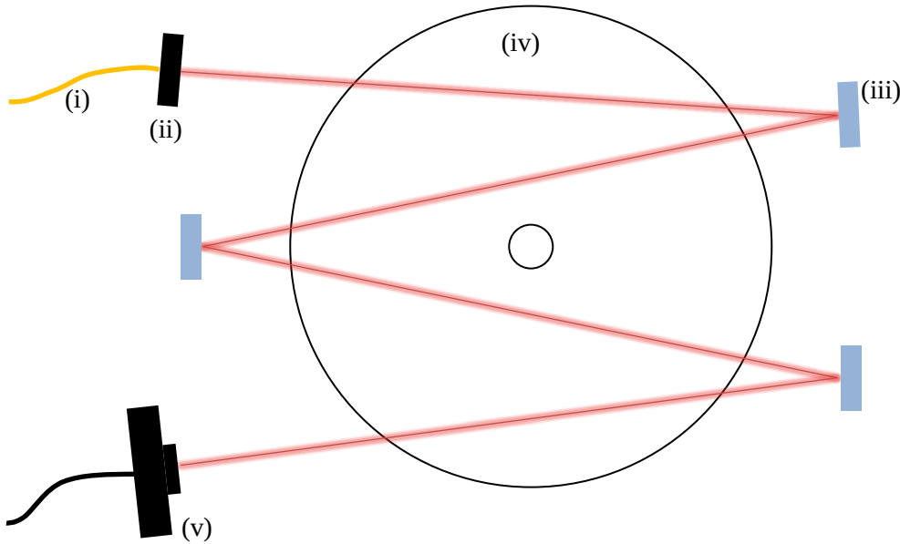
Fig. 55-Diagram of TDLAS experiment (top view). The laser is produced by a tunable diode laser, transmitted through a fiber (i), transmission optics (ii), reflected by mirrors across the hot exhaust gases above the burner (iv), and then into receiving optics and a photodiode (v).
