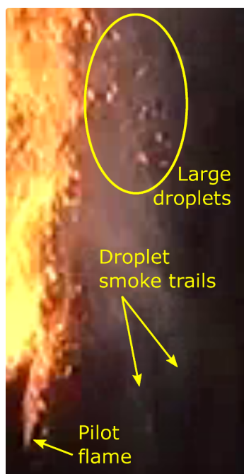
Fig. 11. Magnified view of boxed area in Fig. 10, showing large burning droplets and smoke trails from partially burned droplets falling to the ground.
