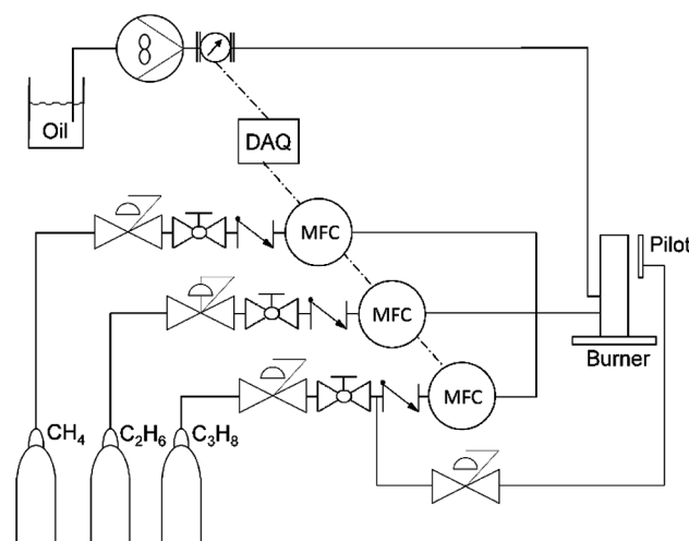
Fig. 3. Plumbing schematic for burn efficiency experiments.
