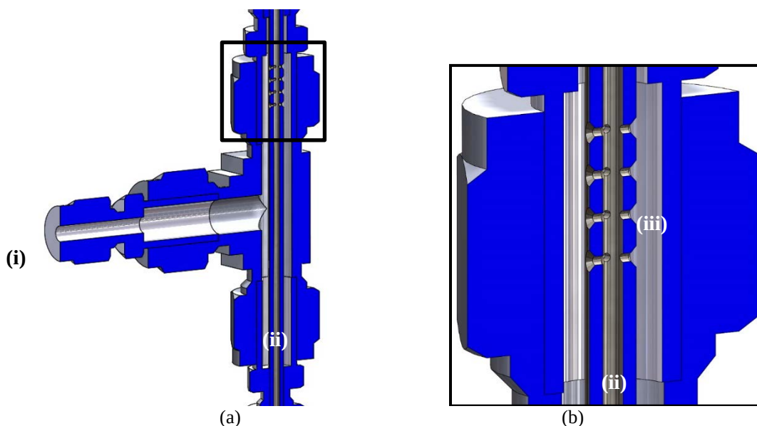
Fig. 17-Cross-sectional images of the (a) entire mixing tee and the details of the (b) mixing section. Liquid flows into the tee through the (i) side port while gas flow from the (ii) bottom along the length of the jet. The liquid then flows through several small ports drilled into the side of the jet (iii) to distribute the liquid into a thin film with a low velocity flow.
