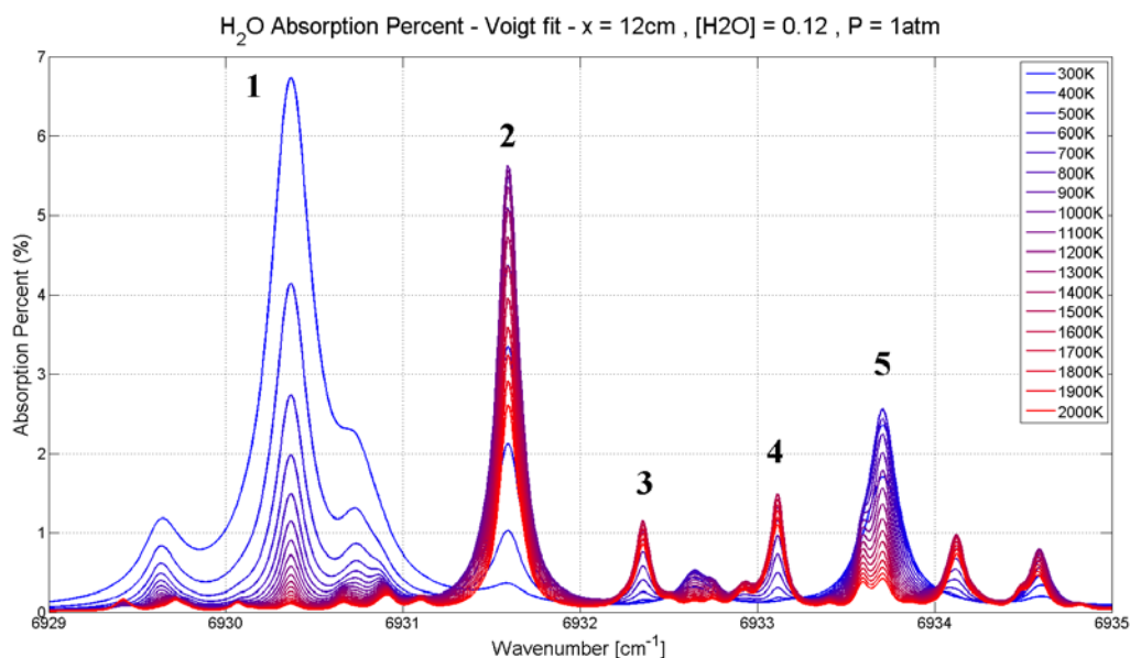
Fig. 56-Theoretical profiles of water vapor absorption features at temperature from 300 to 2000 K.
