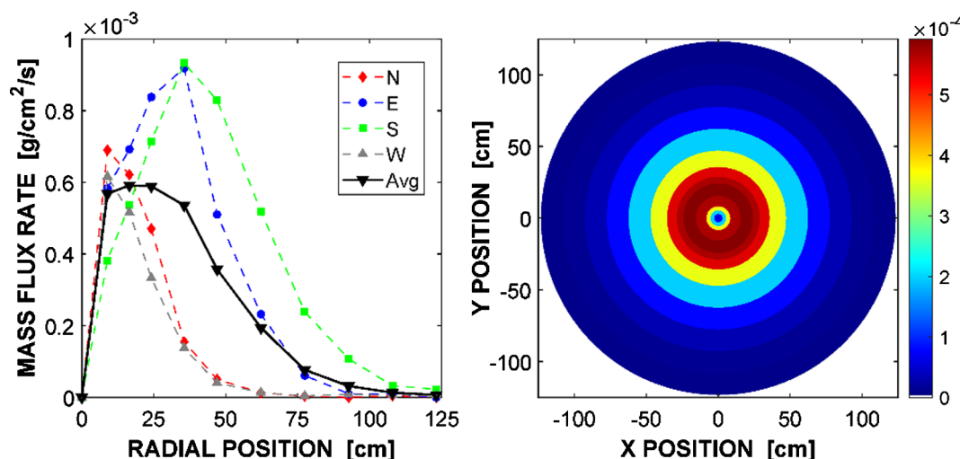
Fig. 7. Individual oil mass flux rate profiles and average profile (left) and full 2D distribution (right) based on average profile.
