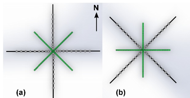
Fig. 5. Overhead schematic of two experimental configurations: (a) standard version with fallout collection in cardinal directions; (b) alternate version with fallout collection directions rotated 45°.
