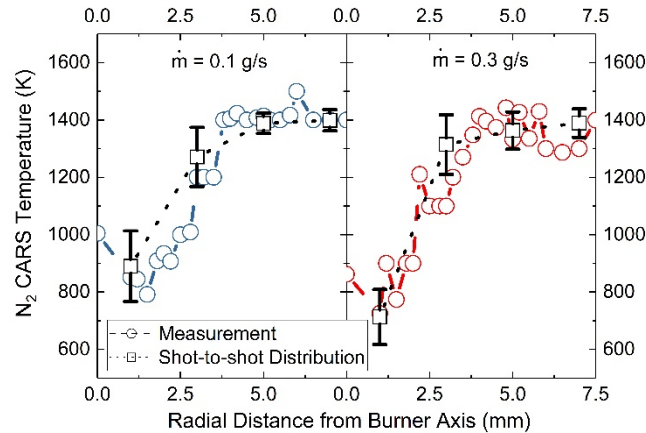
Fig. 54-Shot-to-shot analysis of the distribution in temperature at various locations in the radial profile at z = 25 mm for two flow rates.
