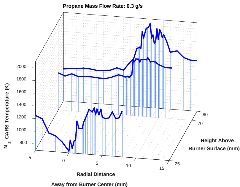
Fig. 27-N 2 thermometric results of a jet flame at 0.3 g/s of propane at 25, 70 and 80 mm above the burner surface.
