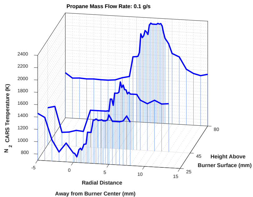
Fig. 25- N_2 thermometry results of a jet flame at 0.1 g/s of propane at 25, 45 and 80 mm above the burner surface.
