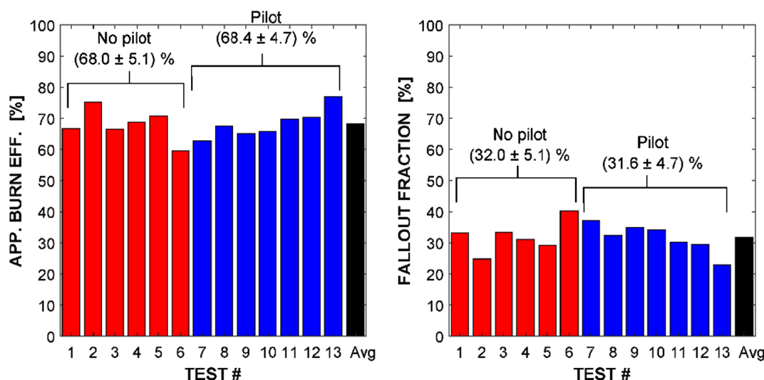
Fig. 13. Apparent burn efficiency (left) and fallout fraction (right) for gas/oil spray flame tests at the baseline flow condition (3 g/s gas; 16 g/s oil), including tests both without and with a small propane pilot flame.
