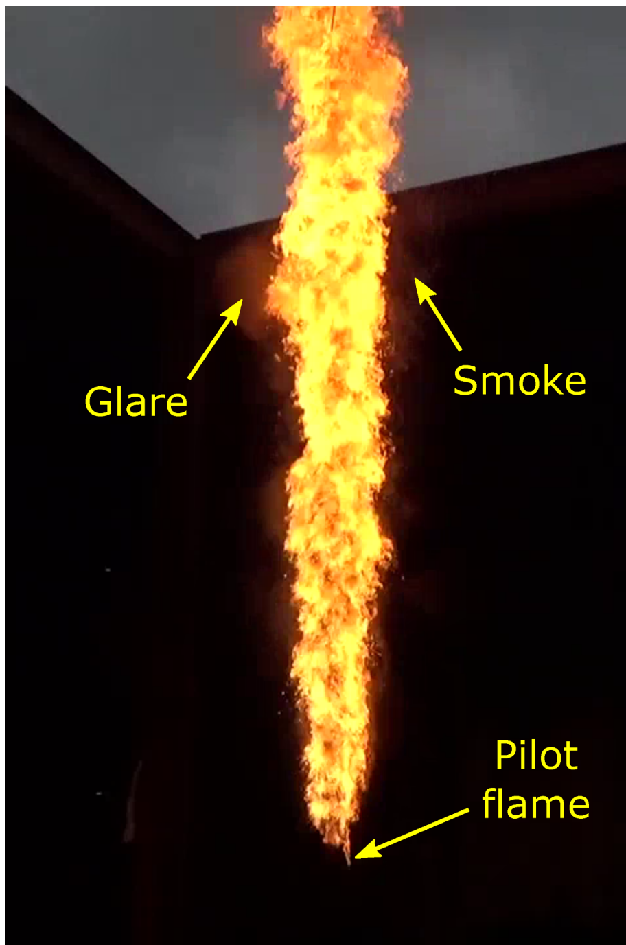
Fig. 12. Video/image of gas/oil spray flame for high flow condition (6 g/s gas, 32 g/s oil), recorded during a burn test on 14 May 2019. View is from the southeast corner of the chamber.
