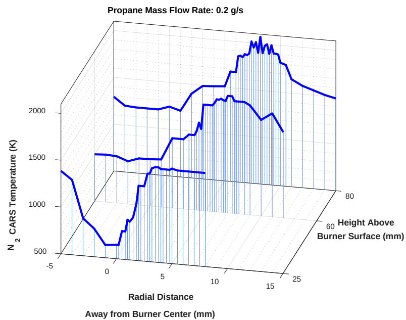
Fig. 26- N_2 thermometry results of a jet flame at 0.2 g/s of propane at 25, 60 and 80 mm above the burner surface.
