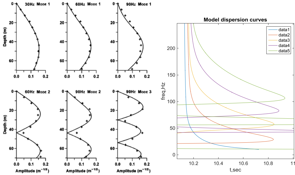
Figure 3.9 Model of \psi_l(z) functions for SWARM experiment conditions (left) and modeled dispersion curves for modes 1-5 (right)
