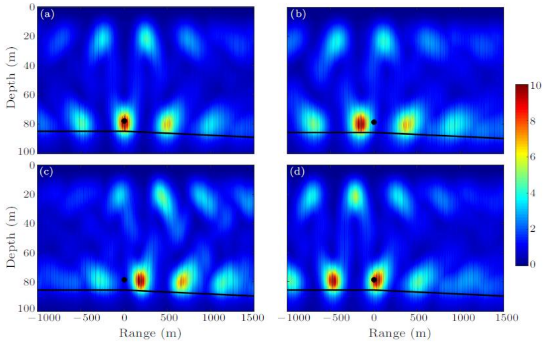
Fig. 1.8. Sensitivity for the position shift of focusing wave field generated by the TRM to the bottom parameters. The sound speed is 1750 m/s and the density is 1.9 g/cm 3 in the bottom for forward wave propagating. The sound speed and density for back-propagating are (a) 1750 m/s and 1.9 g/cm 3 , (b) 1700 m/s and 1.9 g/cm 3 , (c) 1850 m/s and 1.9 g/cm 3 , and (d) 1750 m/s and 1.5 g/cm 3 . In each panel, the black dot denotes the position of the sound source, and the bathymetry is indicated by a thick black line.
