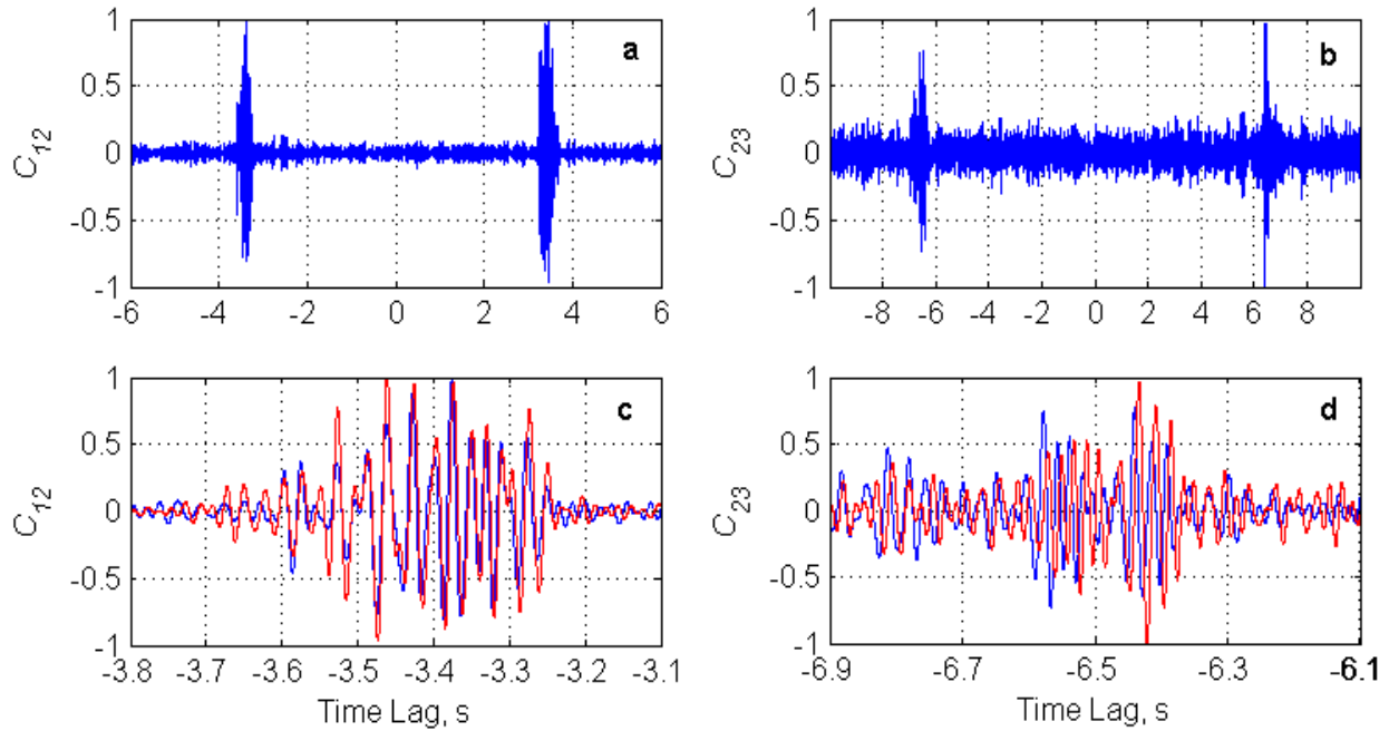
Fig. 1. 3. Cross-correlation functions of ambient noise in the Straits of Florida. (a) Measured cross-correlation functions C_{12}(t) for the 1-2 instrument pair in the 20–70 Hz frequency band. (b) Same as (a) but for the 2-3 instrument pair. (c) Fine structure of the cross-correlation function C_{12}(t) at negative time delays (blue) and of the time-reversed cross-correlation function C_{12}(-t) at t > 0 (red). (d) Same as (c) but for the 2-3 instrument pair.
