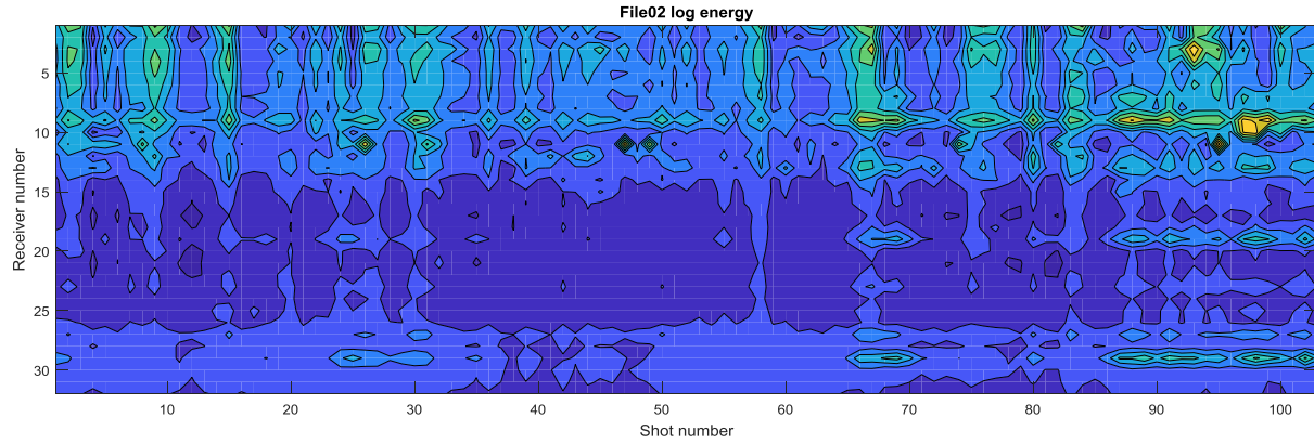
Figure 3.5 File02.mat visualized as signal energy for each airgun shot. Air gun location depth was 15 m. GMT time: 07:10:00-07:46:00.
