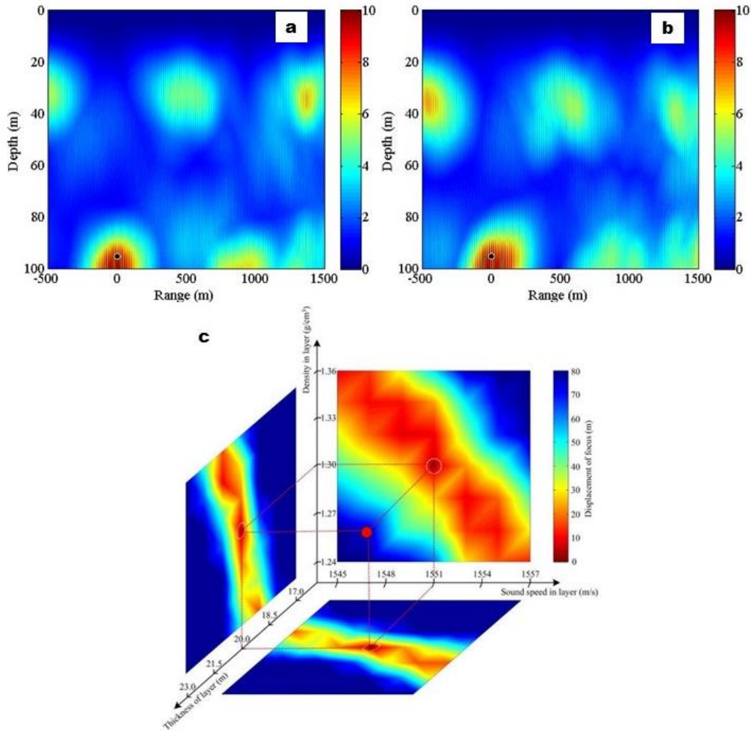
Fig. 1.5. Time-reversal of the acoustic noise cross-correlations measured in the Straits of Florida. The negative (a) and positive (b) time-delay parts of the cross-correlation function C_{12}(t) of noise recorded by instruments 1 and 2 are back-propagated in the environmental model obtained through a geoacoustic inversion. The normalized peak intensity of the back-propagated acoustic field in the vertical cross-section of the waveguide is shown by color. The black dot indicates position of the virtual sound source. Panel (c) shows the absolute value of the horizontal displacements of the main focus from the virtual sound source, which are caused by deviations of the sound speed, density, and thickness of the sediment layer from their optimal values. The plot is obtained by back-propagating the negative time-delay part of C_{12}(t) .
