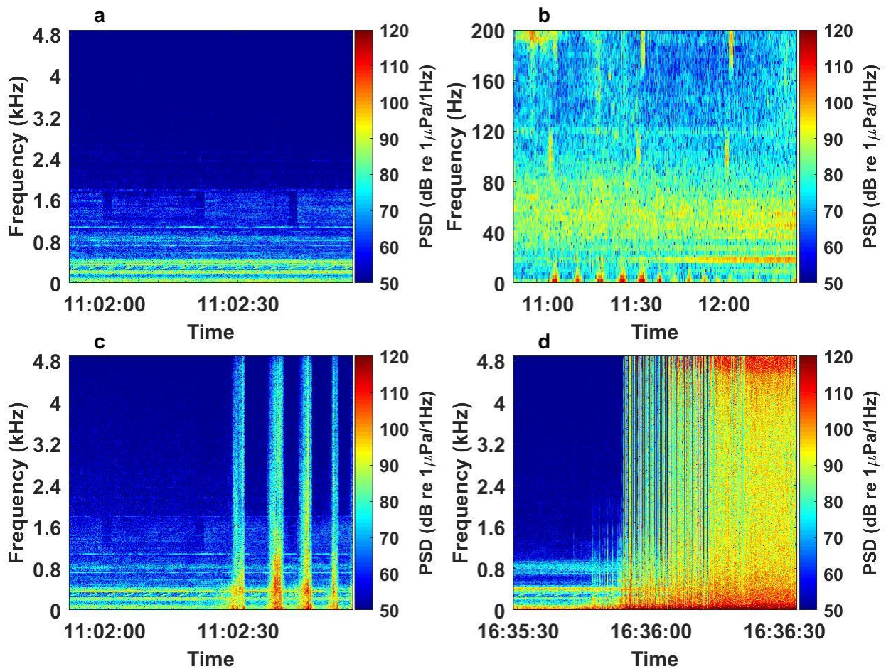
Figure 5.6. Spectrograms of acoustic field recorded by hydrophones on vertical (VLA) and horizontal (HLA) arrays during passage of a train of nonlinear internal waves. Spectrograms are shown of acoustic pressure on a VLA hydrophone at depth of 62 m (a); low-frequency part of the acoustic pressure on the same hydrophone (b); on a hydrophone in the middle of HLA (c);
