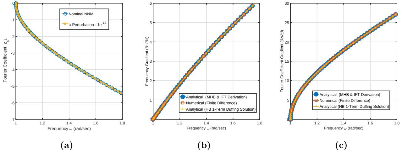
Fig. 44: Comparison of the gradients of the SDOF duffing oscillator with pure hardening nonlinearity. (a) Nonlinear Normal Modes. (b) Frequency gradient. (c) Fourier coefficient gradient.
