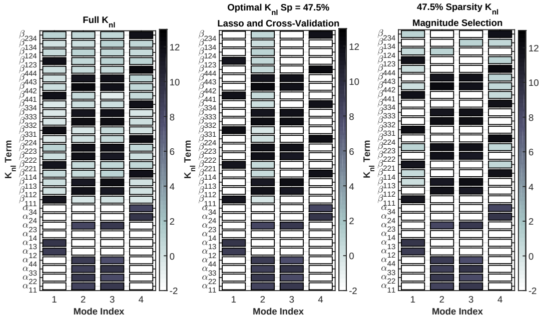
Fig. 15: Nonlinear stiffness coefficient matrices for three different sets of sparsity approaches 1.) The Least Squares solution (all terms shown would be retained), 2.) the optimal solution identified via cross-validation (terms in white are eliminated), and 3.) a solution in which terms with the smallest magnitude are removed (terms in white are eliminated).
