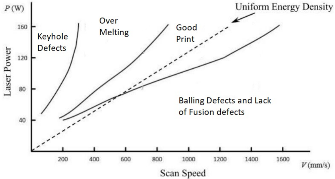
Figure 4. Velocity vs. Power showing the optimal printing balance. The regions represent various density effects. This curve does not come from Inconel 718. However, despite differing alloys, the graph consists of the same general regions [1].
