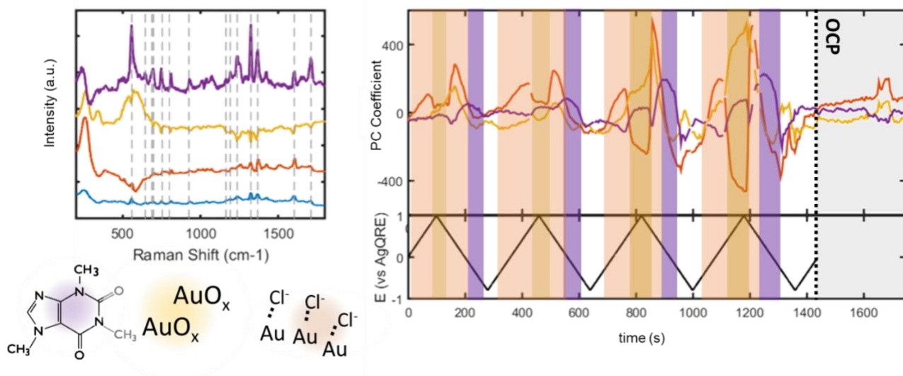
Figure 13. Principal component Analysis of the caffeine experiment. The eigenvectors of the data matrix can be interpreted spectrally.
