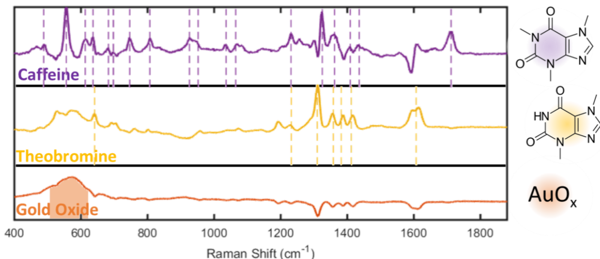
Figure 14. Separation of similar molecules by PCA of EC-SERS experiments. Eigenvectors extracted from a total of 700 spectra, t \sim 3500 \text{ s} . One can clearly identify the presence of caffeine peaks on the 4 th PC (top), while the 3 rd shows theobromine vibration bands (middle), and the 2 nd primarily contains the broad mode associated with gold oxide, albeit with a parasitic presence of theobromine bands due to correlation between theobromine adsorption and oxide presence.
