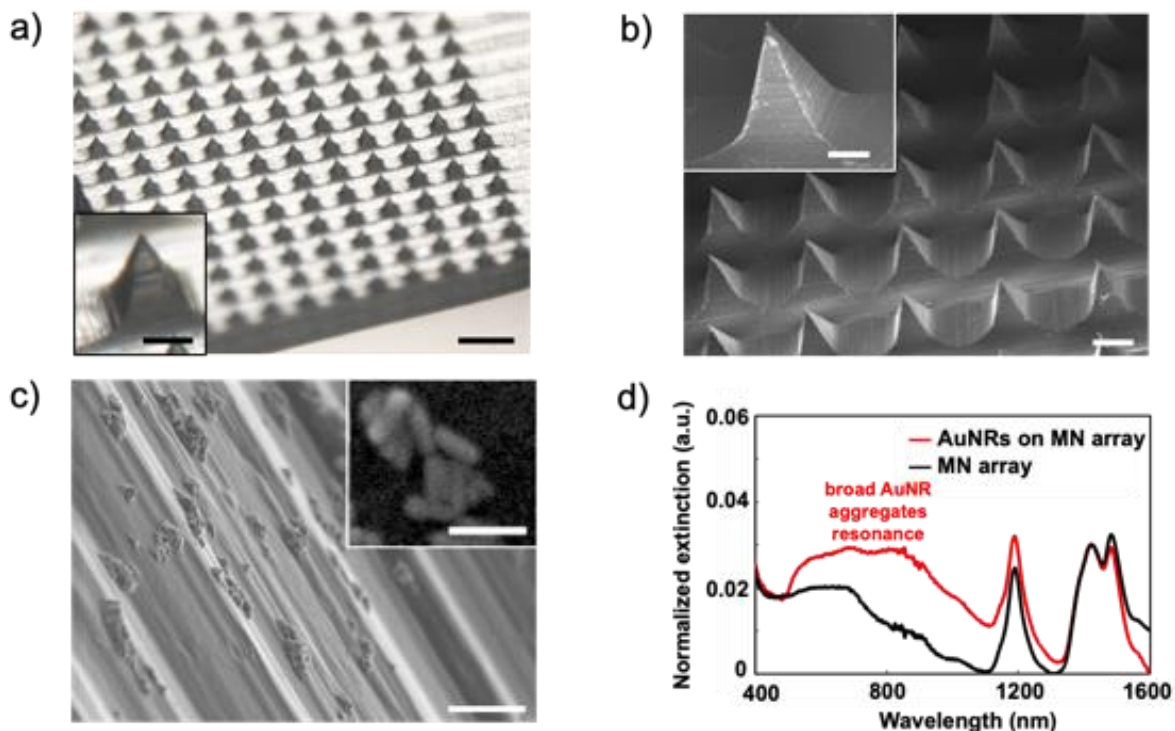
Figure 2. Optical characterization of plasmonic microneedle arrays. a) optical image of the microneedle arrays (scale bars: 500 \mu\text{m} and 100 \mu\text{m} (inset)), b) SEM image of the microneedle arrays (scale bars: 200 \mu\text{m} and 100 \mu\text{m} (inset)), c) SEM image of AuNRs on a microneedle tip
