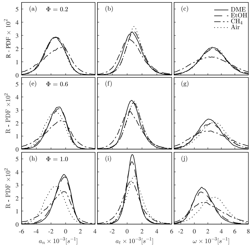
Fig. 12: PDF of the rate of strain along the reactant fluid surface ( R ) for DME, EtOH and \text{CH}_4 at varying \Phi . The dotted line indicates the mixing case (i.e. air with \Phi = 0.0 ) for reference. First column: Normal strain; Second column: Tangential strain; Third column: Vorticity. First row: \Phi = 0.2 ; Second row: \Phi = 0.6 ; Third row: \Phi = 1.0 .
