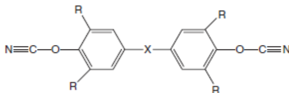
Figure 2 General structure of cyanate ester monomers where the linkage X and substituent R are chemical structures that vary across the polymer family [18].
