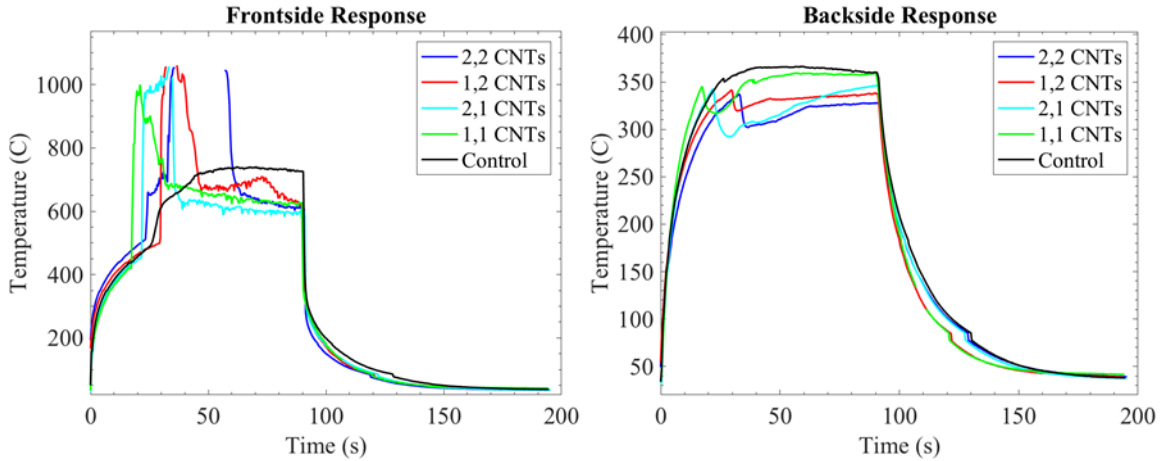
Figure 43. Thermal response of the average hottest pixel when the hybrid samples with 1-2 CNT center and outer layers were exposed to an average irradiance of 6.48 \text{ W/ cm}^2 . The control contained no CNT layers and is annotated in black.
