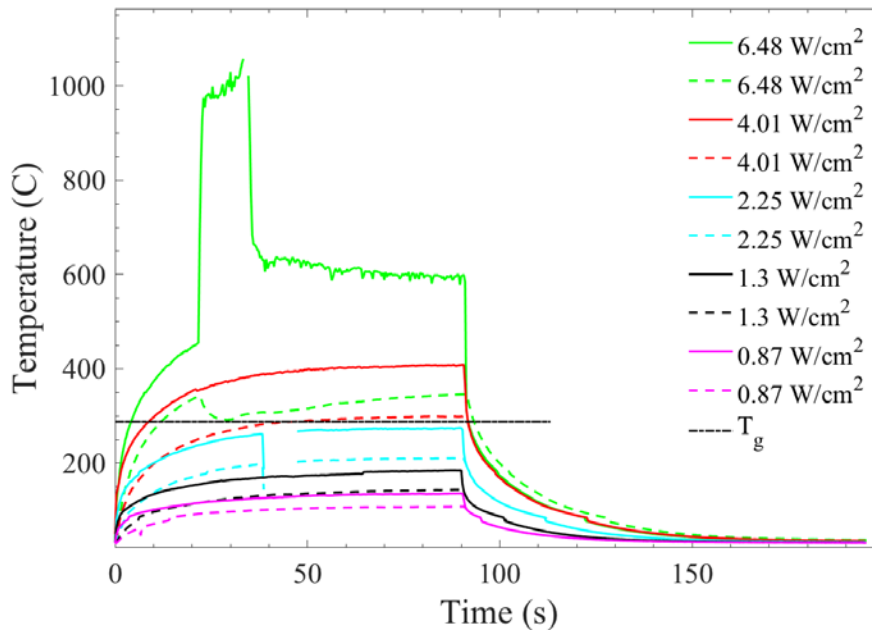
Figure A. 9 Thermal response of Sample 3.6 (2 CNT Center Layers, 1 CNT Outer Layers) repeatedly exposed to various irradiances. Solid lines are frontside curves, dashed lines are backside curves.
