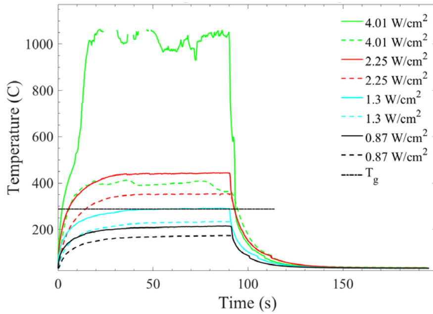
Figure A. 18 Thermal response of Sample 2.3 (20 CNT plys, 45-degree orientation) repeatedly exposed to various irradiances. Solid lines are frontside curves, dashed lines are backside curves.
