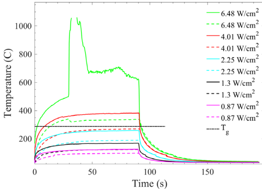
Figure A. 10 Thermal response of Sample 3.7 (1 CNT Center Layers, 2 CNT Outer Layers) repeatedly exposed to various irradiances. Solid lines are frontside curves, dashed lines are backside curves
