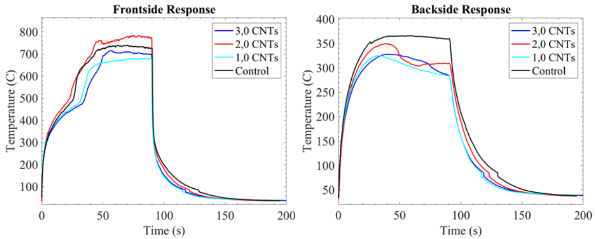
Figure 42. Thermal response of the average hottest pixel when the hybrid samples with 1-3 CNT center layers were exposed to an average irradiance of 6.48 \text{ W}/\text{cm}^2 . The control contained no CNT layers and is annotated in black.
