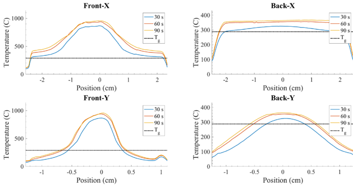
Figure 29. The spatial distribution of the heat in sample 1.1 (0 degree Orientation) when exposed to an average irradiance of 6.48 \text{ W/cm}^2 . (---) 30 secs, (---) 60 secs, (---) 90 secs. The horizontal line is the glass transition temperature of 288 \text{ }^\circ\text{C} .
