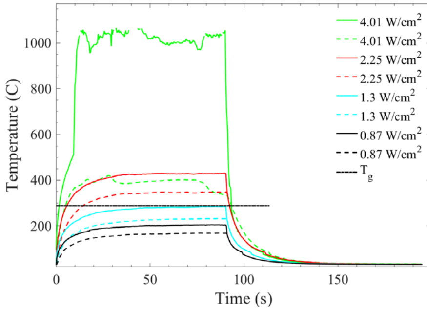
Figure A. 16 Thermal response of Sample 2.1 (20 CNT plys, 0-degree orientation) repeatedly exposed to various irradiances. Solid lines are frontside curves, dashed lines are backside curves.
