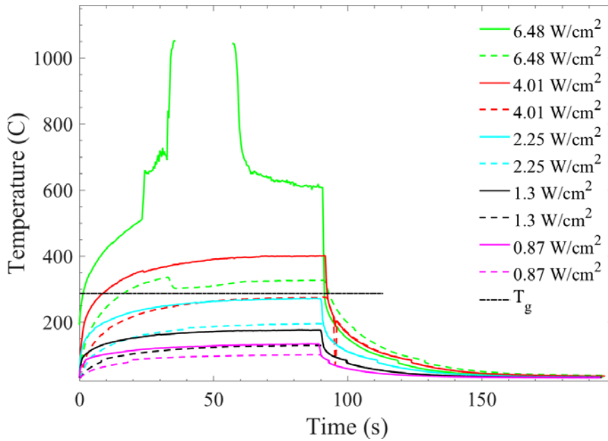
Figure A. 11 Thermal response of Sample 3.8 (2 CNT Center Layers, 2 CNT Outer Layers) repeatedly exposed to various irradiances. Solid lines are frontside curves, dashed lines are backside curves.
