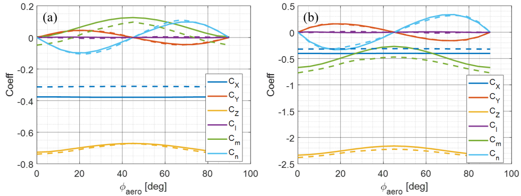
Fig. 16 Static aerodynamic coefficients of the projectile flight body at \alpha = 4^\circ (a) and \alpha = 10^\circ (b) computed by Cart3D (dashed lines) and CFD++ (solid lines) across aerodynamic roll angle, at M_\infty = 2
