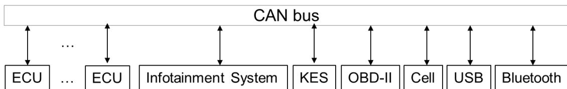
Figure 9. Vehicle Architecture
