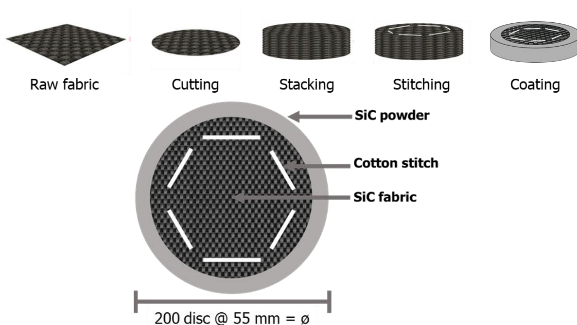
Figure 3.9. Preform fabrication route for a non-impregnated SiC f /SiC composite.
