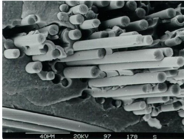
Figure 2.5. A micrograph showing the fibre pull-out mechanism in a CMC and subsequent fracture of the reinforcing fibres [62].
