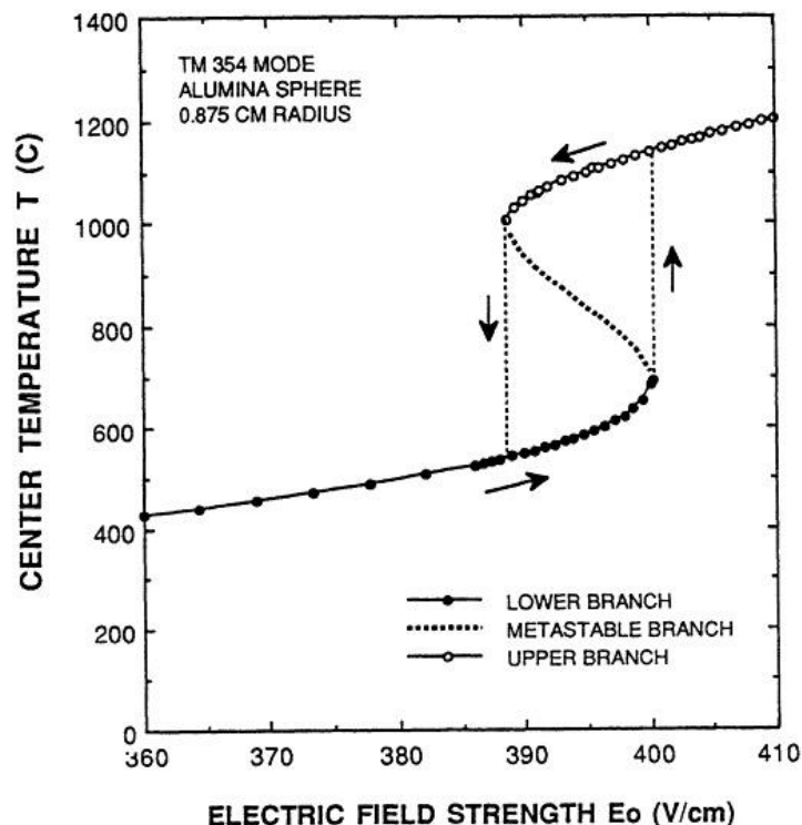
Figure 2.36. Graph showing the principle of thermal runaway showing an instantaneous temperature increase with no change in electric field strength [266].
