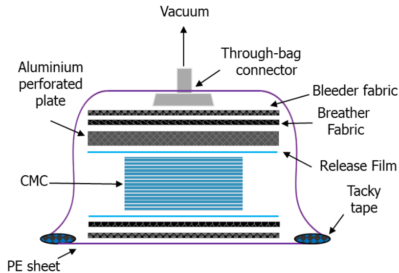
Figure 3.12. Schematic of vacuum bagging arrangement used to impregnate SiC fabric with an aqueous SiC slurry.
