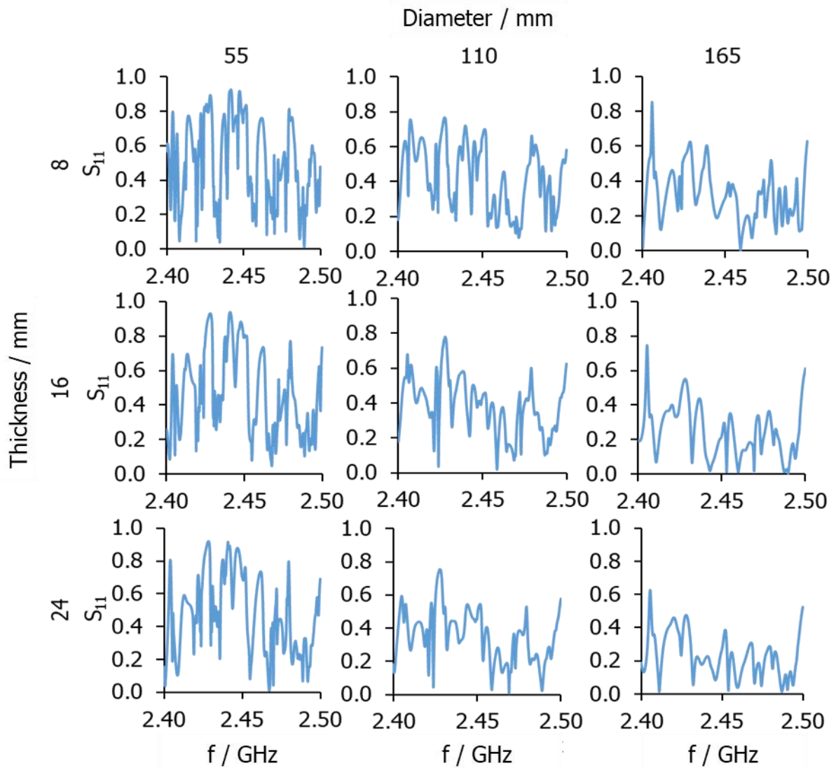
Figure 4.53. Nine graphs showing the effect of SiC fibre preform dimensions on the reflection coefficient inside the cavity and the number of induced resonances at room temperature.
