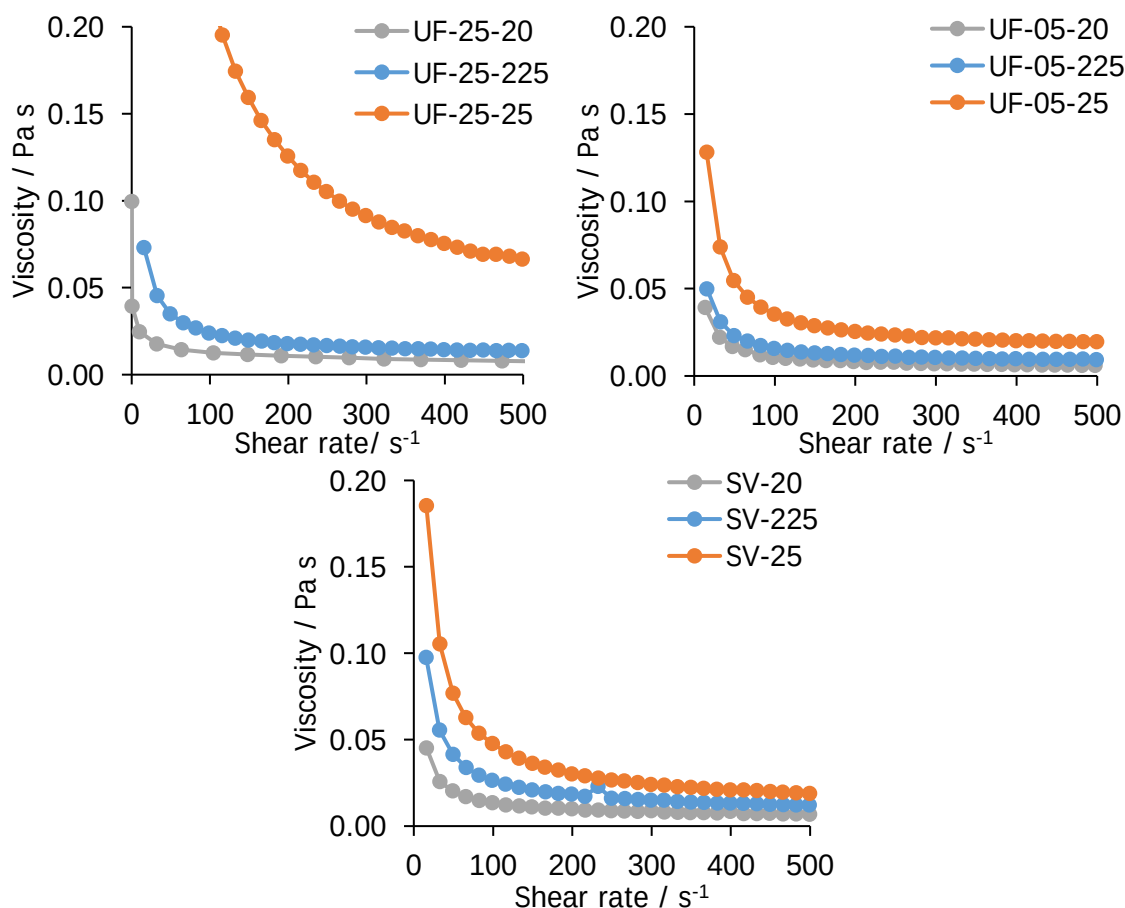
Figure 4.61. Three graphs showing the change in viscosity as a function of shear rate, with changing solids loading of the slurry and increasing particle size, from left to right UF-25, UF-05 and SuperVac.
