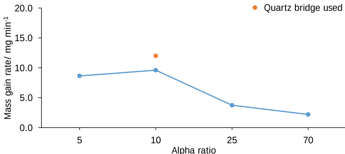
Figure 4.3. SiC matrix growth rate as a function of changing alpha ratio. All samples were processed at 925^{\circ}\text{C} , 400 mbar and Q_{\text{MTS}} = 0.2 \text{ g min}^{-1} . Q_{\text{H}_2} was changed to alter the alpha ratio.
