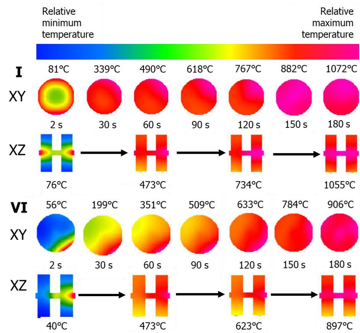
Figure 4.58. Visualisations of the temperature profile during heating at two different frequencies, I = 2.4163 GHz and VI = 2.4901 GHz over 180 s showing how the temperature profile changes with time, temperature and frequency.
