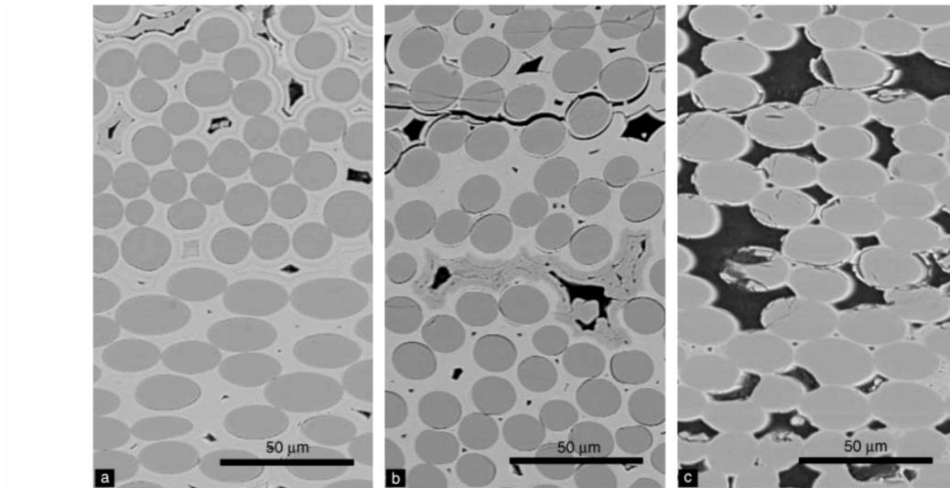
Figure 2.42. Micrographs showing the variation of deposit thickness in the CMC using MCVI; moving from the centre (far left) to 10mm from the centre (middle) and outer edge approximately 20 mm (far right) [13].
