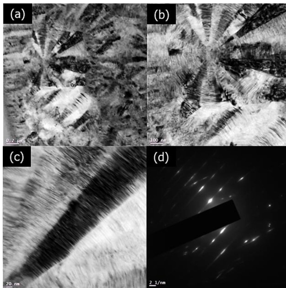
Figure 4.33. (a) A low magnification bright-field image of the 'flower' inclusion near the fibre (bottom left corner), (b) magnified image of the feature, (c) a single grain showing high contrast indicating different orientations and horizontal striations caused by stacking faults in the lattice which were confirmed in the diffraction pattern seen in (d).
