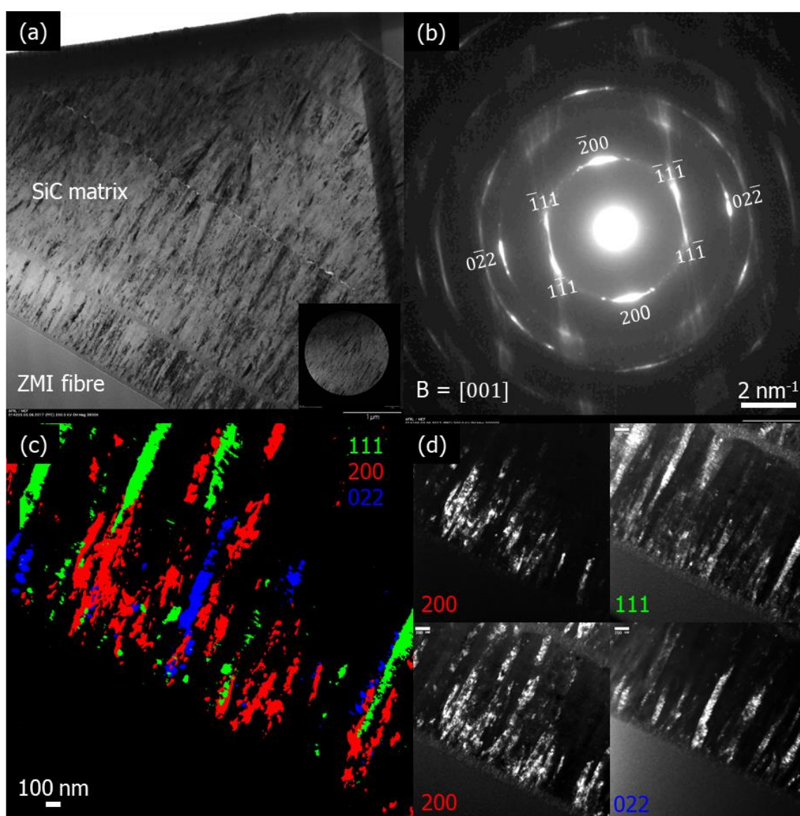
Figure 4.31. (a) A bright-field image of a SiC f /SiC foil taken at the centre of 1000°C 300 mbar sample, (b) a selected area diffraction pattern of the SiC matrix rotation of the pattern was applied, (c) four overlaid and coloured dark-field images corresponding to the images in (d).
