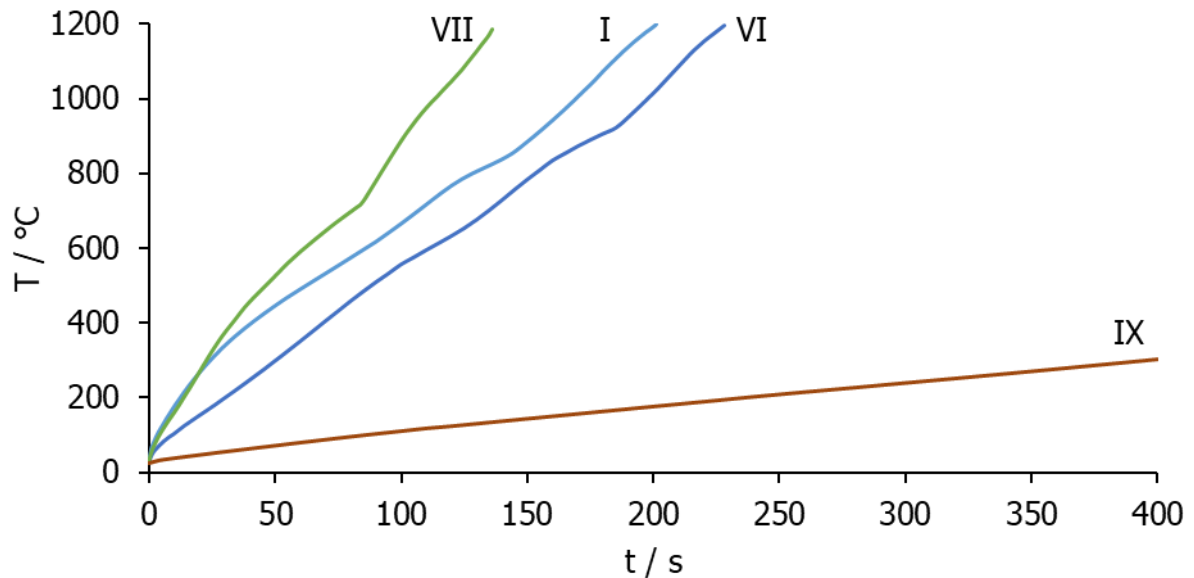
Figure 4.57. A graph showing the four frequencies selected as representative of the four scenarios showing how the temperature of the SiC f preform changed with time.
