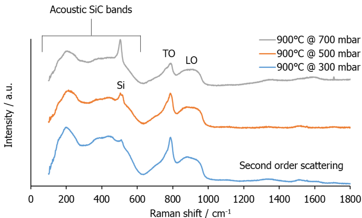
Figure 4.25. Raman spectra of the SiC deposit produced at different infiltration pressures.
