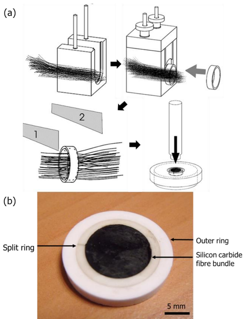
Figure 3.23.(a) LFA 427 fibre sample holder showing four key steps; (from the top left) alignment, compression, cutting and mounting in laser flash [342], (b) showing the fibre sample and the two-ringed arrangement for clamping the fibres.
