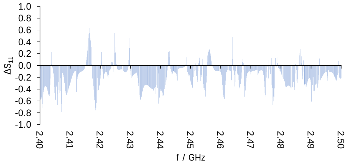
Figure 4.55. Bar graph representing the change in the value of S_{11} parameter between RT and 1200°C, showing across all frequencies a 23% decrease in the mean value of the reflection coefficient.
