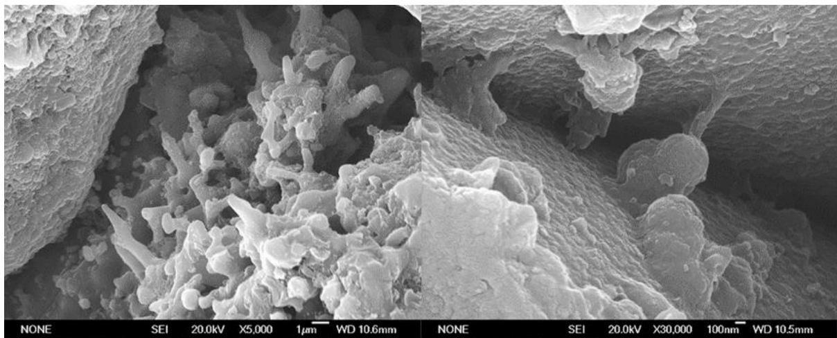
Figure 4.20. SEM micrographs showing the spine-like and large pustule regions of growth seen at 1000°C and 700 mbar.
