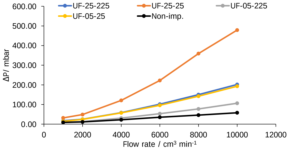
Figure 4.84. The effect of increasing flow rate on the pressure difference across the SiC f /SiC p thickness, showing the samples with higher solids content and particle size have a greater difference and vice versa.
