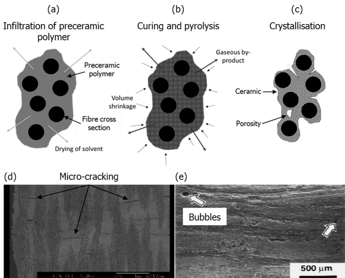
Figure 2.20. (a) A liquid preceramic precursor is impregnated into the fabric; (b) curing and pyrolysis begins, resulting in shrinkage through the evolution of gaseous by-products as the polymer is converted to ceramic; (c) a porous network is formed in the preform, with micro-cracks and pores shown in the matrix phases [150]; (d) SEM micrographs of the aforementioned micro-cracks [164] and (e) bubbles created by inadequate process control [165].
