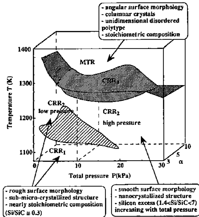
Figure 2.32. A temperature-pressure-alpha phase diagram showing the trends in the physicochemical properties of the resulting SiC deposit.
