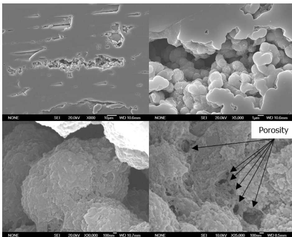
Figure 4.12. High magnification micrographs showing the deposition of SiC onto SiC powder particles and the micro-porosity that appears to have not yet been filled by the deposit.
