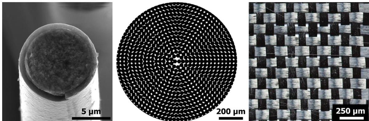
Figure 2.12. Scanning electron microscope image of a single silicon carbide filament coated in a carbon interface, (b) schematic representation of a fibre tow comprised of 800 filaments [114] and (c) a photograph of a basket/matt weave SiC fabric.
