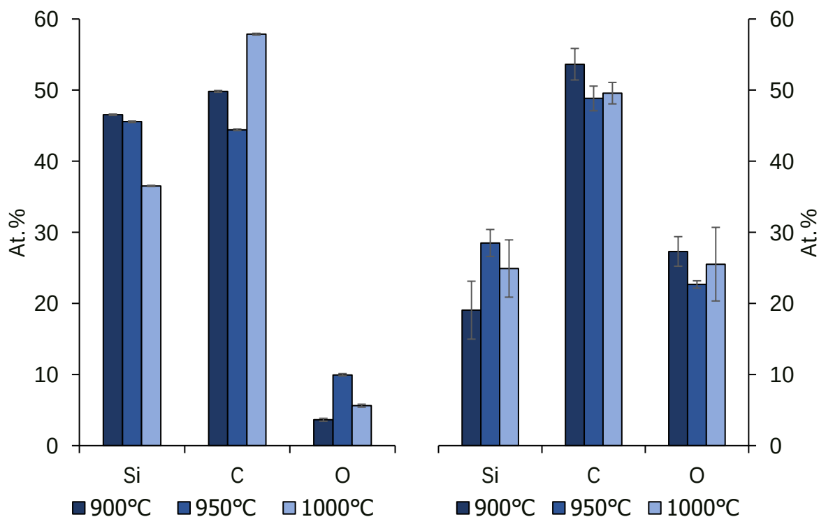
Figure 4.22. Bar graphs showing the composition of the SiC deposit at different temperatures using EDS (left) and WDS (right).
