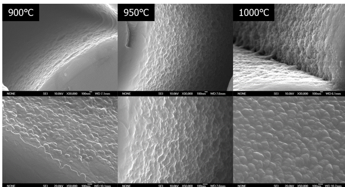
Figure 4.18. Six micrographs showing the effect of different temperatures on the surface morphology of the SiC deposit.
