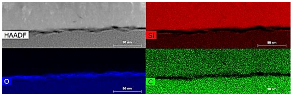
Figure 4.35. Elemental maps of the amorphous oxide band, most likely \text{SiO}_2 , found at the matrix-fibre interface, corresponding to 1(a) in figure 4.34.
