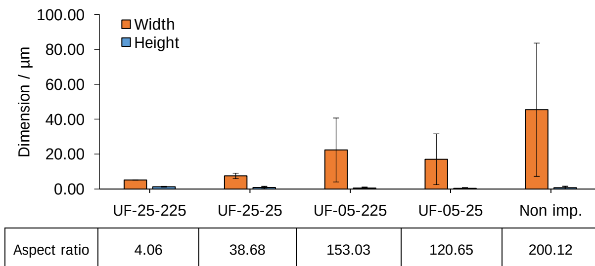
Figure 4.78. A bar graph showing the ratio of width to height in the impregnated samples with a table below corresponding to the aspect ratio.
