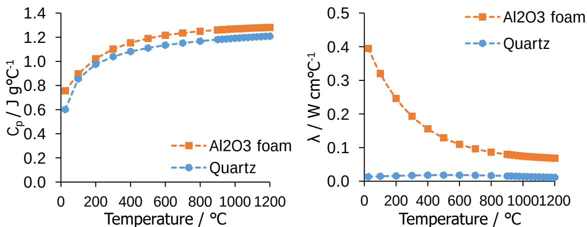
Figure 4.52. Left: Specific heat capacity of the Al 2 O 3 foam and quartz after post-processing. These were fitted with a Lorentz fit with R^2 = 0.99 and a logistic model with R^2 = 0.99 , respectively. Right: the thermal conductivity of the Al 2 O 3 foam and quartz after processing, fitted to a first-order exponential decay with R^2 = 0.97 and a Lorentz fit with R^2 = 0.99 . The graphs are plotted on the same Y-axis scale as figure 4.50 for comparative purposes.
