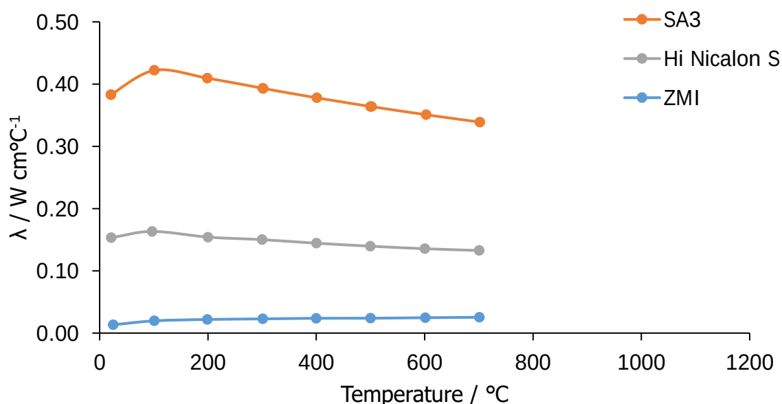
Figure 4.50. Thermal conductivity data for the three fibre types with increasing temperature calculated from measured values and accounting for thermal expansion. Note that the unit on the Y-axis is specific to the QWED 3D requirements and is not an SI notation.
