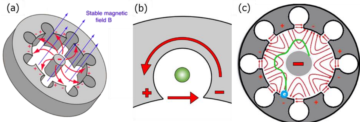
Figure 2.39. (a) A schematic adapted from [277], showing the direction of electron flow inside the anode after emissions from the cathode (red arrows) caused the intersecting magnetic field (blue arrows), (b) zoomed-in representation of a cavity, acting like a single turn inductor, showing the direction of current flow and the resultant electromagnetic wave produced extending out of the page parallel to the magnetic field and (c) the interaction of the electron with the electric field induced by the cavity-causing the retardation of the electron.
