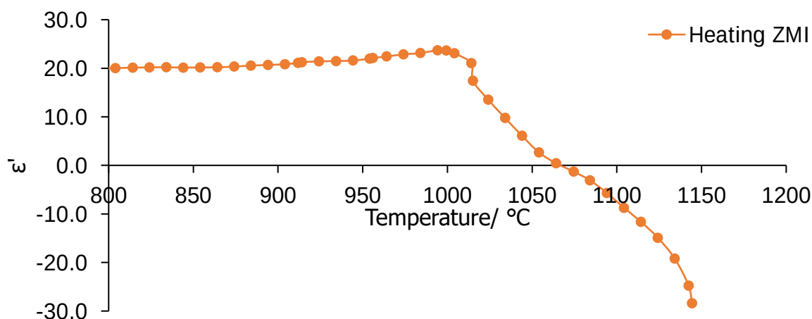
Figure 4.2. The dielectric permittivity of the Tyranno ZMI fibre as a function of temperature, showing the fibre stops behaving as a dielectric at ~1060°C.
