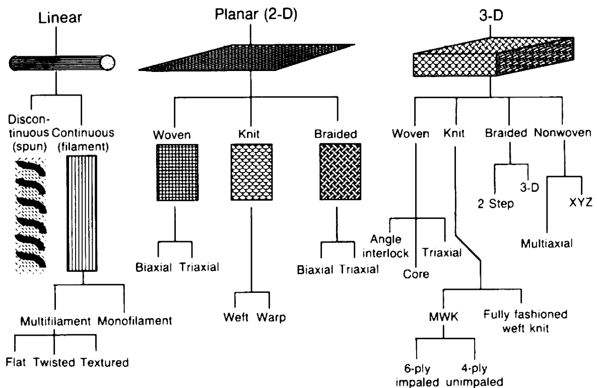
Figure 2.13. Classification of fibre architectures [115].
