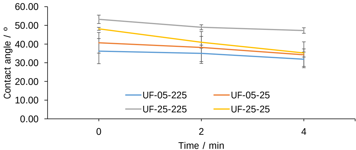
Figure 4.70. Change in contact angle of SiC slurry droplet as a function of time.
