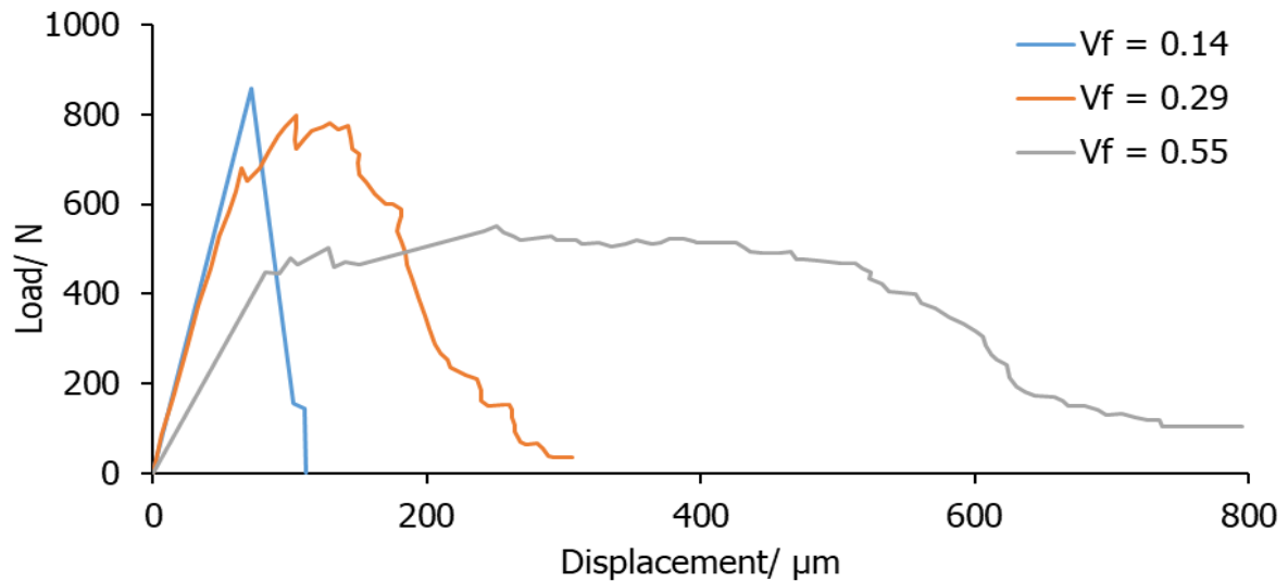
Figure 2.16. Three load-displacement curves as a function of volume fraction ( V_f ), reproduced from [122].
