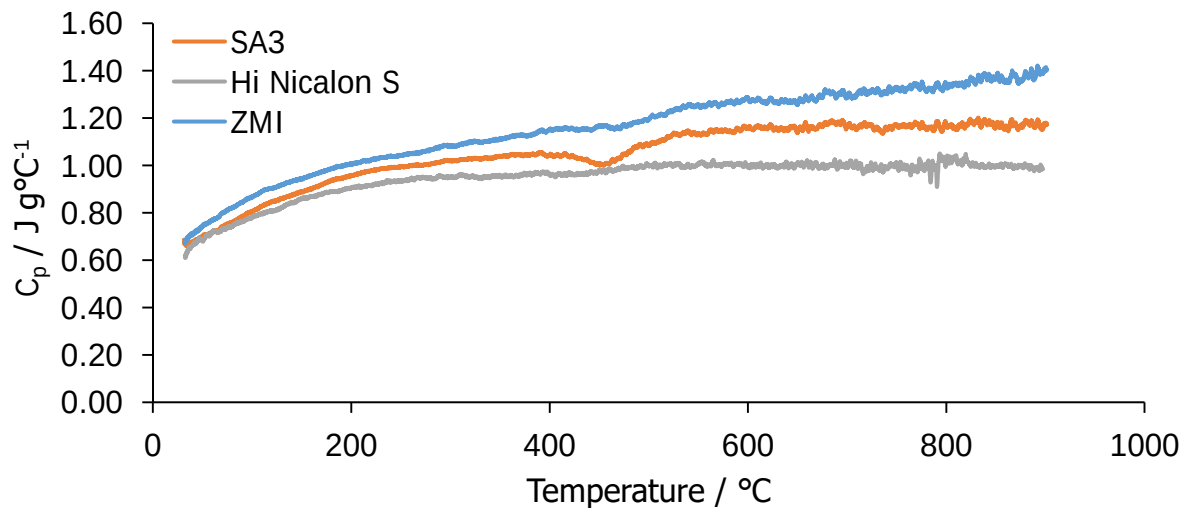
Figure 4.49. Measured specific heat capacity data for the three fibres up to 900^{\circ}\text{C} , in the units required for the QWED 3D simulation.
