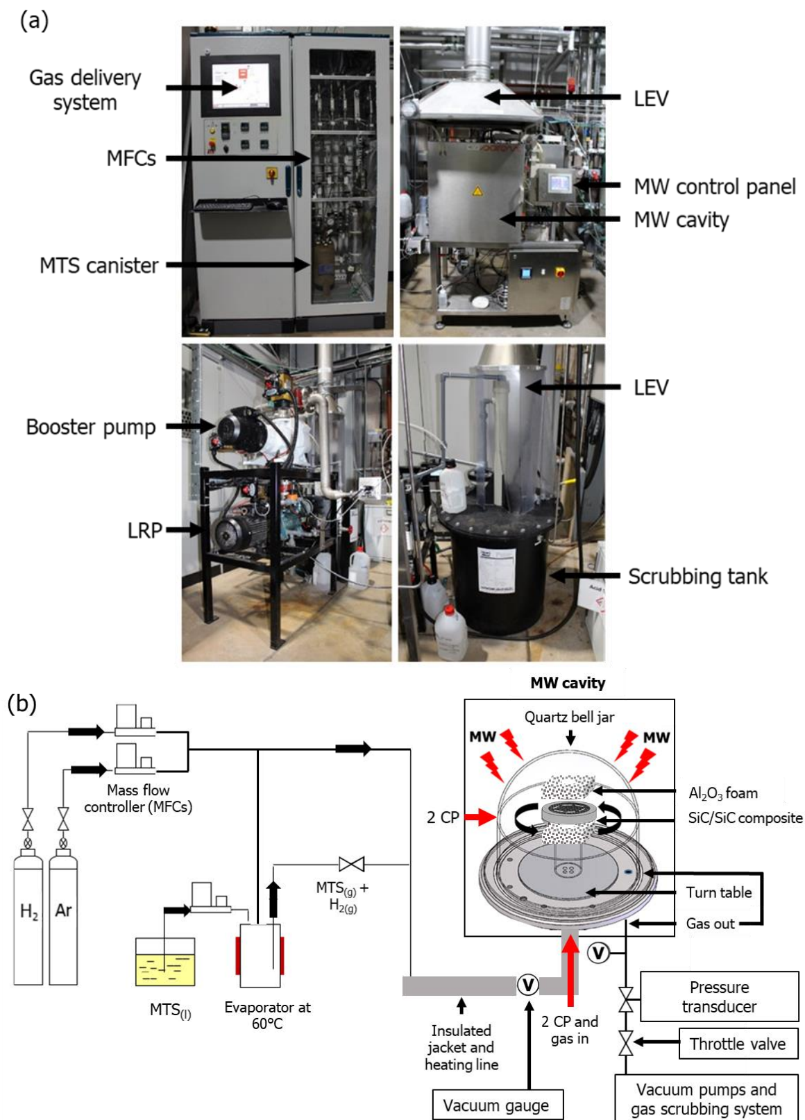
Figure 3.1. (a) Labelled photos of the MCVI system and (b) a schematic representation of the system.
