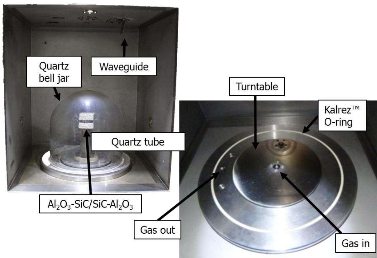
Figure 3.7. Photo of the microwave cavity with the bell jar inside and an image of the turntable and gas inlet and outlet.
