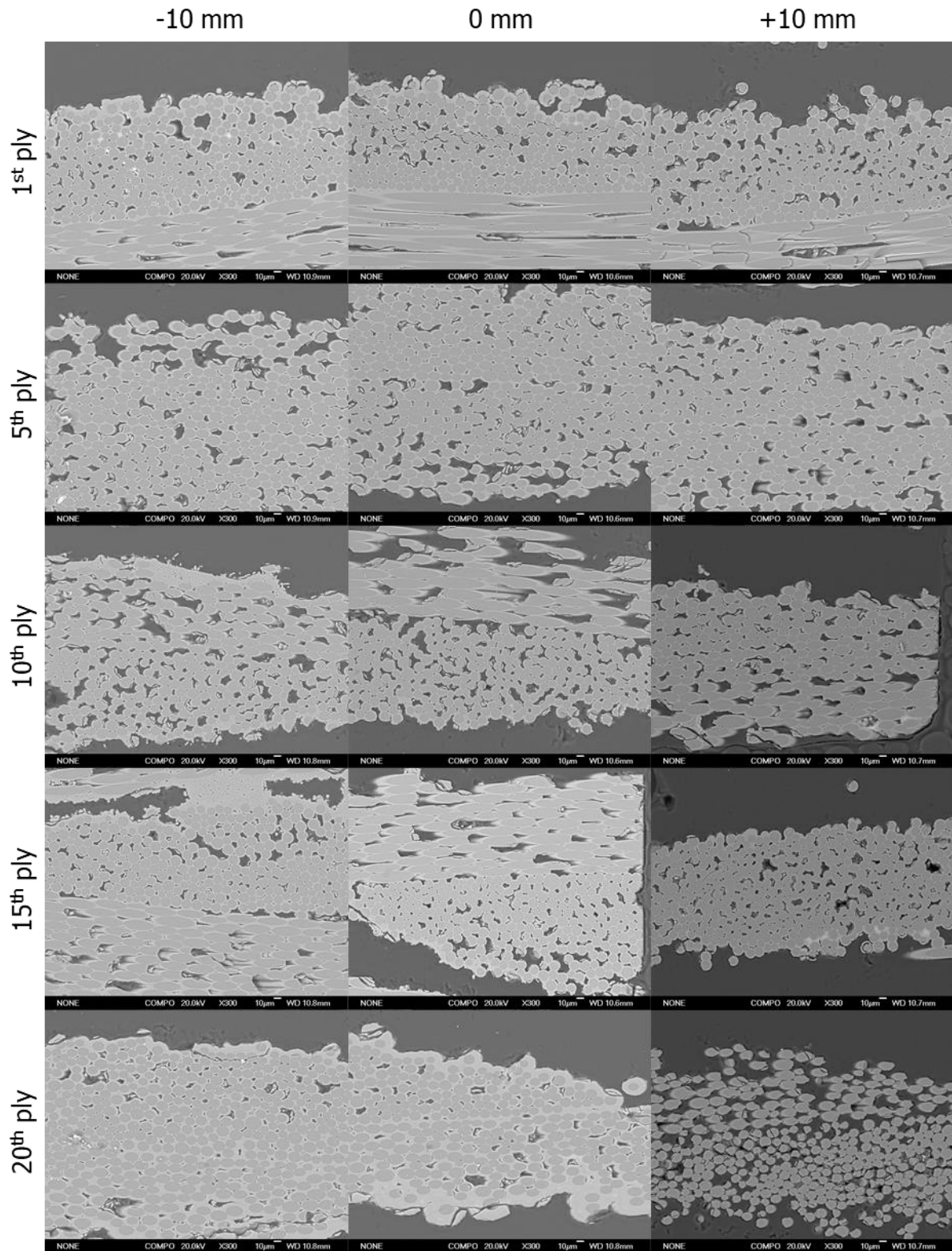
Figure 4.9. Micrographs of the uniform deposition coating seen over the thickness and 20 mm of the sample infiltrated at 1000°C at 300 mbar.
