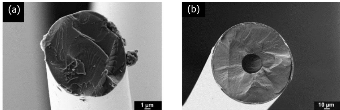
Figure 2.9. (a) Cross sectional images showing the mesostructure of a fibre produced using the preceramic polymer technique and (b) using CVD, note the different scales [89].
