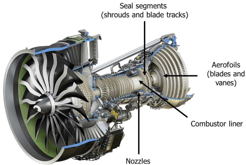
Figure 2.17. Cross-section of the next generation large three-shaft civilian turbofan engine the GE9x from General Electric [124].
