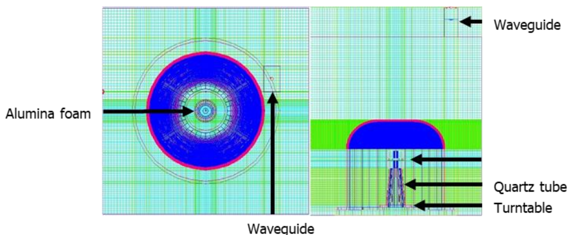
Figure 3.27. A top-down view and front-on view of the non-uniform meshes applied to the simulation.
