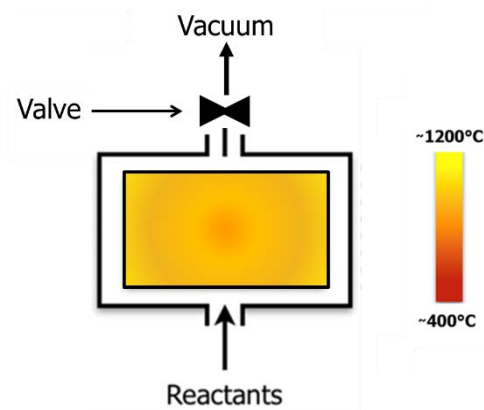
Figure 2.26 Schematic showing the key components of the pulsed pressure system and the respective temperature profile [150].
