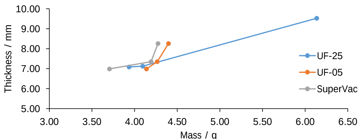
Figure 4.64. The increase in thickness as a function of the mean mass gain of the preforms when impregnated with different powders and solids content. From left to right in terms of data points (20, 22.5, 25 vol.%).
