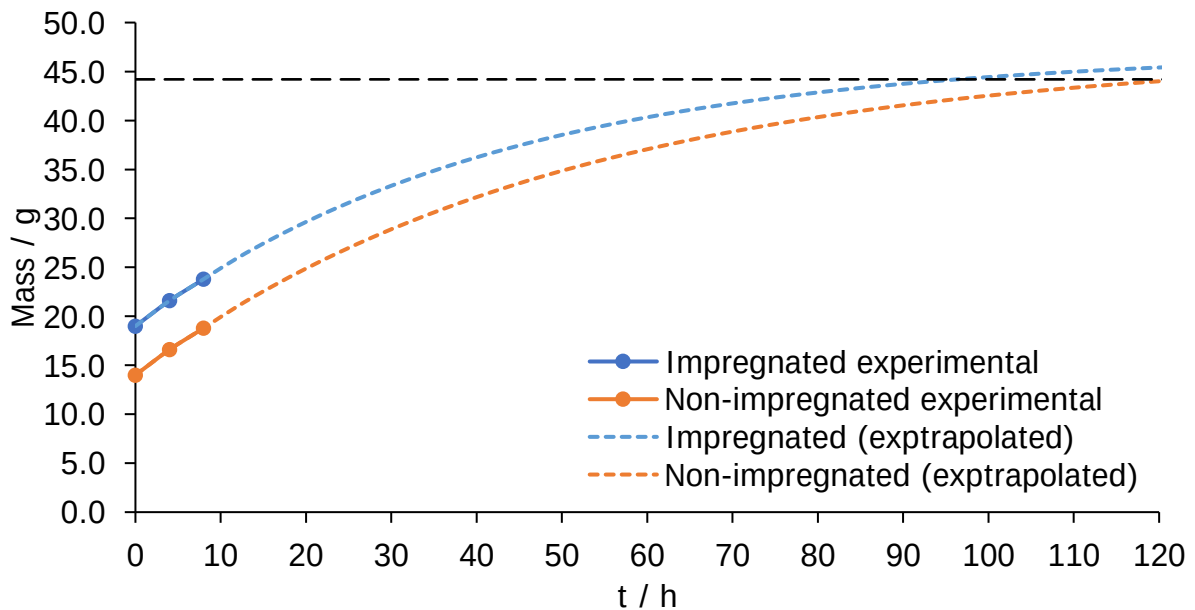
Figure 4.5. Extrapolated plots of the densification of the SiC f /SiC composite using natural logarithmic decay function based on the rate of mass gain seen in sample QB over the first 8 h (2+2+4 h), table 3.3. It shows a potential reduction in the time afforded by the introduction of the SiC slurry phase.
