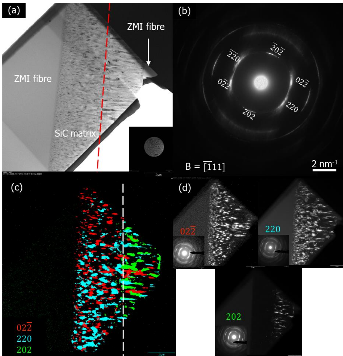
Figure 4.30. (a) A bright-field image of a SiCf/SiC foil taken at the centre of 950°C 300 mbar sample, the dashed line shows the fibre merging interface, (b) a selected area electron diffraction pattern of the SiC matrix, rotation of the pattern was applied, (c) three overlaid and coloured dark-field images corresponding to the images in (d).
