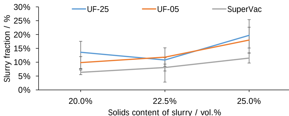
Figure 4.63. The volume fraction as a percentage of slurry added to the SiC f /SiC p preforms impregnated with different solids content slurries and different particle sizes.
