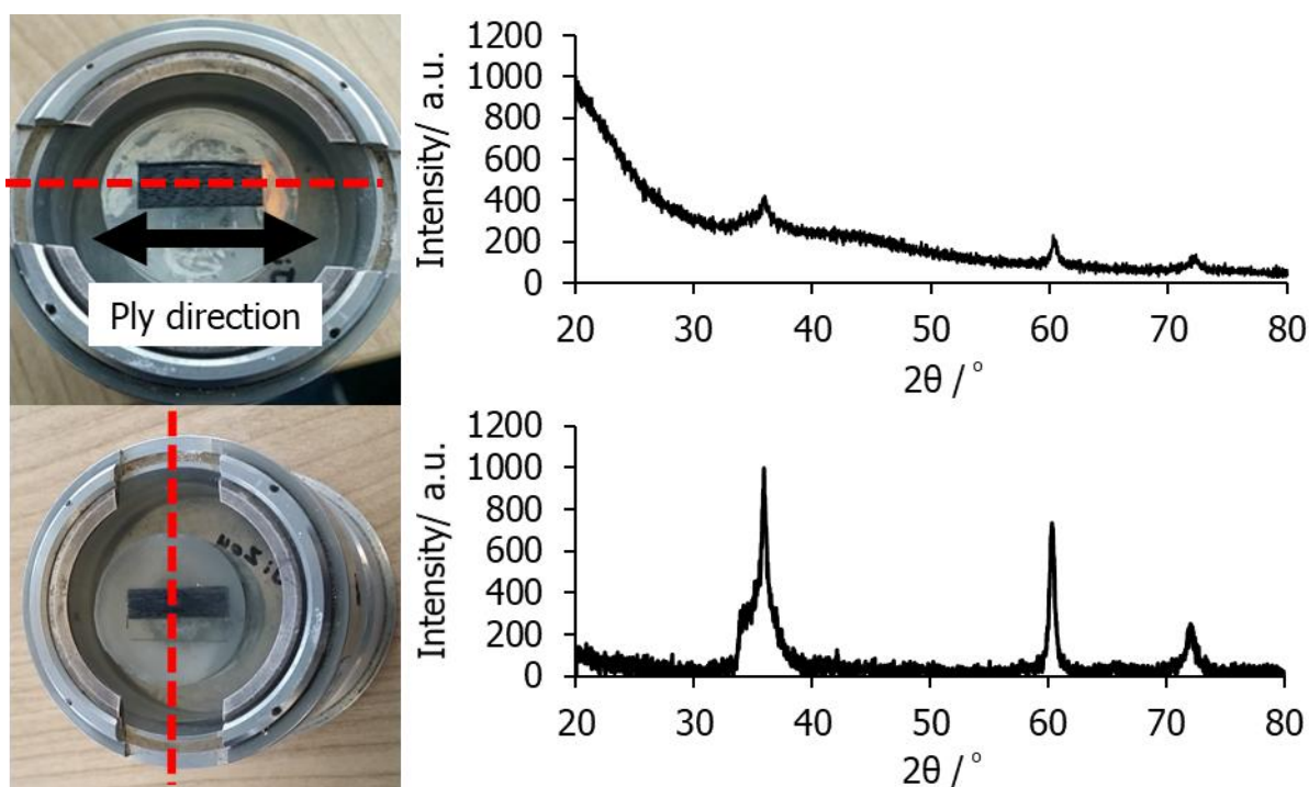
Figure 3.20. Corresponding XRD diffractograms demonstrating the scanning orientation effect on the signal intensity. Red dashed line corresponds to the orientation.
