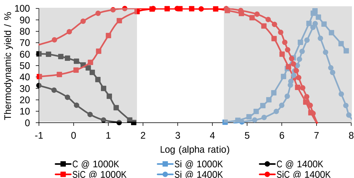
Figure 2.31. Thermodynamic yields for the solid deposition of silicon carbide and its co-deposits as a function of alpha ratio, adapted from [9].
