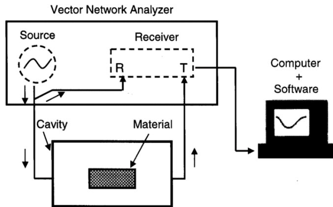
Figure 2.37. A generic schematic of the resonant cavity set up used for measuring dielectric properties [270].
