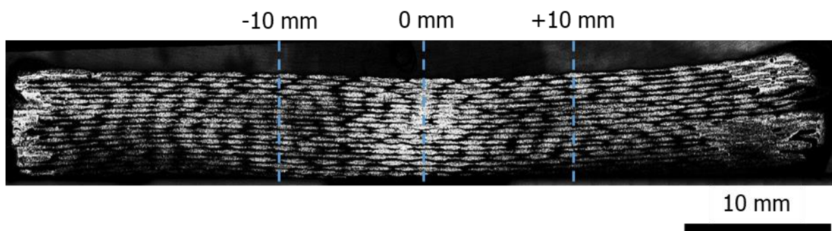
Figure 4.16. A series of stitched micrographs of the densification profile of a SiC f preform. The conditions by which it was infiltrated are as follows: T = 925^{\circ}\text{C} , P = 400 \text{ mbar} , \alpha = 10 and Q_{\text{MTS}} = 0.2 \text{ g min}^{-1} Q_{\text{H}_2} = 300 \text{ cm}^{-3} \text{ min}^{-1} .
