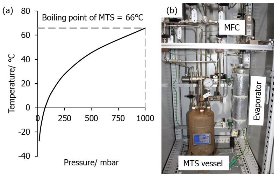
Figure 3.6. (a) Effect of pressure on the boiling point of MTS [322] and (b) a photo the MTS storage vessel connected to the evaporator that heated up the liquid to a vapour.
