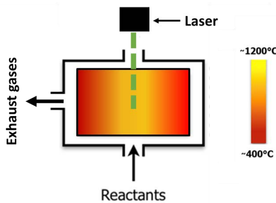
Figure 2.27. Schematic showing the key components of the laser-assisted process and the respective temperature profile [150].
