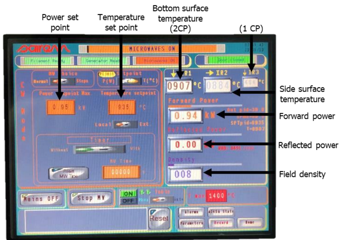
Figure 3.15. Labotron control panel for operating the microwave generator unit.
