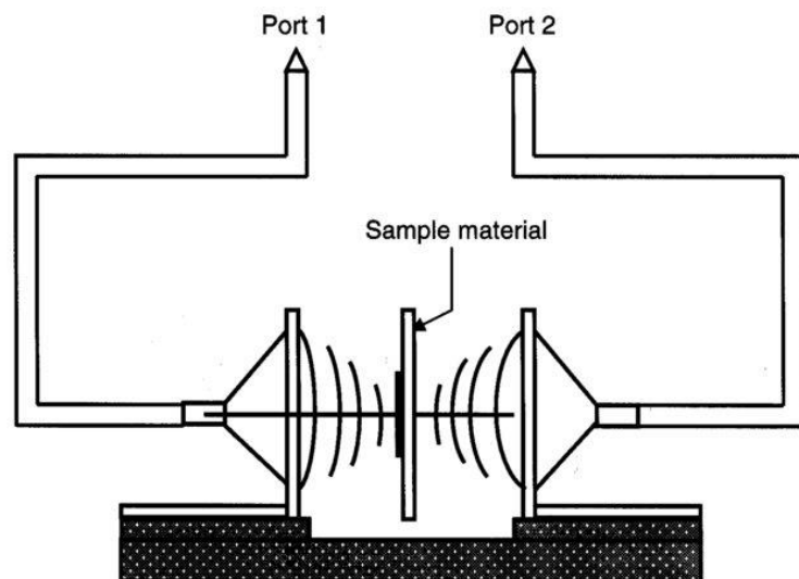
Figure 2.38. A diagram of the free space method that can be used to measure dielectric properties [270].
