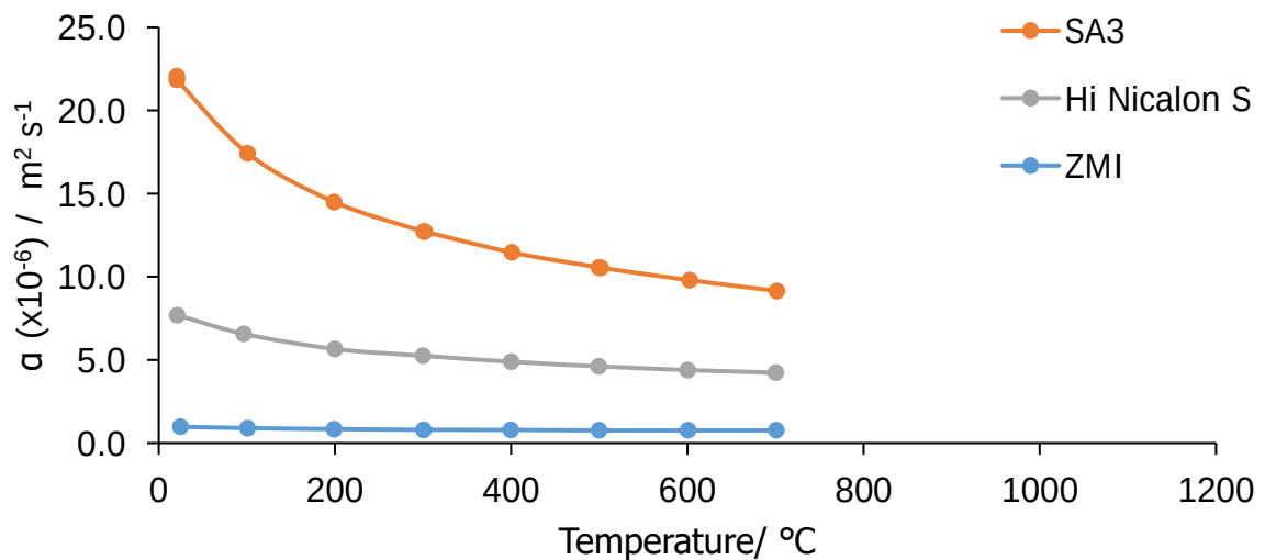
Figure 4.48. Measured thermal diffusivity values for the three SiC fibres. Note that the units used are SI as QWED did not require thermal diffusivity data input for the simulation.
