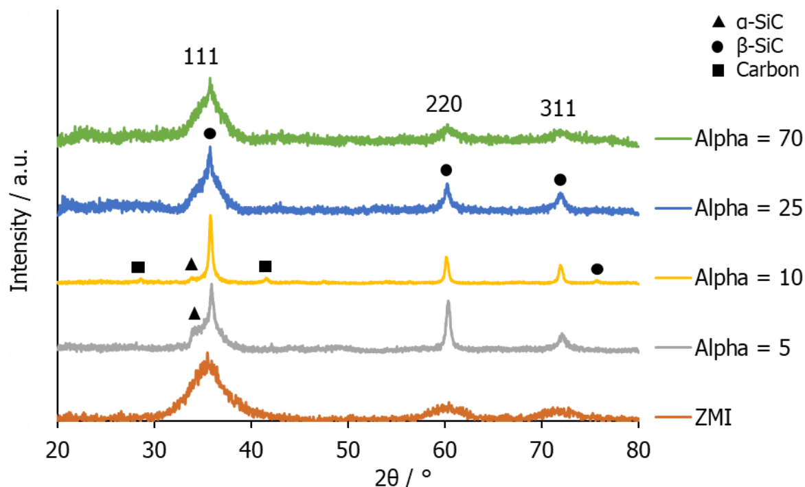
Figure 4.37. XRD diffraction patterns for the samples infiltrated using different alpha ratios.
