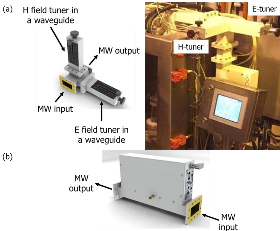
Figure 3.2. (a) Manual tuning system and (b) automatic tuners that were used to minimise the reflective power inside the MW cavity to improve the efficiency of heating.
