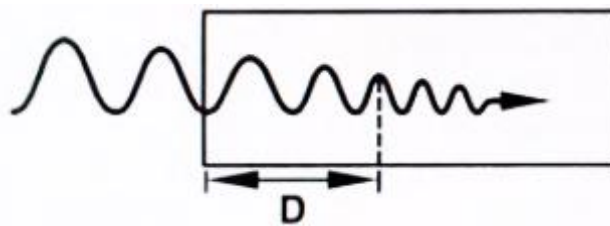
Figure 2.34. The absorption of microwaves to half-power depth (skin depth).
