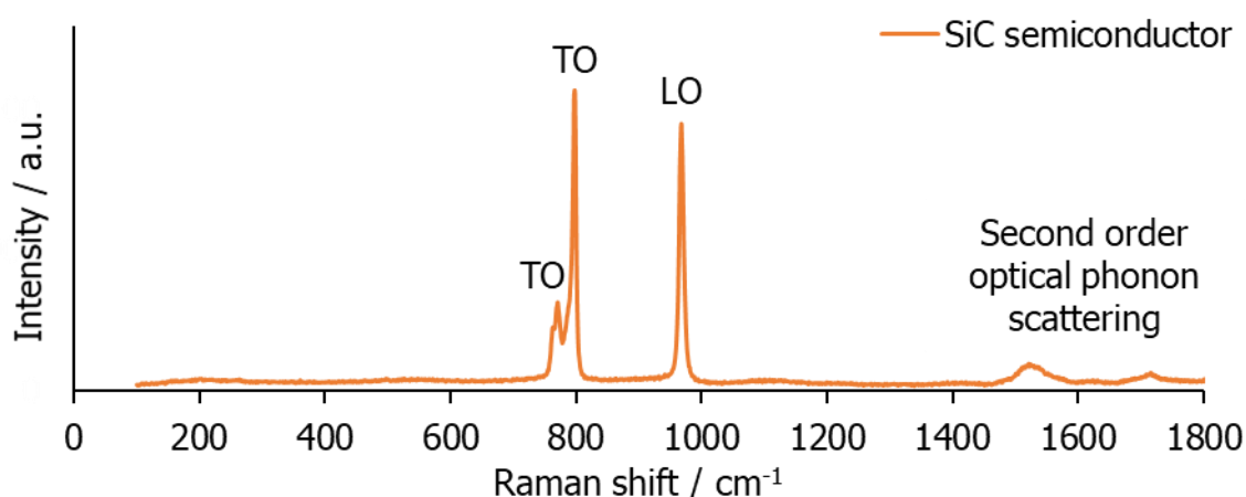
Figure 4.23. Raman spectra for the semiconductor standard showing the presence of both longitudinal and transverse optical phonons.
