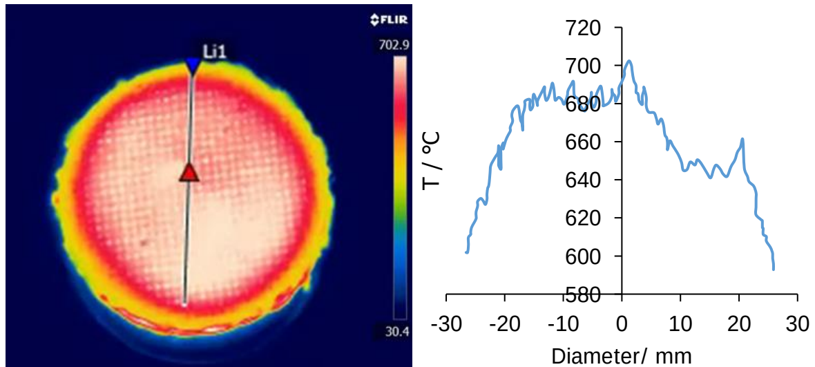
Figure 4.43. The formation of inverse temperature profiles at \sim 700^{\circ}\text{C} in a 55 mm 20 ply SiC fibre preform using microwave energy and the concordant graph showing temperature profile along the intersecting line.
