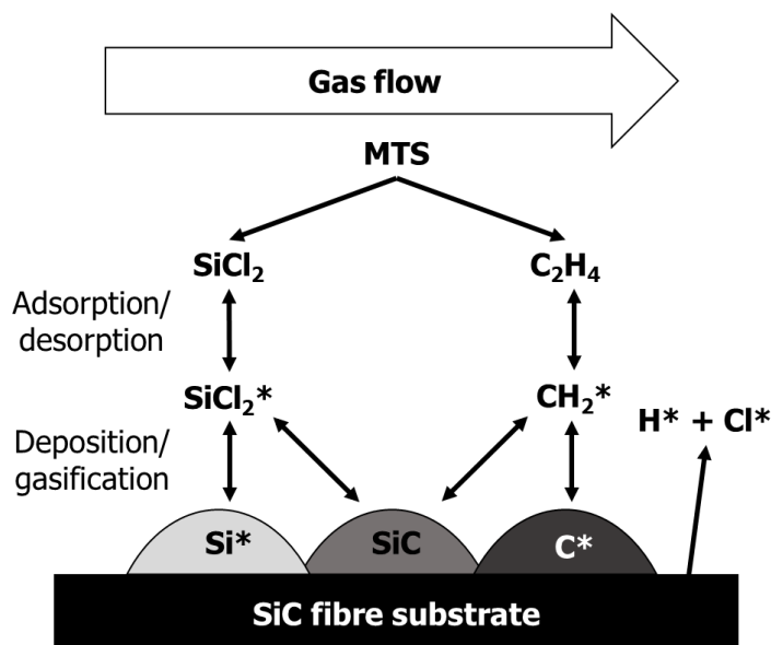
Figure 2.29. Schematic representation of the adsorption and deposition of SiC constituents to the fibre surface, adapted from [225].
