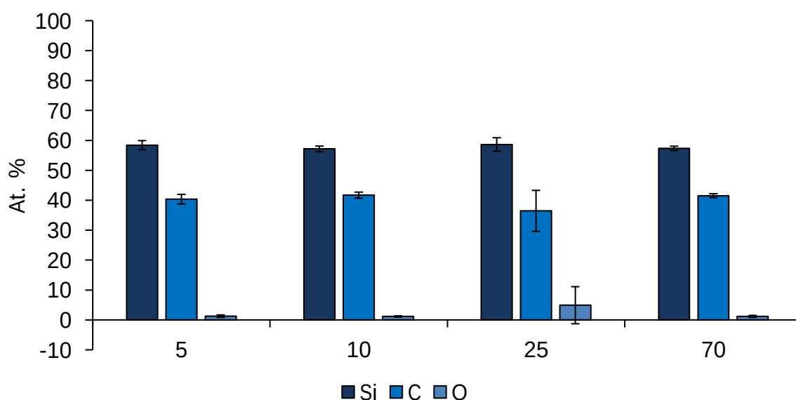
Figure 4.28. The Si:C:O ratio in the SiC f /SiC samples infiltrated with different alpha ratios with T = 925 \pm 15^{\circ}\text{C} and P = 400 \pm 8 mbar.
