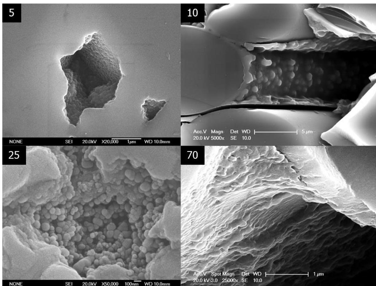
Figure 4.21. SE micrographs showing the variation of the SiC deposit morphology with changing alpha ratios.
