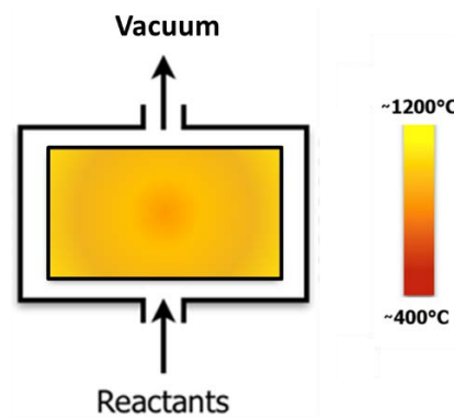
Figure 2.25. Schematic showing the key components of the isothermal forced flow process and the respective temperature profile [150].
