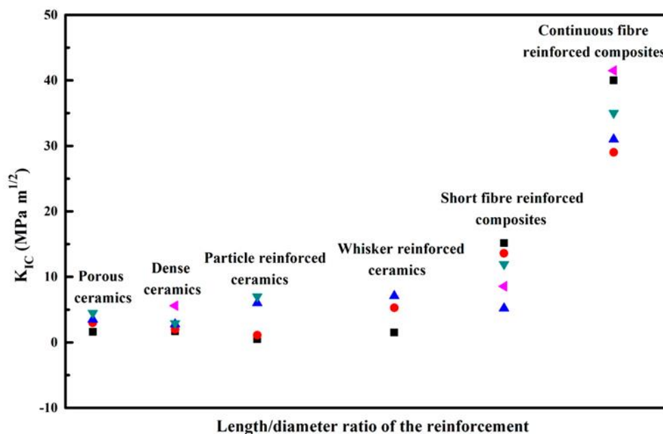
Figure 1.1. A graph indicating the dependence of fracture toughness of ceramic materials on the increasing length/diameter ratio of potential reinforcing phases, adapted from [4], showing continuous fibre reinforced CMCs to have the most superior fracture toughness.
