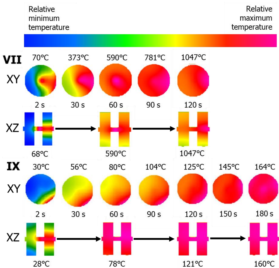
Figure 4.58. (Continued) Visualisation of curves VII and IX, 2.4189 GHz and 2.4632 GHz, respectively.
