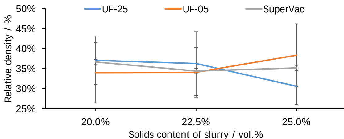
Figure 4.62. The relative density of \text{SiC}_f/\text{SiC}_p preforms impregnated with different solids content slurries and different particle sizes.
