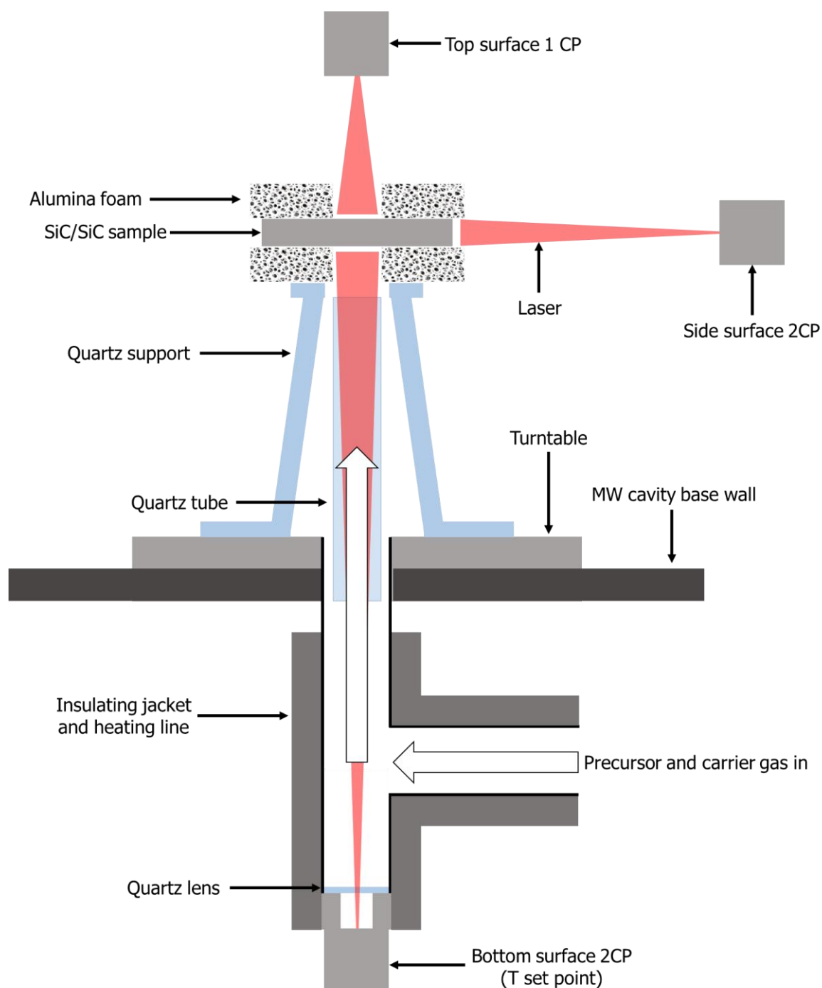
Figure 3.4. A cross-sectional view of the temperature control arrangement of two-colour pyrometers, sample and gas flows.
