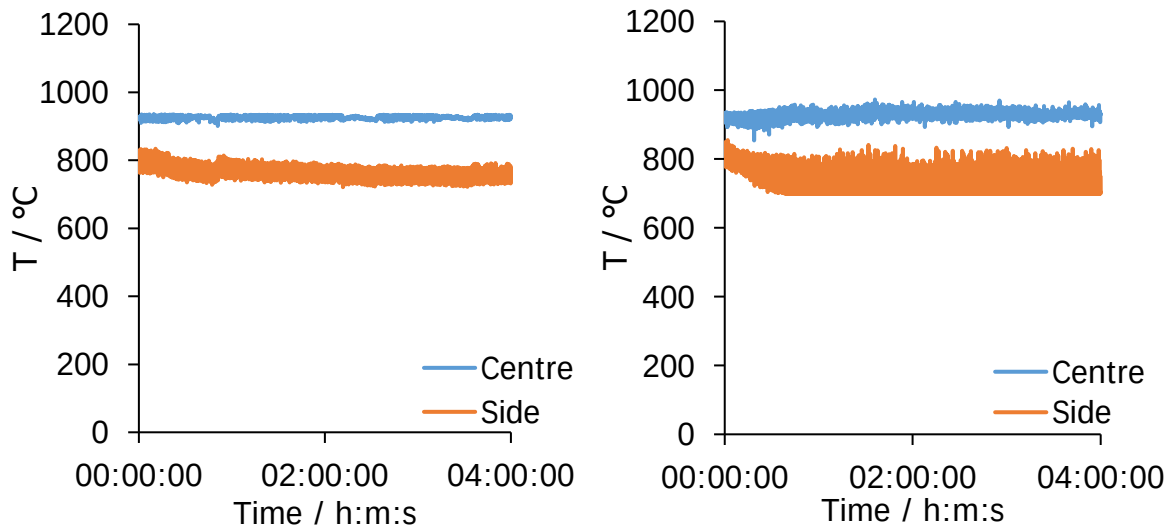
Figure 4.4. Left: Infiltration temperature over time at an alpha ratio of 10 showing a relatively constant centre and side temperature. Right: equivalent graph for alpha 70 showing significant fluctuation for both the side and centre temperatures.
