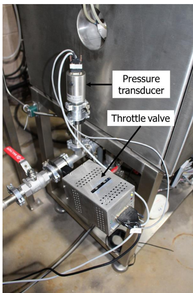
Figure 3.5. Photo of the pressure transducer that monitored the vessel pressure and the throttle valve that enacted changes to the pressure.
