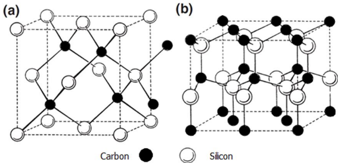
Figure 2.8. (a) Zinc blend cubic structure of \beta -SiC and (b) the Wurtzite hexagonal structure of \alpha -SiC. Adapted from [88].
