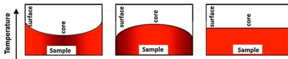
Figure 2.35. Schematic illustrations of the temperature profiles within samples heated (left to right) conventional, microwave (inverse temperature profile) and hybrid heating [256].
