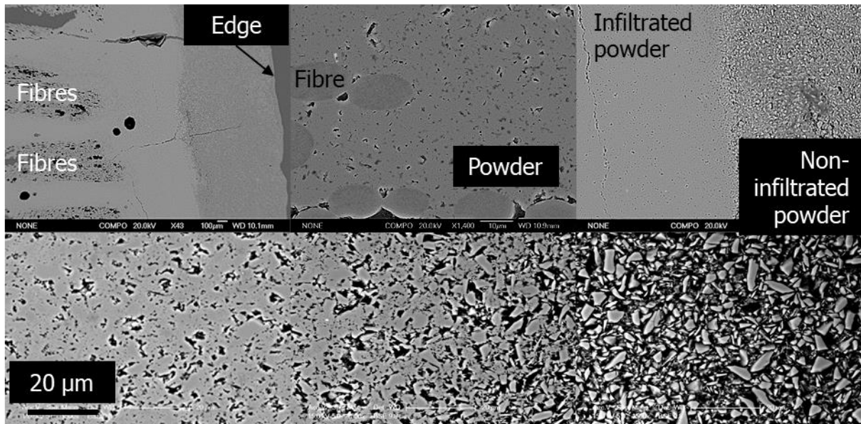
Figure 4.11. The top three images show the densification of the sides of the preform coated in SiC slurry. The bottom three show the transition from infiltrated powder to non-infiltrated powder, from left to right over a 250 \mu\text{m} distance.
