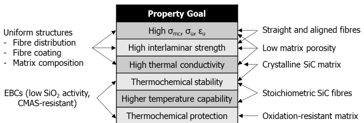
Figure 2.6. Microstructural goals for achieving property goals of SiC f /SiC composites. \sigma_{mc} = matrix crack stress, \sigma_u is the ultimate tensile strength and \epsilon_u is tensile failure strain, adapted from [70].
