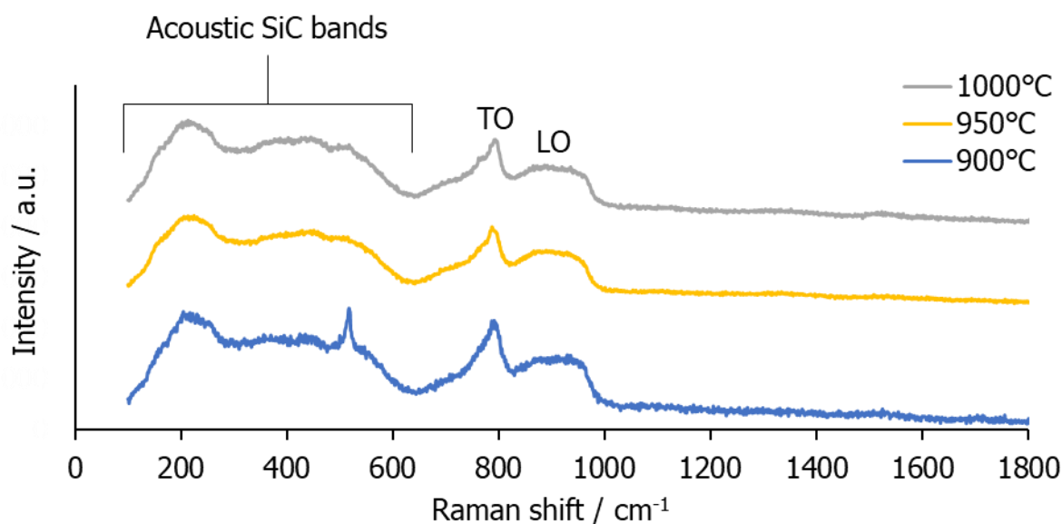
Figure 4.24. Raman spectra of the SiC deposit produced at different infiltration temperatures with a constant pressure of 300 mbar.
