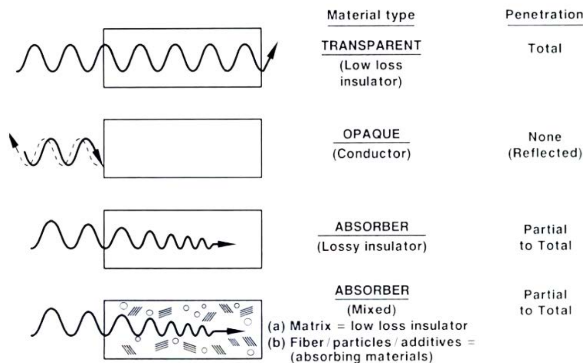
Figure 2.33. Series of diagrams showing the microwave-matter interactions possibilities [258].
