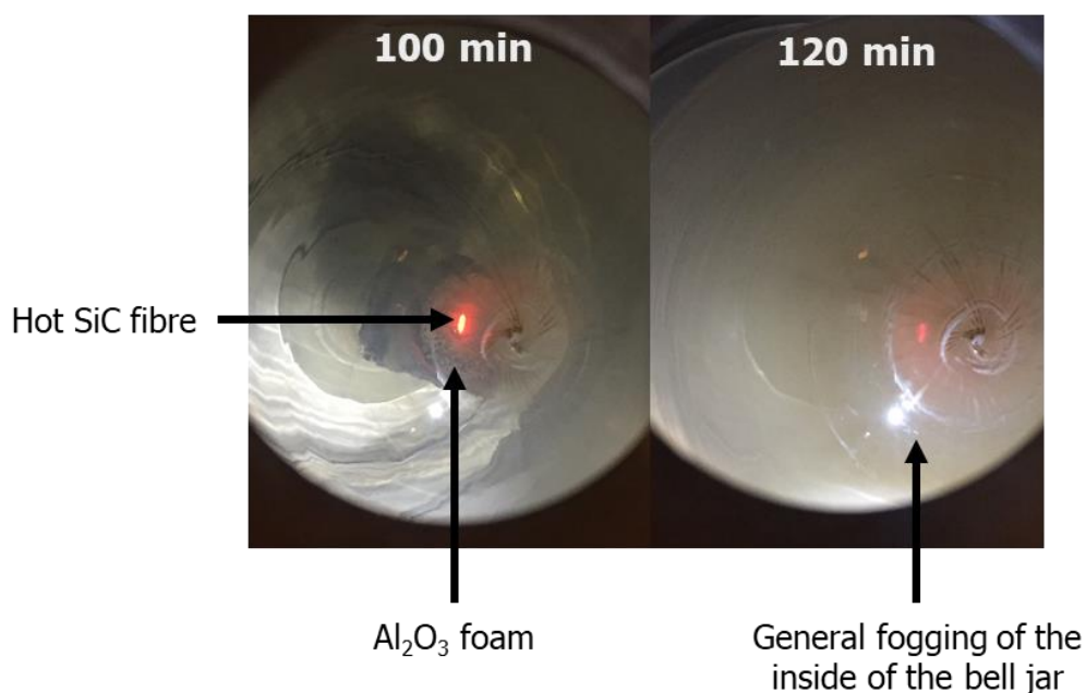
Figure 3.16. Photographs showing the development of the \text{SiO}_x\text{Cl}_x layer on the top of the inside surface of the top of the bell jar after 2h.
