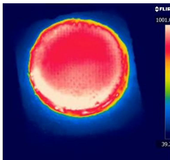
Figure 4.44. TIC image showing the SiC preform at 1001^{\circ}\text{C} after 2 minutes of heating.
