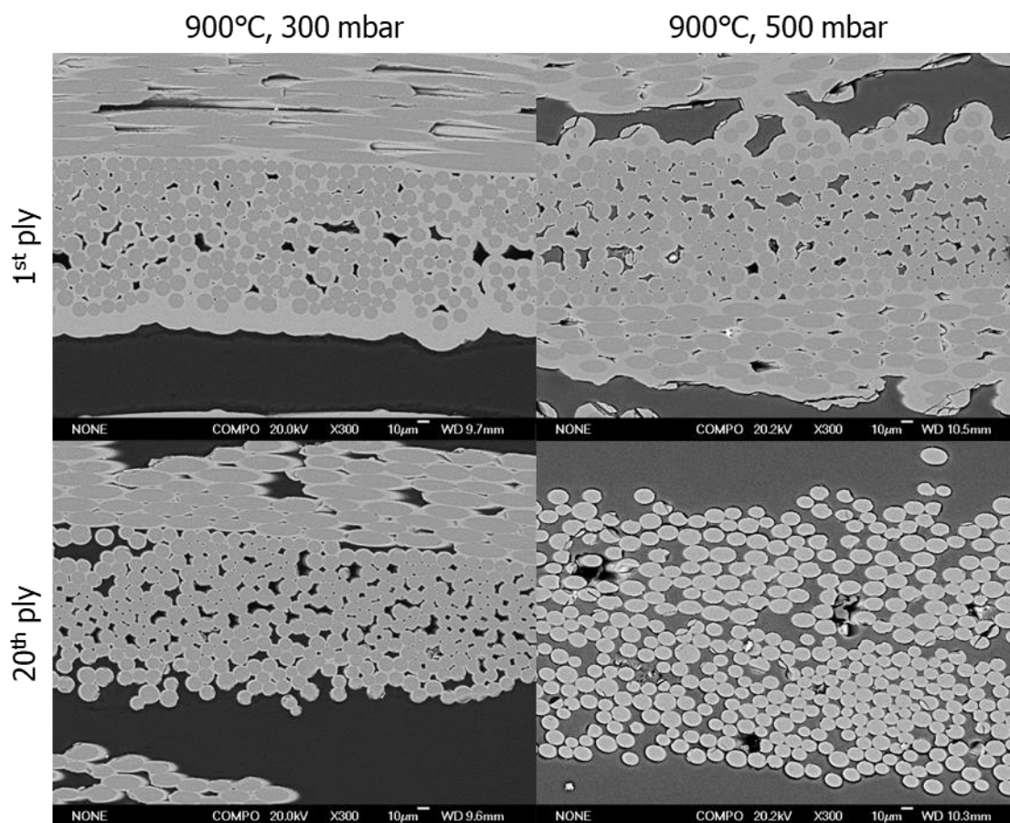
Figure 4.8. The difference in fibre coating thickness between the 1 st ply (top row) and the 20 th ply (bottom row) in samples infiltrated at 900°C at different pressures.
