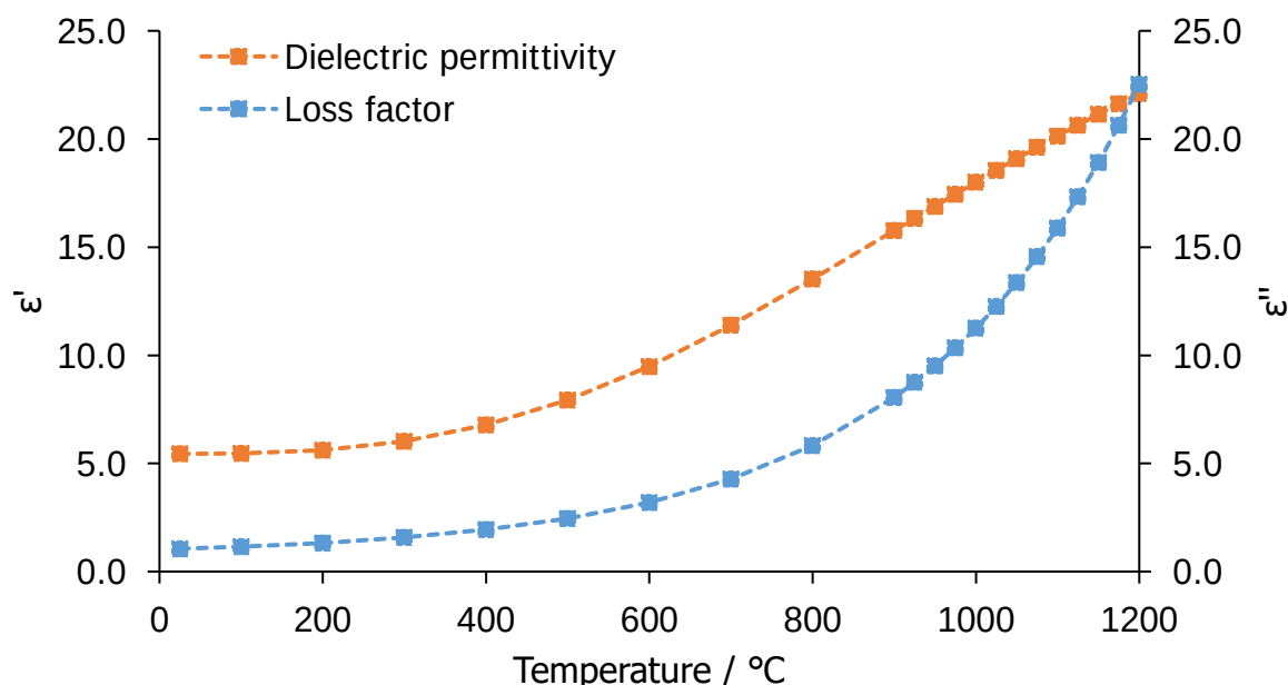
Figure 4.46. The dielectric permittivity (primary axis) and the loss factor (secondary axis) of the Hi Nicalon S fibres after interpolation using Origin. \epsilon' was fitted with a logistic model with R^2 = 0.99 , the \epsilon'' was fitted using a Boltzmann model with R^2 = 0.97 .
