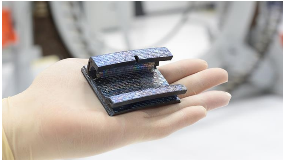
Figure 2.18. A SiC f /SiC shroud component produced by Rolls Royce PLC [6].
