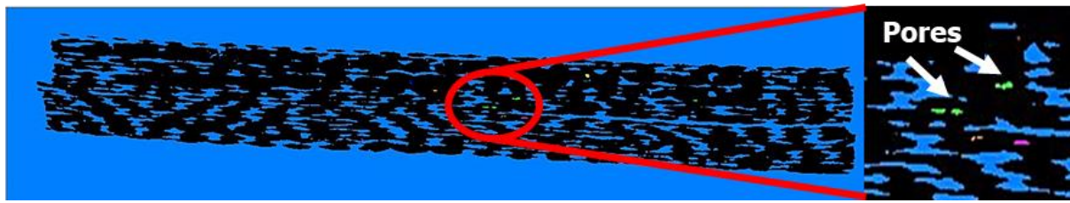
Figure 4.74. Images from Avizo showing the identification of small closed porosity in the green SiC f /SiC composite.
