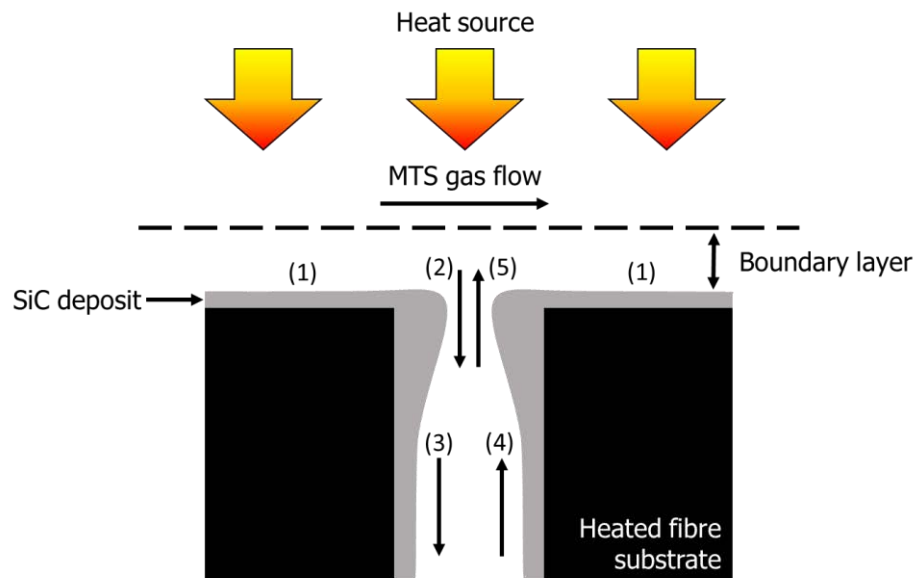
Figure 2.30. Schematic showing the different steps in the iso-thermal CVD process, adapted from [9, 14].
