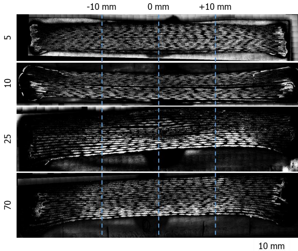
Figure 4.13. Stitched micrographs of the densification profiles of \text{SiC}_f preforms infiltrated at alpha ratios 5-70, where T = 925^\circ\text{C} , P = 400 \text{ mbar} , Q_{\text{MTS}} = 0.2 \text{ g min}^{-1} were constant and the Q_{\text{H}_2} was changed between samples.
