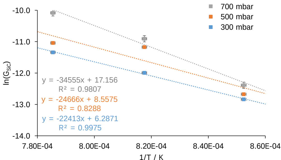
Figure 4.6. Natural logarithm of the SiC matrix growth rate against the reciprocal temperature for three different pressures at the same flow conditions.
