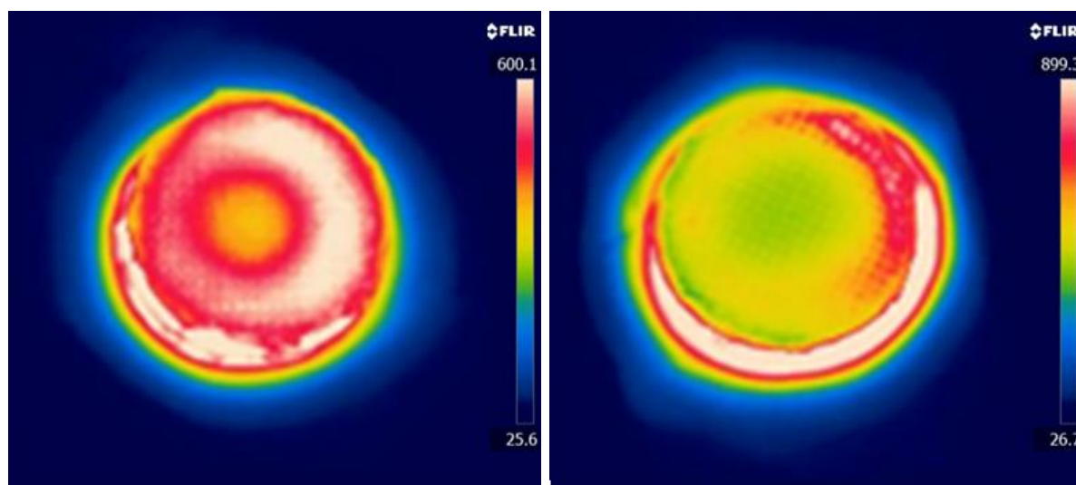
Figure 4.42. Left: An annular temperature profile of 10 ply 55 mm diameter SiC preform heated using microwave energy. Right: Non-uniform heating of 55 mm diameter sample made with 30 ply showing hot edges.
