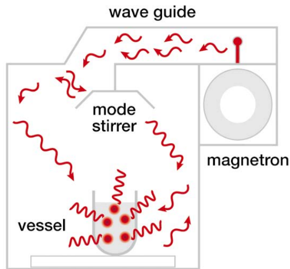
Figure 2.41. Diagram of a multimode cavity with mode stirrer [289].
