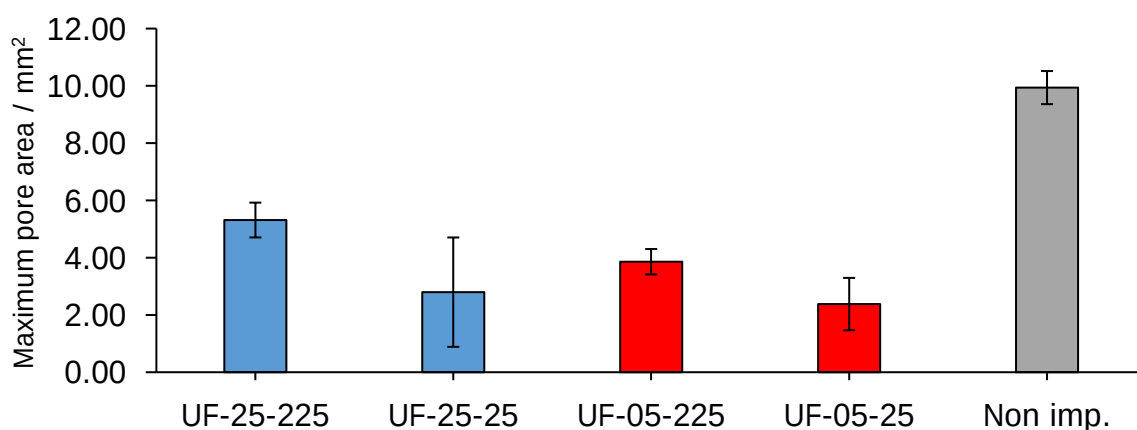
Figure 4.77. The mean maximum pore area measured using the MATLAB script based on micro-CT data.
