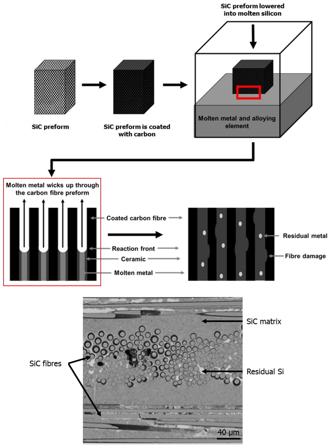
Figure 2.19. The reactive melt infiltration process adapted from [150] and SEM image from the literature showing residual silicon phase between fibres [151].
