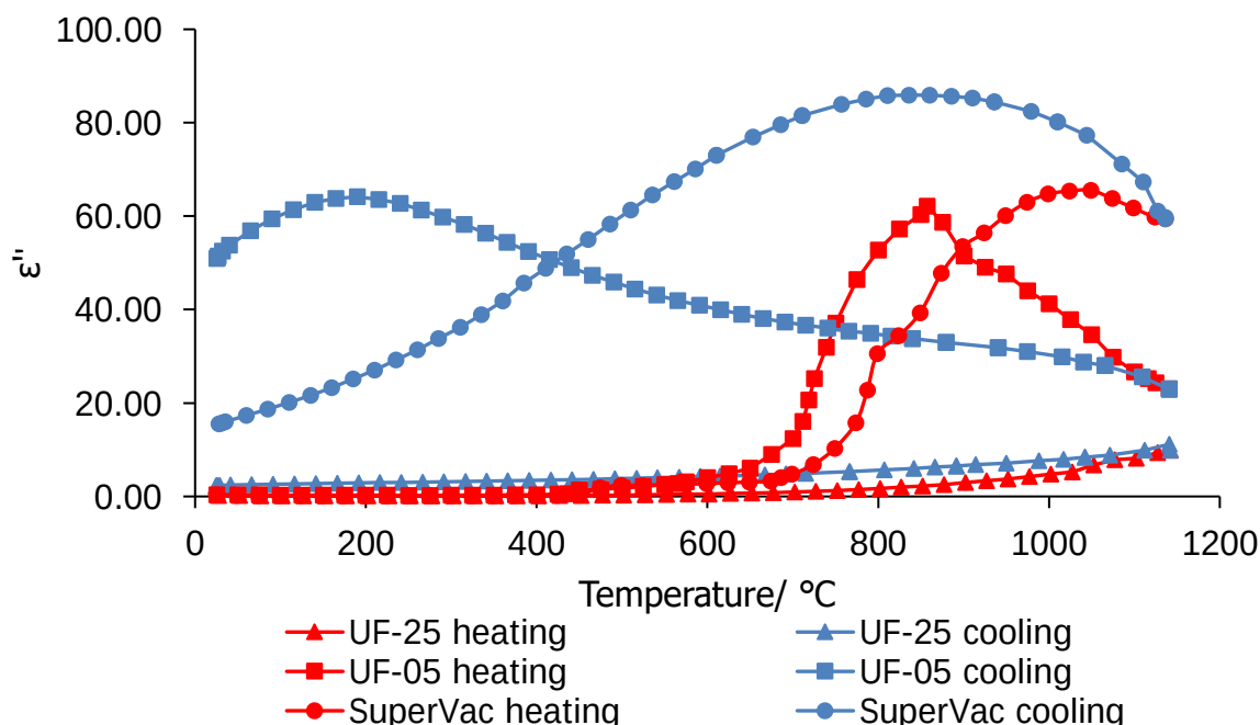
Figure 4.67. The changing loss component of the dielectric permittivity (imaginary part) of the three powders with increasing temperature upon heating (red) and cooling (blue).
