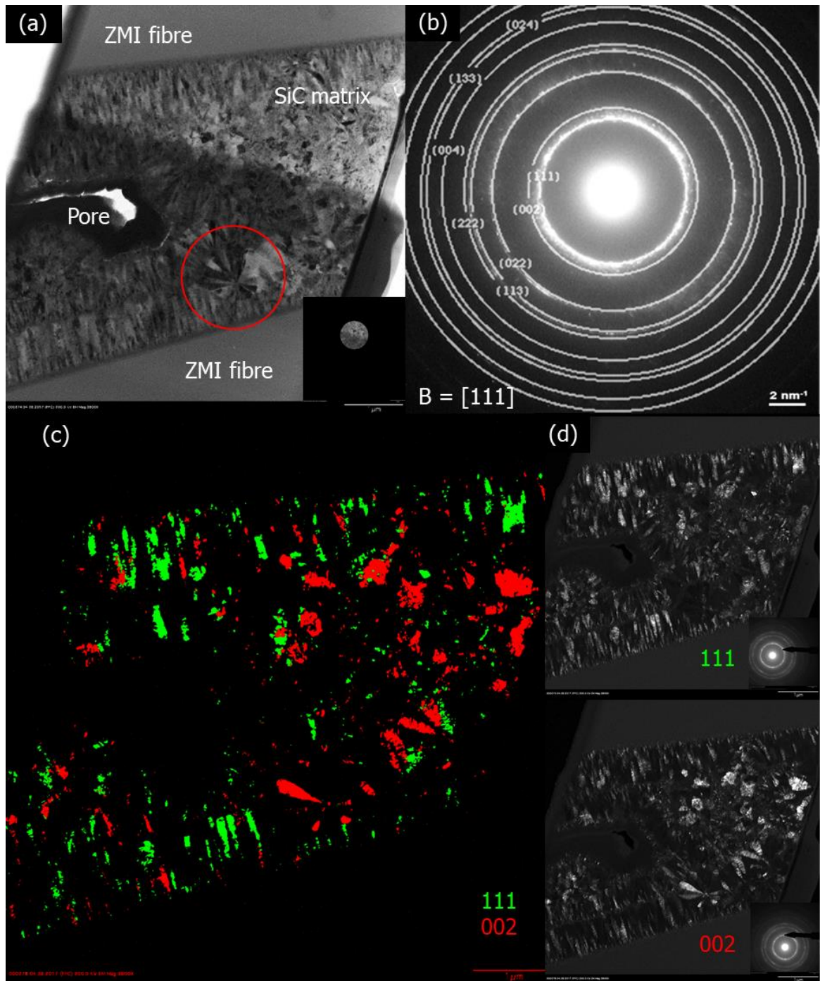
Figure 4.29. (a) A bright-field image of a SiC f /SiC foil taken at the centre of 900°C 300 mbar sample, (b) selected area electron diffraction pattern of the SiC matrix, (c) two overlaid and coloured dark-field images corresponding to the images in (d).
