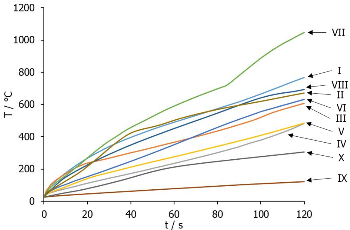
Figure 4.56. Graph showing the ten frequencies selected and how the temperature of the \text{SiC}_f preform changed with time.
