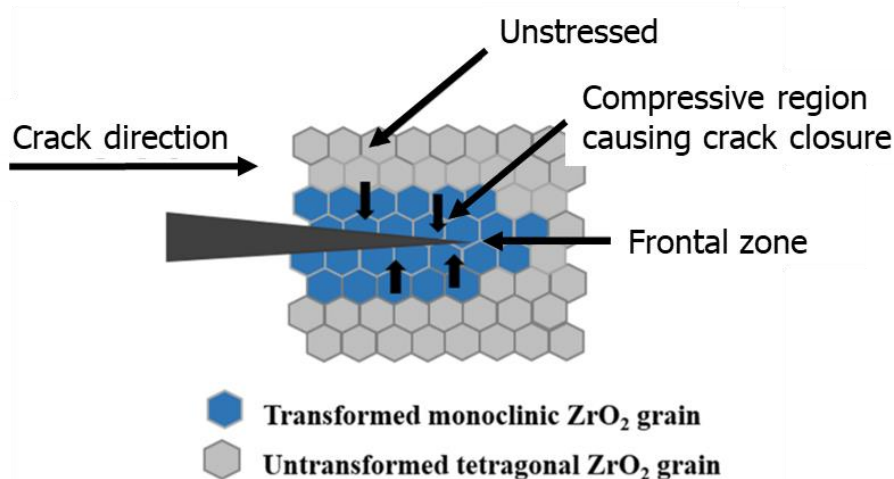
Figure 2.3. The transformation toughening mechanism in partially stabilised YSZ, adapted from [56].
