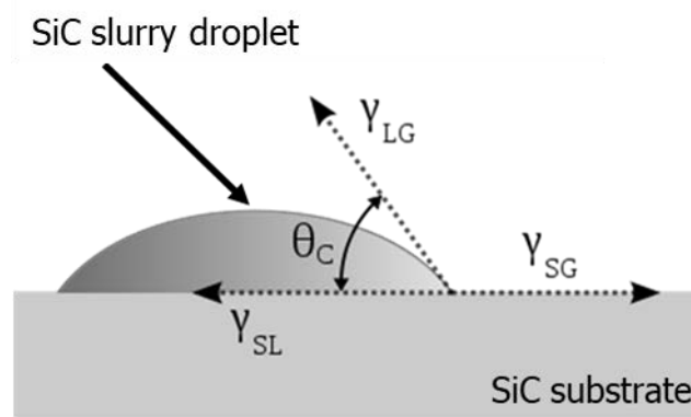
Figure 4.68. A schematic representation of the sessile drop test of the SiC slurry droplet on a SiC substrate where \gamma_{SL} , \gamma_{LG} and \gamma_{SG} are solid-liquid, liquid-gas and solid-gas respectively. Figure adapted from [396].
