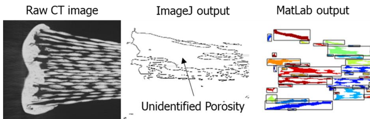
Figure 4.83. Three images detailing the differences pore detection between the ImageJ tools and the MATLAB script.
