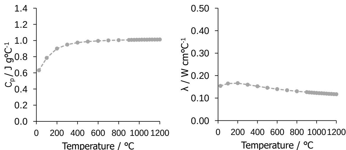
Figure 4.51. Left: Specific heat capacity of the Hi NiC S SiC fibre after post-processing, which was fitted with a logistic model with R^2 = 0.98 . Right: the thermal conductivity of the SiC fibre after processing fitted to a logistic curve with R^2 = 0.99 . Note that the units are specific to the QWED 3D software.
