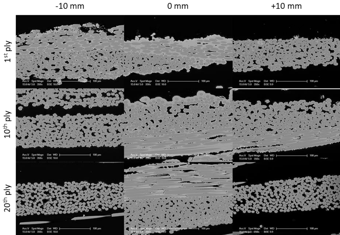
Figure 4.17. Higher magnification micrographs showing the effect of the quartz bridge on another alpha 10 sample, showing densification occurring preferentially in the centre region.
