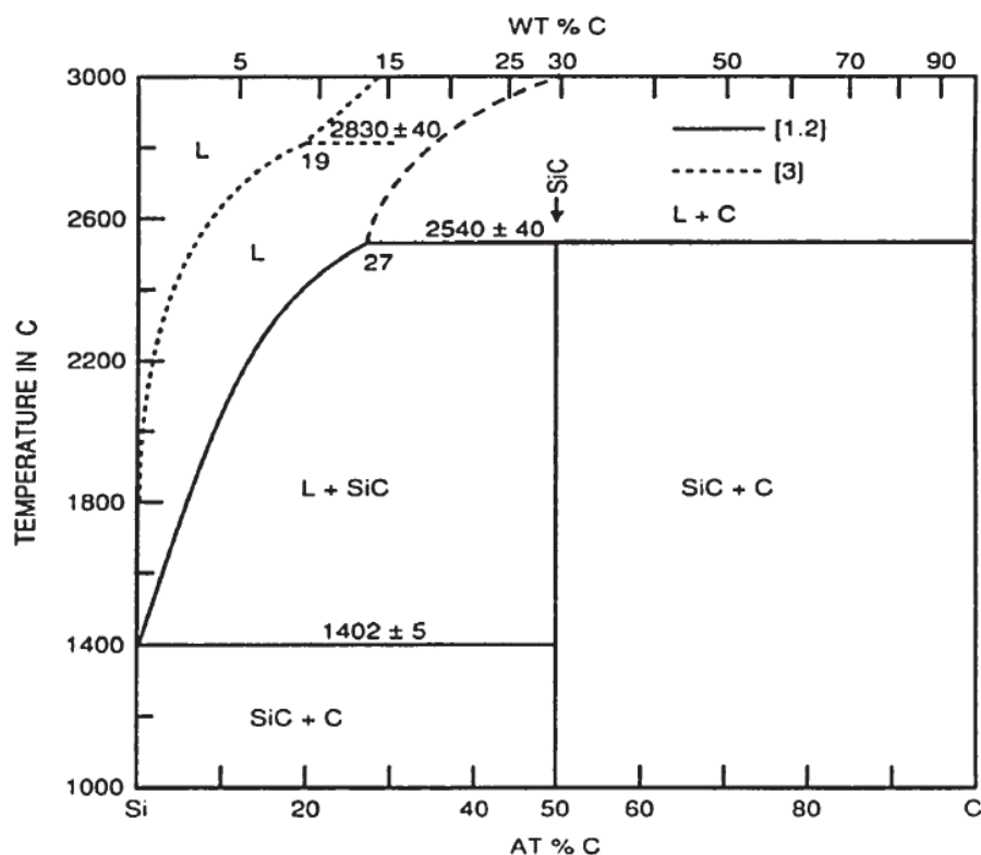
Figure 2.7. An example of part of the SiC phase diagram [79].
