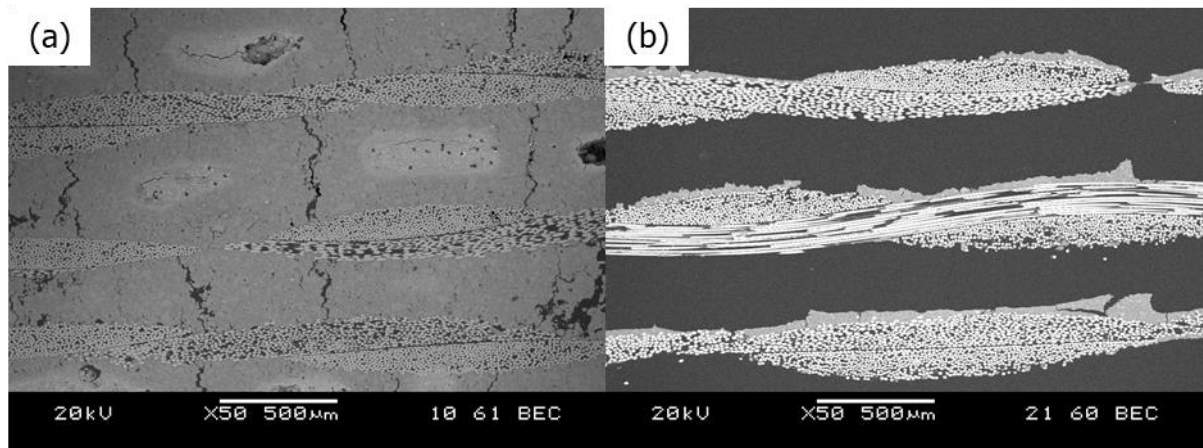
Figure 3.10.(a) SEM micrograph of a polished cross-section of a dipped sample, and (b) the polished cross-section of a painted sample that has delaminated.
