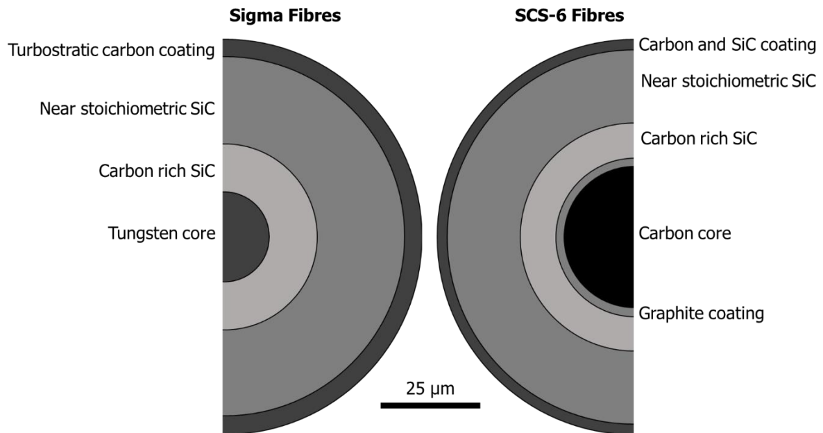
Figure 2.10. Schematic representation of the cross-sections of the two commercially available CVD SiC fibres adapted from [89].
