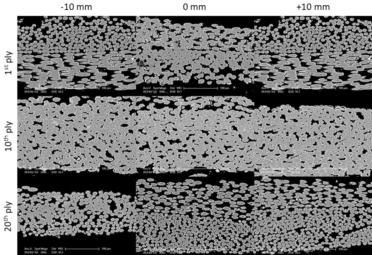
Figure 4.14. Higher magnification micrographs of the alpha 5 sample, showing uniform densification.
