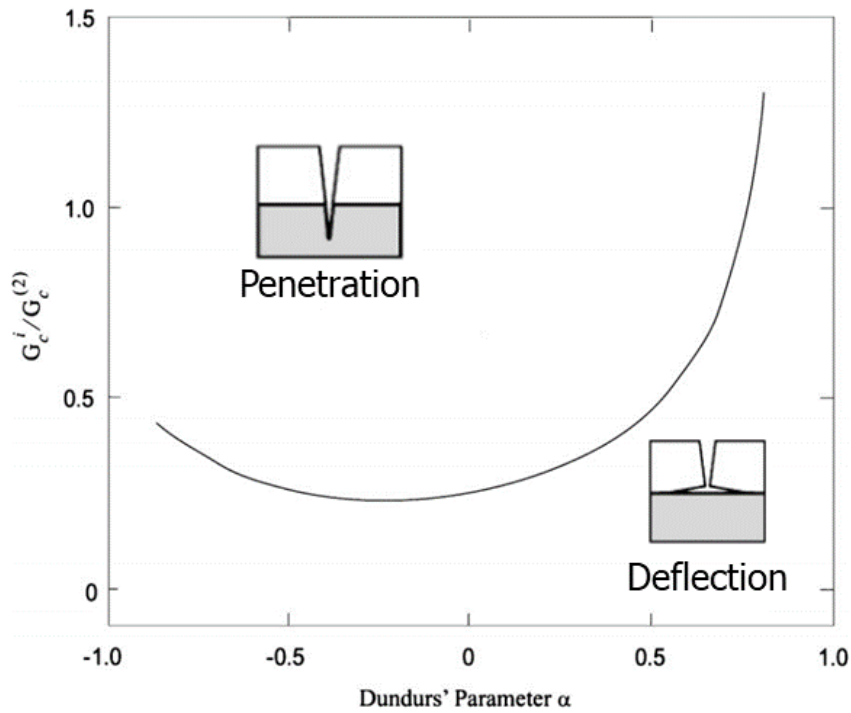
Figure 2.4. A graphical contour separating two regions of crack deflection and penetration based on toughness against the Dundur's parameter that describes the elastic mismatch between components, adapted from [20, 59].
