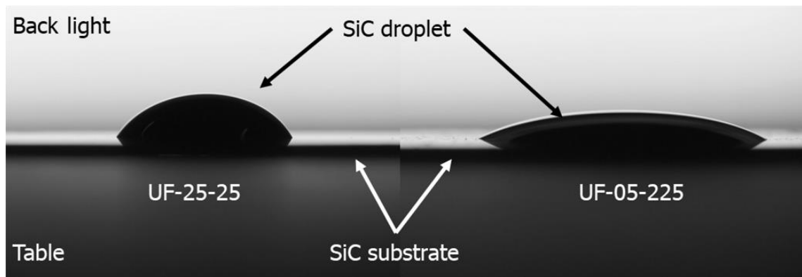
Figure 4.71. Difference between the least wetting and most wetting slurries respectively at T_0 .
