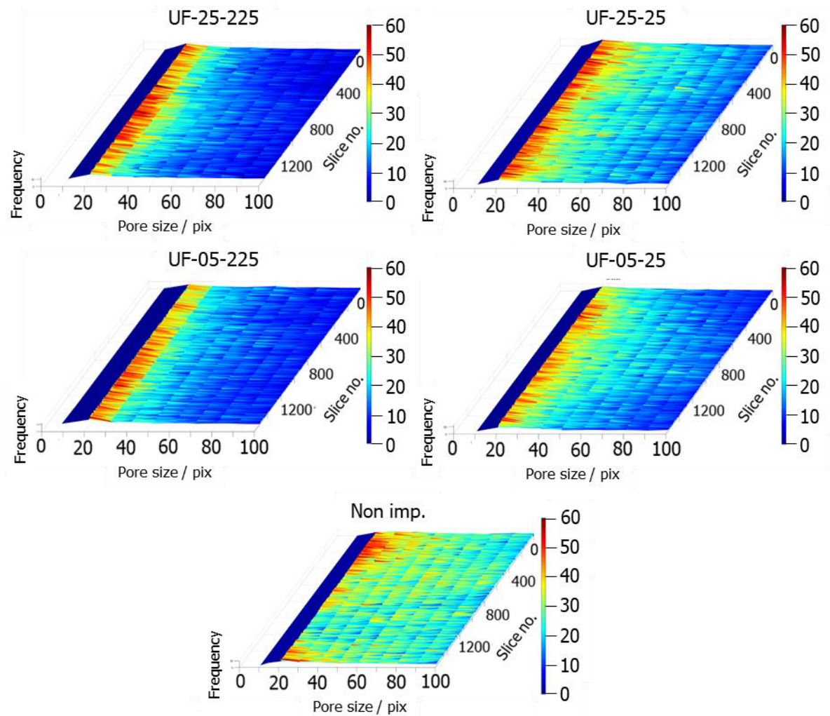
Figure 4.80. Histograms showing the pore count distribution for one composite from each sample set as a function slice number taken from the YZ plane, with a bin size of 10 and a max range of 100 pixels.
