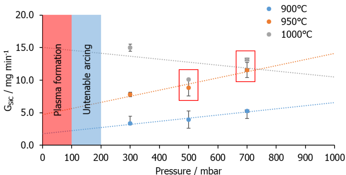
Figure 4.1. SiC matrix growth rate as a function of increasing chamber pressure for samples processed at different temperatures. Gas flow rates and alpha ratio were kept constant at Q_{H_2} = 300\ cm^{-3}\ min^{-1} , Q_{MTS} = 0.2\ g\ min^{-1} and \alpha = 10 respectively. Details for samples inside the red boxes with reduced infiltration times can be seen in Figure 4.7.
