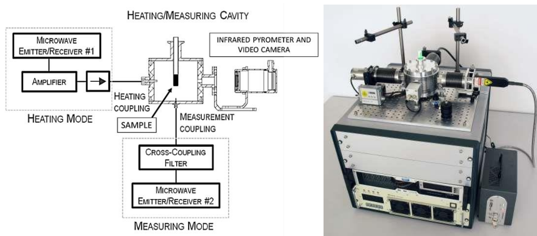
Figure 3.25.(a) Microwave system design for measuring samples' dielectric properties as a function of temperature, adapted from [344] and (b) a photograph of the respective equipment [345].
