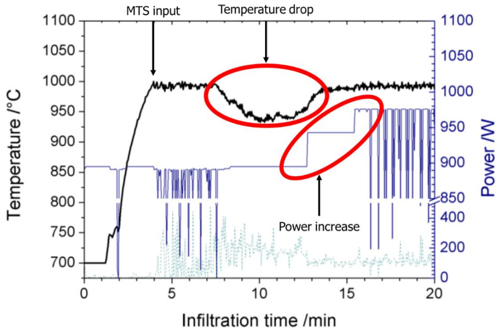
Figure 3.17. Adapted from [250] showing the decrease in temperature after MTS is introduced into the reaction vessel and the power increase needed to regain the lost temperature.
