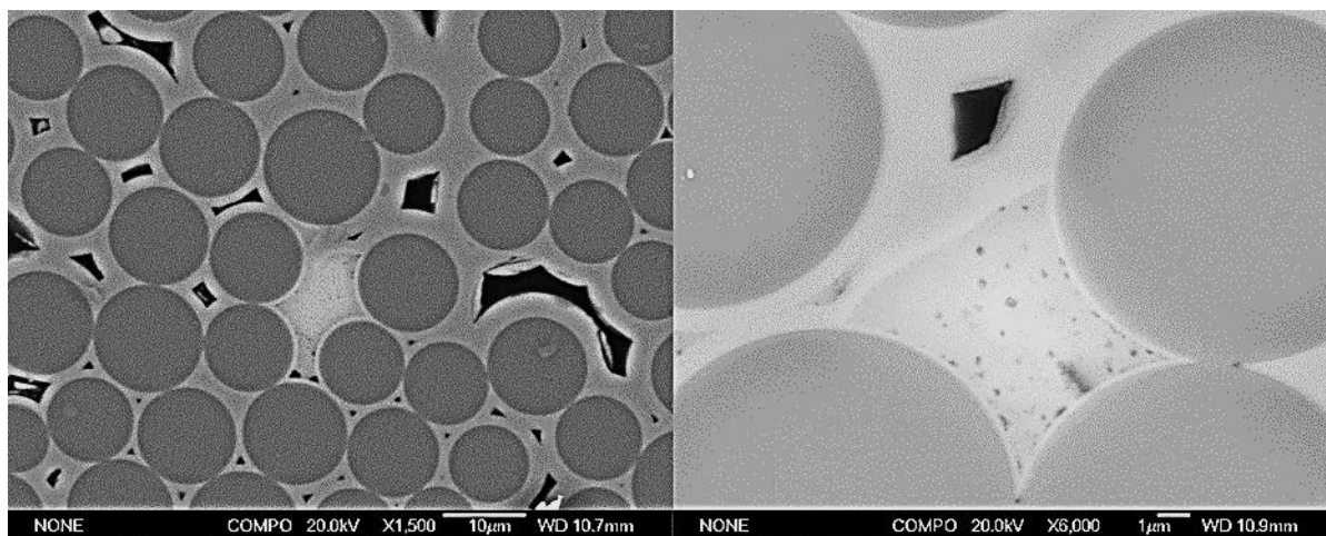
Figure 4.27. Two micrographs showing the free silicon in between the SiC fibres.
