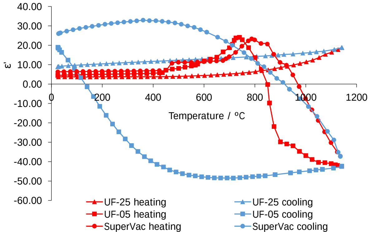
Figure 4.66. The changing dielectric permittivity (real part) of the three powders with increasing temperature upon heating (red) and cooling (blue).
