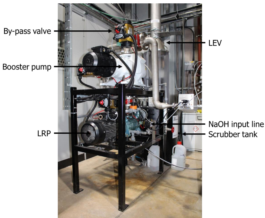
Figure 3.8. Photo of the pumping stack with the key components labelled.
