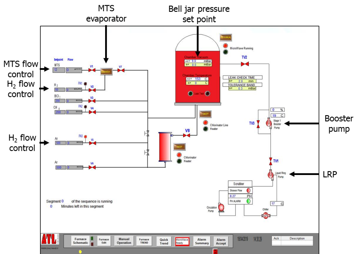
Figure 3.14. Gas delivery system control panel, where gas flow rates, pressure and pumps could be controlled.
