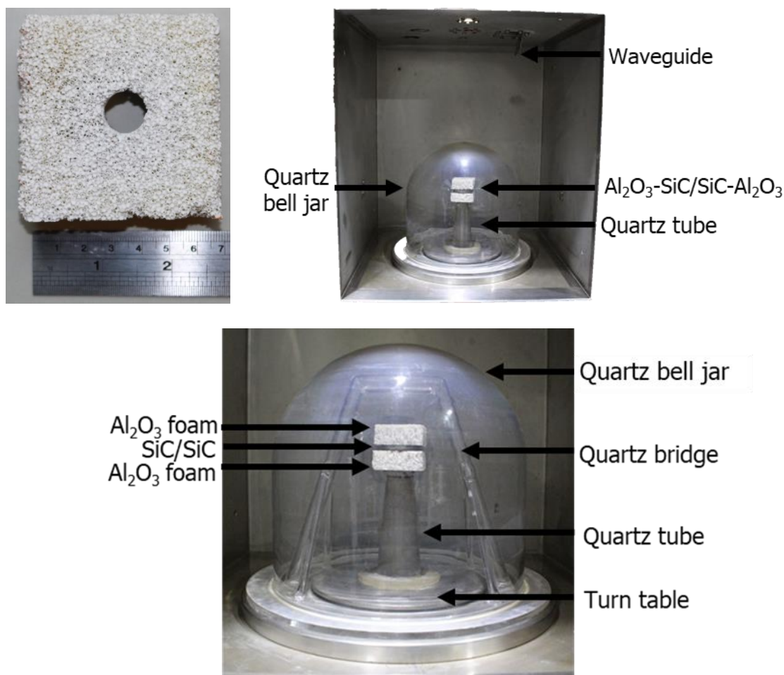
Figure 3.13. Image of the Al 2 O 3 foam used and the setup of the cavity, in later experiments a quartz bridge was used to modify flow this is described in more detail in section 4.1.1.2.
