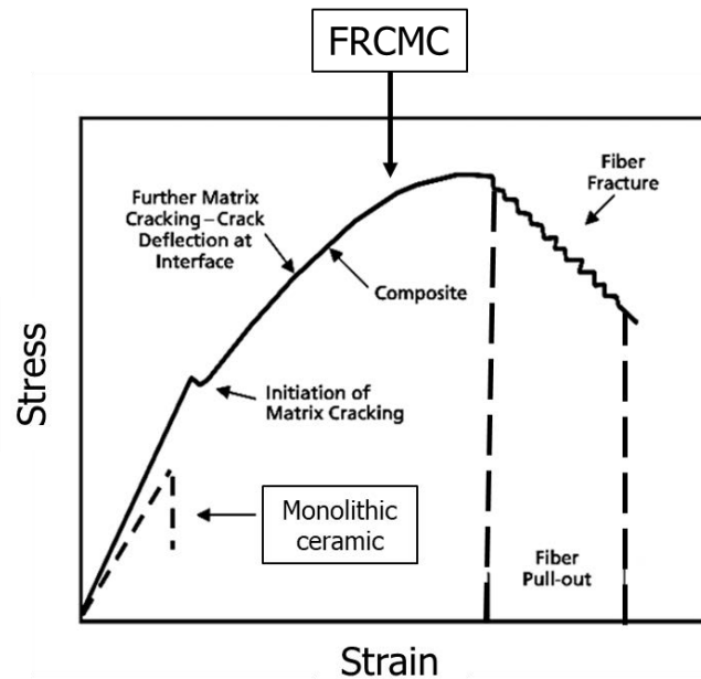
Figure 2.1. Annotated stress-strain curve showing the fracture of a FRCMC compared to a monolithic ceramic [12].
