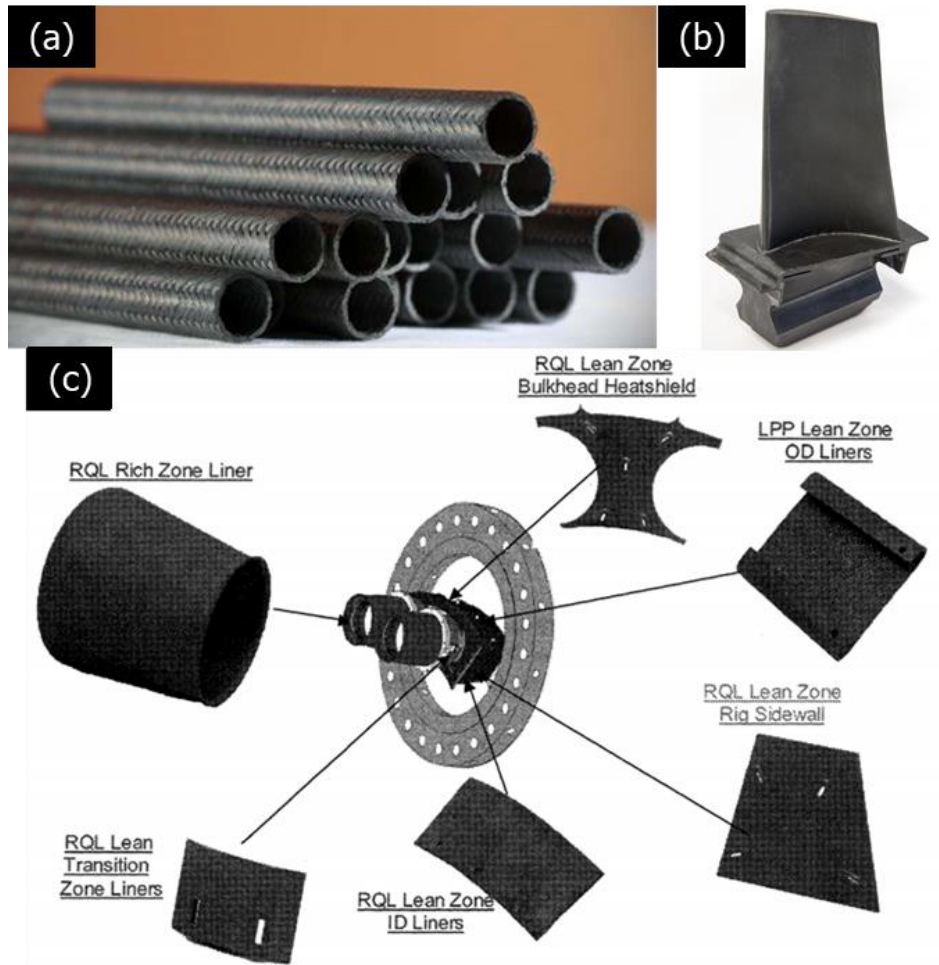
Figure 5.1. (a) Nuclear fuel cladding rods, (b) GE CMC blade from LEAP engine and (c) various components of combustor liner for simulated gas turbine engine cycle.
