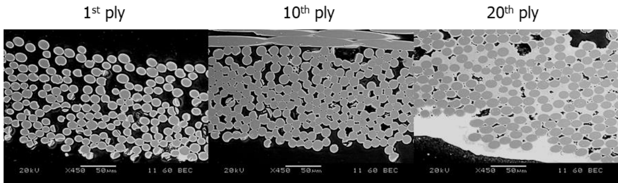
Figure 4.10. Three micrographs showing the localised Si-SiC deposition on the bottom surface of the 1000°C 700 mbar sample compared to the 1 st ply.
