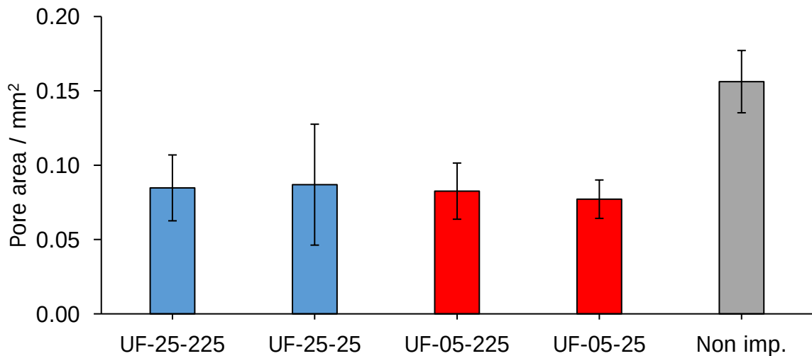
Figure 4.75. A bar graph showing the mean pore area inside the SiC f /SiC.
