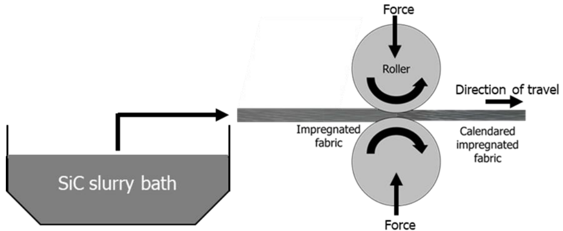
Figure 3.11. Schematic of the calendaring process showing the decreasing saturation of SiC fibre with SiC slurry.
