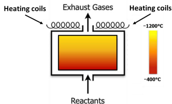
Figure 2.24. Schematic showing the key components of the thermal gradient process and the respective temperature profile [150].
