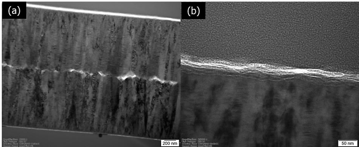
Figure 4.38. BF images showing delamination of the matrix from the fibre from \alpha = 5 .
