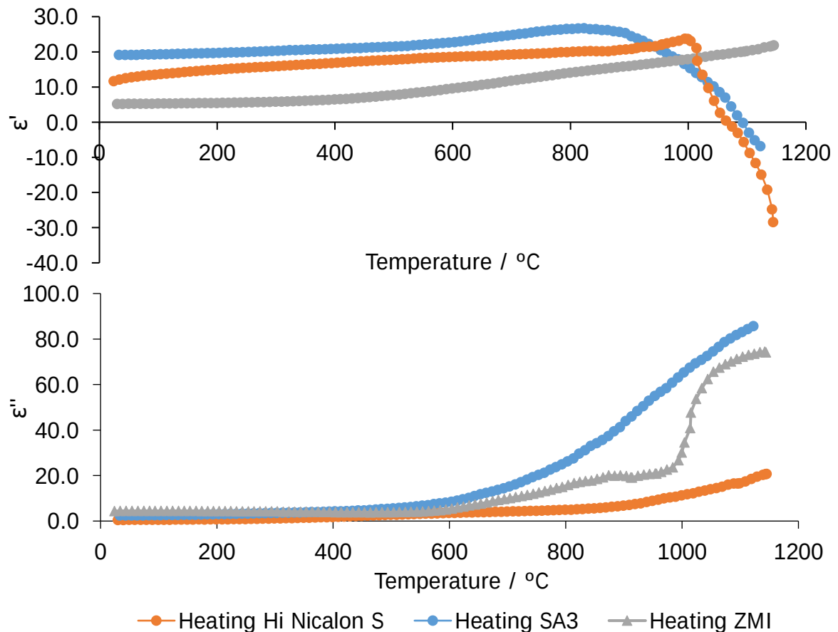
Figure 4.45. Changing dielectric properties of the 3 types of SiC fibres, top: \epsilon' , bottom: \epsilon'' ; note the unusual behaviour of the SA3 and ZMI fibres at temperatures >800^{\circ}\text{C} .
