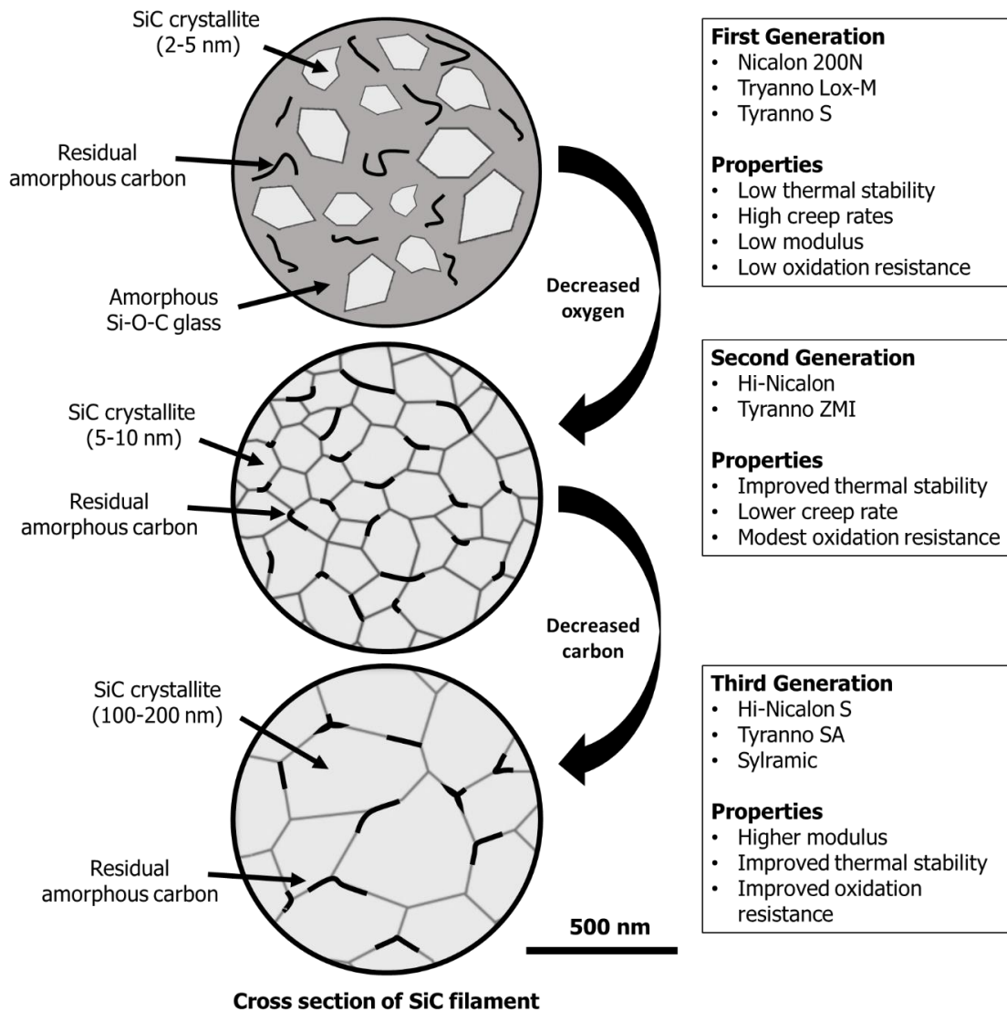
Figure 2.11. Schematic cross-sectional representations of the microstructure of three generations of commercially available SiC fibres, adapted from [89, 104].
