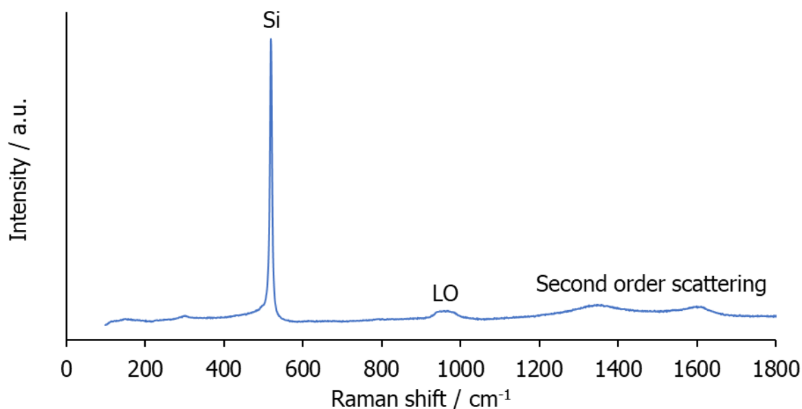
Figure 4.26. Raman spectra of the free silicon in the SiC deposit produced at high infiltration pressures.
