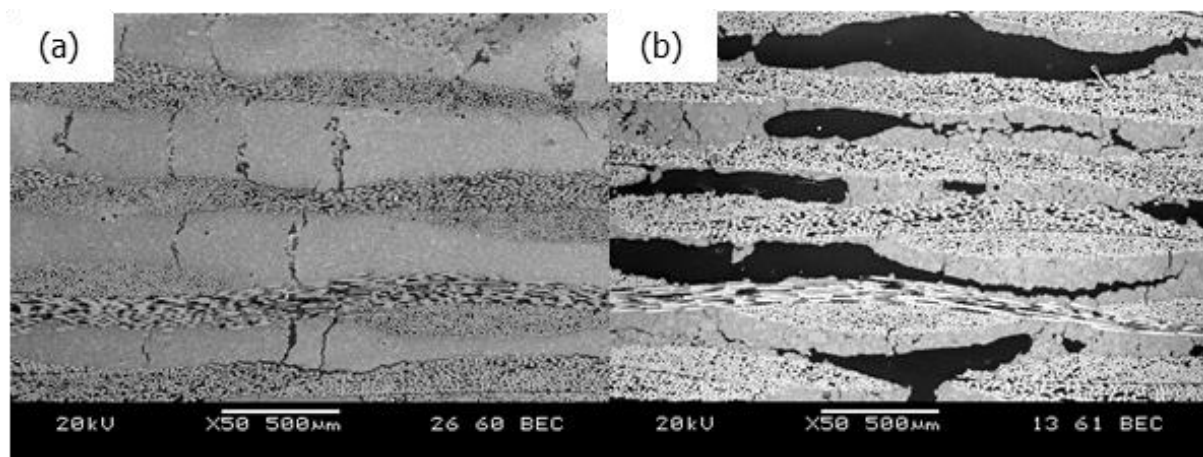
Figure 4.65. (a) An SEM cross-section of UF-25-25 preform, showing the fibres crossing the image horizontally and the large crack SiC powder matrix, (b) the thinner and more porous cross-section of the SV-25 preform.
