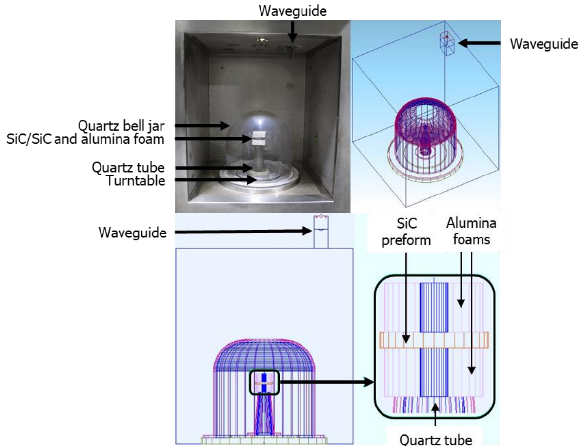
Figure 3.26. Labotron HTE M30KLB Pro; cavity, 3D view of the internal structure and components and a magnified view of the SiC f /SiC-Al 2 O 3 foam arrangement.
