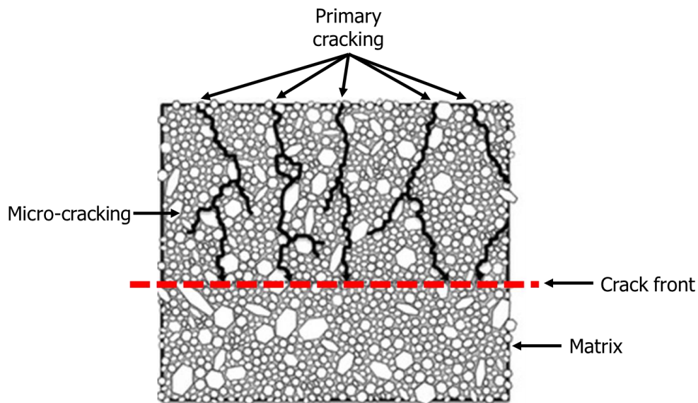
Figure 2.2. Schematic of the micro-cracking process, adapted from [44].
