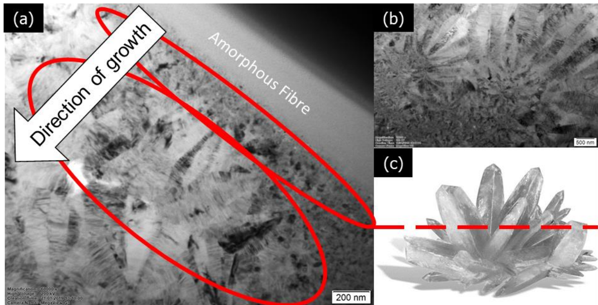
Figure 4.40. (a) Change in the crystal size as the grain growth proceeds from the fibre in \alpha = 10 , (b) higher mag image of the flow-like structures produced by the sectional of crystals growing radially from a central point, as illustrated in (c).
