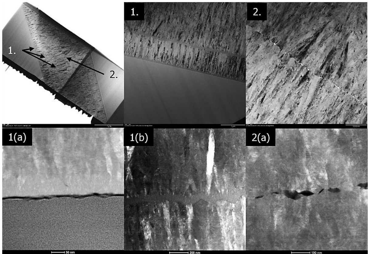
Figure 4.34. High-resolution BF images of the microstructural features seen in 1000°C 300 mbar sample. 1. Amorphous \text{SiO}_2 banding at the fibre-matrix interface, and 2. Nano-porosity formed between converging SiC grains from neighbouring fibres.
