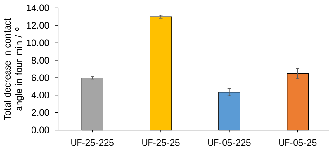
Figure 4.72. The total decrease in contact angle over a four-minute period of the four different slurries.
