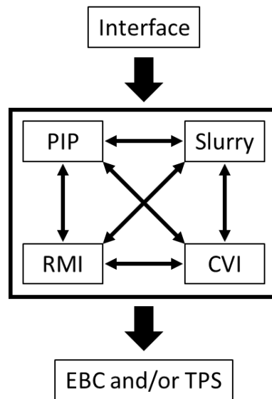
Figure 2.28. Schematic representation of the combinations of matrix formation techniques after an interface material is applied and before an EBC or TPS.
