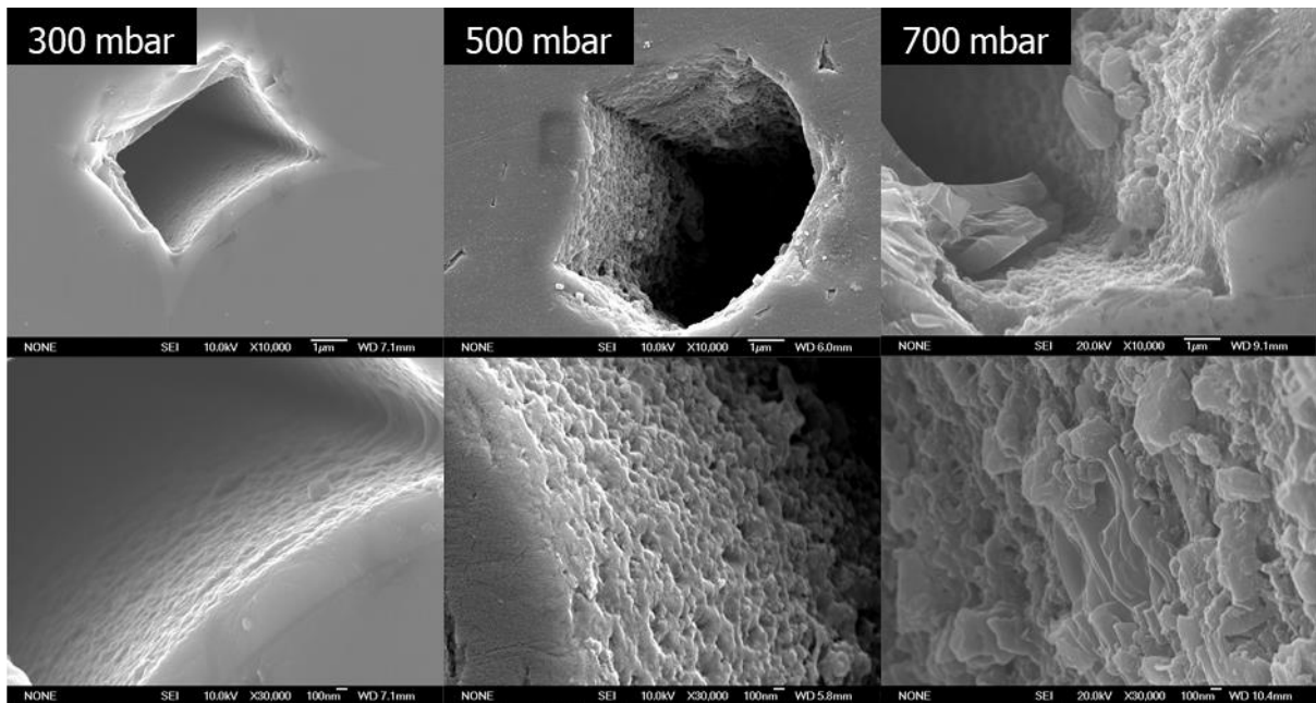
Figure 4.19. Images of the SiC deposit at different pressures but using the same magnification showing a significantly increased surface roughness with increasing pressure.
