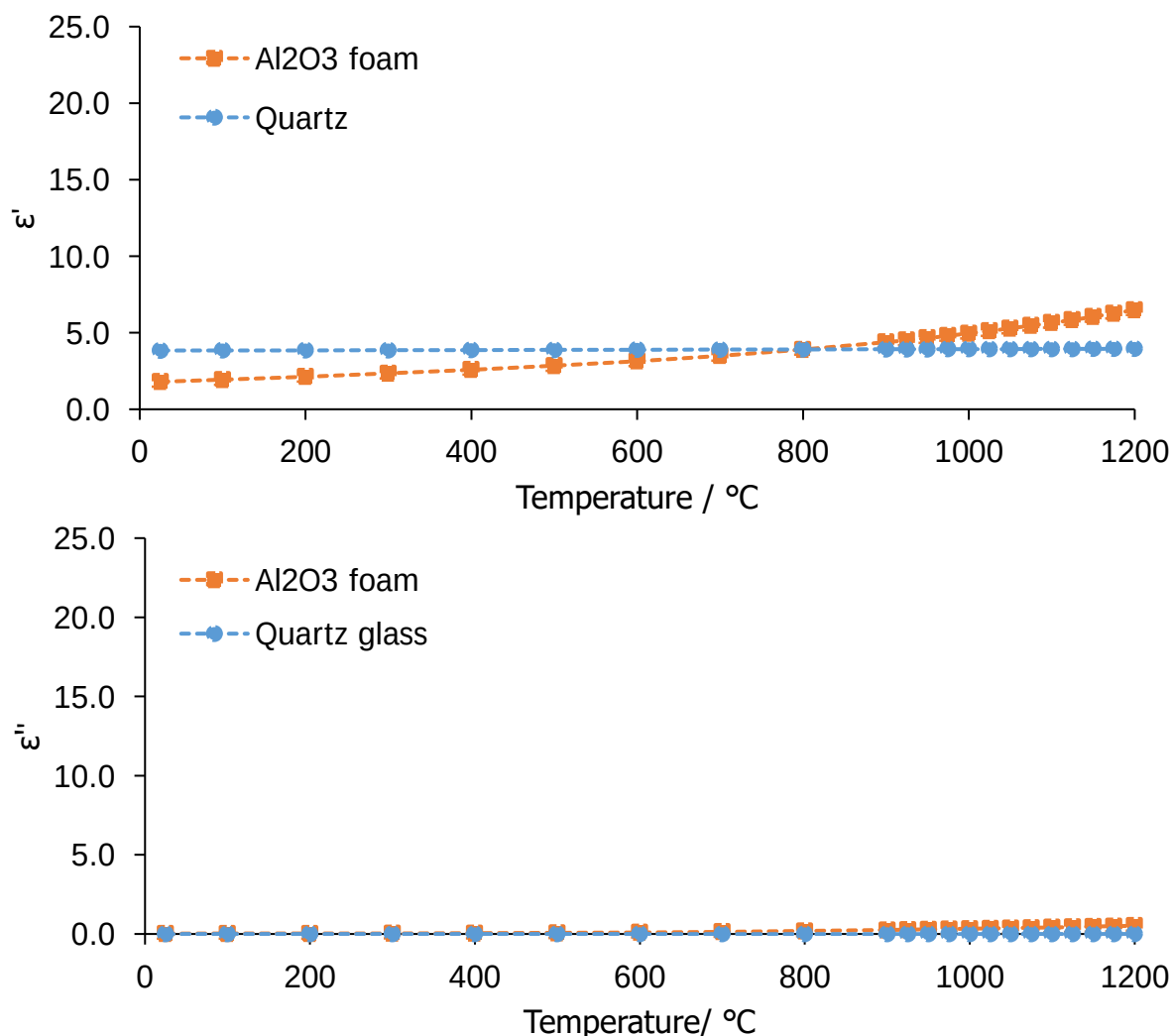
Figure 4.47. Top: The dielectric permittivity for the \text{Al}_2\text{O}_3 foam and quartz after interpolation using Origin. \epsilon' for the \text{Al}_2\text{O}_3 foam was fitted with a two-phase exponential decay function with R^2 = 0.96 and \epsilon' for the quartz was fitted using a Boltzmann model with R^2 = 0.98 . Bottom: Dielectric loss factor for the \text{Al}_2\text{O}_3 foam and quartz after interpolation using Origin. \epsilon'' for the \text{Al}_2\text{O}_3 foam with a Logistic model with an R^2 = 0.98 . \epsilon'' for quartz was fitted using an exponential growth model with an R^2 = 0.93 .
