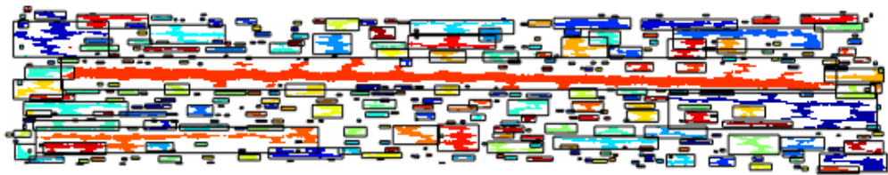
Figure 4.76. Image produced by the MATLAB script highlighting the internal delamination (orange) in UF-25-25 thus skewing the error bar.
