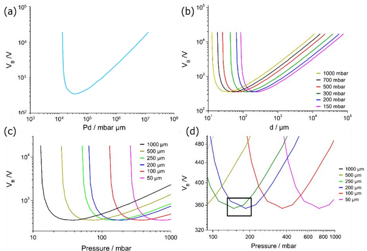
Figure 3.18. Paschen's curve in a hydrogen environment illustrating the relationship between the pressure and electrode distance on the threshold of the breakdown voltage, (b) showing the minimum spacing between electrodes as pressure changes, (c) a graph illustrating the minimum operating pressure for a given set of electrode separations, and (d) magnified
