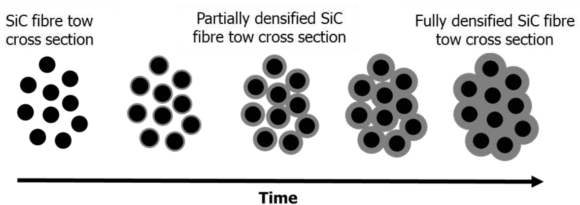
Figure 2.21. An illustration of the development of SiC deposit on the cross-section of the SiC fibres over time, adapted from [150].
