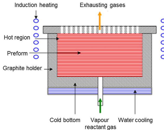
Figure 2.22. Schematic of generic CVD equipment [168].
