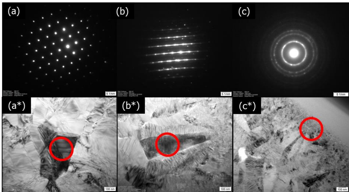
Figure 4.39. (a) SAD pattern showing a grain \alpha -SiC found in the \alpha = 10 sample, (b) a crystalline but heavily twinned grain of SiC and (c) the transitional region between the fibre and textured region of the SiC as indicated.
