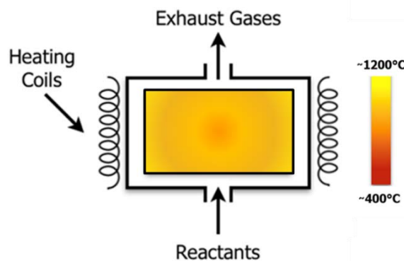
Figure 2.23. Schematic showing the key components of the conventional process and the respective temperature profile [150].
