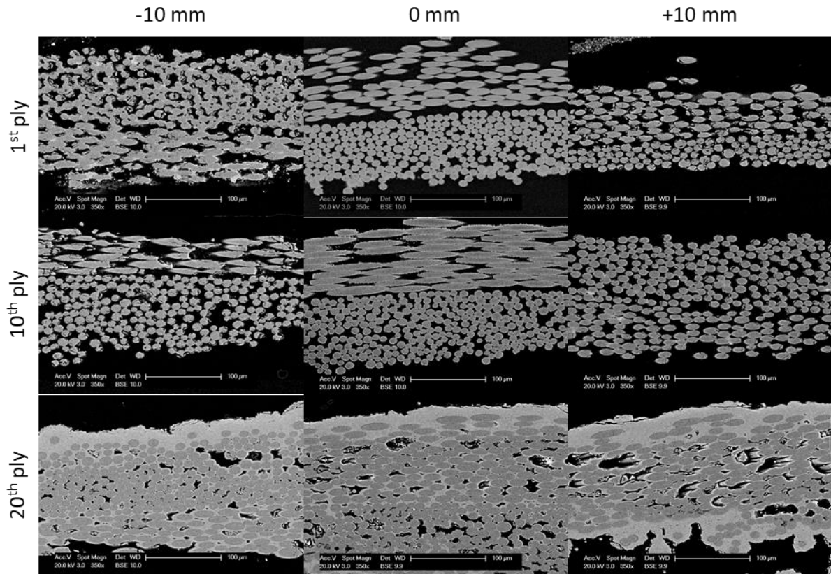
Figure 4.15. Higher magnification micrographs of the alpha 25 sample, showing densification in the 20 th ply only.
