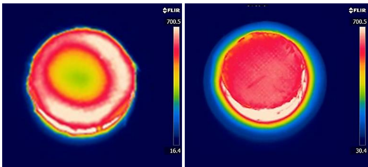
Figure 4.41. Left: An annular temperature profile of 10 ply 34 mm diameter SiC preform heated using microwave energy. Right: Non-uniform heating of 34 mm diameter sample made with 30 ply showing hot edges.
