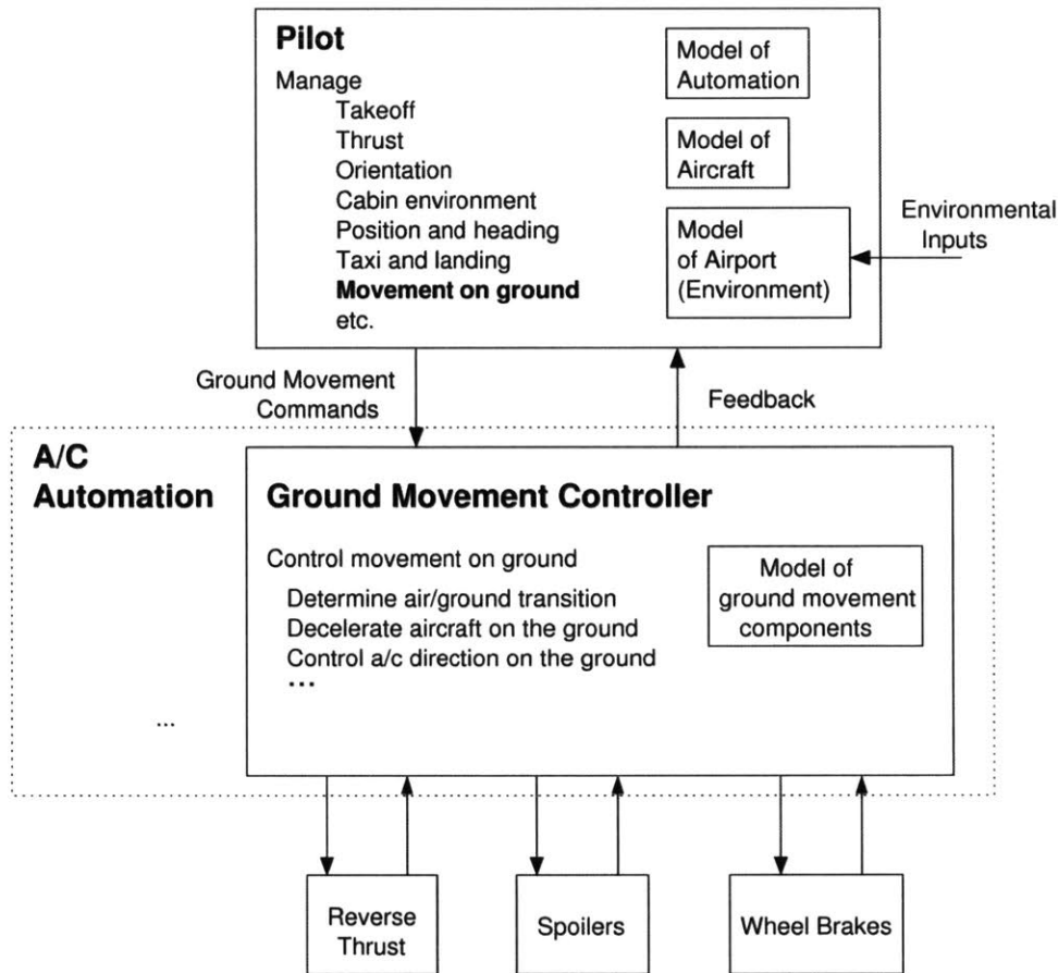
Figure 12. The portion of the safety control structure related to deceleration on the ground.
