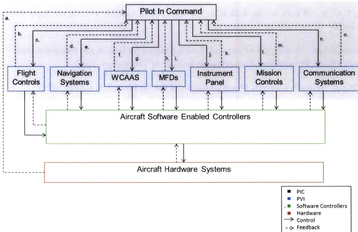
Figure 28. Details of the interactions of the PIC with the different parts of the Pilot Vehicle Interface (PVI) (hardware and software). To make the model more readable, only the details of the PIC and PVI are shown, with the other boxes providing overall context. The blue boxes represent physical interfaces as well as embedded software.
