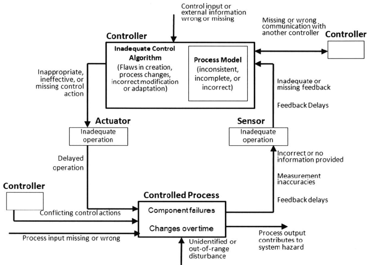
Figure 23. Some control flaws that can lead to unsafe control. Note that component failures are included but control flaws other than component failures are also considered
