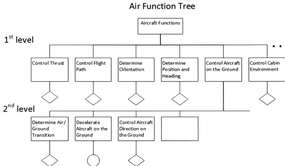
Figure 10. Two levels of a classic functional decomposition for an aircraft [18]
