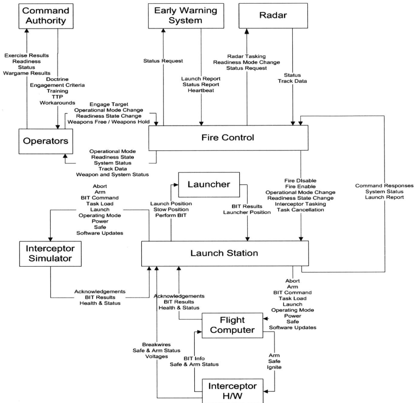
Figure 9. Safety Control Structure for a fictional Ballistic Missile Defense System. [17]
