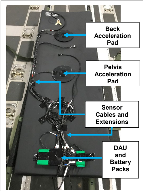
Figure 3. DAU and batteries, back and pelvis acceleration pads attached to litter.
