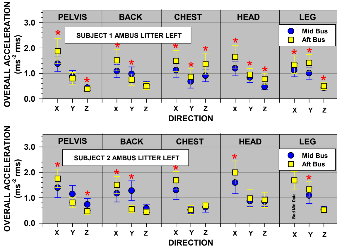
Figure A-3. Mean Overall Unweighted Accelerations ± One Standard Deviation: Mid vs Aft Litter Location (Note: X (Vertical), Y (Lateral), Z (Longitudinal))
