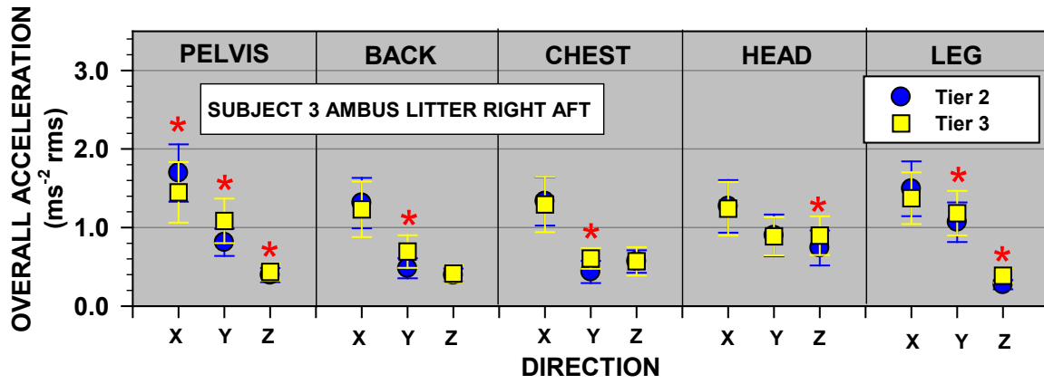
Figure A-5. Mean Overall Unweighted Accelerations ± One Standard Deviation: Tier 2 vs Tier 3
