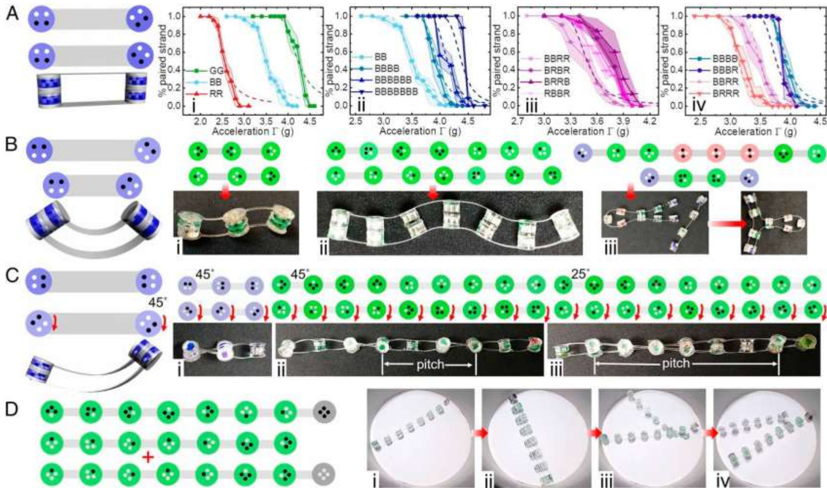
Figure 3. Magnetic strands and the resulting secondary structures.
