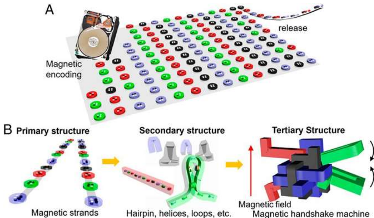
Figure 5. Vision for assembly of magnetic handshake materials.
