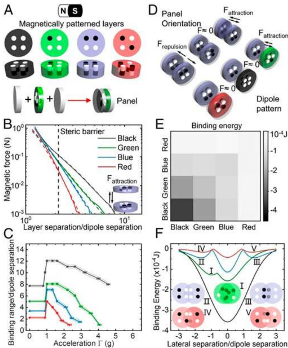
Figure 1. Encoding information into magnetic panels to generate specific interactions.
