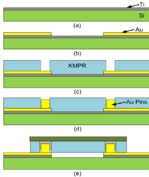
Figure 9: Process flow for fabrication of metal pins on the carrier substrate and final assembly of MMIC chip.
