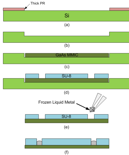
Figure 8: Process flow for liquid metal deposition on the MMIC chip.
