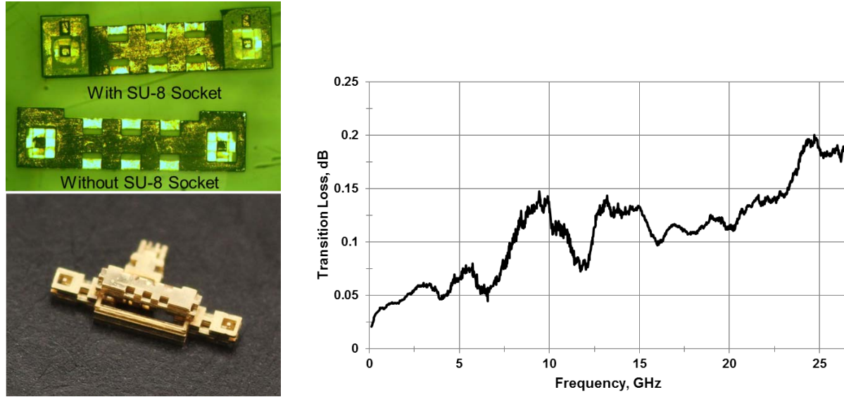
Figure 17: (Left) Micrograph of fabricated Polystrata test structure with rectacoax through line “jumper” in place of MMIC for structural validation and calibration purposes. (Right) Measured transition loss deembedded from two-port S-Parameter measurements of the Polystrata jumper structure.
