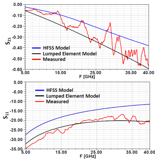
Figure 20: A comparison of a single liquid metal interconnect assembly measured results with HFSS simulation results and simulations of the extracted lumped element model of the assembly.
