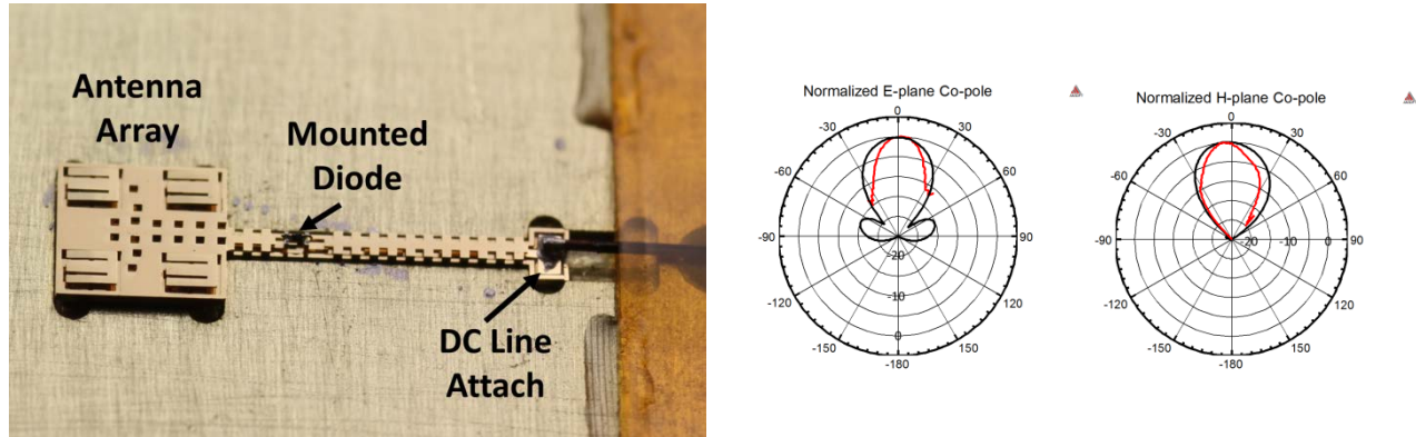
Figure 13: (Left) Mounted Polystrata antenna array with integrated diode detector and DC line. Diode and DC line are attached using silver conductive epoxy. (Right) Normalized E and H plane co-pol patterns: black – simulated with HFSS, red – measured [7].
