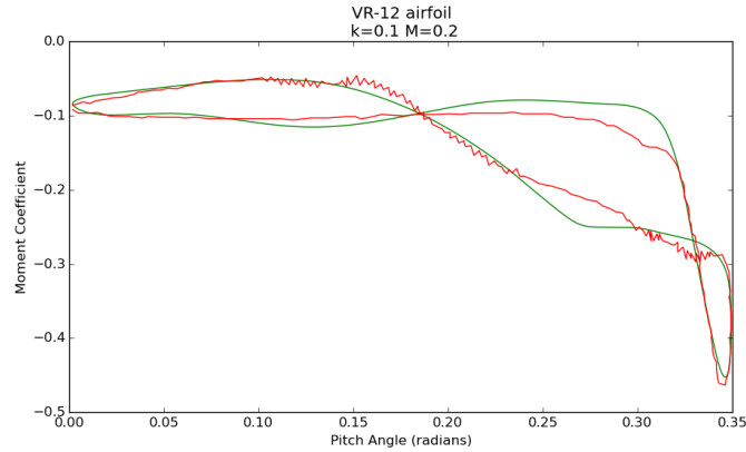
Figure 6: Primary stall model compared to VR-12 data without any secondary peak.
