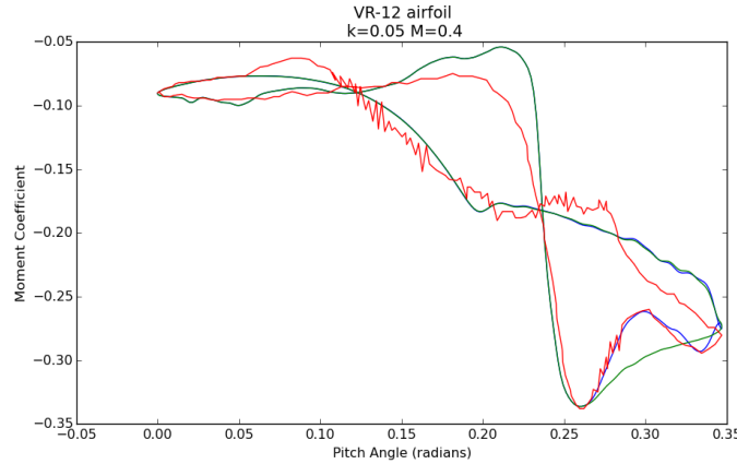
Figure 5: Correlation of pitching moment with data, VR-12, k=0.05 , M=0.4 .
