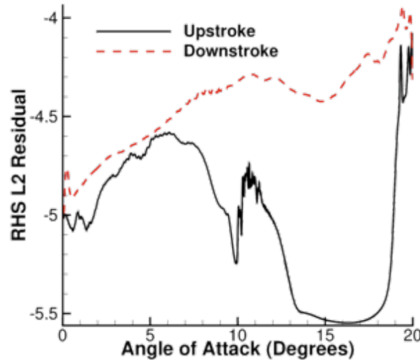
Figure 3: Evaluation of residual behavior over a dynamic stall event.
