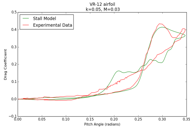
Figure 6: Primary stall model compared to VR-12 data without any secondary peak.
