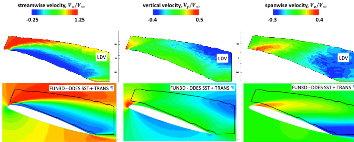
Figure 2: OA209 Wing CFD correlation with PIV Velocity Field at 80% R, \alpha = 19.4^\circ , downstroke
