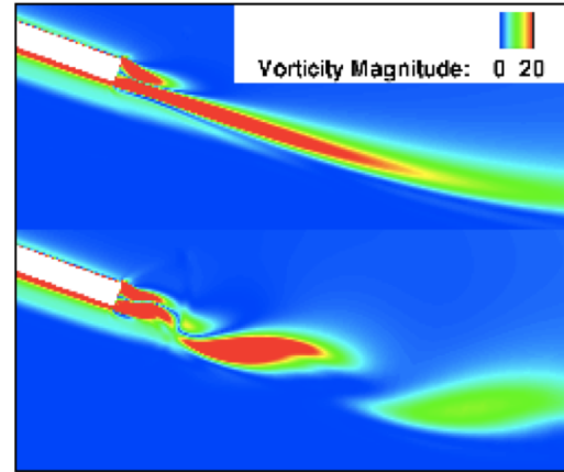
Figure 1: Vorticity at blunt trailing edge for stalled VR7 flow at the same physical time with two different time steps; \Delta t = 0.01 on top and \Delta t = 0.005 on bottom.
