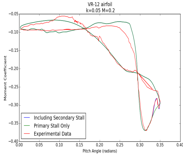
Figure 4: Correlation of pitching moment data for VR-12, k=0.05 , M=0.2 .
