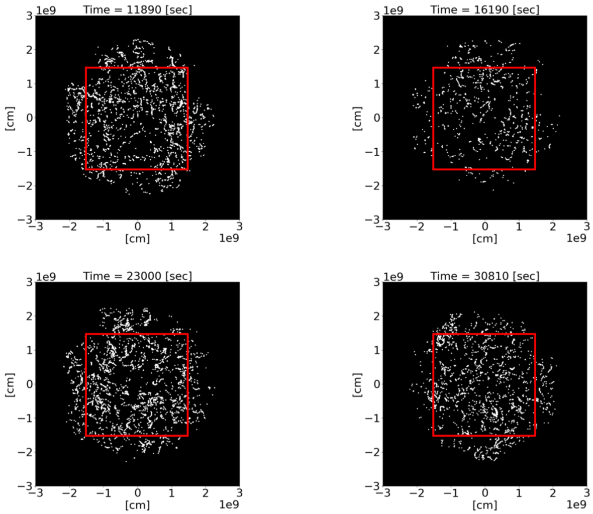
Figure 11 - Map of reconnected field lines at several times during our simulation. The maps show white if reconnection has occurred, and black if there has been no reconnection.
