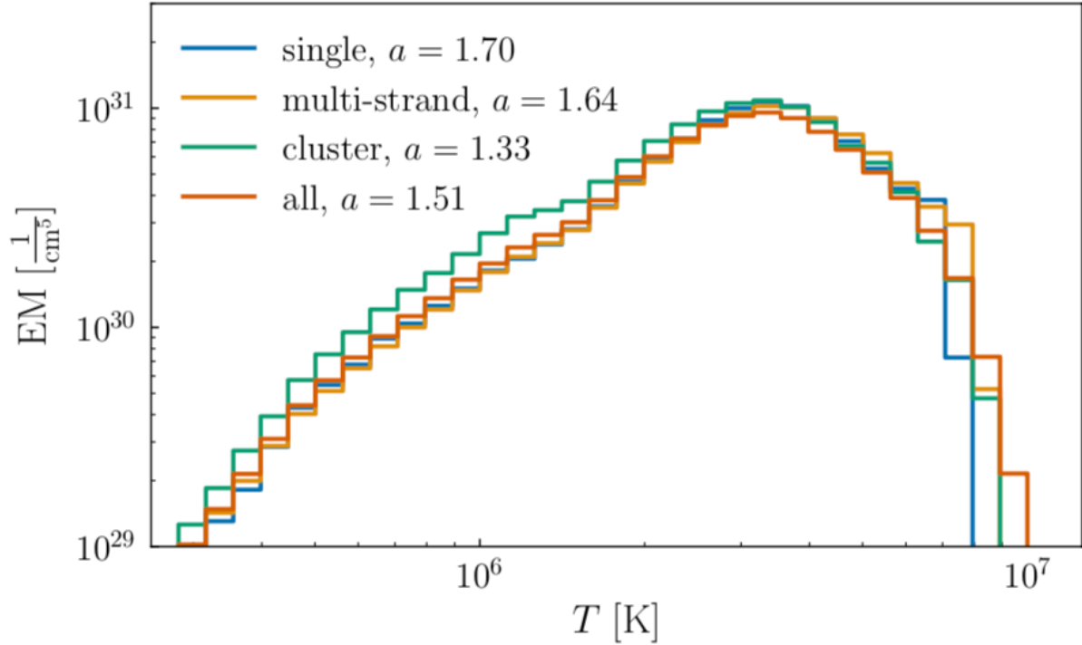
Figure 14 - Emission measure distribution for a single field line, a set of 25 field lines, a set of 350 field lines, and 40000 field lines considered together.
