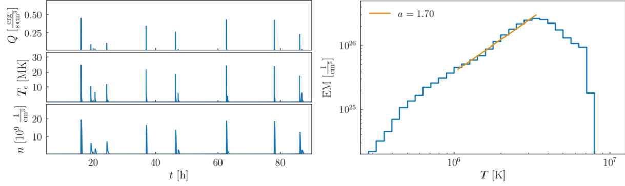
Figure 13 - Left: Heating, temperature, and density profile as determined by EBTEL along a field line chosen at random from our MHD model. Right: Emission measure for this field line.
