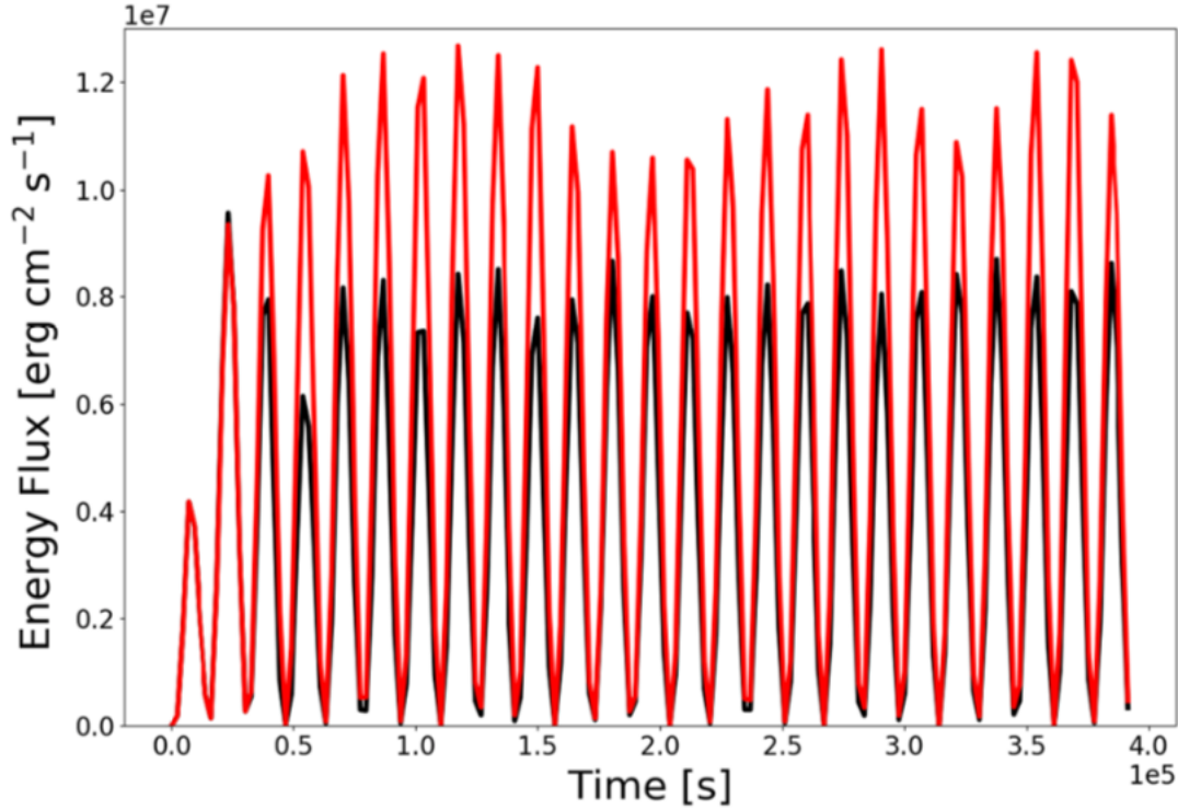
Figure 10 - Poynting Flux injected into the corona by our simulations with all cells rotating clockwise (black) and with half of the cells rotating clockwise and half counterclockwise (red).
