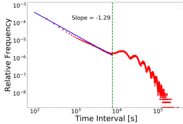
Figure 12 - Distribution of time delays between reconnection events for our simulation, along with a power law slope of best fit.
