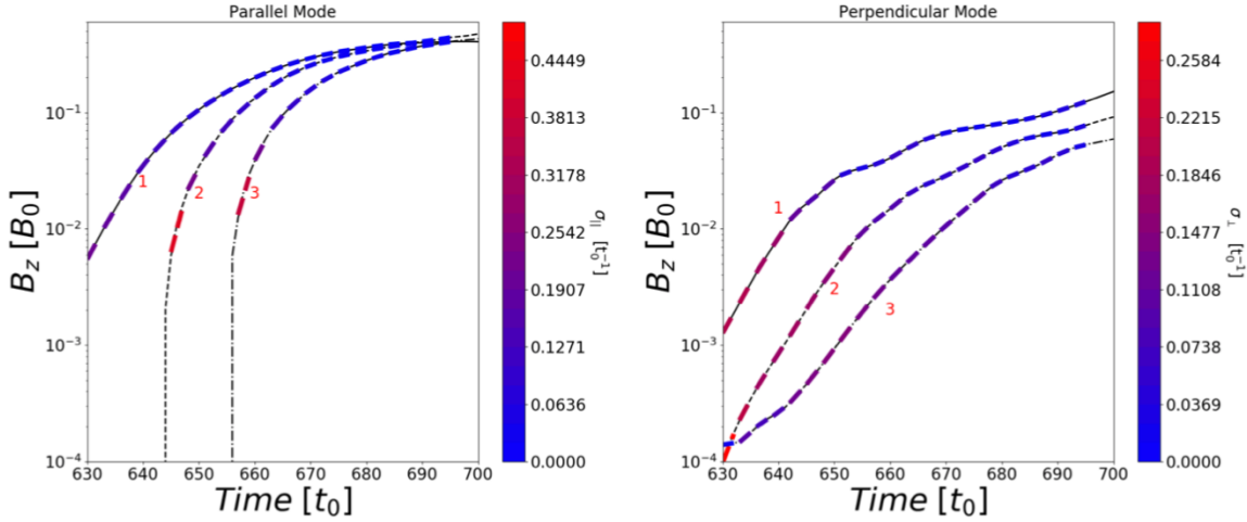
Figure 7 - The amplitude of the three peaks labeled in Figure 5 and Figure 6 as functions of time. The color shading represents the instantaneous growth rate, determined by fitting the data to an exponential function.
