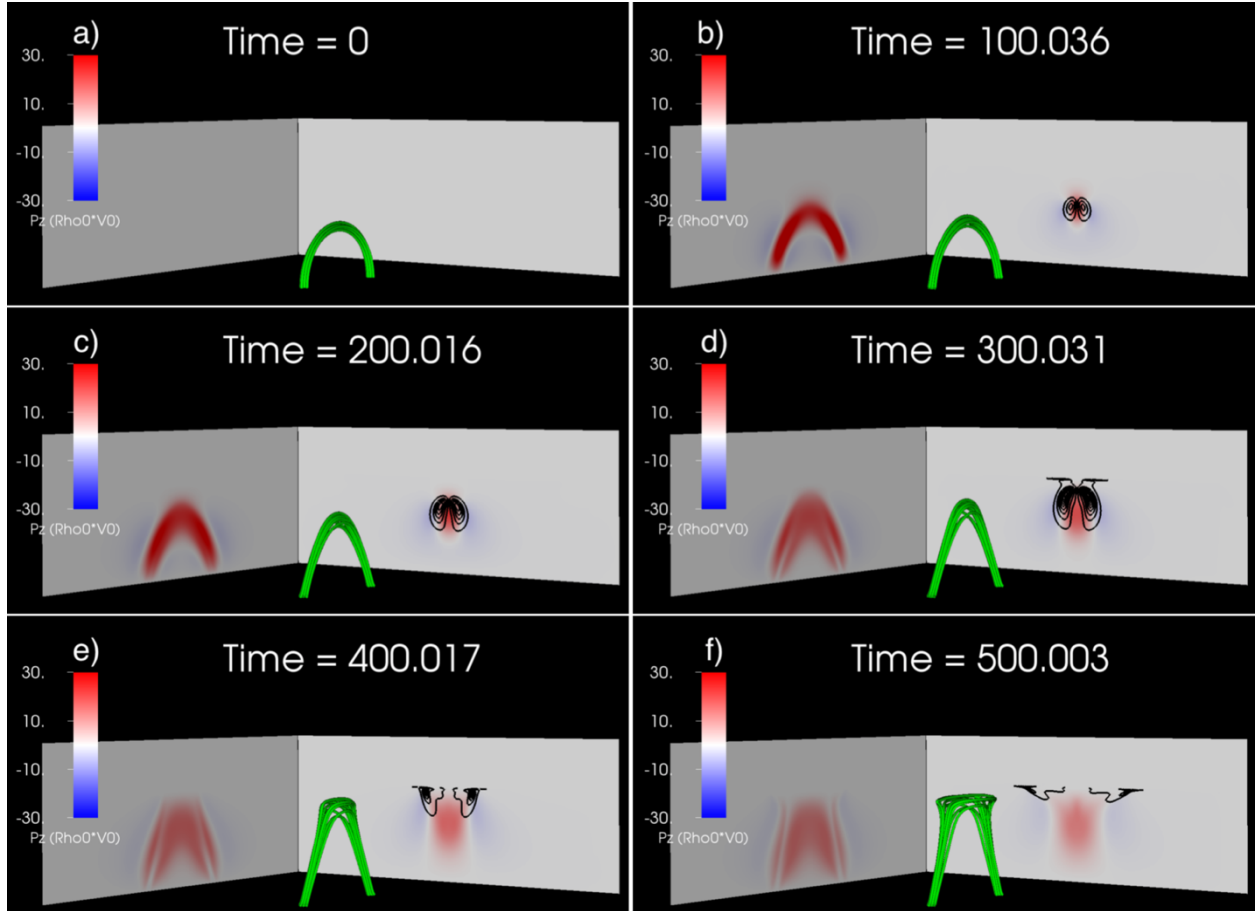
Figure 1 - Field lines in the torus at different times during the simulation, traced from the bottom boundary. Color shading shows vertical momentum, and contours show out of plane vorticity. The two vertical cuts are taken in the x = 0 and y = 0 mid-planes, respectively.
