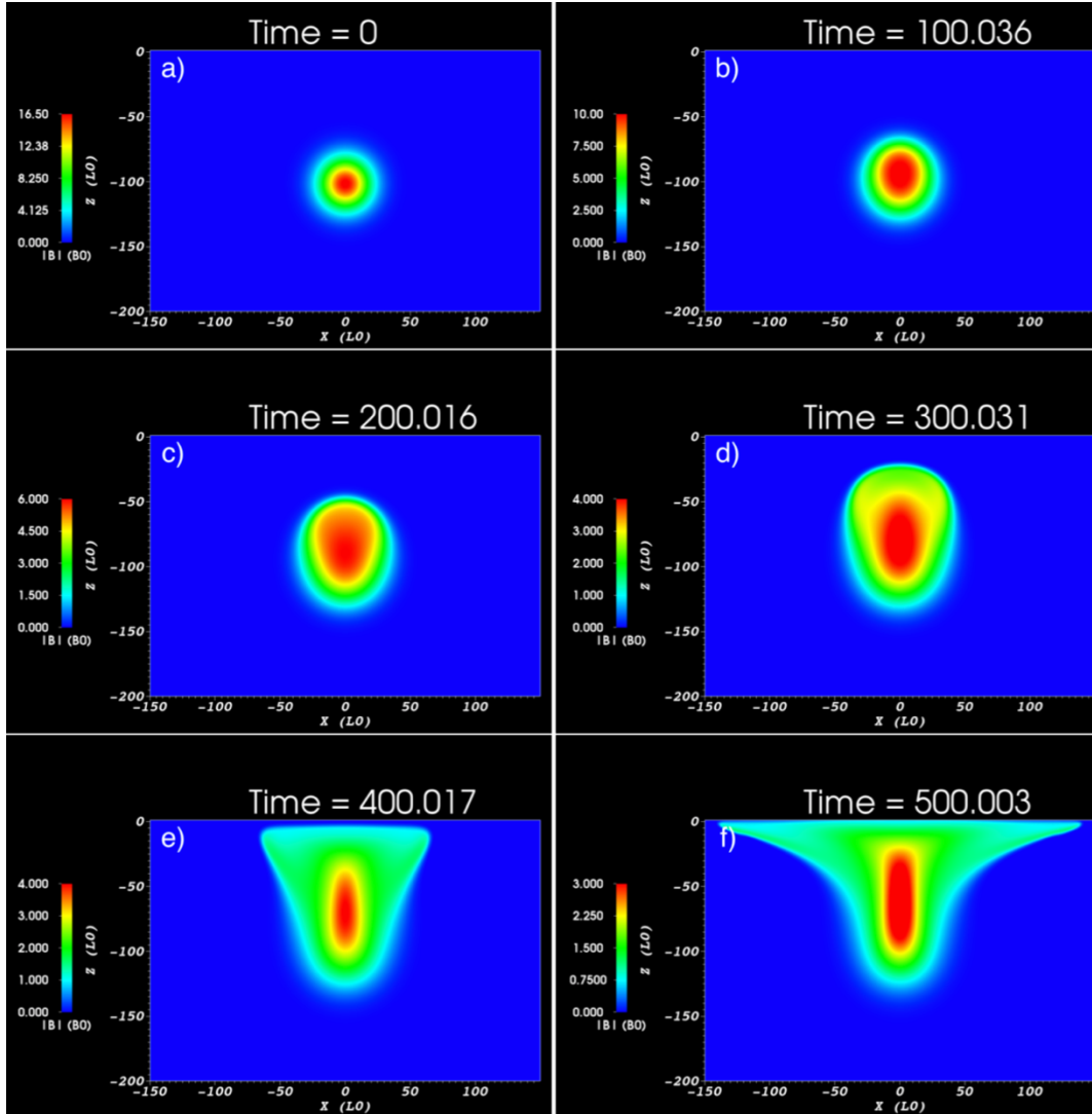
Figure 2 - Contours of magnetic field strength at different times during the simulation in the x-z plane
