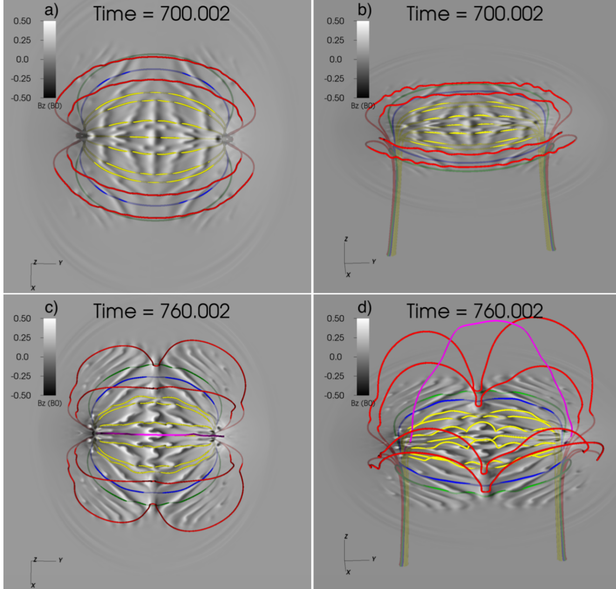
Figure 4 - Field lines, overplotted on maps of the vertical component of the photospheric magnetic field, at various stages of the simulation.
