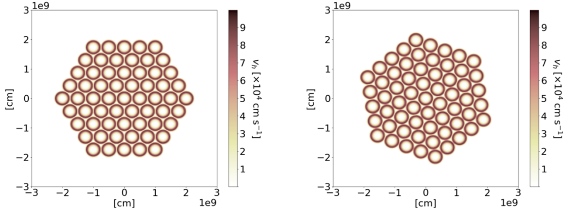
Figure 9 - Azimuthal velocity profile during two rotation cycles of the third simulation
