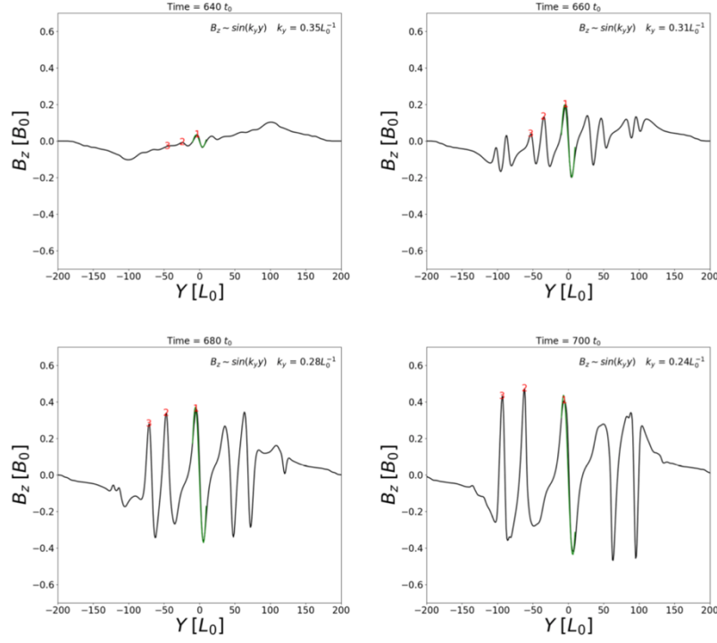
Figure 5 - A cut of the vertical component of the magnetic field taken at x=z=0 at several times during the simulation. The green curve is a portion of a sinusoid fit to the central peak, with fit properties stated in the panel, and the red numbers label the peaks whose amplitude will be studied below in Figure 7.
