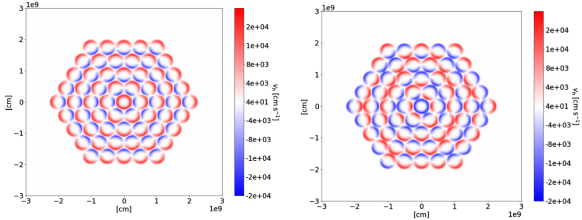
Figure 8 – Azimuthal velocity on the photosphere in the simulations in Knizhnik (2020)
