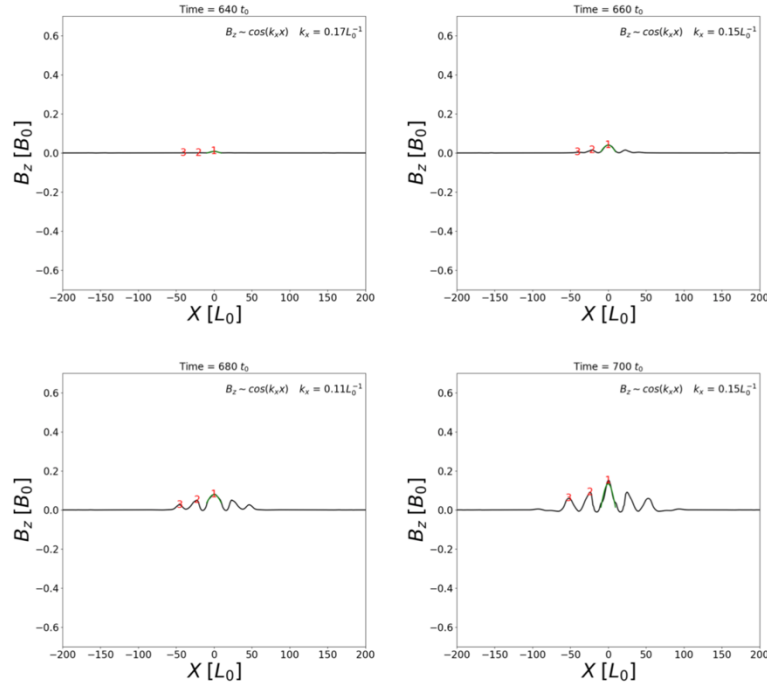
Figure 6 - Same as Figure 5 but at y=z=0 .
