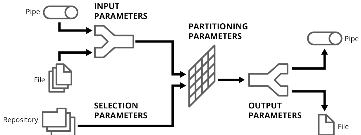
Figure 2.2: rwfilter Parameter Relationships
