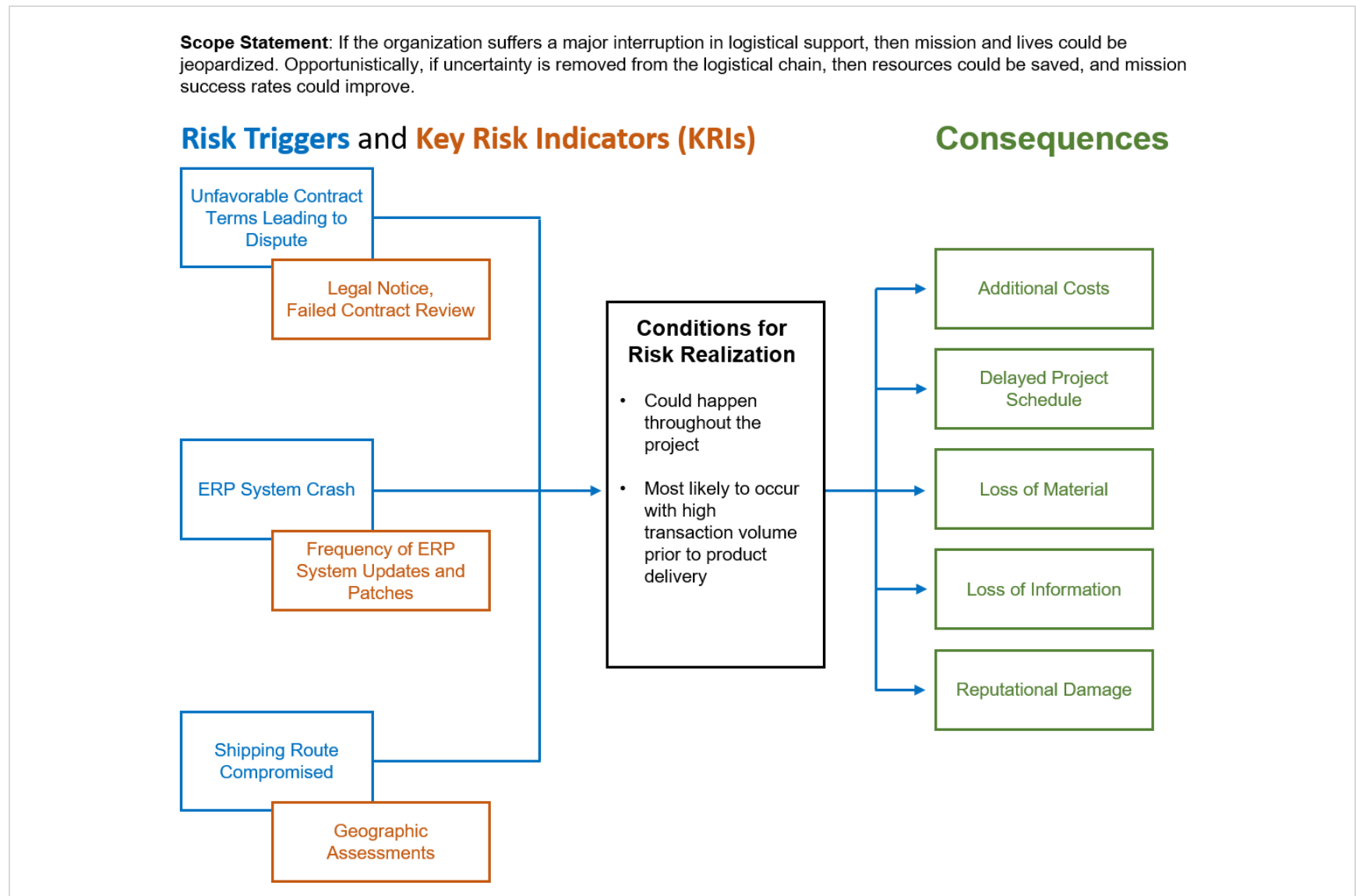
Figure 14: Sample Bow Tie Analysis
