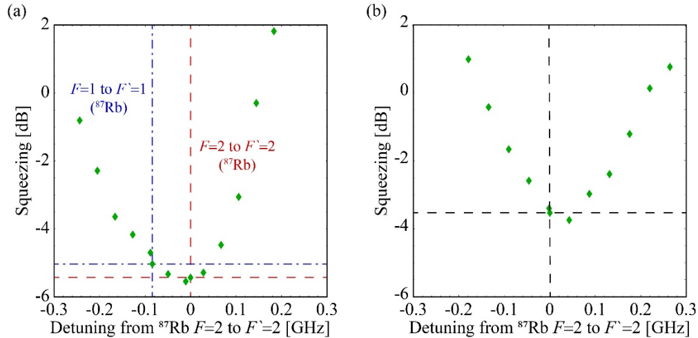
Fig. 2. On-resonance two-mode squeezed states of light. Intensity-difference squeezing measured as a function of the detuning of the probe from the D1 F=2 to F'=2 transition in ^{87}\text{Rb} . (a) Configuration in which either the probe or conjugate is on resonance with a transition in the D1 line of ^{87}\text{Rb} . The vertical and horizontal red dashed (blue dashed-dotted) lines indicate the frequency at which the probe (conjugate) is on resonance and the corresponding level of squeezing, respectively. (b) Configuration in which the probe and conjugate are simultaneously on resonance with transitions in the D1 of ^{87}\text{Rb} . The vertical and horizontal dashed lines indicate the resonance frequency for the probe and conjugate and the corresponding level of squeezing, respectively. Adapted from [1].
