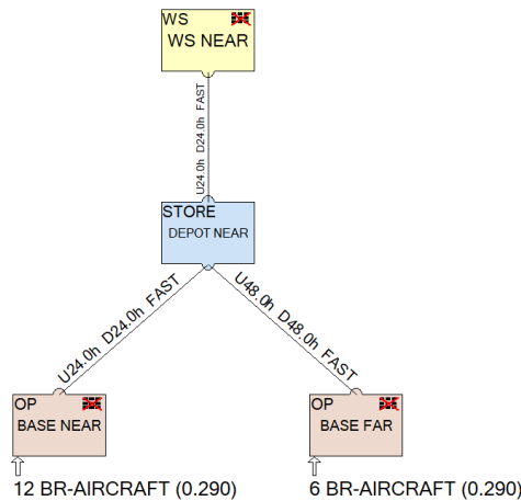
Figure 7. OPUS10 station structure for the first scenario (BLS) - both transportation times (to send and return components) are considered the same
