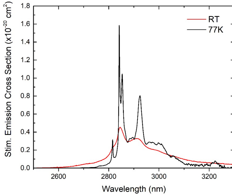
Fig. 10 Stimulated emission cross sections for \text{Dy}^{3+}:\text{BaF}_2 at room temperature and 77 K
