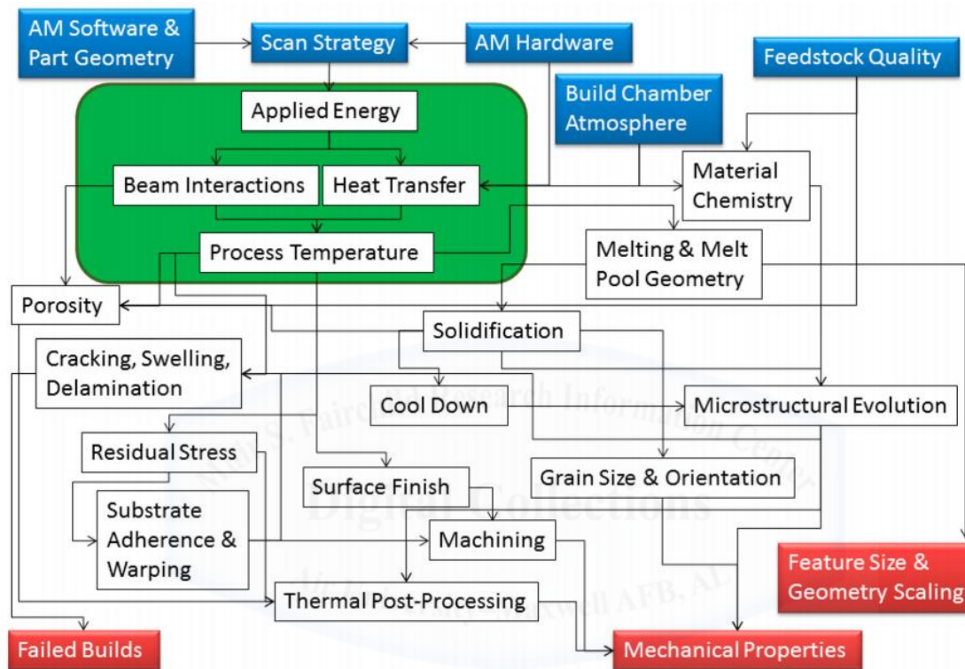
Figure 2: Process map showing complex relationship of AM parameters to outputs 23
