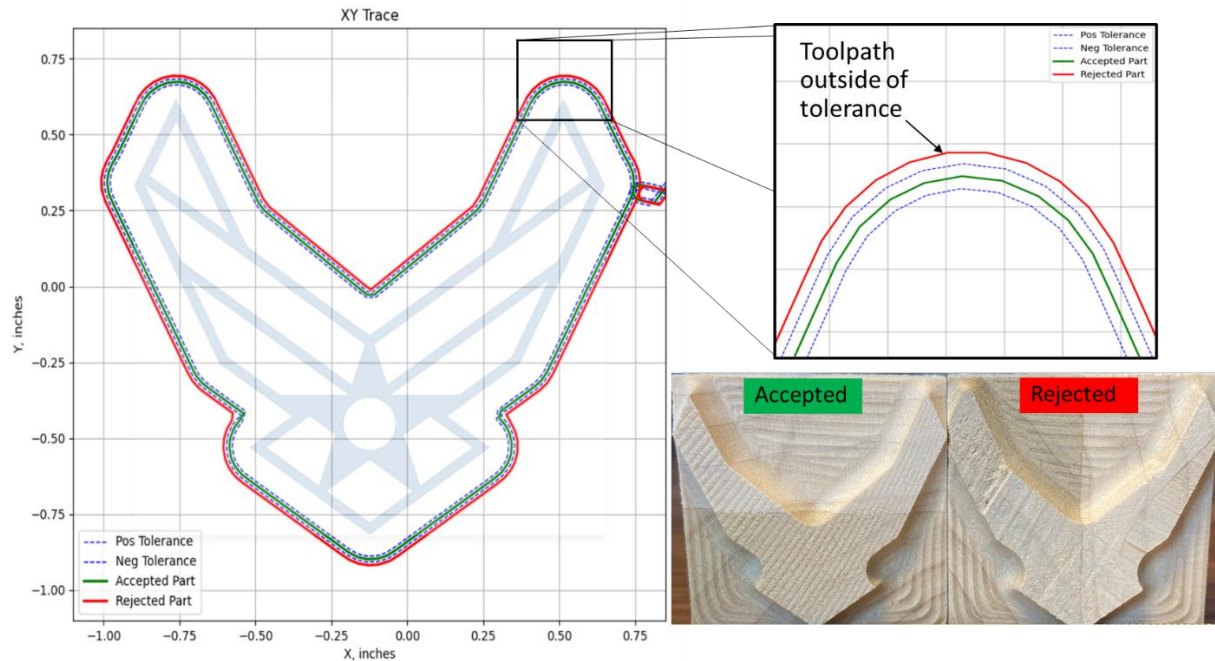
Figure 11: Resulting XY-plane trace and analysis of final contour toolpath
