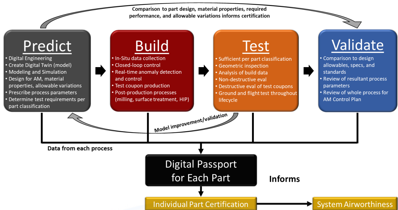
Figure 8: Proposed AM part certification model
