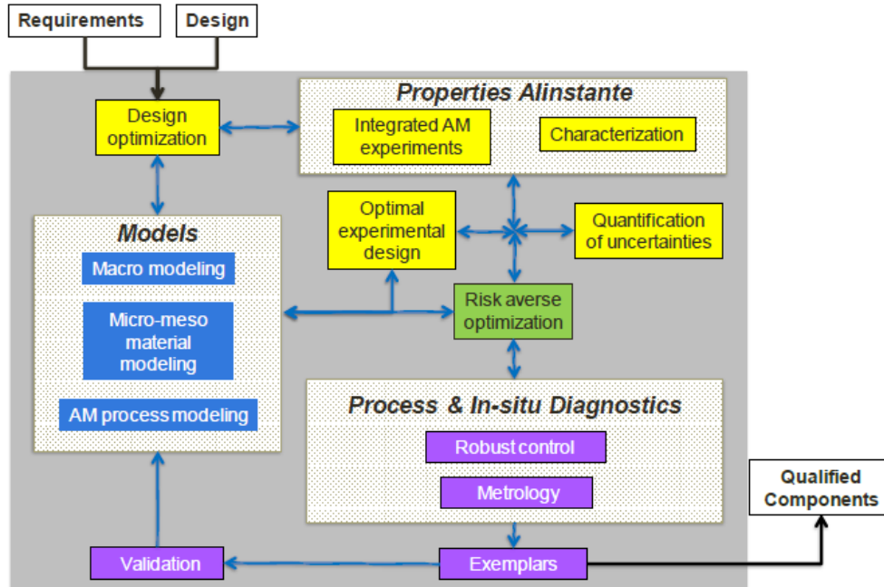
Figure 4: Sandia's Born Qualified Framework 47
