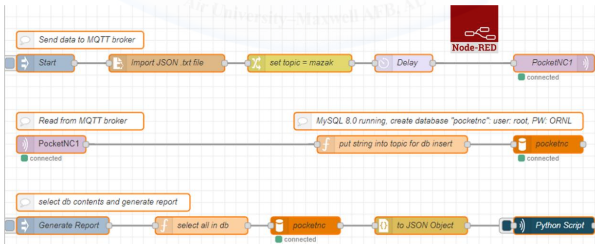
Figure 10: Example Node-RED flow to collect machine data and send for analysis
