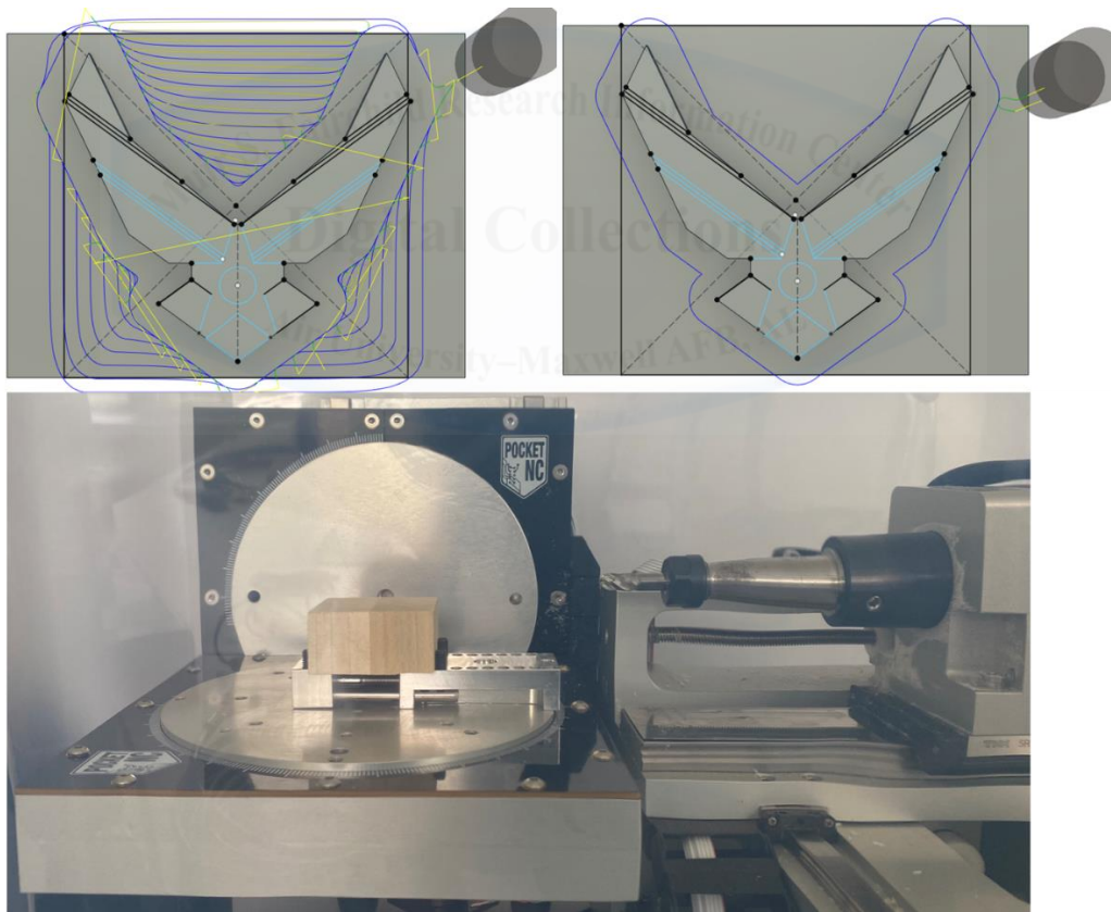
Figure 9: Planned adaptive and contouring toolpath (top) and PocketNC setup (bottom)
