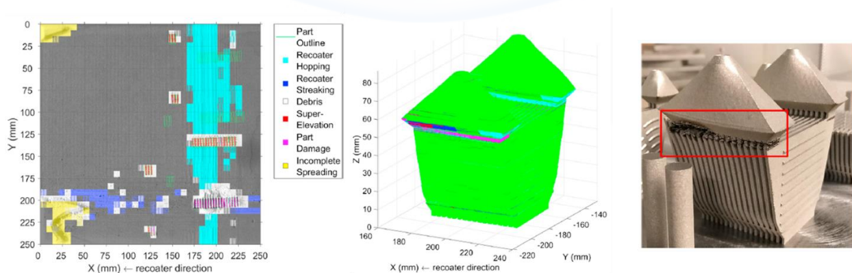
Figure 7: (left to right) An anomaly detection algorithm output of a single spreading layer, a composite model of anomalies in the build volume, and the as-built part with defects visible 69
