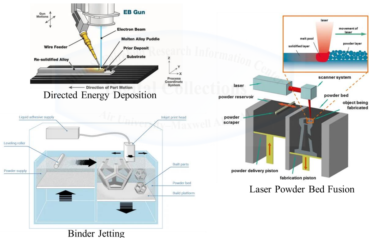
Figure 1: Three common AM techniques for metal part manufacturing 12
