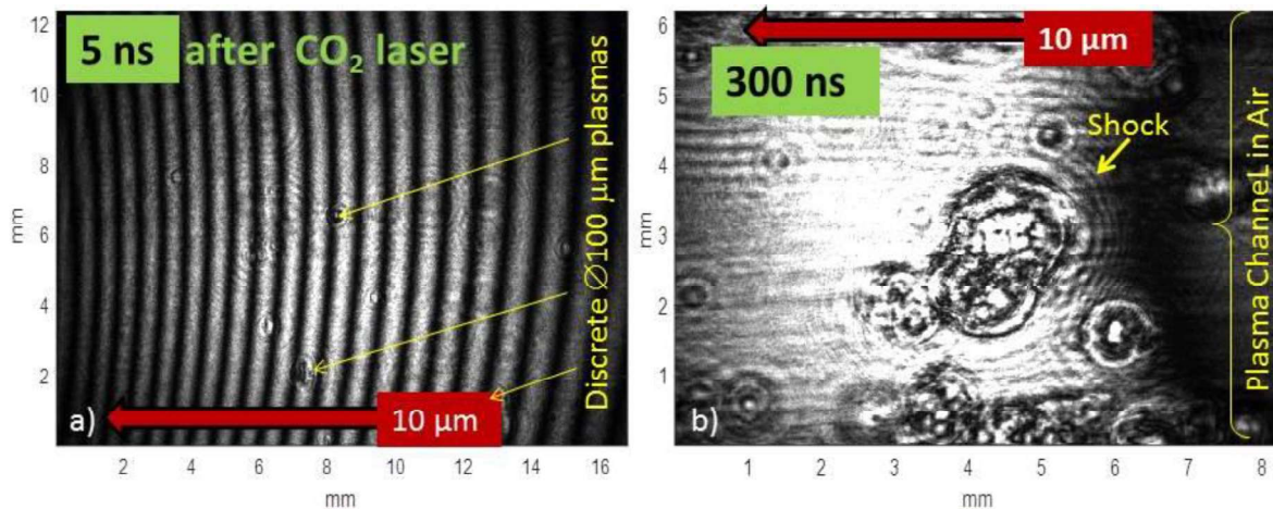
Figure 10. Green pulse interferograms taken at a) 5 ns and b) 300 ns after the multiterawatt CO 2 laser pulse.
