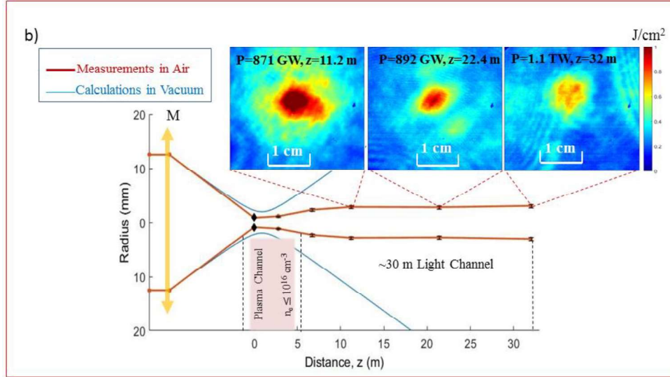
Figure 3. Measurements of spatial evolution of the CO 2 laser beam propagating in air in the range of distances from z = 0 to z = 32 m (red dots) from the nonlinear focus of the mirror, M . Black diamonds indicate laser size measurements in the focus obtained by a thermosensitive paper. The blue lines show the calculated propagation of the Gaussian beam in vacuum. Typical spatial beam profile of the self-channeled \sim 1 TW CO 2 laser at z = 11.2 m, z = 22.4 m, and z = 32 m measured by a two-dimensional pyroelectric array is shown on a side inset.
