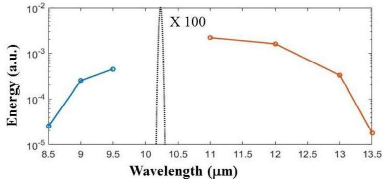
Figure 6. Spectral broadening of an initial 3.5 ps CO 2 laser pulse self-guided in air recorded at z=22.4 m.
