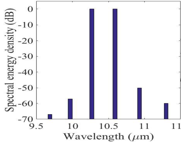
Figure 1. FWM spectrum obtained in laboratory air at an intensity of \sim 15 \text{ GW/cm}^2 .
