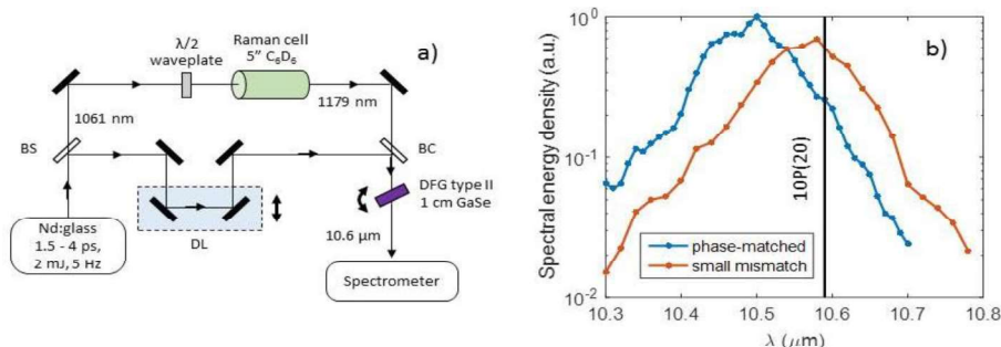
Figure 7. a) Experimental set-up for 10 \mu\text{m} DFG using a 1 \mu\text{m} Nd:glass pump laser and Raman shifter. BS and BC are beam splitter and beam combiner, respectively. b) Measured 10 \mu\text{m} idler spectra when the output is maximized (blue) and slightly detuned from phase-matching to match the 10P(20) CO 2 laser transition at 10.59 \mu\text{m} .
