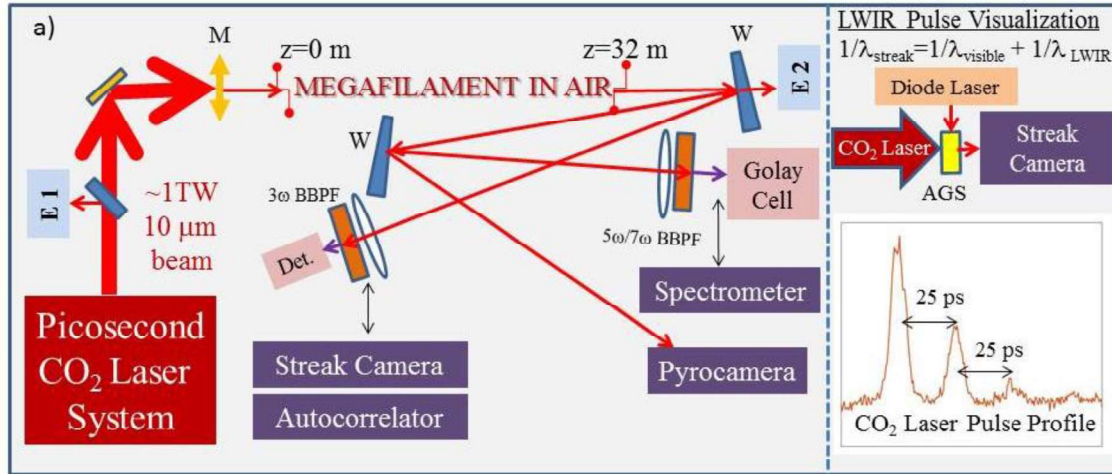
Figure 2. Experimental set-up. The TW CO 2 laser beam was focused by a mirror, M ( f=11\text{m} ) in air with a focus located at z=0 and intercepted at a distance z=2 to 32\text{ m} by a pair of NaCl wedges, W each of which produce two reflected beams with \sim 4\% of the incident energy. Two energy meters E1 and E2 were used to measure energy before and after propagation, respectively. These beams were analyzed by a pyroelectric array of a Pyrocamera and other diagnostics. A grating spectrometer could be replaced by odd-harmonic diagnostic comprised of broadband pass filters (BBPF) centered at 3\omega - 3.41\text{ }\mu\text{m} , 5\omega - 2.04\text{ }\mu\text{m} , or 7\omega - 1.46\text{ }\mu\text{m} of the CO 2 laser and either a calorimeter detector, \text{Det.} for 3\omega or a Golay cell for 5\omega and 7\omega measurements. Alternatively the CO 2 laser pulse was sent to a streak camera or a single-shot autocorrelator for pulse profile measurements. Right hand panel describes the visualization technique via sum frequency mixing of a red diode laser and 10\text{ }\mu\text{m} beams in a \text{AgGaS}_2 nonlinear crystal (AGS). The typical measured CO 2 laser pulse consisted of a leading \sim 1\text{TW} power picosecond pulse and postpulses separated from the first pulse by a 25\text{ ps} period.
