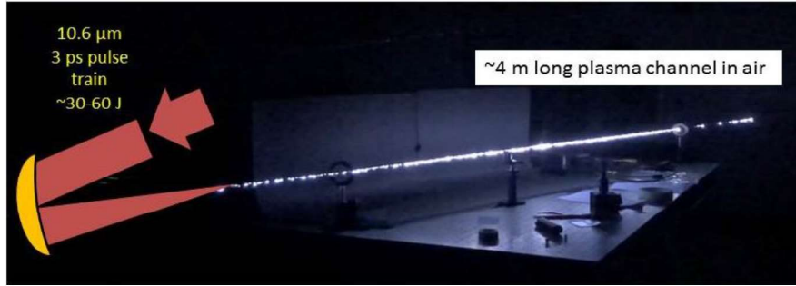
Figure 9. A CCD camera image of the many meter long plasma formed in air by focusing of the multiterawatt \text{CO}_2 laser beam at the UCLA Neptune Lab.
