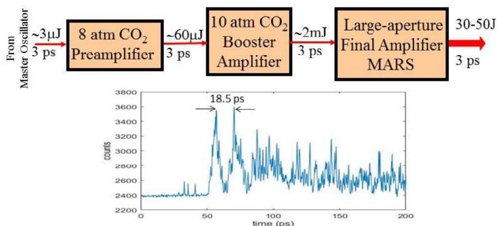
Figure 8. Simplified optical schematic of a picosecond CO 2 laser chain built at the UCLA Neptune Laboratory and a typical pulse profile as measured by a streak camera for 2 mJ pulse output of the Booster amplifier.
