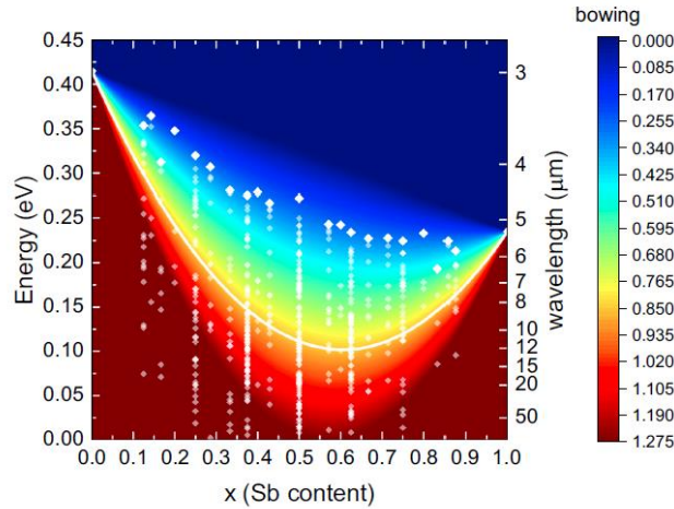
Figure 1 - Band gap values obtained by the PBE- modified Becke-Johnson exchange potential calculations for the different atomic configurations using supercells of up to 16 atoms. The color map illustrates the different bowing parameters as a guide to the eye.
