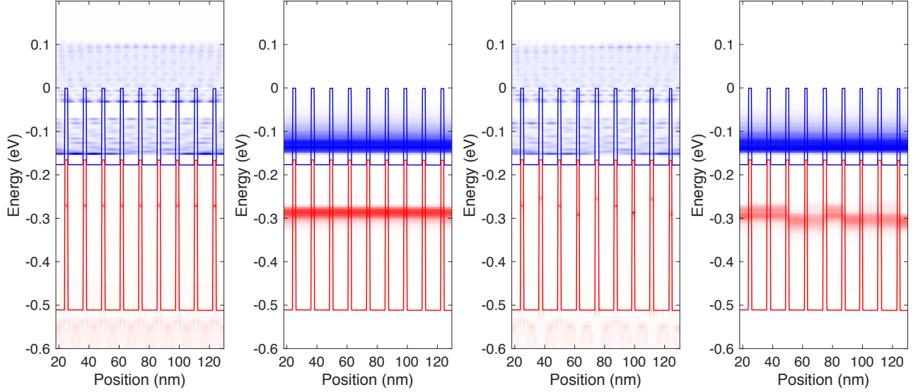
FIG. 5. Local density of states shown for \vec{k} = 0 , computed for the ordered (a) and disordered SL (c). The applied electric field is F = 0.1 kV/cm. The first valence miniband (the sharp red peaks in the LDOS) is strongly localized in both energy and space; energy alignments are severely disrupted by the disorder, while the wider conduction minibands are not visibly affected, suggesting that hole transport is likely to be more sensitive to disorder. This is confirmed by the spatially-resolved current spectrum shown in the ordered (b) and disordered (d) structure. The energy-integrated current drops by approximately one order of magnitude in the presence of geometrical fluctuations at T = 200 K.
