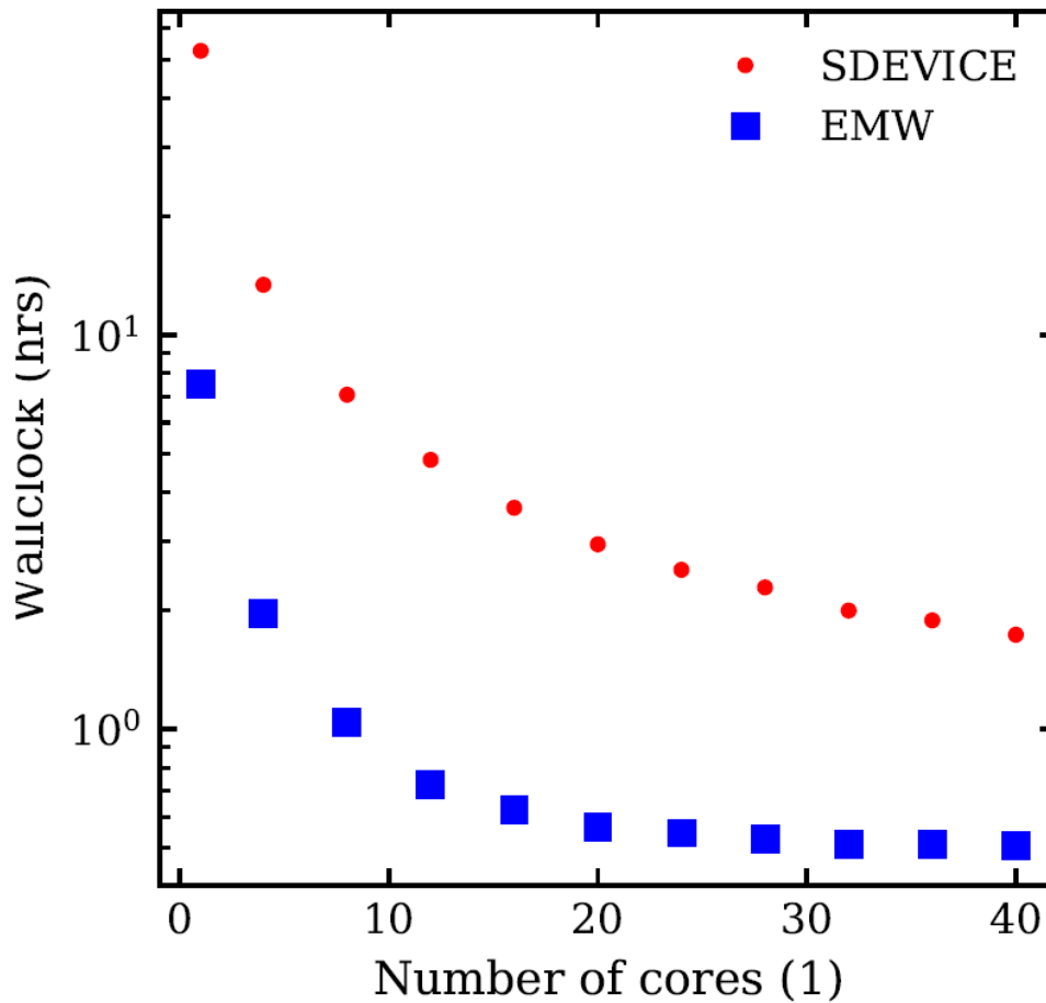
Figure 11 - Wall clock time required for a steady-state solution as a function of the number of cores used.
