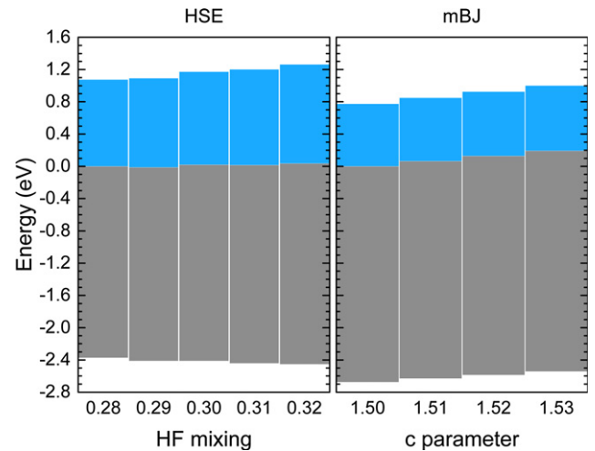
Figure 5. The effect of a variable Hartree–Fock mixing (HSE) and c (mBJ) parameter on the branch point energy of GaN. The first branch point energy of each method is set to 0 eV for convenience. The blue and gray boxes indicate the difference from the branch point energy to the conduction and valence band edge, respectively.
