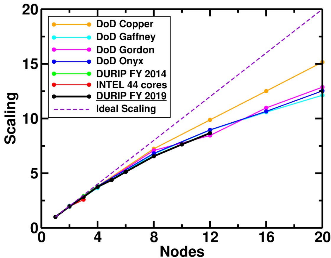
Figure 6 – Scaling for a 96 atom system with increasing the number of nodes.
