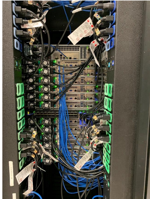
Figure-5(b) Rear view of the cluster installed in the rack. The blue cables are for the 10Gb Ethernet, the black cable on the right of the servers are for the EDR InfiniBand.
