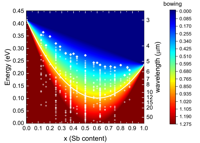
FIG. 3. Band gap values obtained by the PBEmBJ calculations for the different atomic configurations using supercells of up to 16 atoms. The color map illustrates the different bowing parameters as a guide to the eye.
