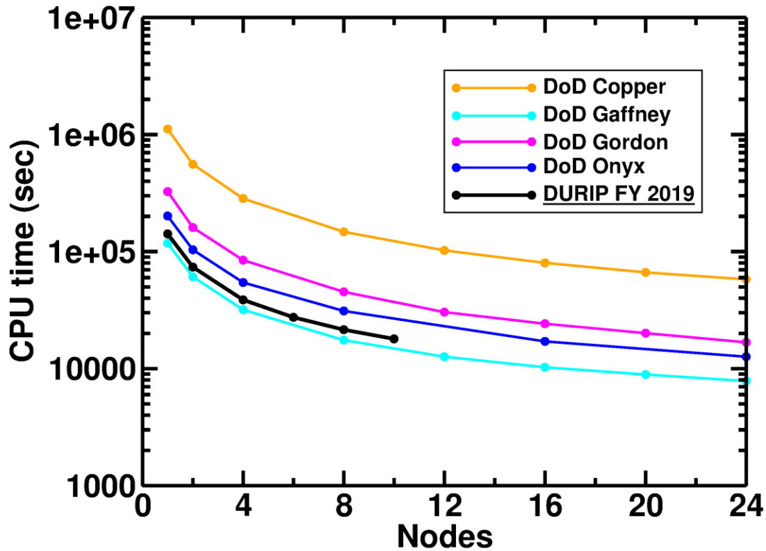
Figure 9 - EPW calculations. Speed up in CPU time (in seconds) with increasing the number of nodes.
