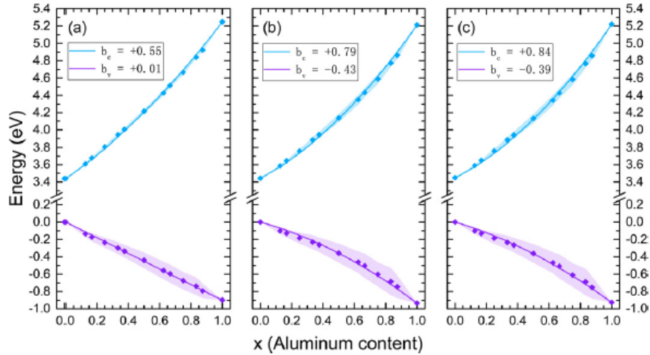
Figure 2 - The band offsets of the alloys obtained by (a) HSE calculations, as well as mBJ calculations with (b) an optimal and (c) a species-specific c parameter. The legends indicate the bowing parameter of the valence and conduction band edges. The valence band edge of GaN is set to 0 eV for convenience.
