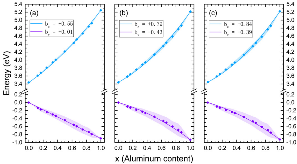
Figure 3. The band offsets of the alloys obtained by (a) HSE calculations, as well as mBJ calculations with (b) an optimal and (c) a species-specific c parameter. The legends indicate the bowing parameter of the valence and conduction band edges. The valence band edge of GaN is set to 0 eV for convenience.
