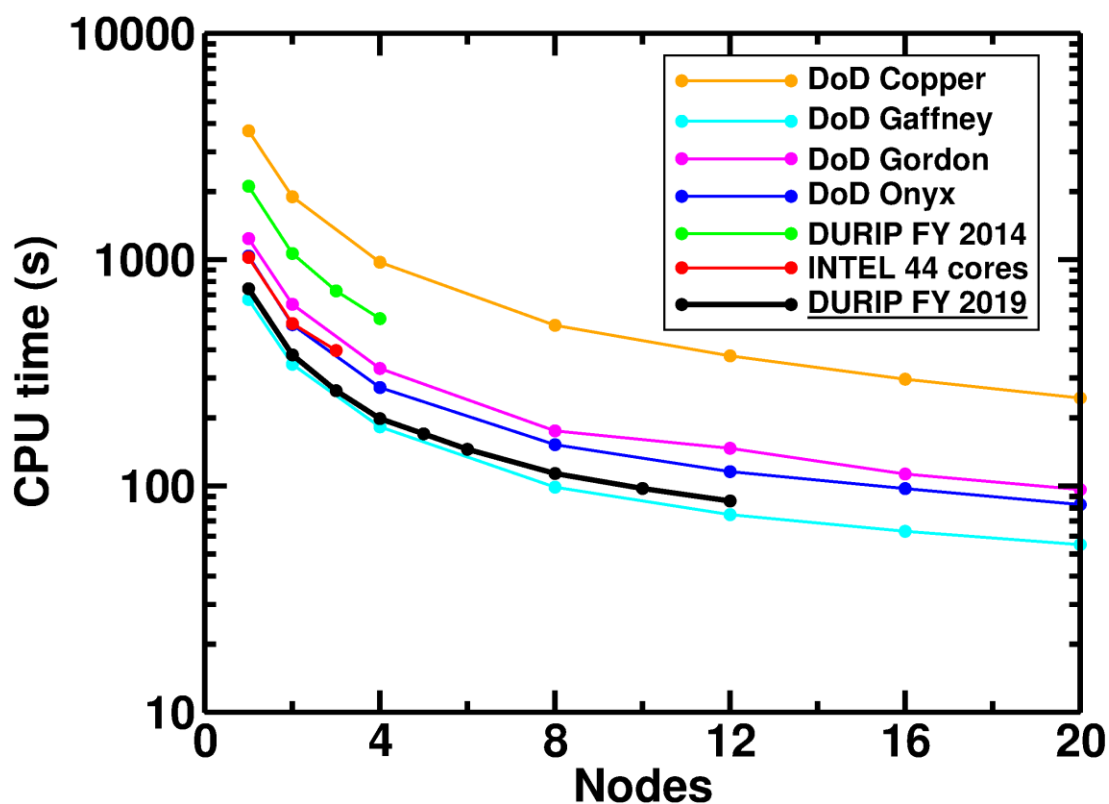
Figure 5 – Execution speed for a 96 atom system. Speed up in CPU time (in seconds) with increasing the number of nodes.
