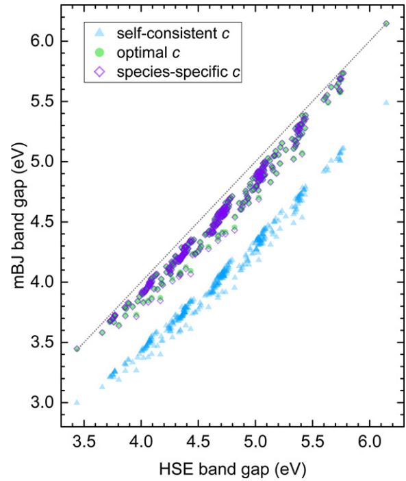
Figure 2. The mBJ values of the band gaps obtained by a self-consistent, optimal, and species-specific c parameter, compared to the values obtained by HSE calculations.
