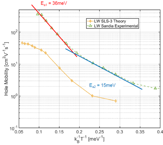
Figure 3(a) – Calculated hole mobility as a function of the temperature (yellow line). Measured hole mobility for a similar LWIR Type-II SLS (green line).
