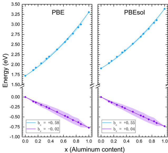
Figure 4. The band offsets of the alloys obtained by PBE and PBEsol calculations. The legends indicate the bowing parameter of the valence and conduction band edges. The valence band edge of GaN is set to 0 eV for convenience.
