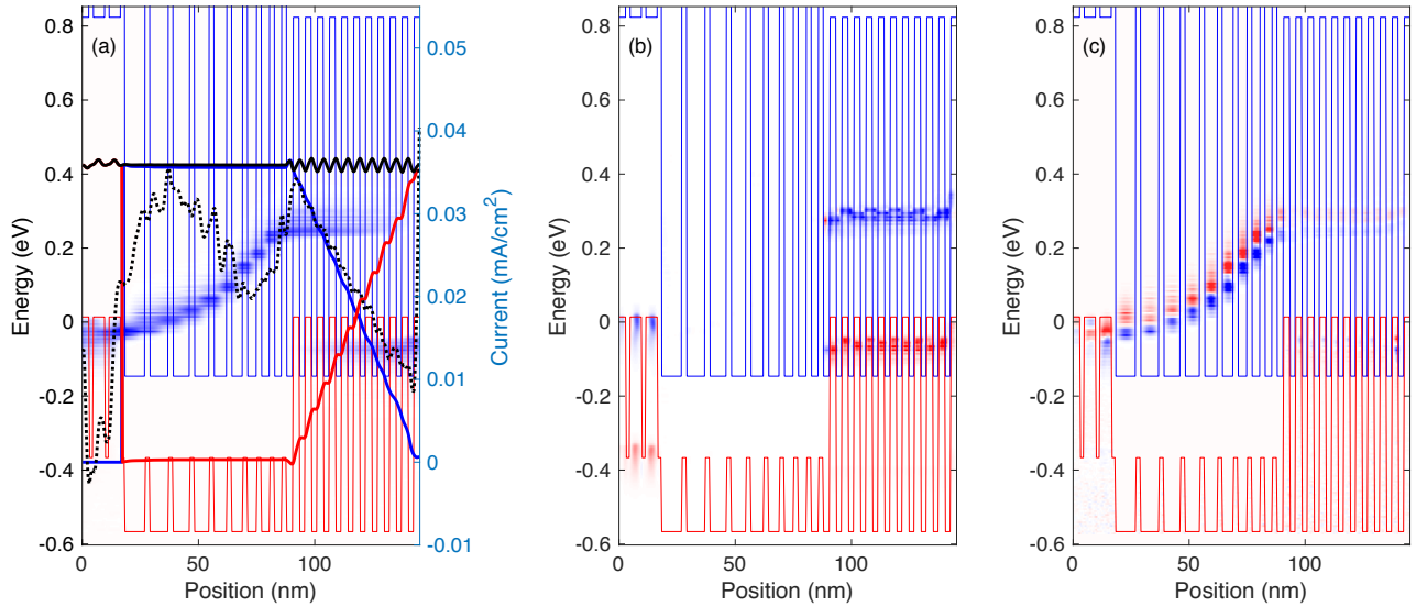
FIG. 2. (a) Spatially resolved photocurrent spectrum under a monochromatic illumination of 1 \text{ W/m}^2 with E_\gamma = 0.3 \text{ eV} (color maps). The corresponding energy-integrated current (black solid line, right axis) is approximately conserved, save for small oscillations due to the incompleteness of the basis set. Blue and red lines indicate electron and hole contributions, respectively. A position-dependent energy threshold was defined according to the local density of states to separate electron and hole contributions (solid blue and red lines, respectively). Current conservation is clearly violated if the contribution of the remote modes is neglected (black dotted line). (b) Spatially resolved radiative generation spectrum (color maps). (c) Spectral scattering current due to coupling to polar optical phonons,[53] showing the relaxation of the carriers (positive/negative values, i.e., in/out-scattering of electrons, have a gradient from white to blue/red).
