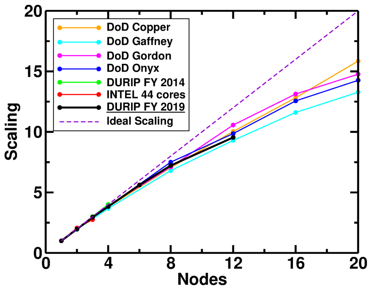
Figure 8 – Scaling for a 192 atom system with increasing the number of nodes.
