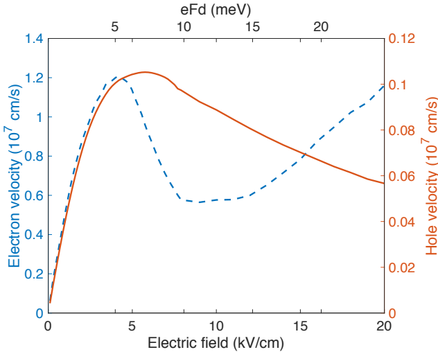
FIG. 6. Electron (left axis, dashed blue curve) and hole (right axis, solid red curve) velocity as a function of the applied electric field (lower axis) and of the potential drop per period eFd (upper axis), at T = 200 K.
