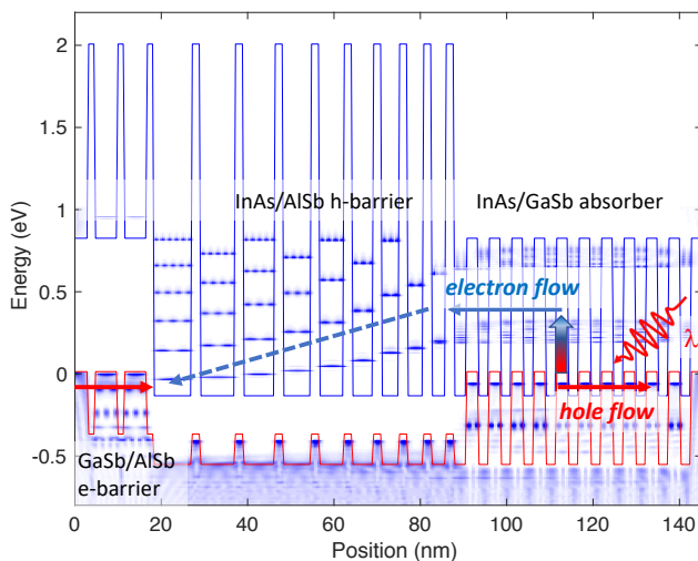
FIG. 1. Local density of states of one stage of a mid-wavelength infrared (MWIR) interband cascade photodetector shown for \vec{k} = 0 (color maps). The arrows indicate the direction of the electron and hole flow: the electron-hole pairs photogenerated in the superlattice absorber diffuse along the respective minibands, the electrons towards the hole barrier, where they relax by polar optical transitions down a Wannier-Stark ladder, until they reach the electron barrier, whereupon they tunnel into the valence miniband of the adjacent stage.
