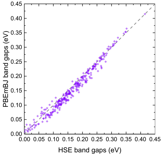
FIG. 2. Comparison of the band gaps obtained by the HSE and PBEmBJ calculations in a subset of 290 atomic configurations.
