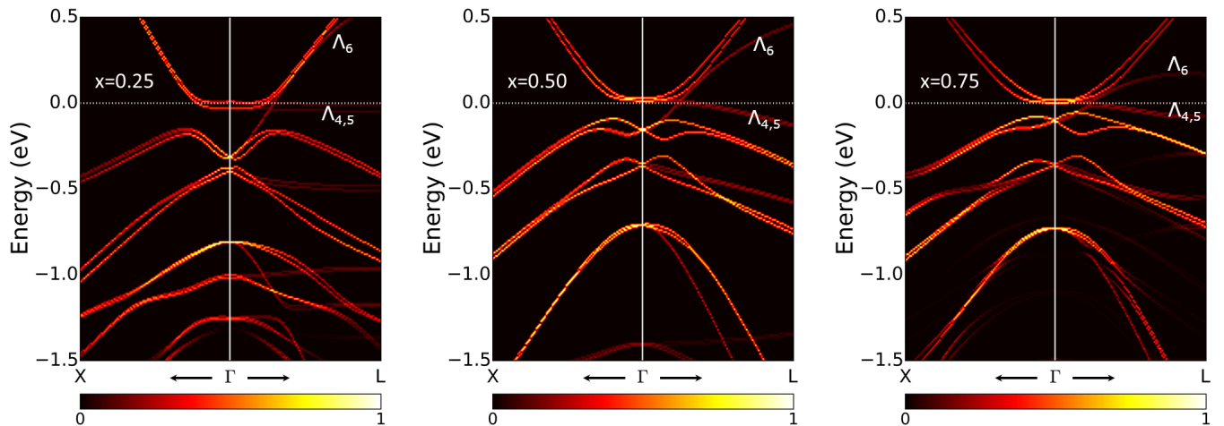
FIG. 5. The effective band structures obtained by the PBE em BJ calculations for the CuPt-ordered alloys with 25%, 50%, and 75% Sb content, around the \Gamma point ( |\mathbf{k}| \leq 0.25 \text{ \AA}^{-1} ). The spectral weights are normalized to one.
