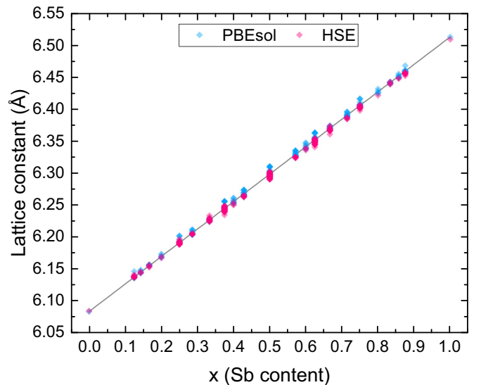
FIG. 1. The lattice constants of the InAsSb alloys for different compositions obtained by calculations using the PBEsol and HSE functionals.
