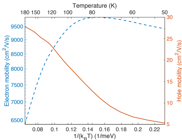
FIG. 7. Electron (left axis, dashed blue curve) and hole (right axis, solid red curve) mobility of the disordered SL as a function of inverse temperature, computed for an electric field of 0.1 kV/cm.
