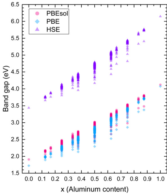
Figure 1. The band gaps of the alloys obtained by HSE, PBE, and PBEsol calculations.
