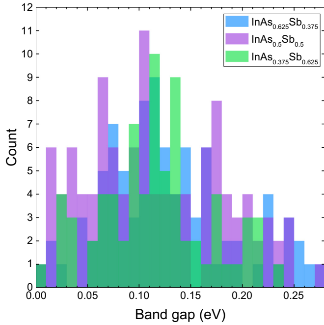
FIG. 4. The frequency of the band gaps for the compositions of 37.5%, 50%, and 62.5% of Sb content.
