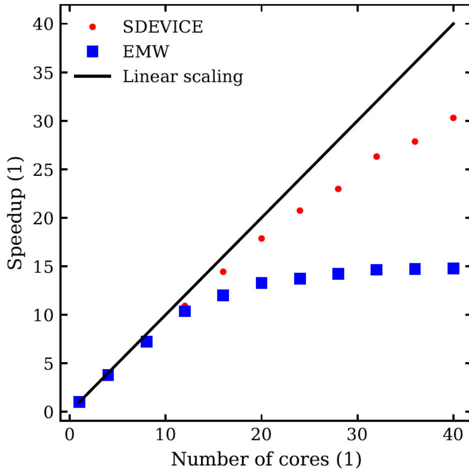
Figure 12 - Speedup performance for a steady-state solution as a function of the number of cores used.
