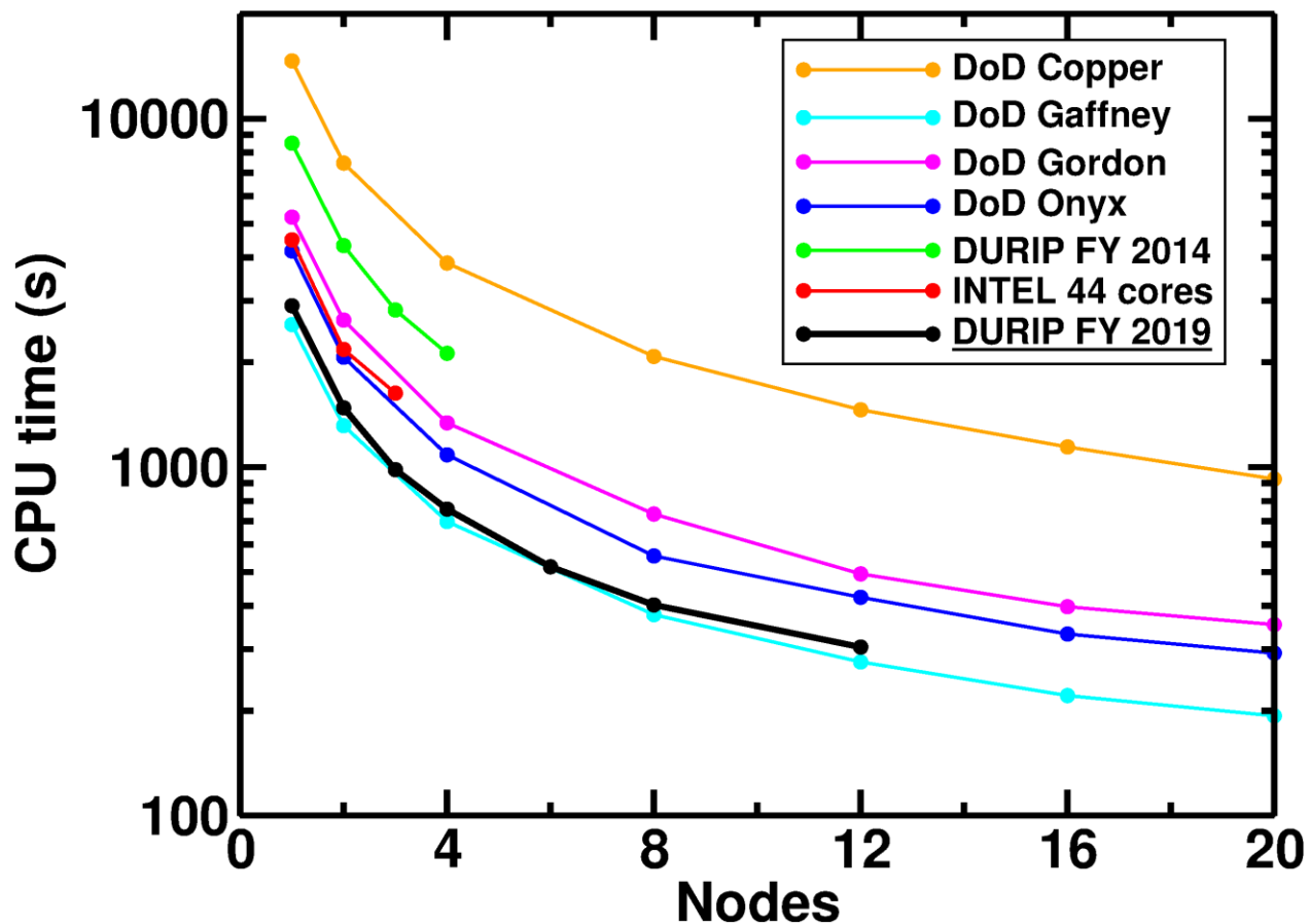
Figure 7 – Execution speed 192 atom system. Speed up in CPU time (in seconds) with increasing the number of nodes
