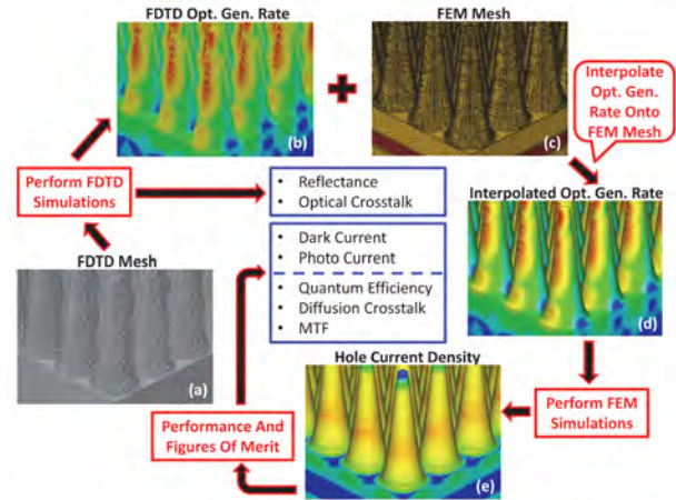
Fig. 1. Overview of modeling steps. Input and output of individual steps include, but are not limited to (a) FDTD structured tensor mesh, (b) optical generation rate saved onto FDTD mesh, (c) FEM unstructured mixed element mesh, (d) optical generation rate interpolated from FDTD mesh onto FEM mesh and (e) hole current density.
