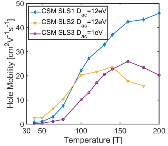
Figure 3(b) – Calculated hole mobility as a function of the temperature for three different random SLS configurations.
