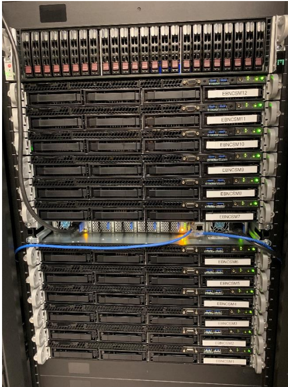
Figure-4(a) Front view of the cluster installed in the rack. From the top we have: the file server, six compute nodes, the EDR 100Gb InfiniBand switch, and six more computer nodes.
