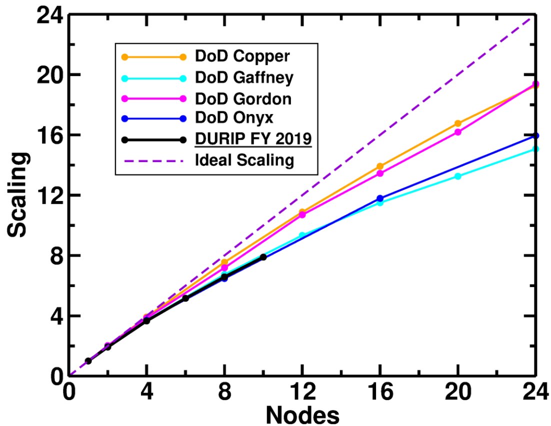
Figure 10 - EPW calculations. Scaling with increasing the number of nodes.
