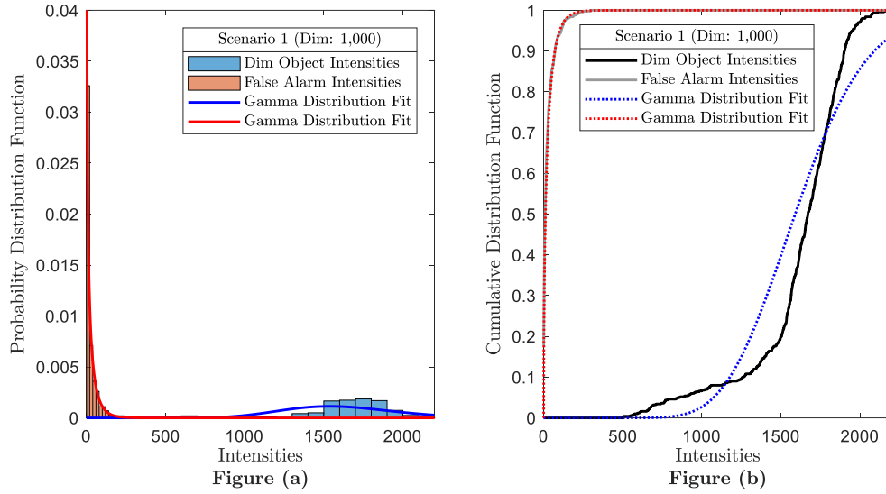
Figure 3.13. The distributions of the intensities of the dim object and the false alarm pixel for Scenario 1 using the MFBF approach.
