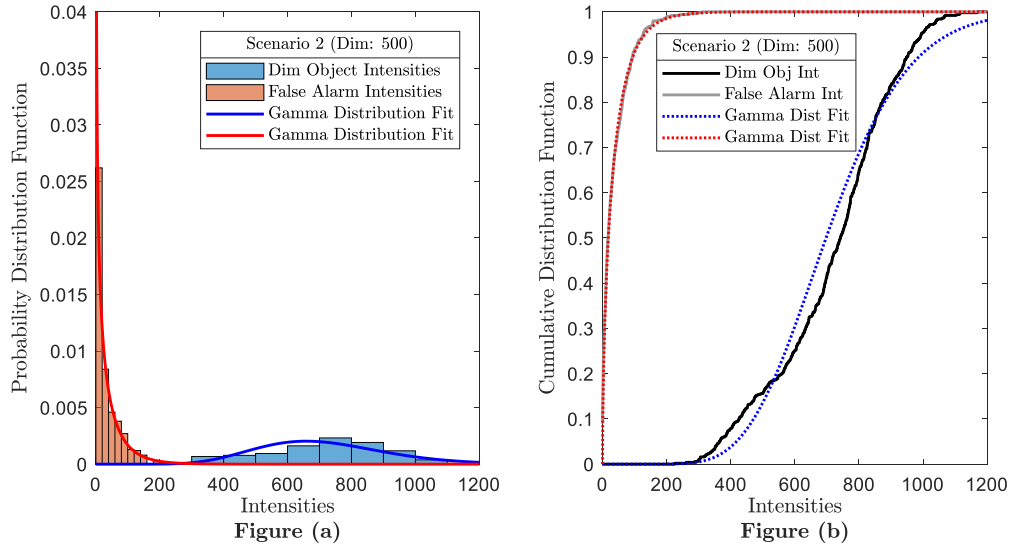
Figure 3.14. The distributions of the intensities of the dim object and the false alarm pixel for Scenario 2 using the MFBF approach.
