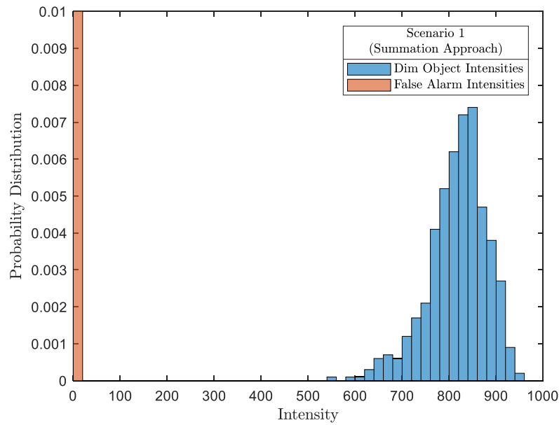
Figure D-1. The Distributions for Dim Object Intensities and False Alarm Intensities for Scenario 1 Using DRBD with Summation Approach.
