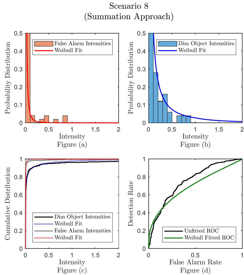
Figure D-5. The Weibull Fitted Distributions for Dim Object Intensities and False Alarm Intensities for Scenario 8 Using DRBD with the Summation Approach.
